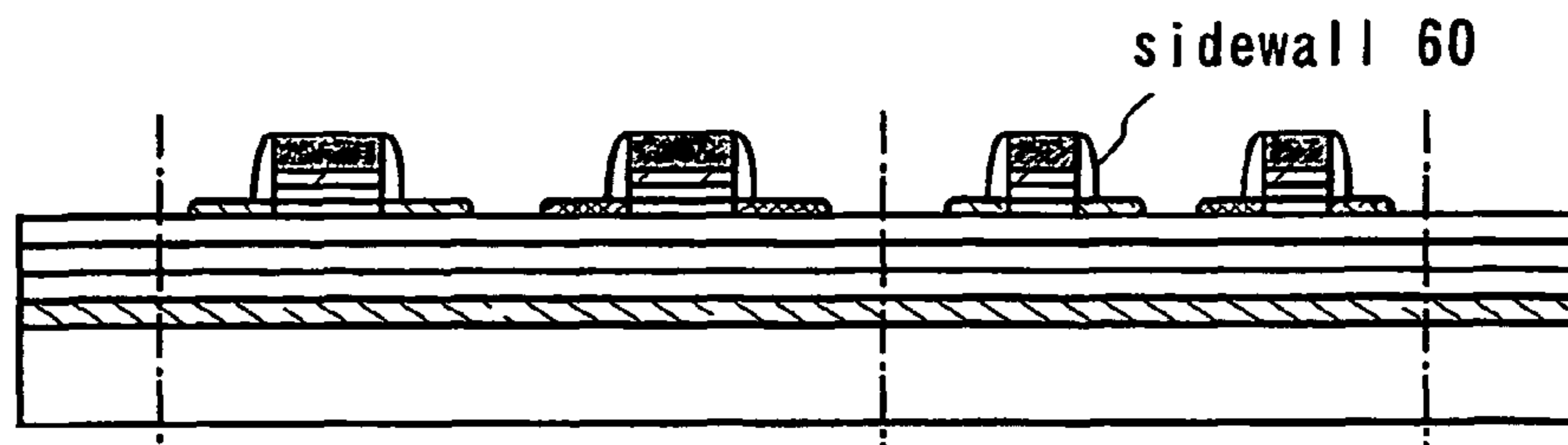
FIG. 8G etchback (forming sidewall)
