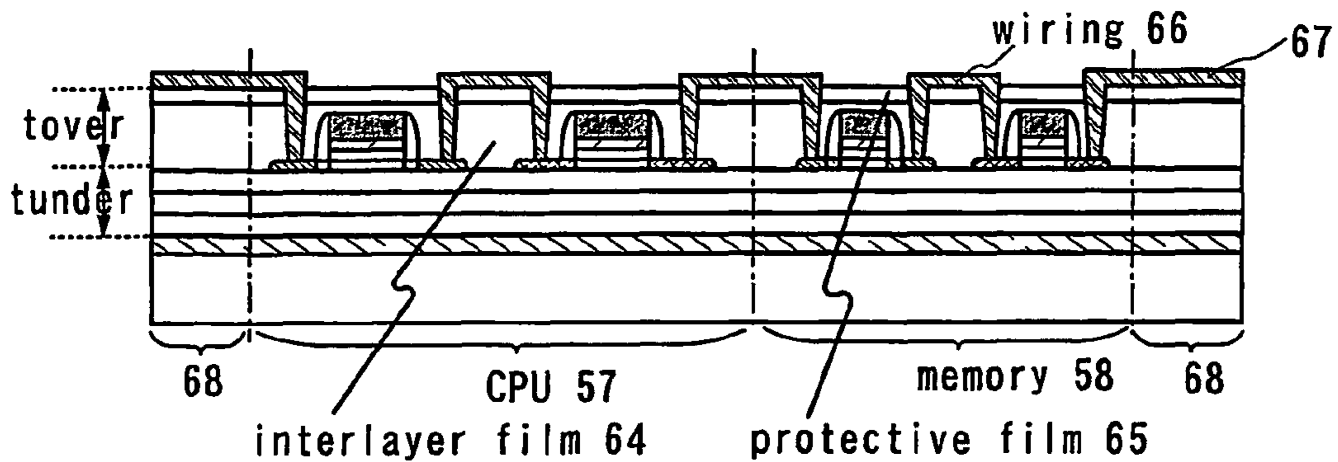
FIG. 8I forming interlayer, protective film and wiring
