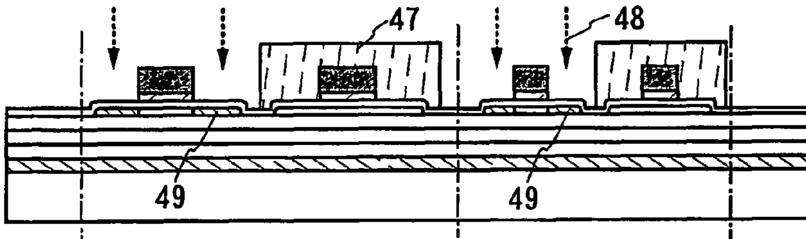
FIG. 7D forming n-type low concentration impurity region
