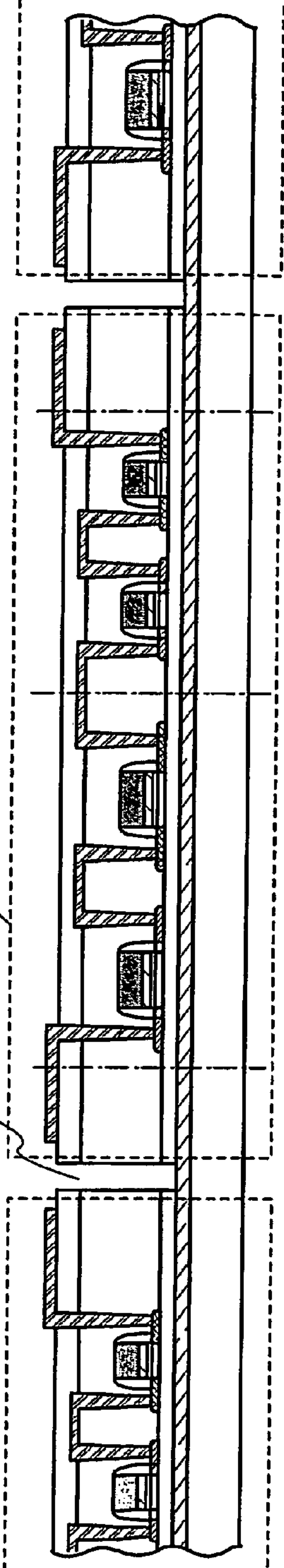
FIG. 9K forming groove 70 thin film integrated circuit portion 69
