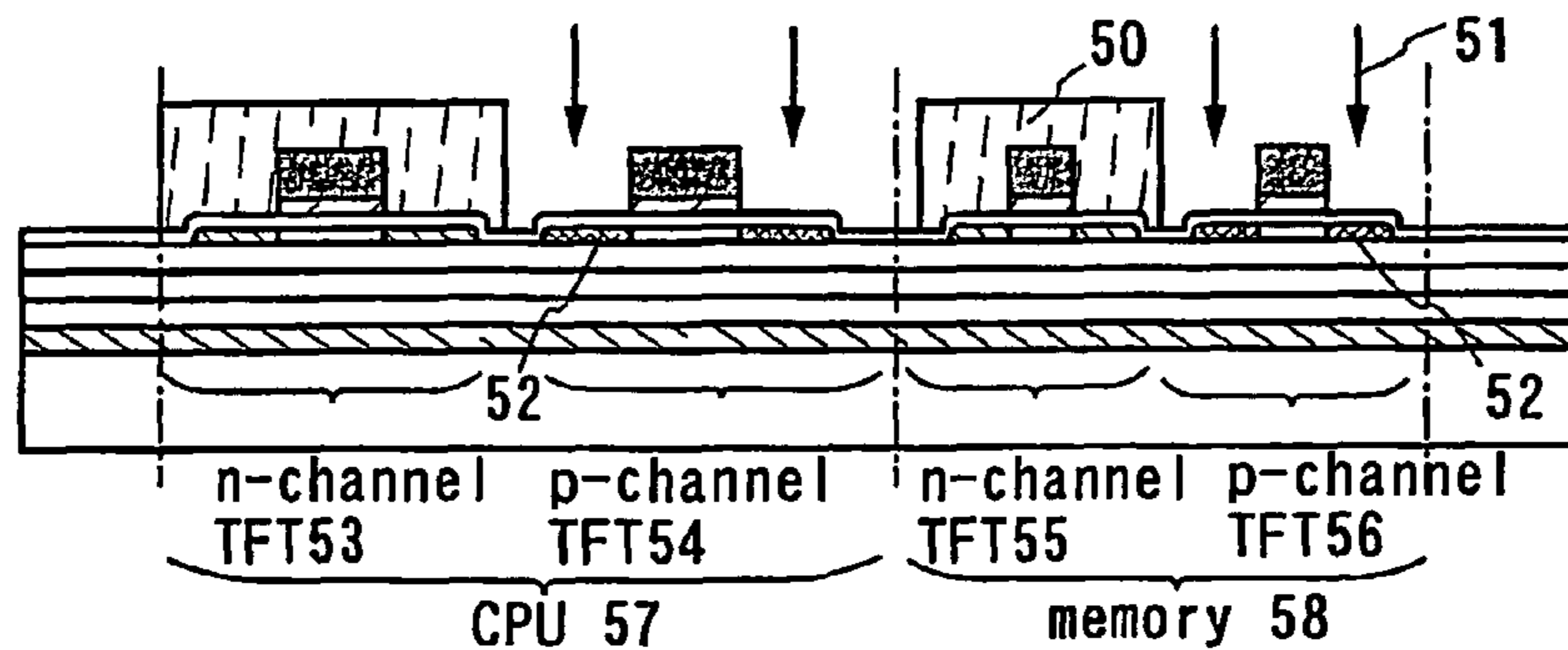
FIG. 7E forming p-type high concentration impurity region
