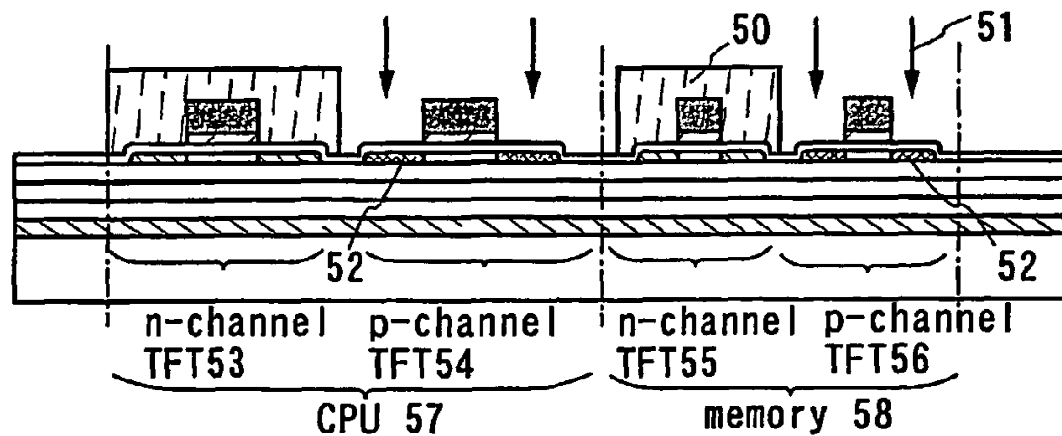
FIG. 7E forming p-type high concentration impurity region
