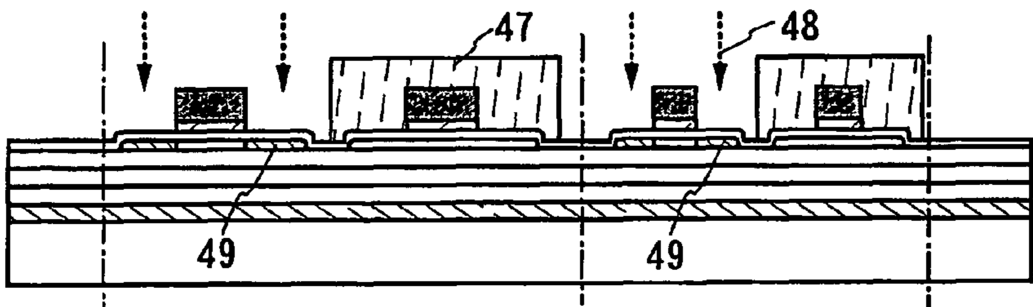
FIG. 7D forming n-type low concentration impurity region
