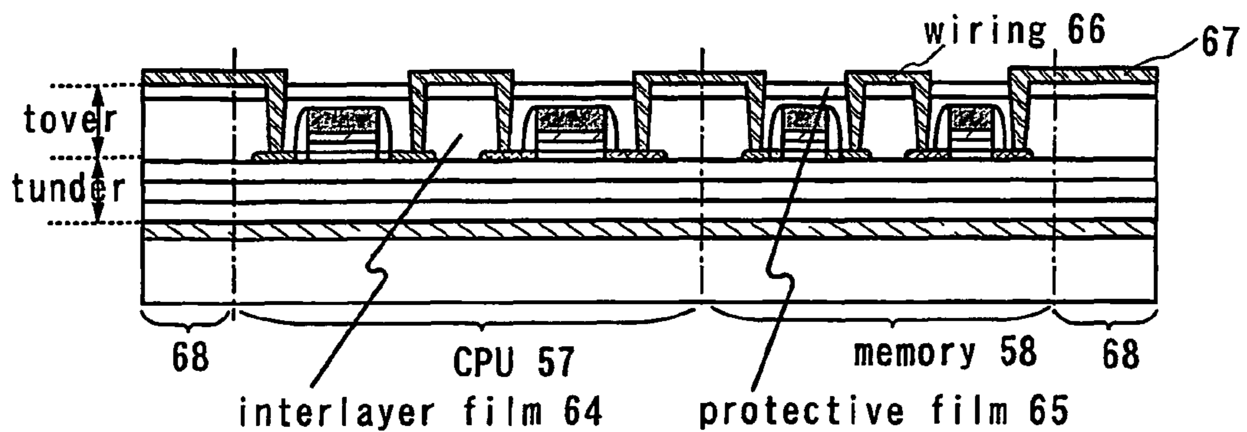
FIG. 8I forming interlayer, protective film and wiring
