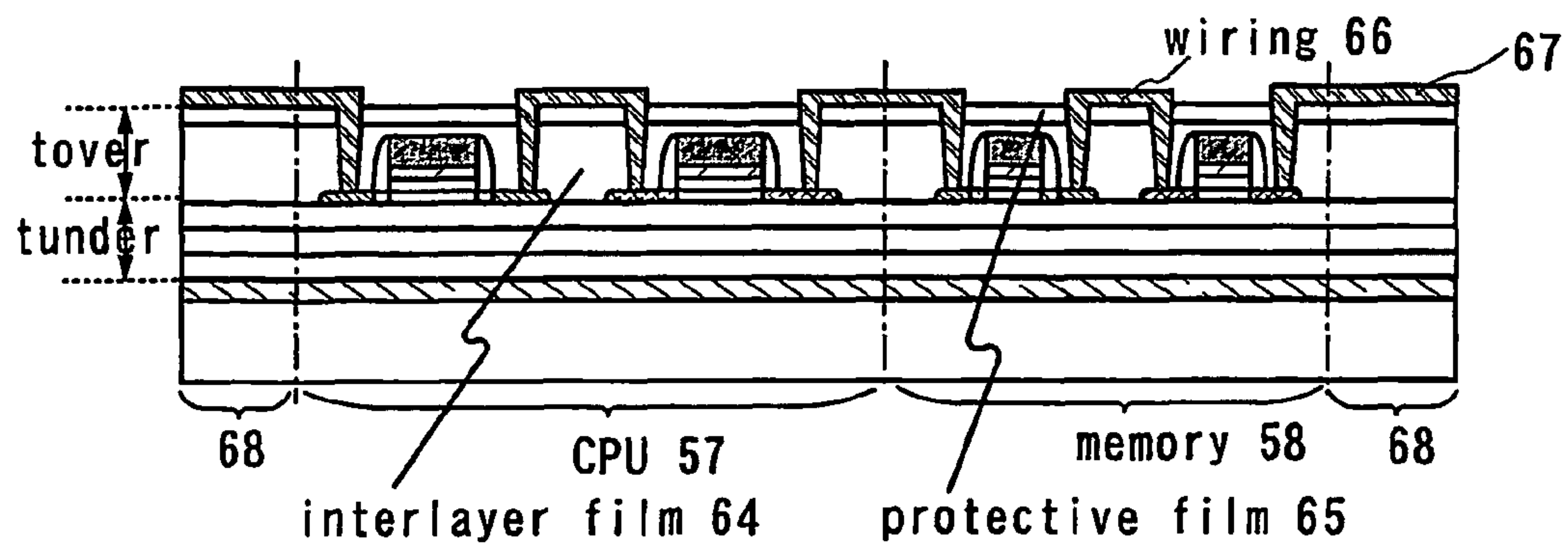
FIG. 81 forming interlayer, protective film and wiring
