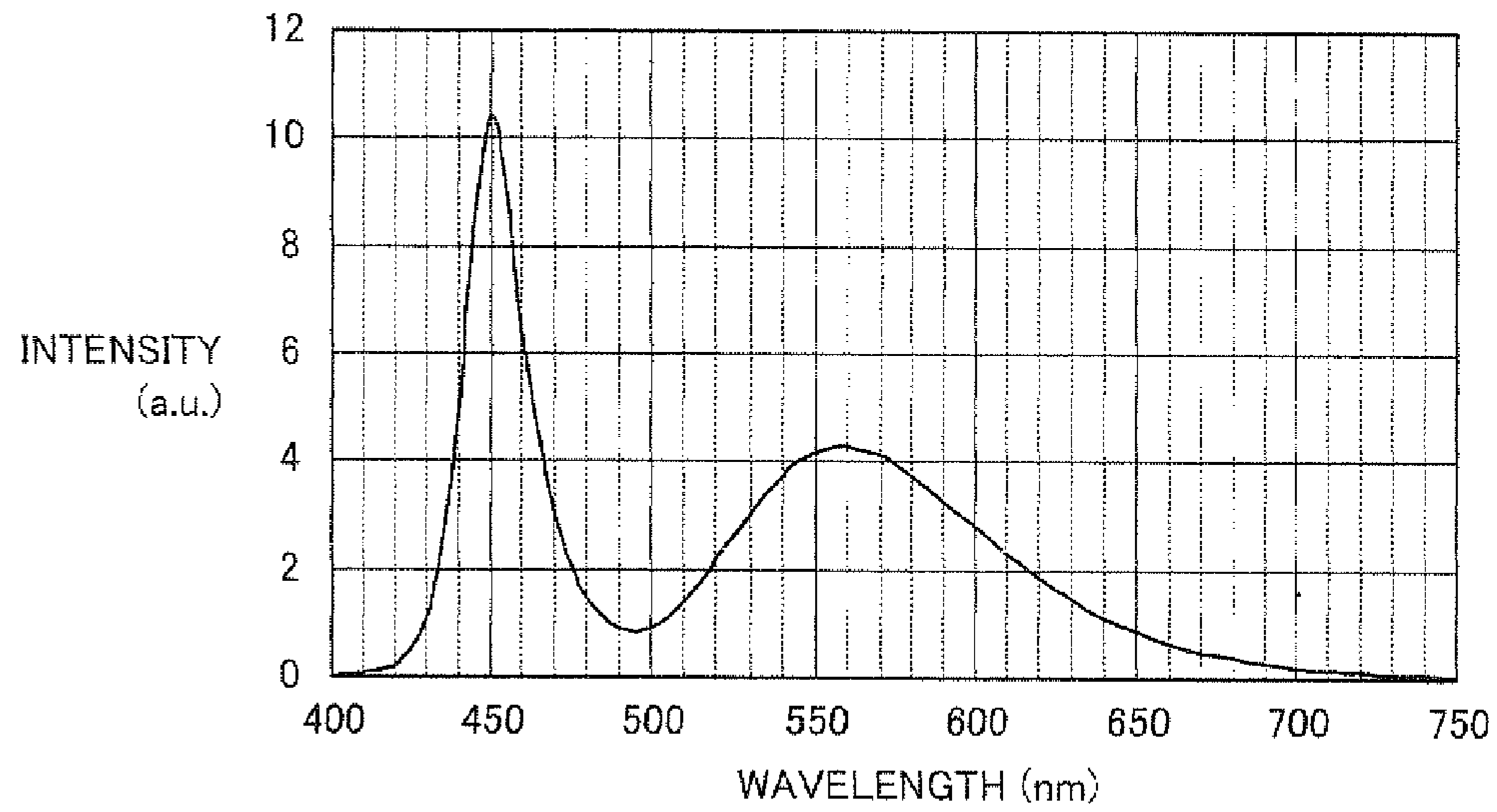
FIG.7 PRIOR ART
