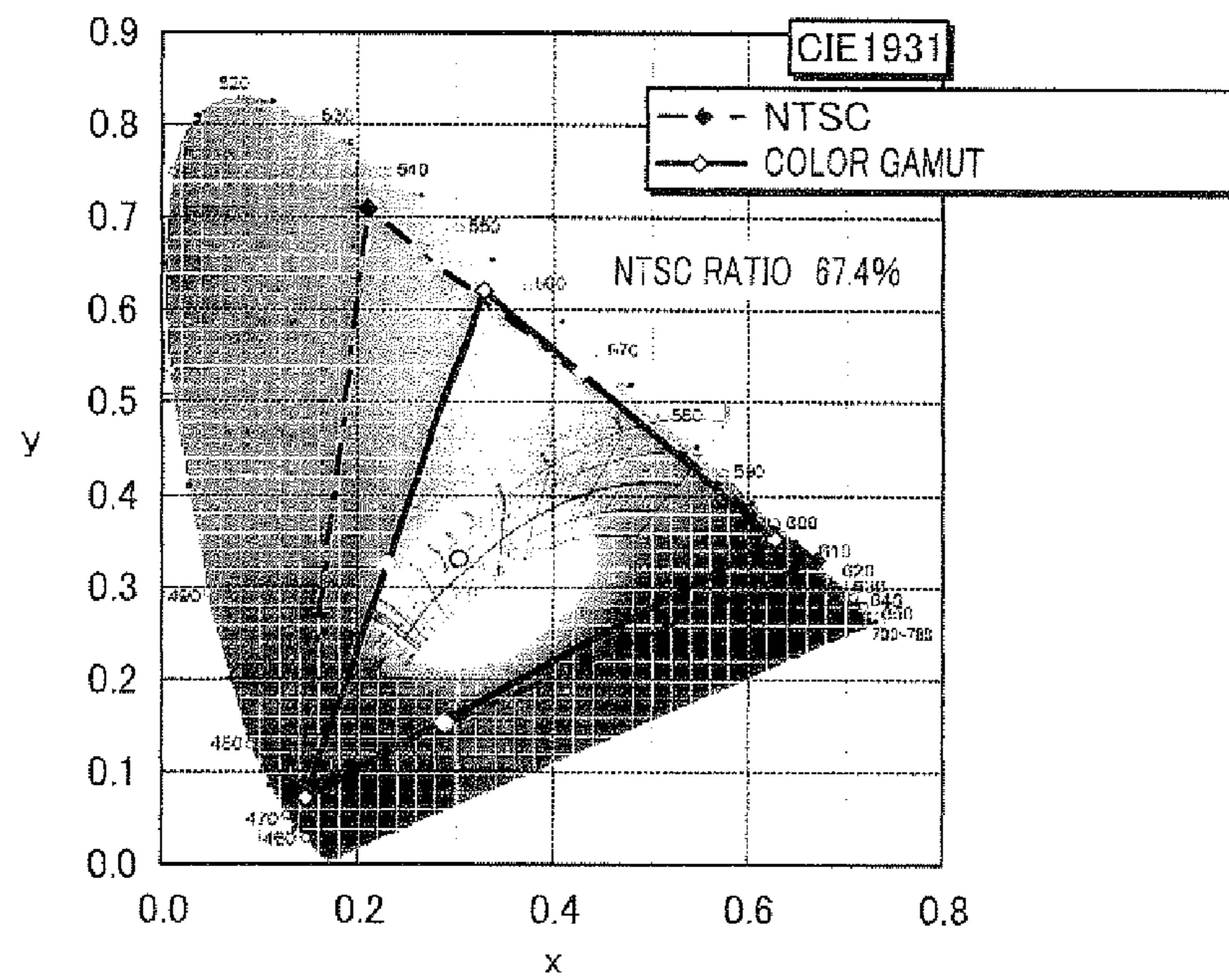
FIG.8 PRIOR ART
