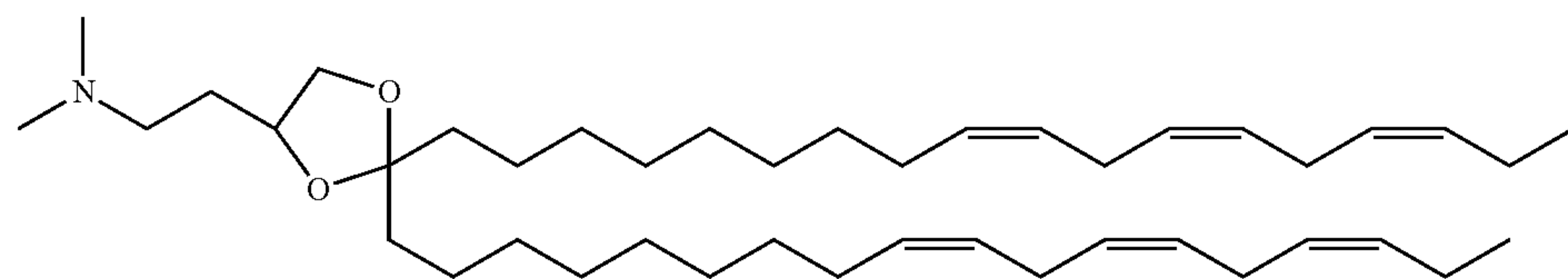
DLen-C2K-DMA
