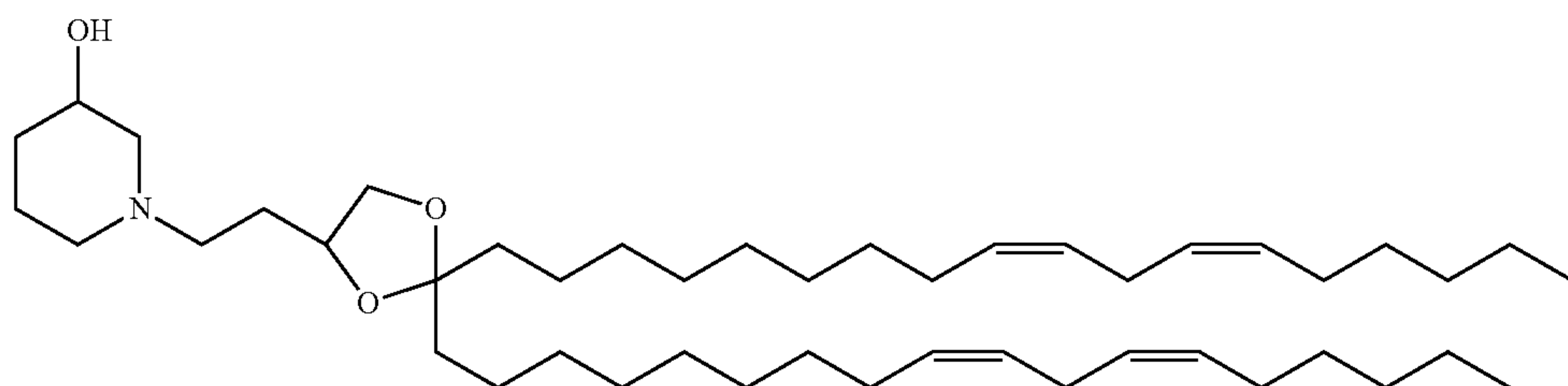
DLin-C2K-Pip-3OH
