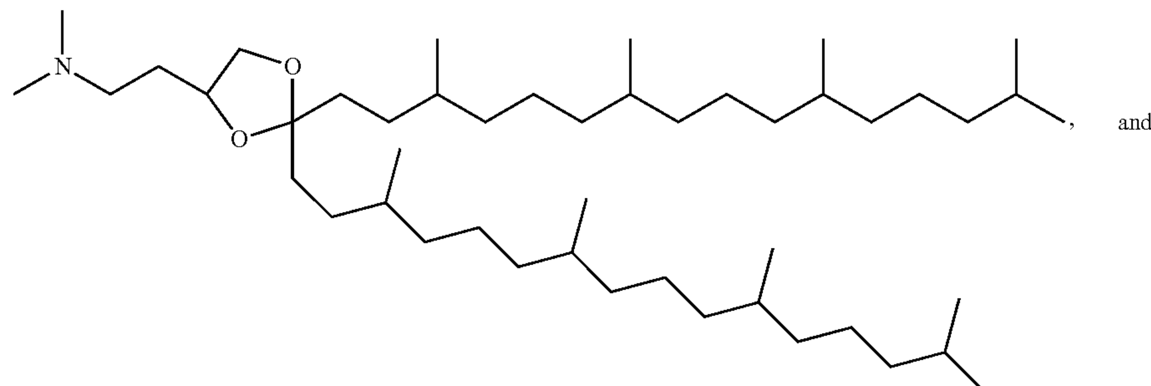
DPan-C2K-DMA
