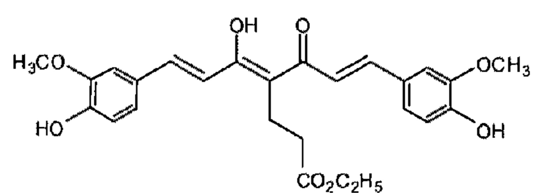
5-Hydroxy-7-(4-hydroxy-3-methoxy-phenyl)-4-[3-(4-hydroxy-3-methoxy-phenyl)-acryloyl]-hepta-4,6-dienoic acid ethyl ester (ASC-J15)
