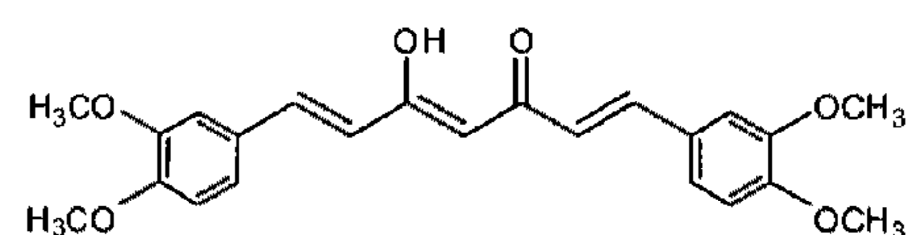
1,7-Bis-(3,4-dimethoxy-phenyl)-5-hydroxy-hepta-1,4,6-trien-3-one (dimethyl curcumin) (ASC-J9)
