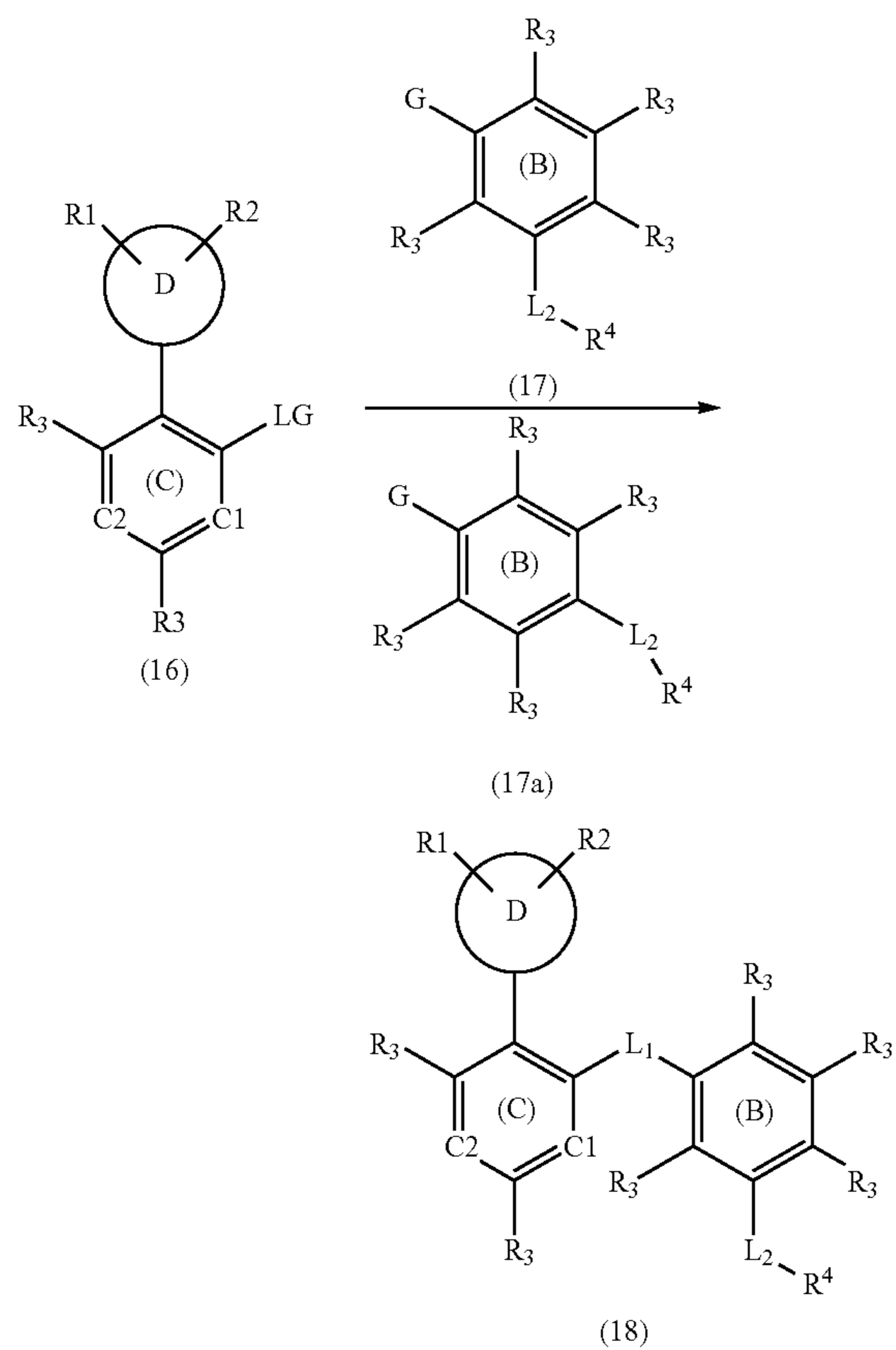
Scheme 2
