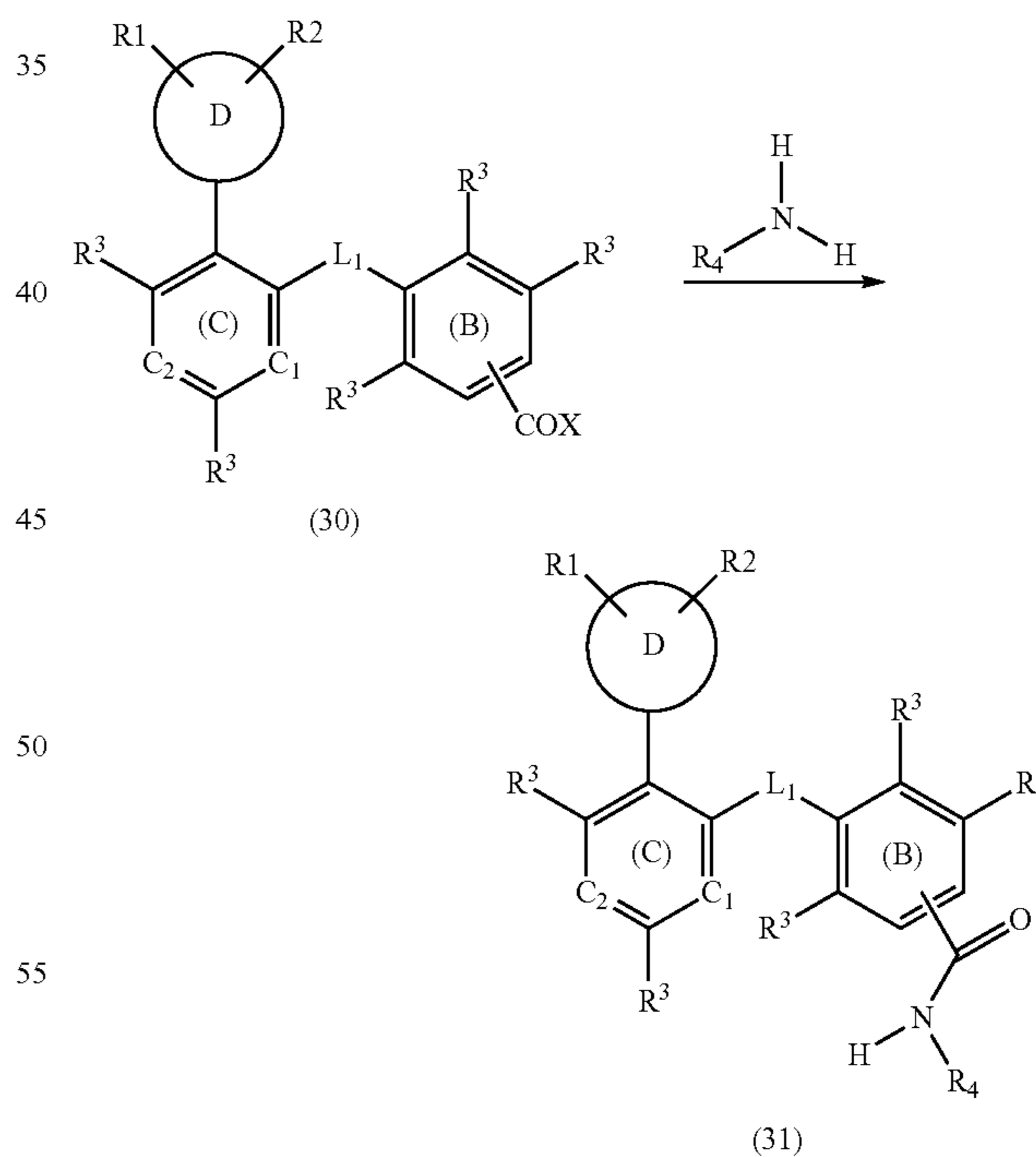
Scheme 3
