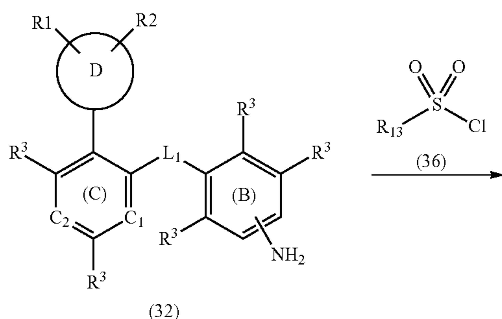
Scheme 5
