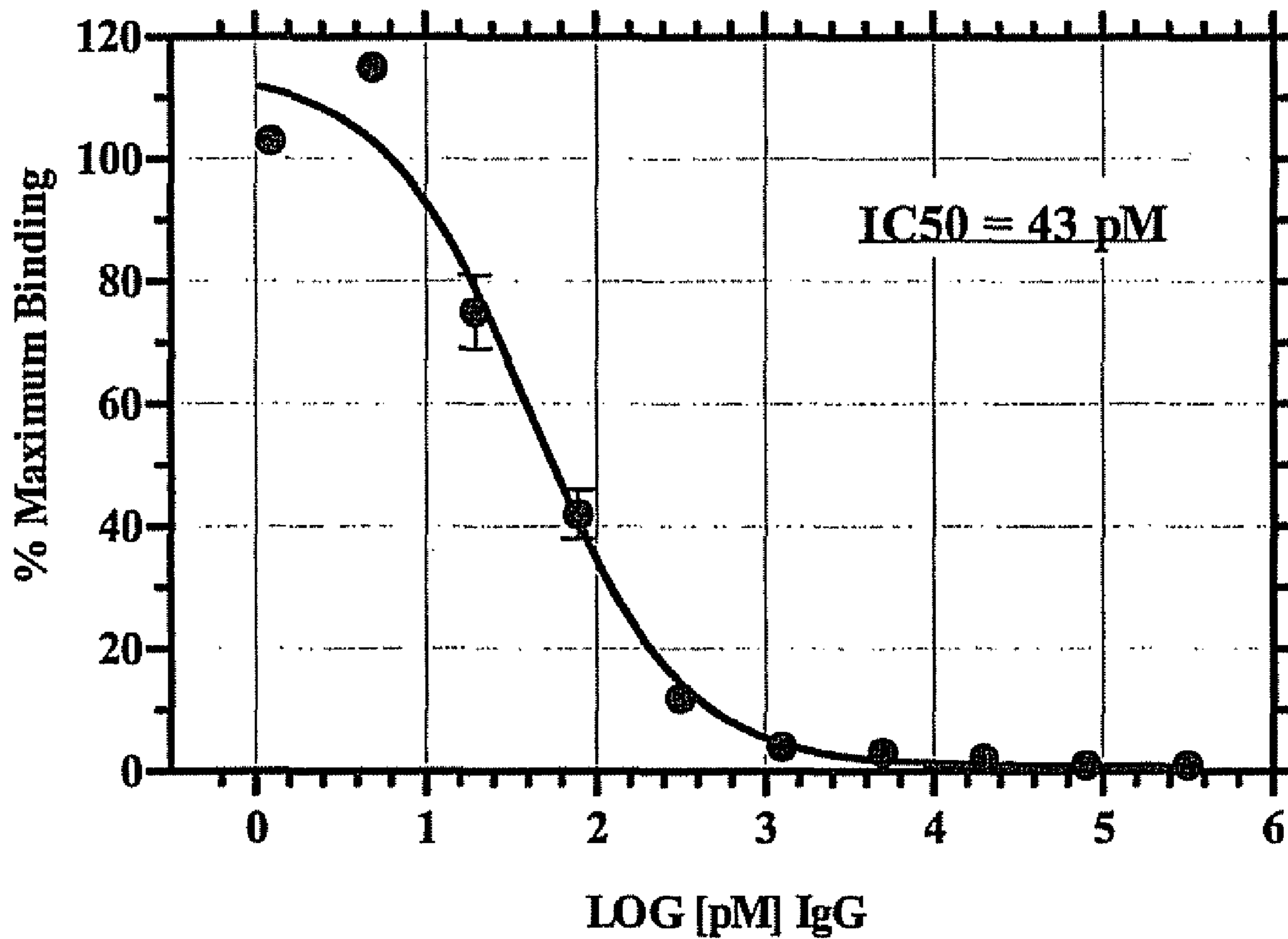
15C4 Competition of IL-1R1/IL-1 \alpha /RAcP Complex Formation
