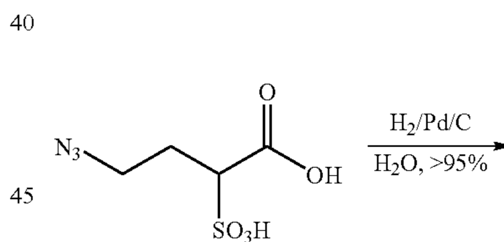
4-Amino-2-sulfo-butyric acid
