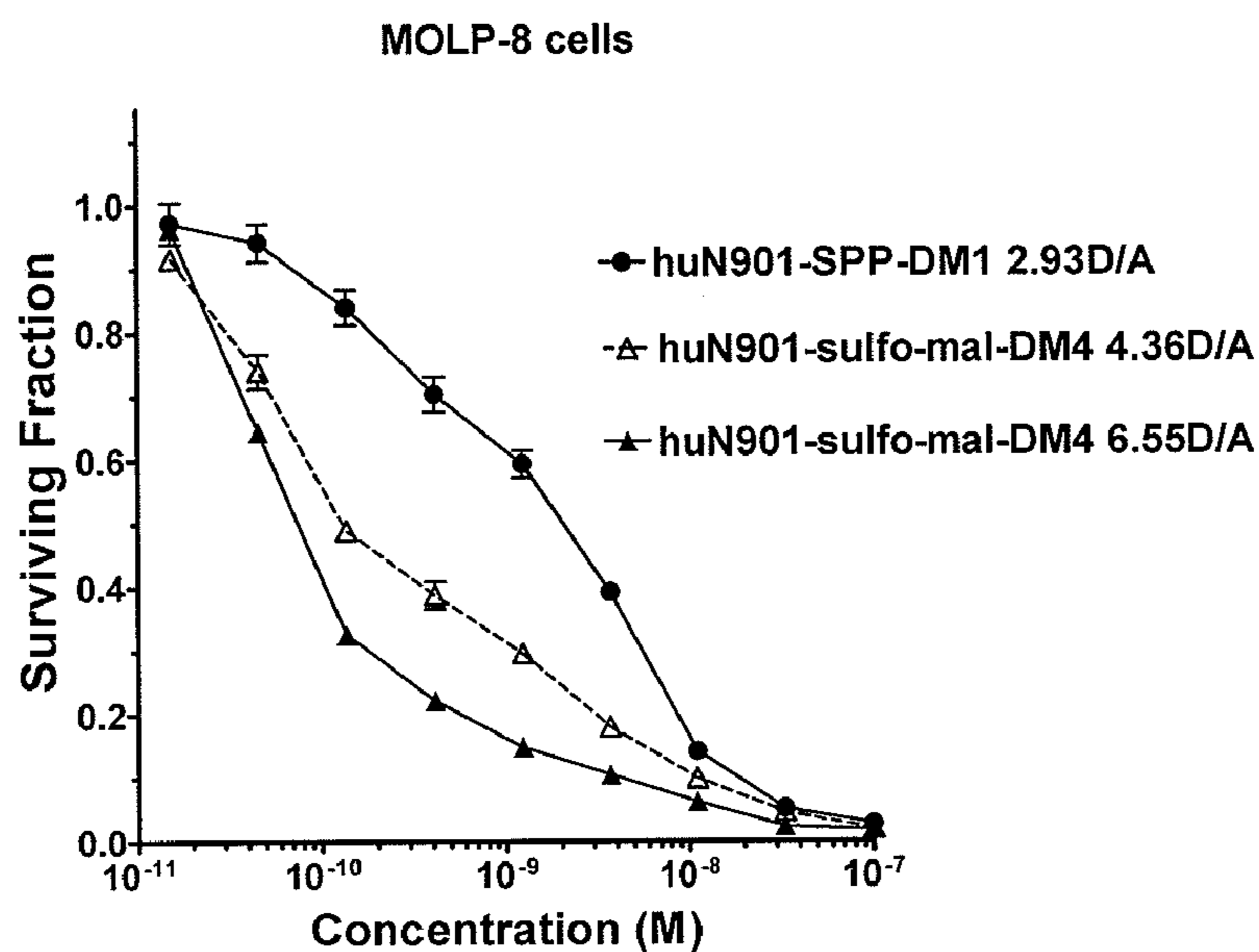
Figure 57(B) Cytotoxicity of anti-CD56(huN901) antibody-maytansinoid conjugates
