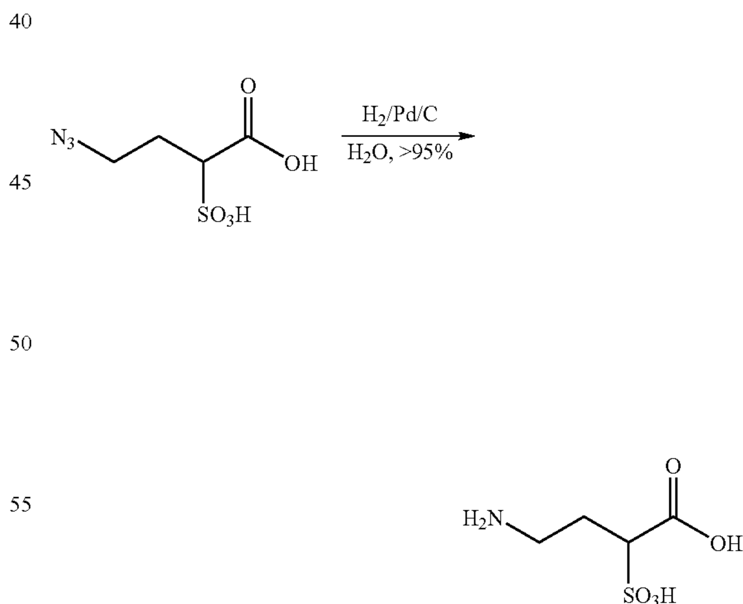
4-Amino-2-sulfo-butyric acid
