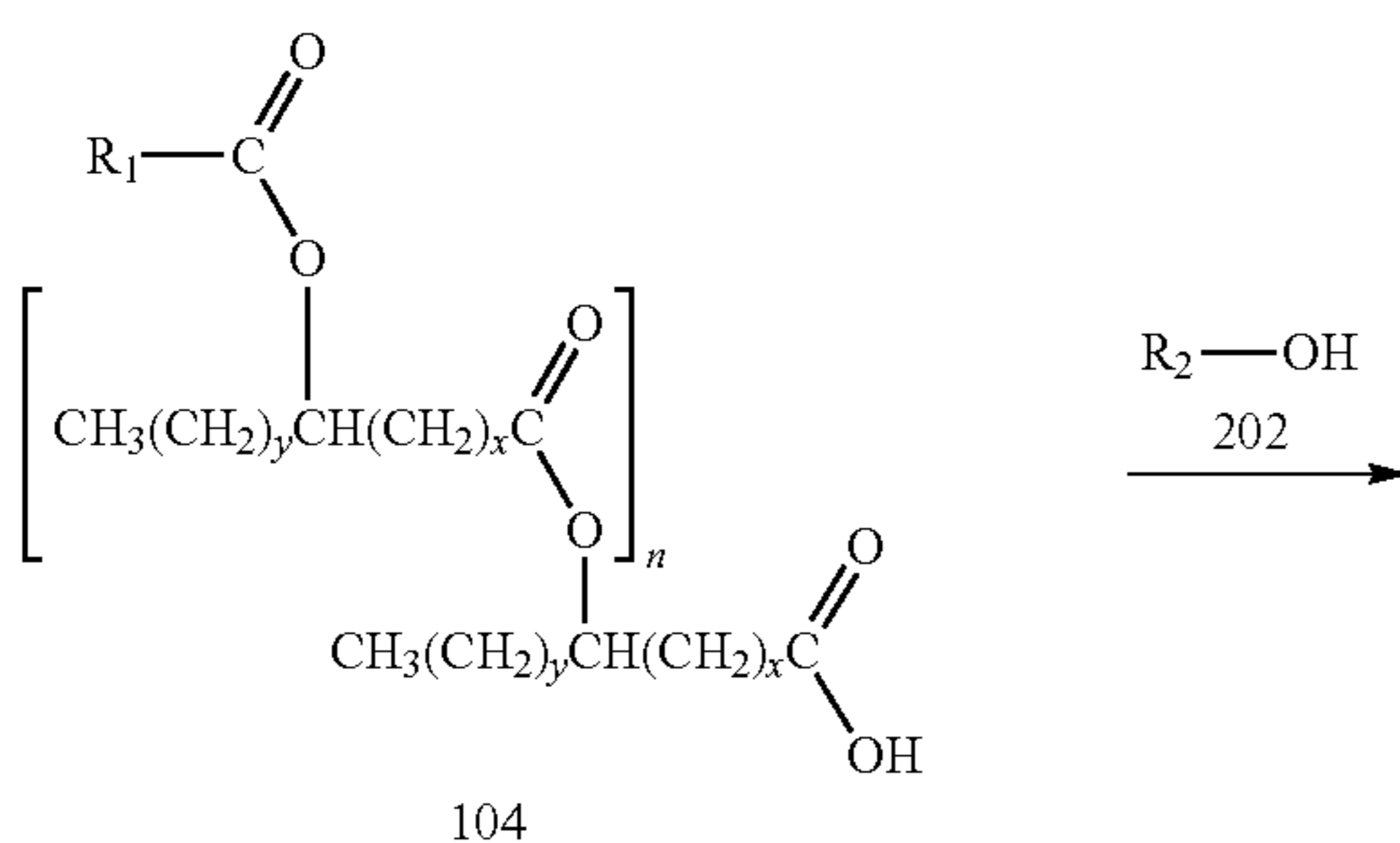
Scheme 2
