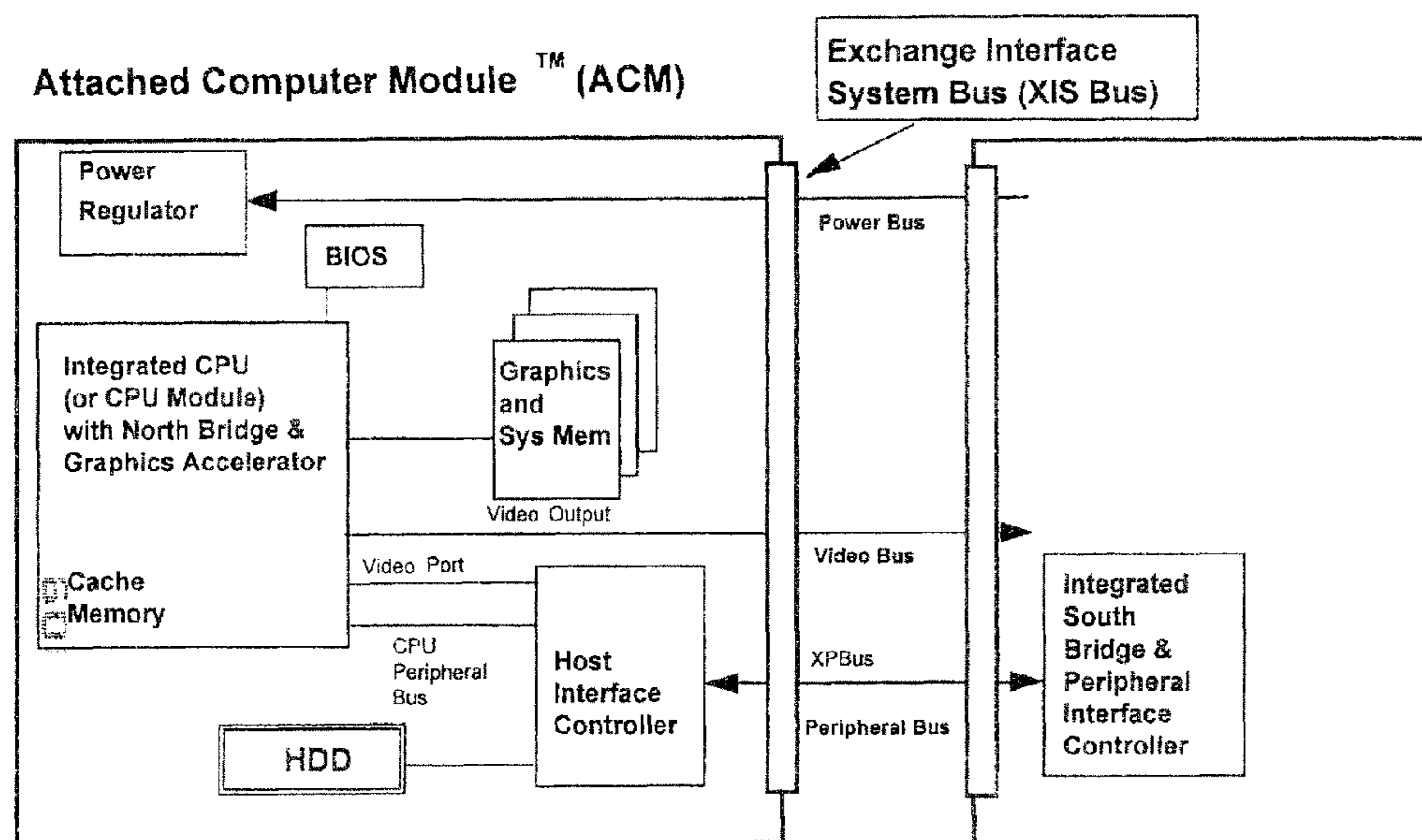
Fig. 8C In the implementation with South Bridge in Peripheral Console, an example of Attached Computer Module with Integrated CPU/North Bridge/Graphics and Peripheral Console with Integrated Peripheral Interface Controller and South Bridge
