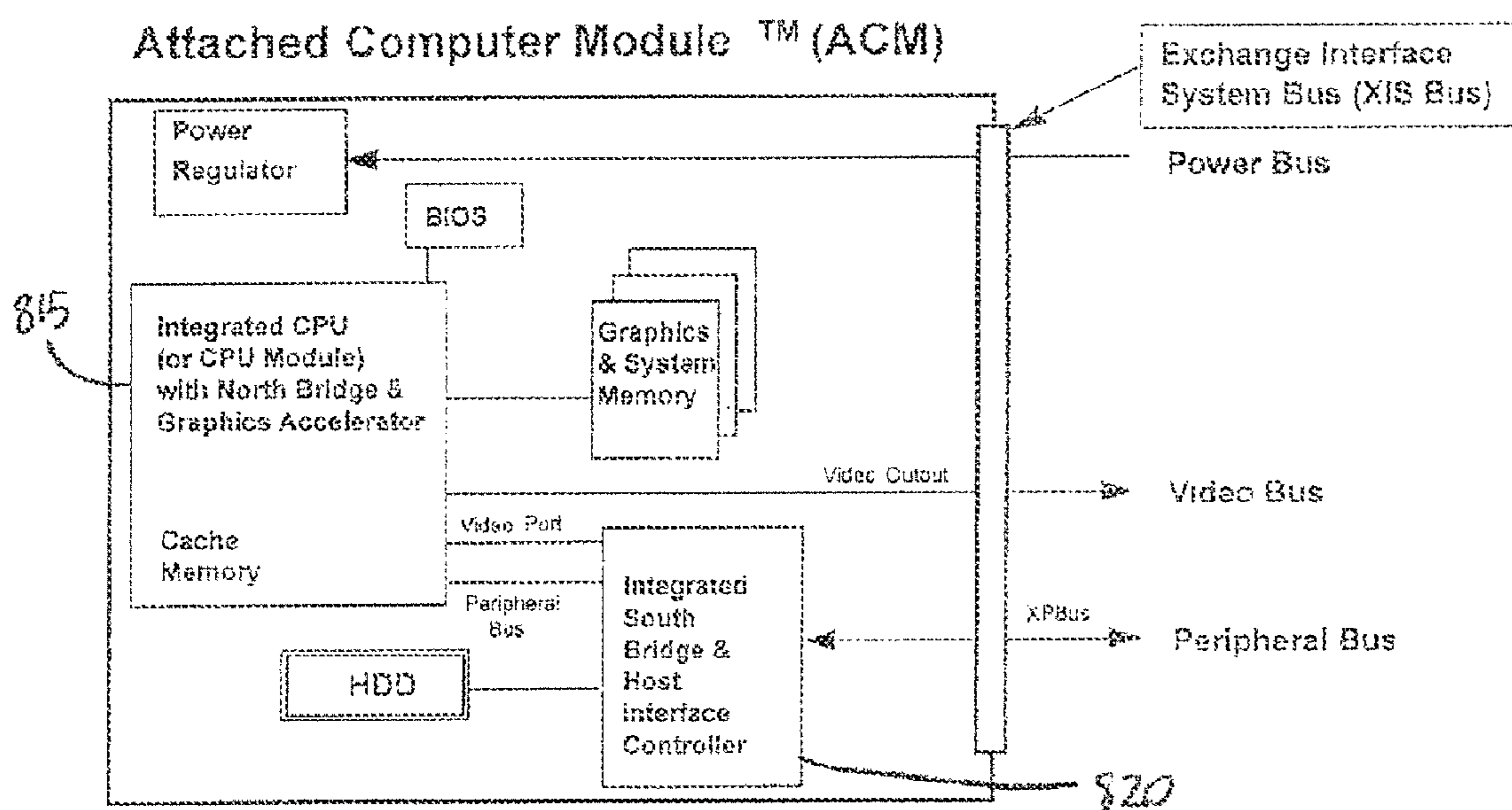
FIG. 8A Attached Computer Module with Integrated CPU/NB/Graphics and Integrated HIC/SB
