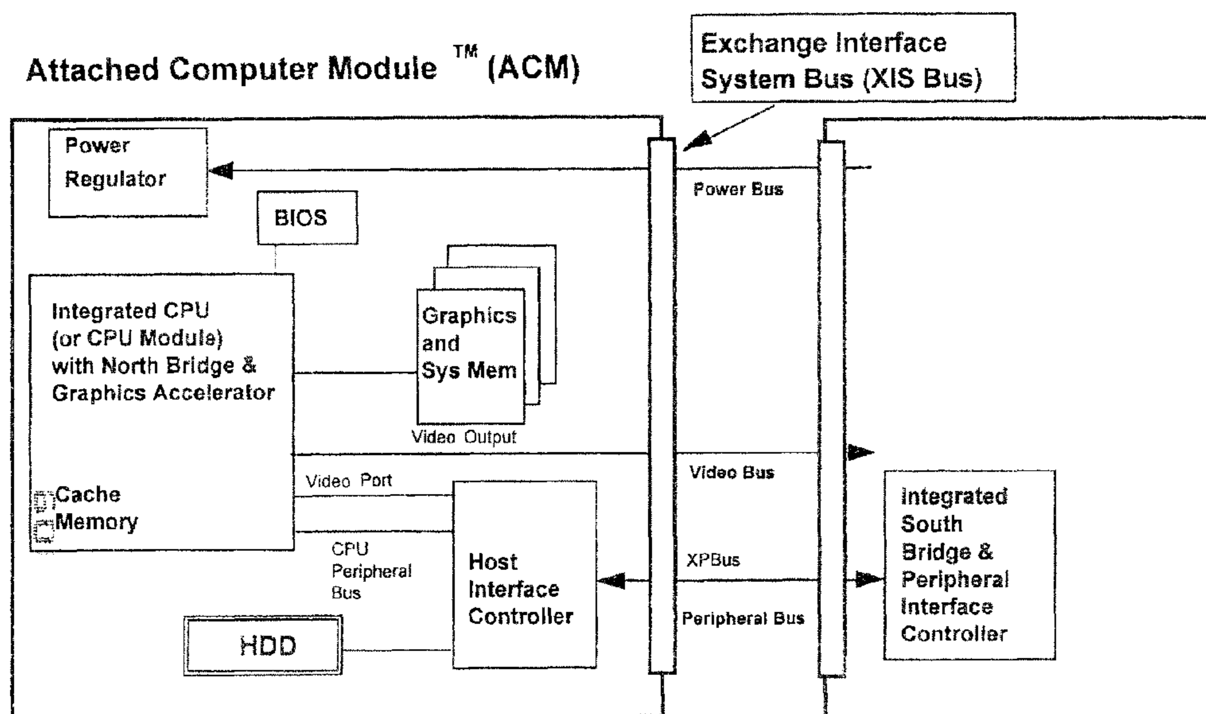
Fig. 8C In the implementation with South Bridge in Peripheral Console, an example of Attached Computer Module with Integrated CPU/North Bridge/Graphics and Peripheral Console with Integrated Peripheral Interface Controller and South Bridge
