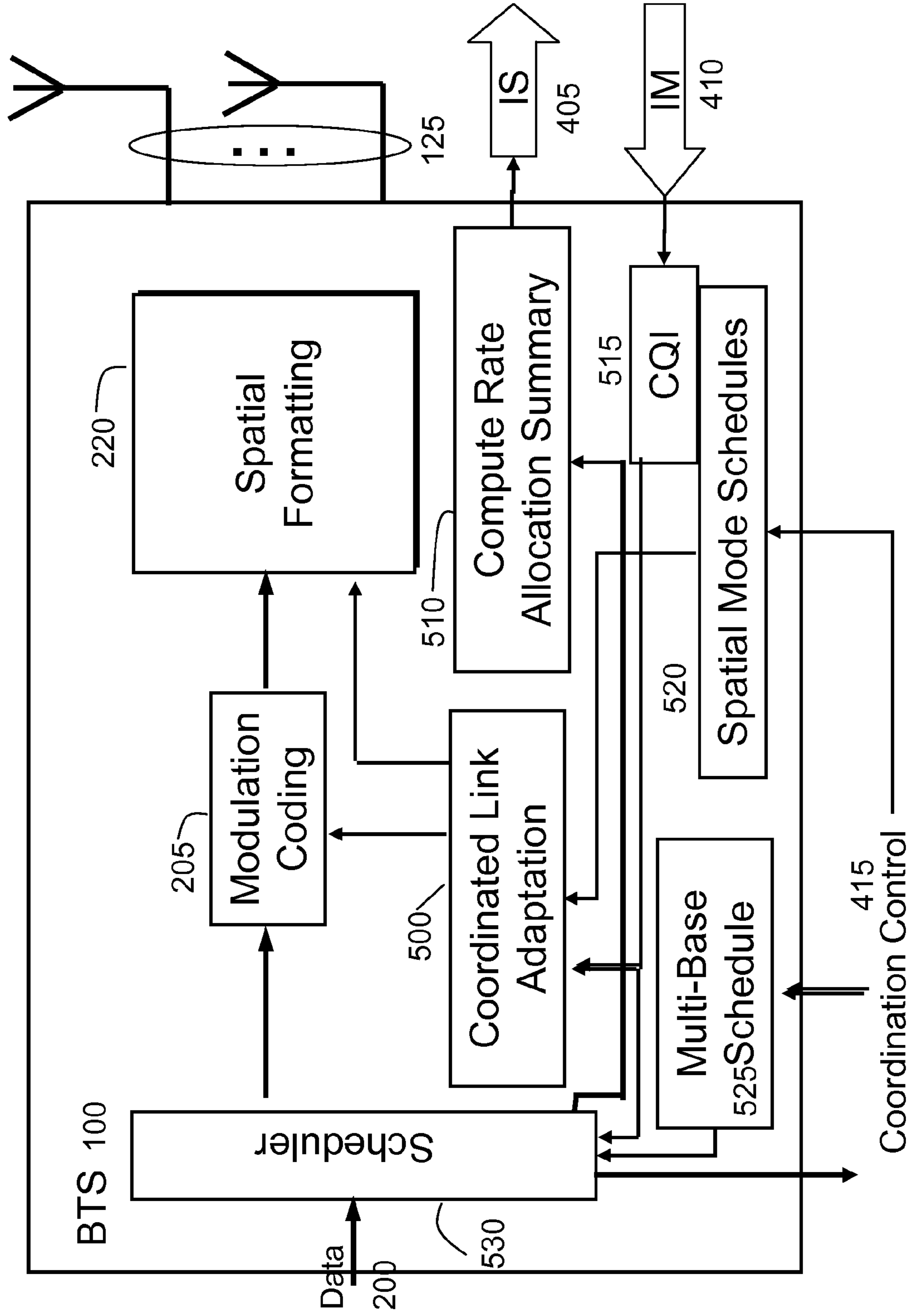
Fig. 5 Base Station Features
