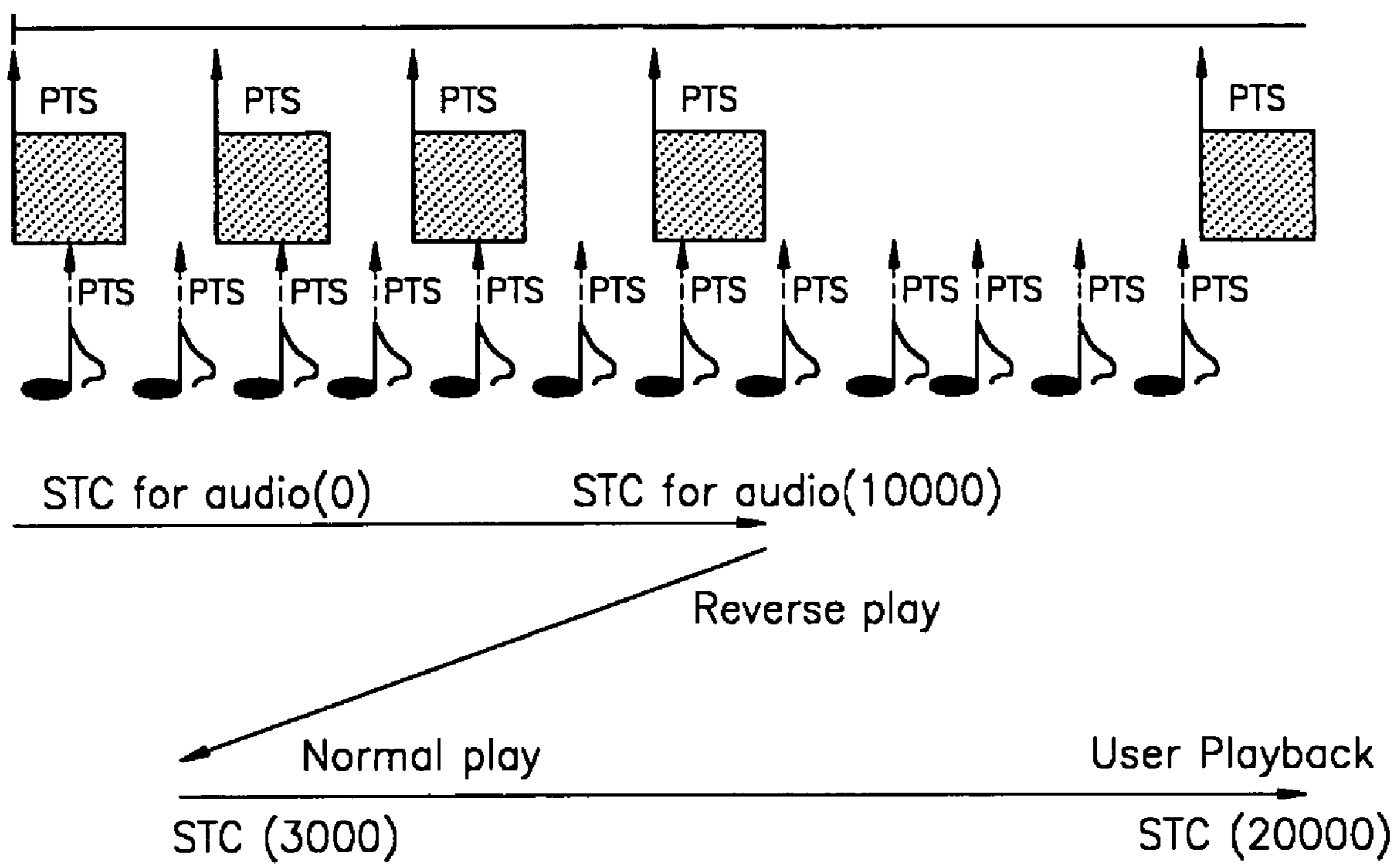
FIG. 7 (PRIOR ART)
