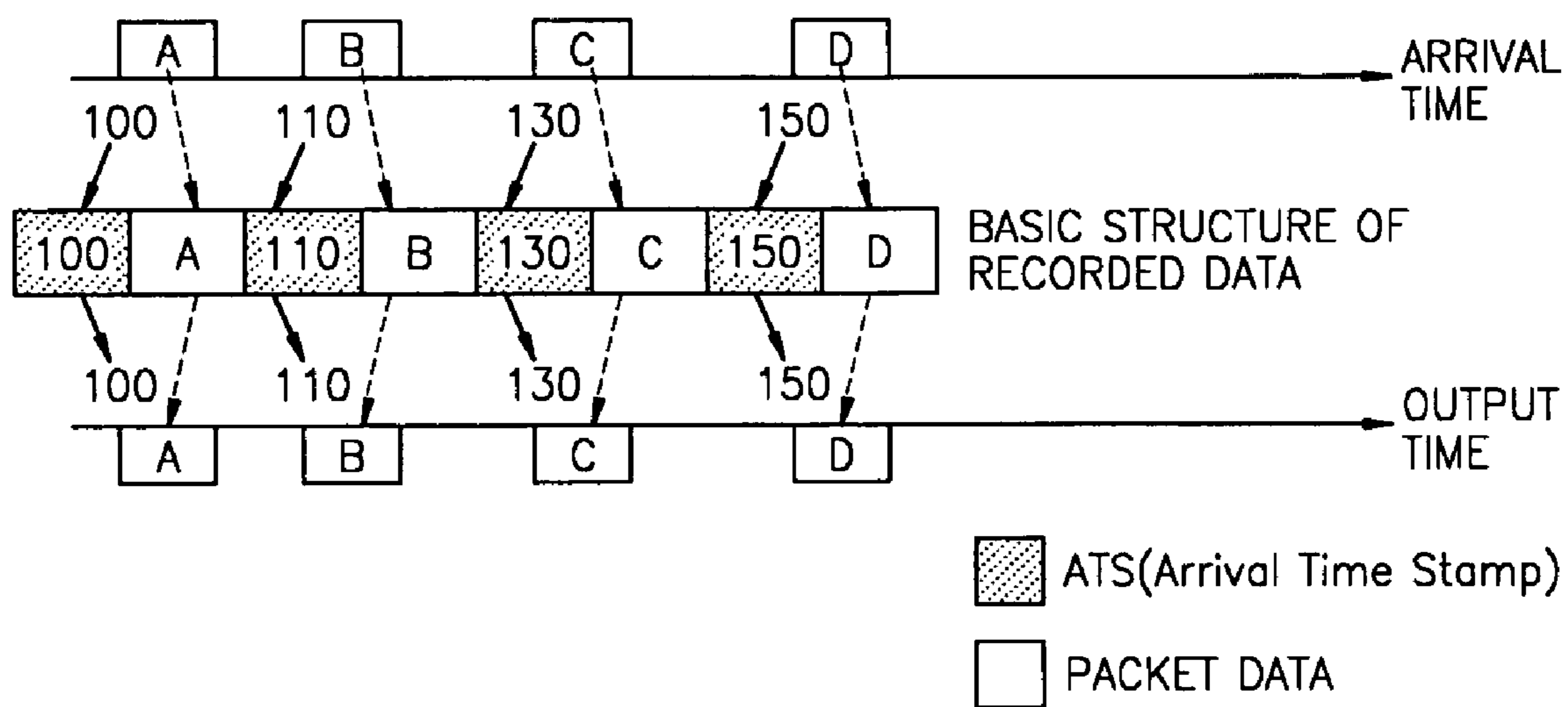
FIG. 3 (PRIOR ART)
