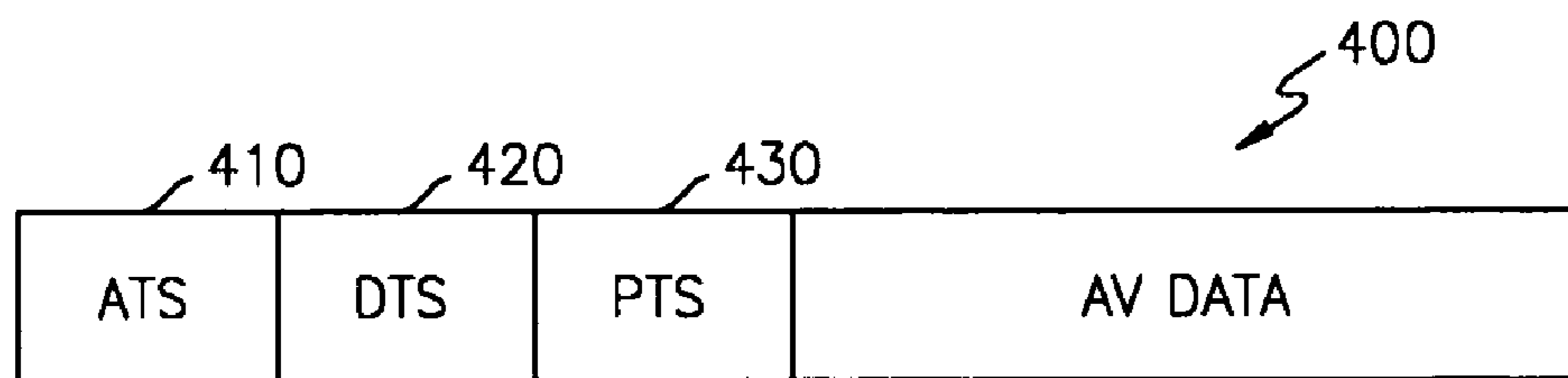
FIG. 4 (PRIOR ART)
