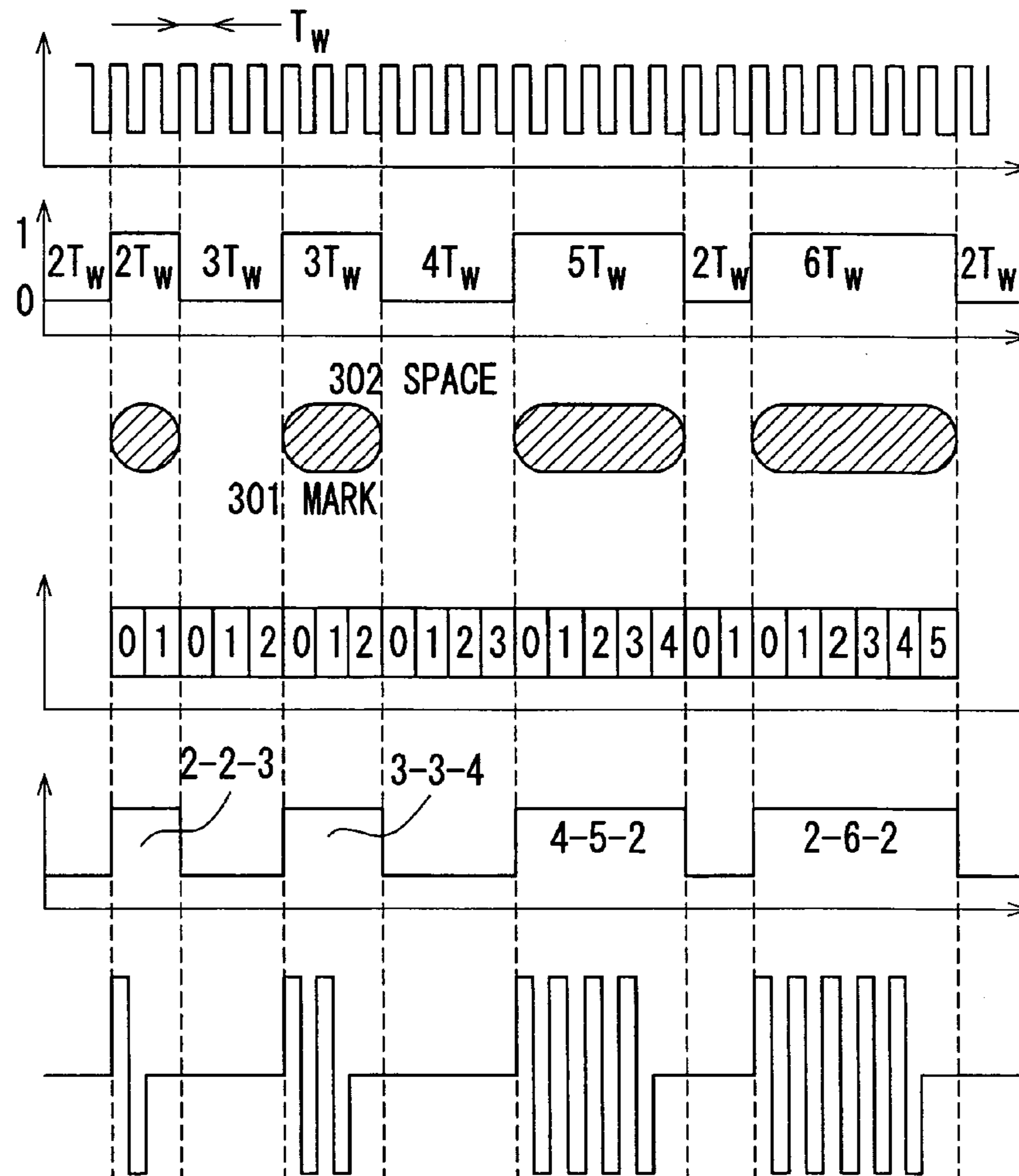
Fig. 2A 128 REFERENCE-TIME SIGNAL
