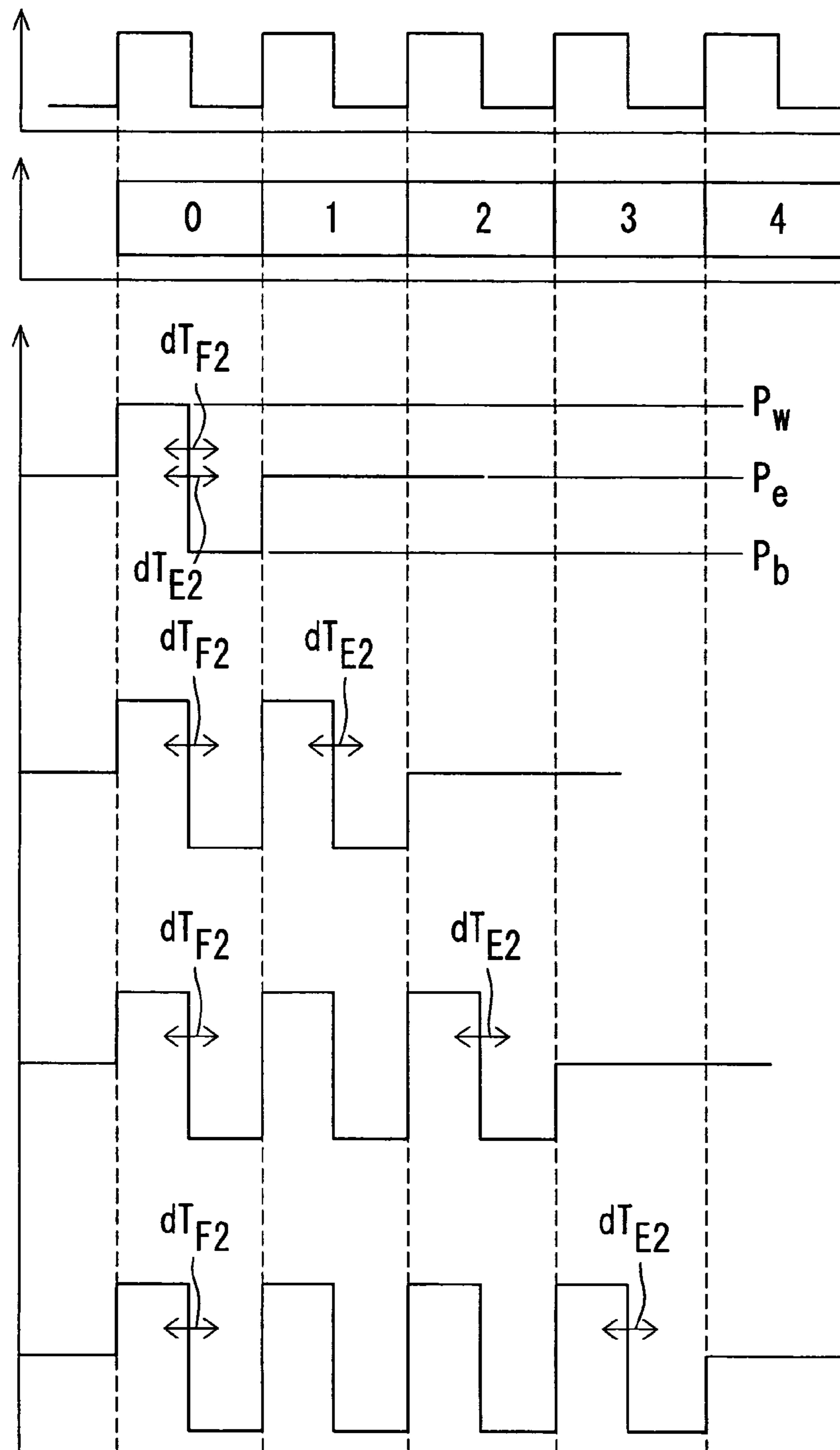
Fig. 3A 128 REFERENCE-TIME SIGNAL
