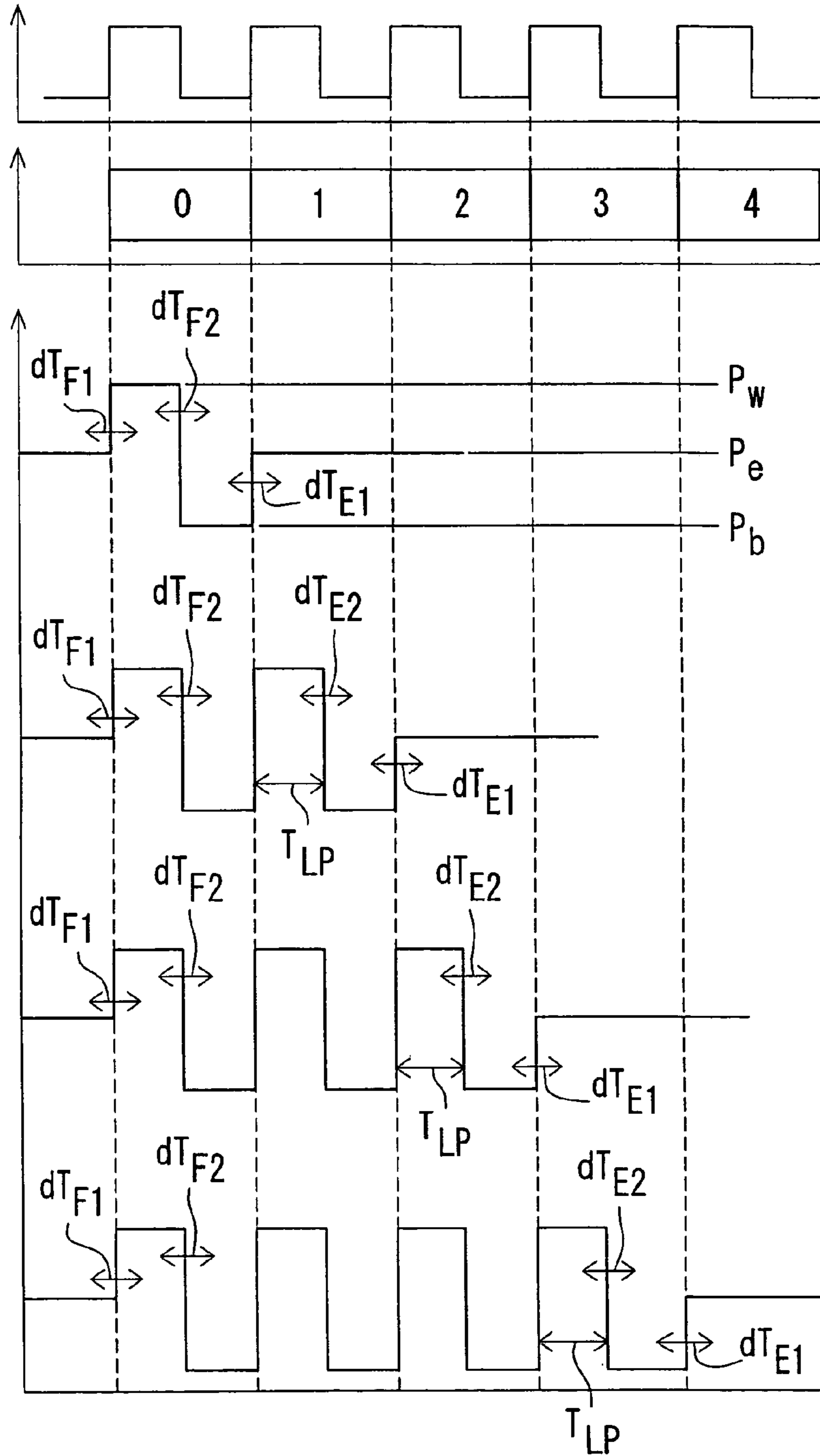
Fig. 9A 128 REFERENCE-TIME SIGNAL
