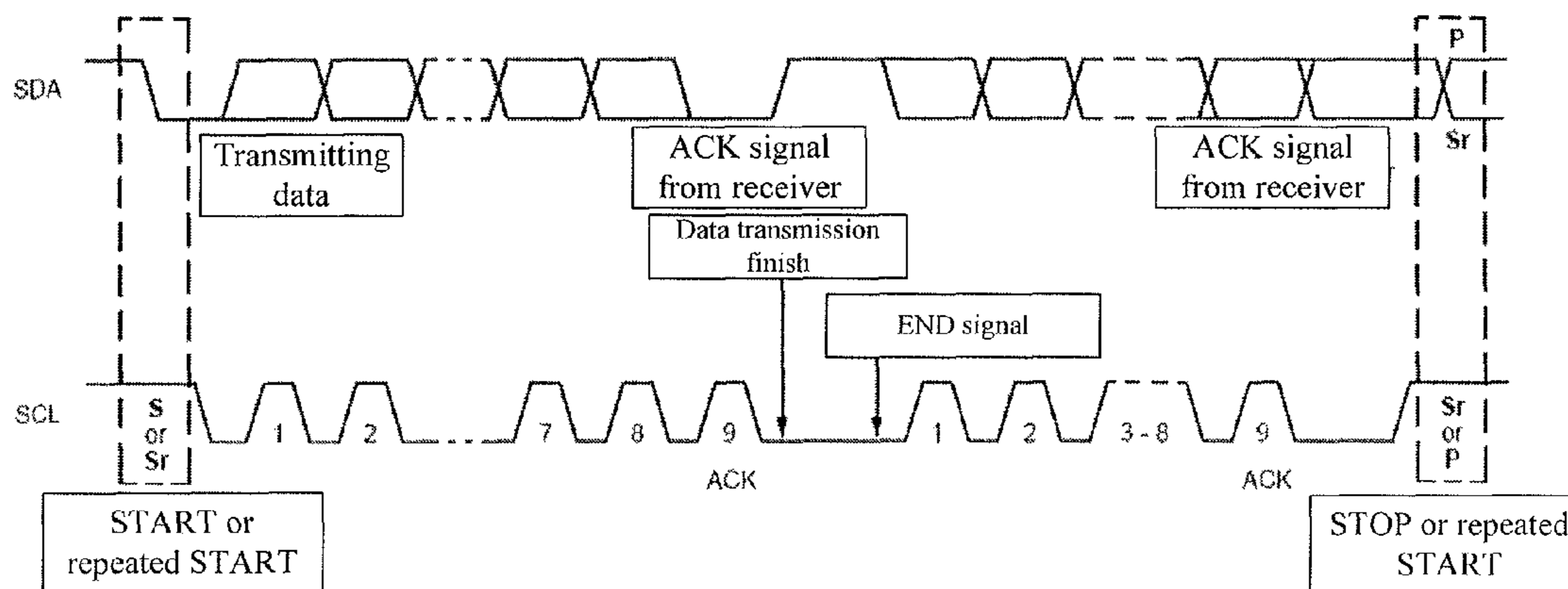
Fig. 2 (Prior Art)
