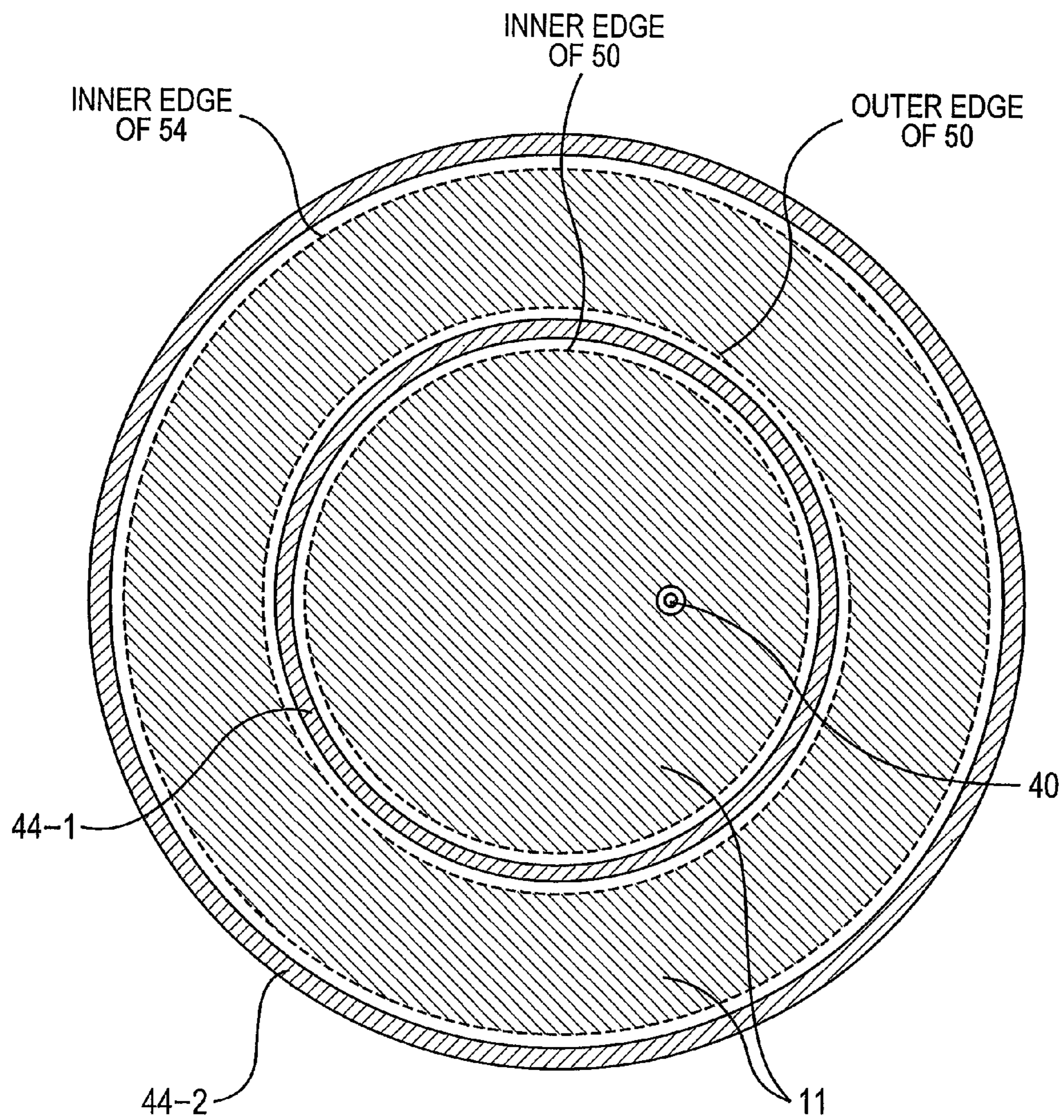
CROSS-SECTIONAL VIEW OF A-A
