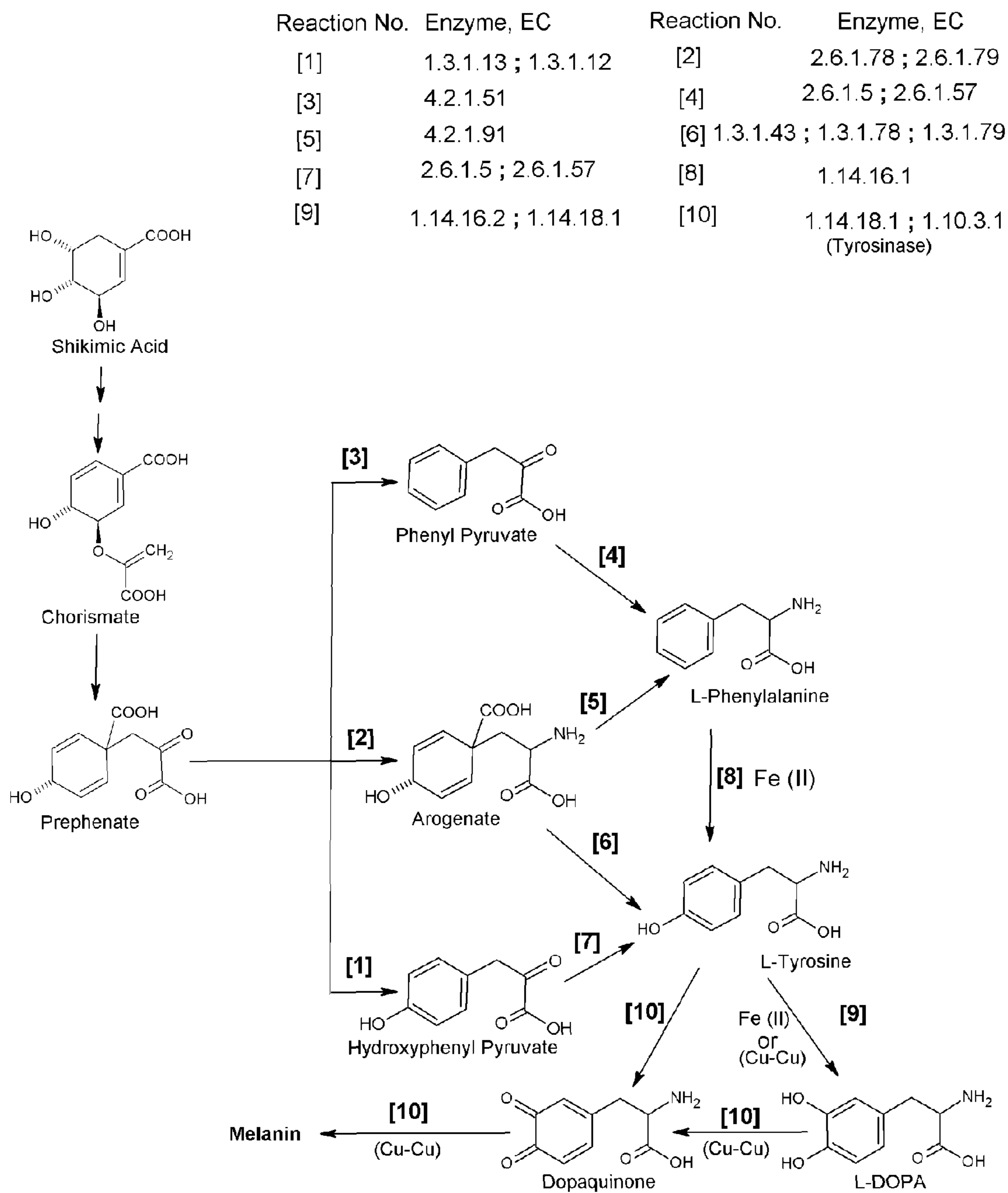
FIG. 2. Melanin Biosynthesis via Shikimate Pathway
