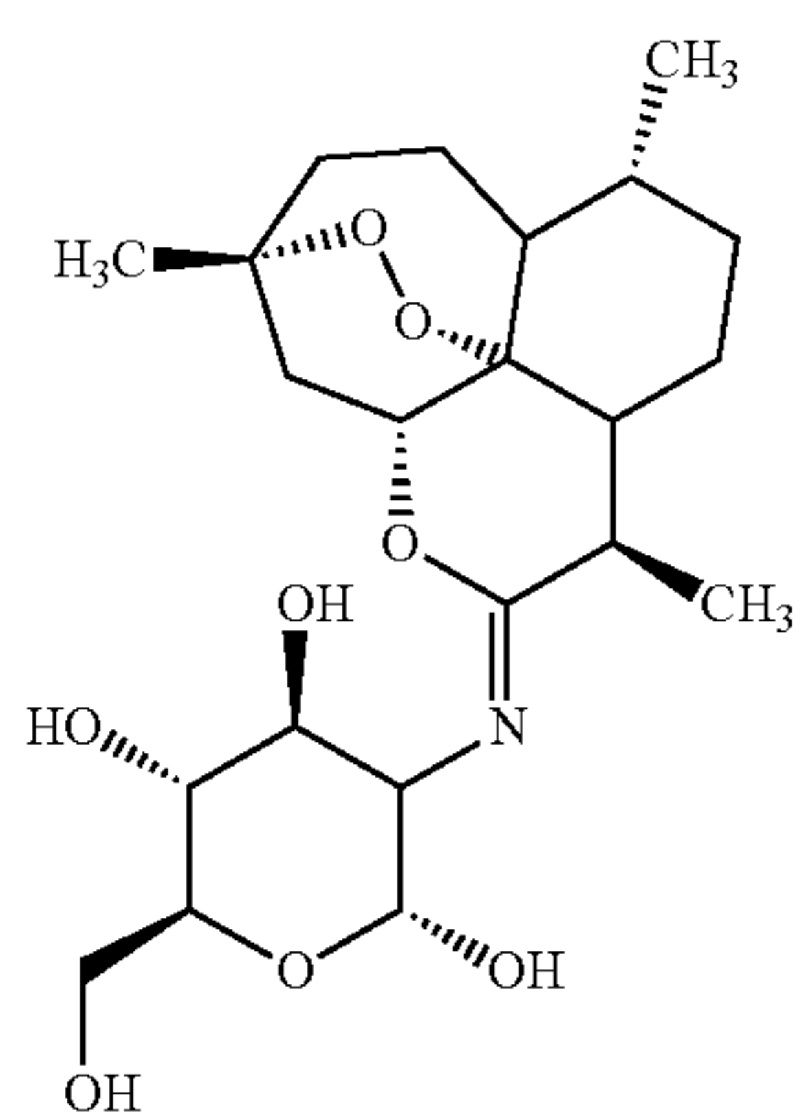
(a) N-[(E)-10-Deoxyartemisinylidene]-glucosamine (b) N-[(Z)-10-Deoxyartemisinylidene]-glucosamine (c) 11-(N-Glucosamino)-azaartemisinin
