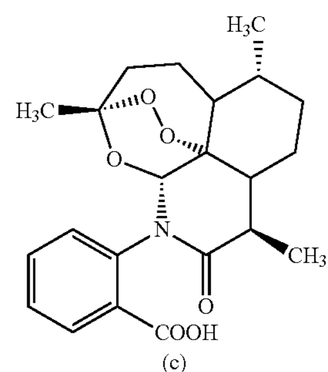
(a) N-[(E)-10-Deoxyartemisinylidene]-anthranilic acid (b) N-[(Z)-10-Deoxyartemisinylidene]-anthranilic acid (c) 11-(N-2-carboxyphenyl)-azaartemisinin
