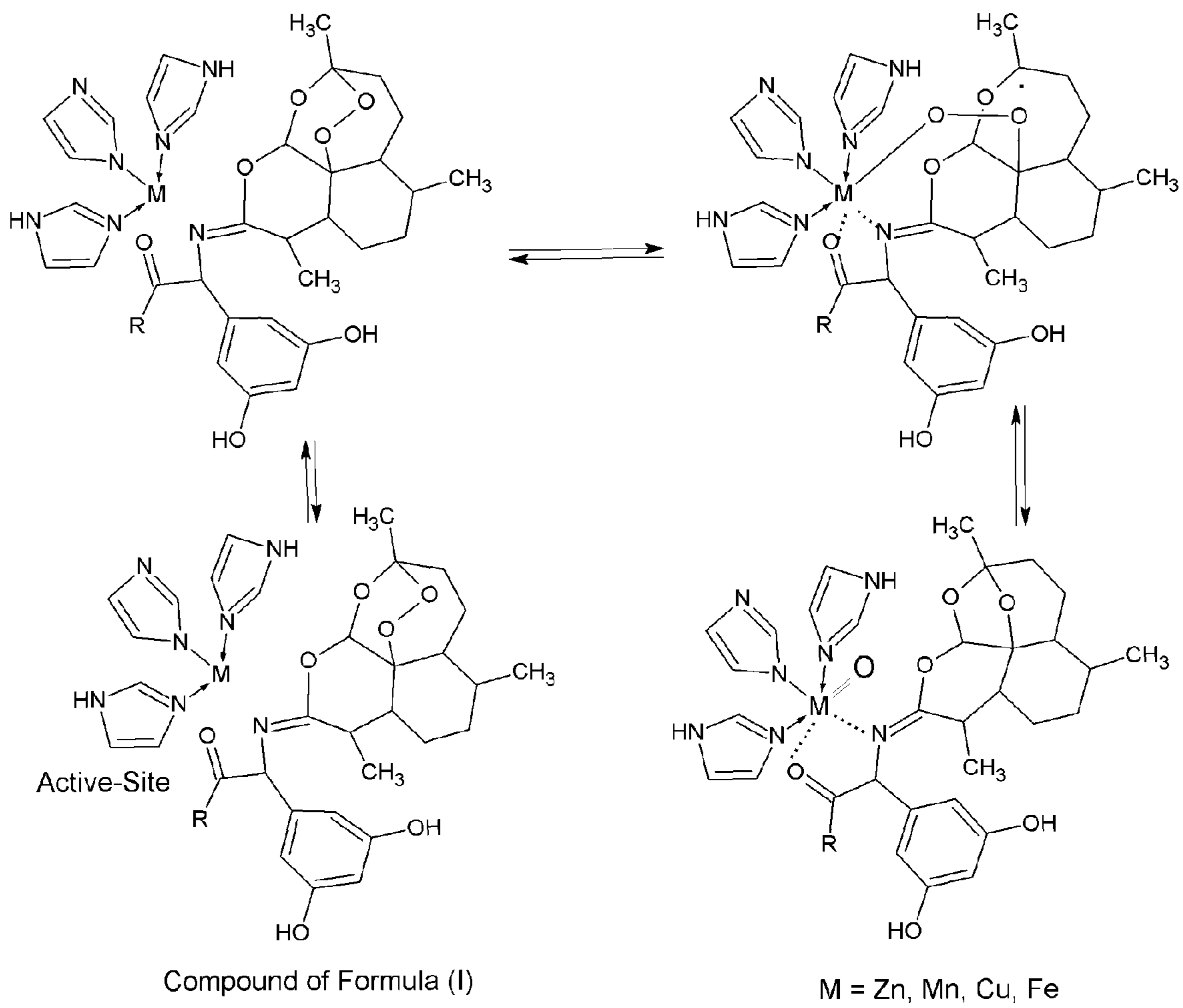
FIG. 5. Binding of Formula (I) with Metalloenzymes
