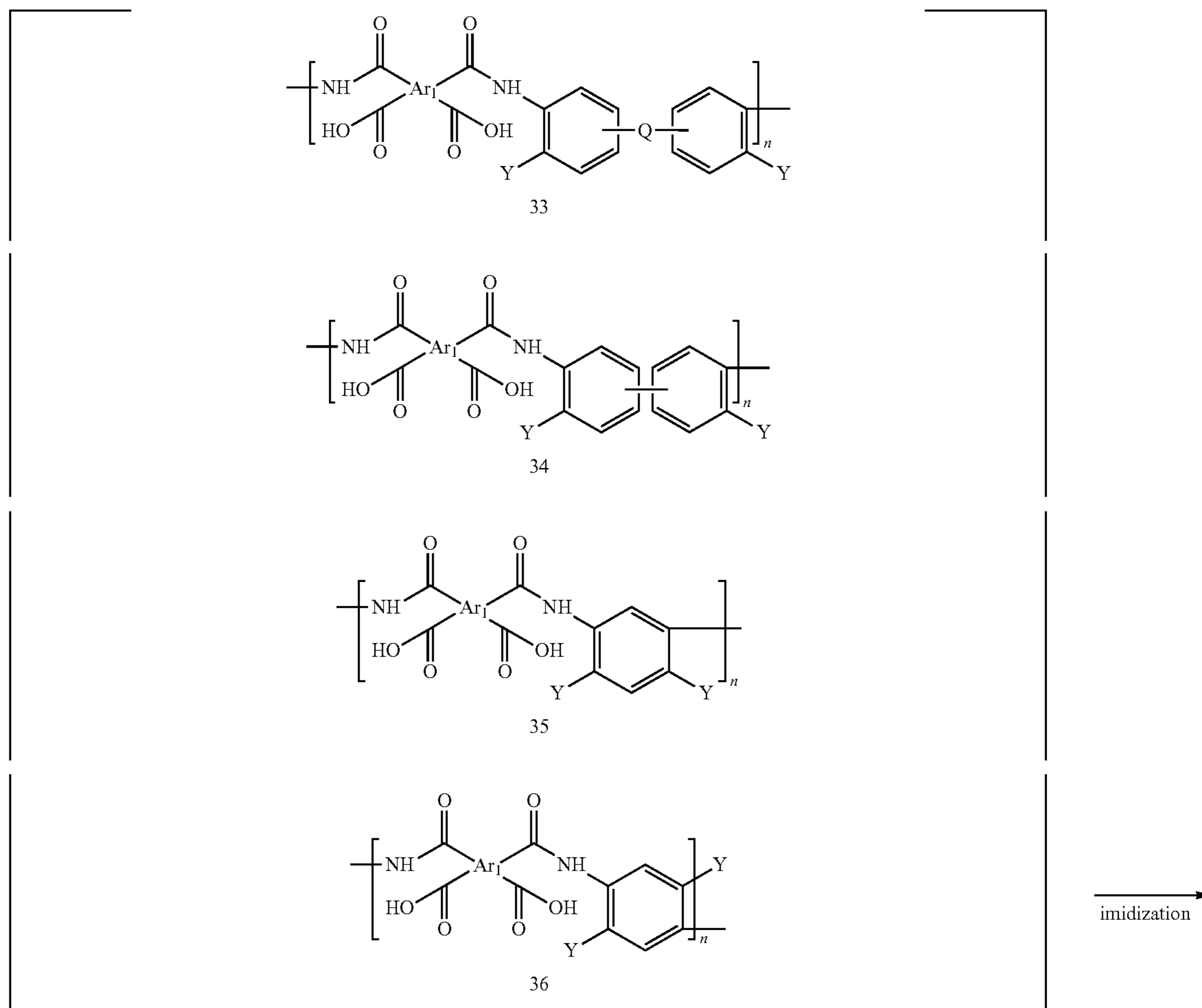
Reaction Scheme 3
