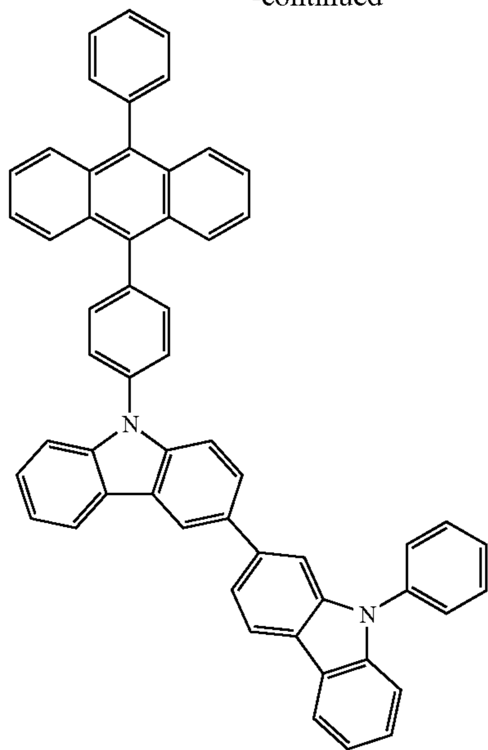
PCCPA
