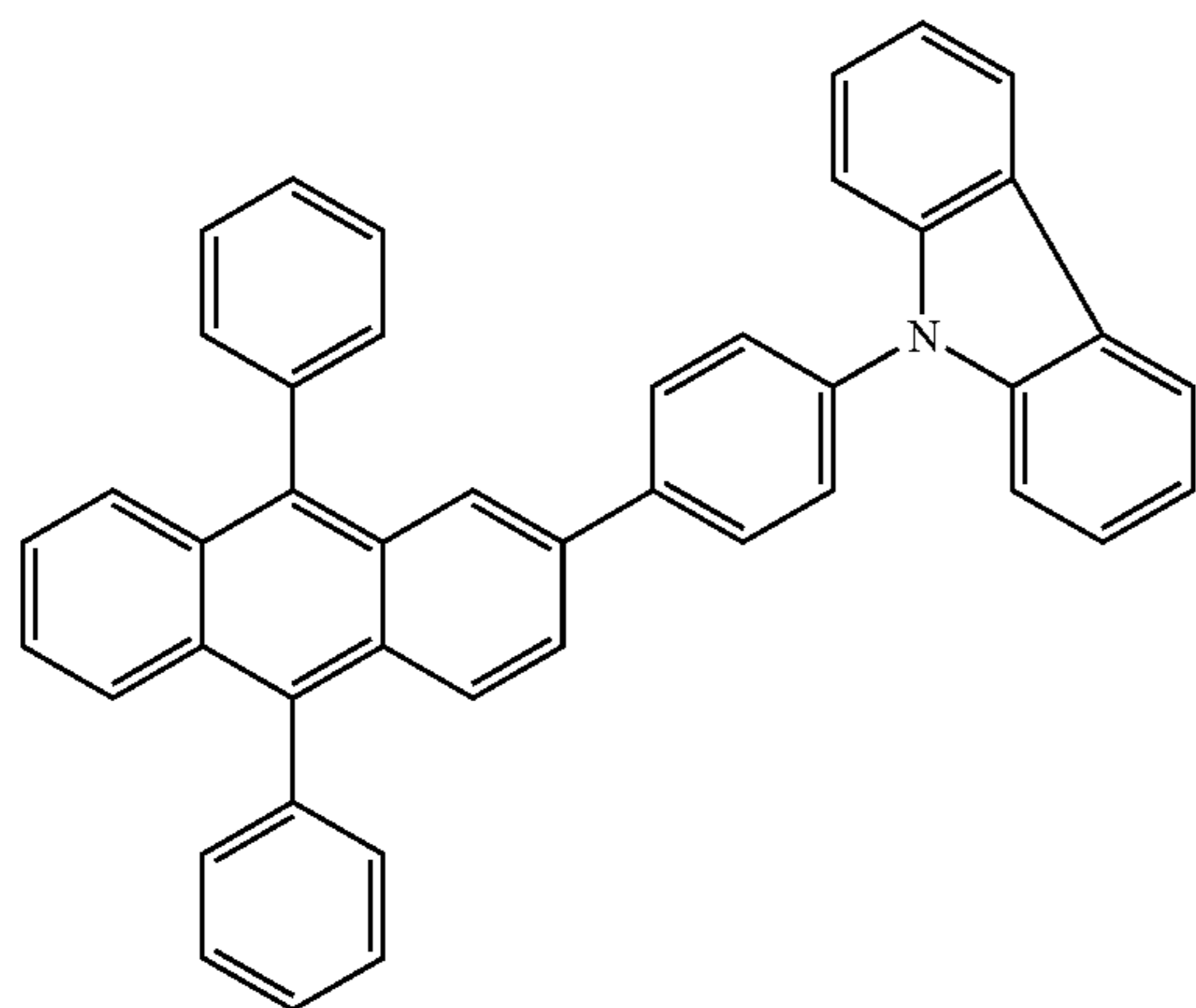
2CzPPA
