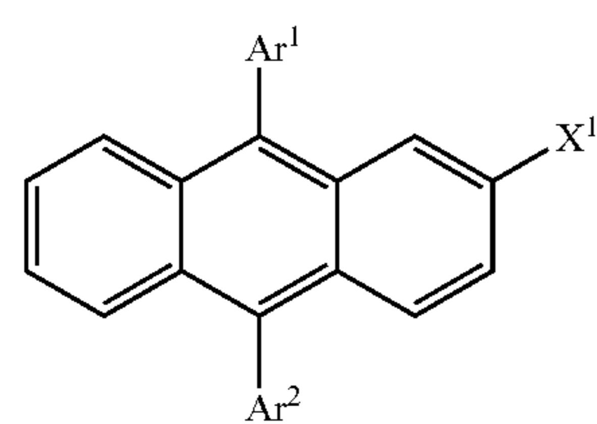
compound 1
