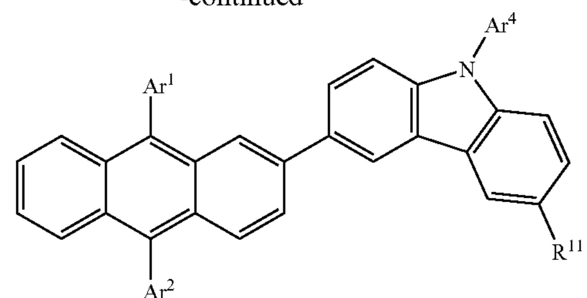
compound 5 (G31-1)
