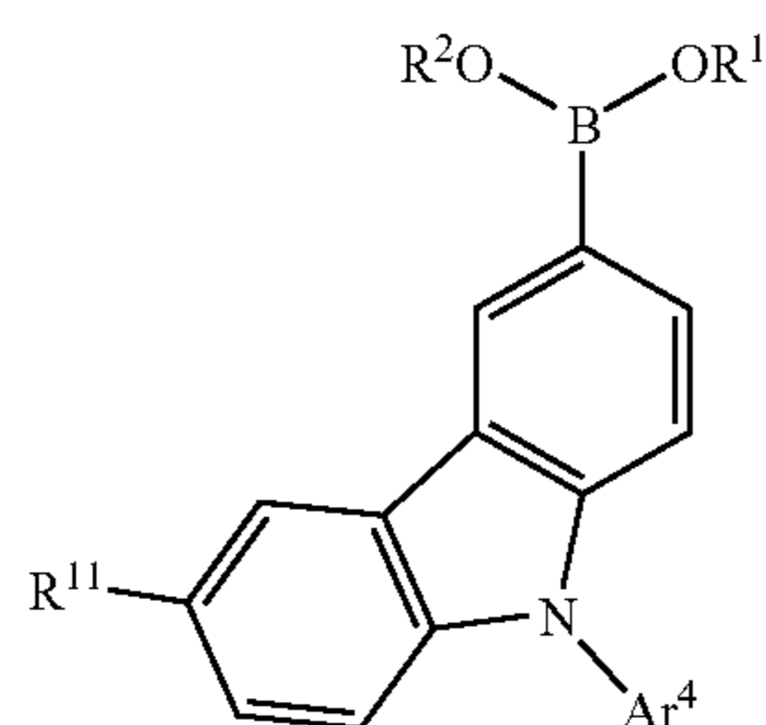
compound 4
