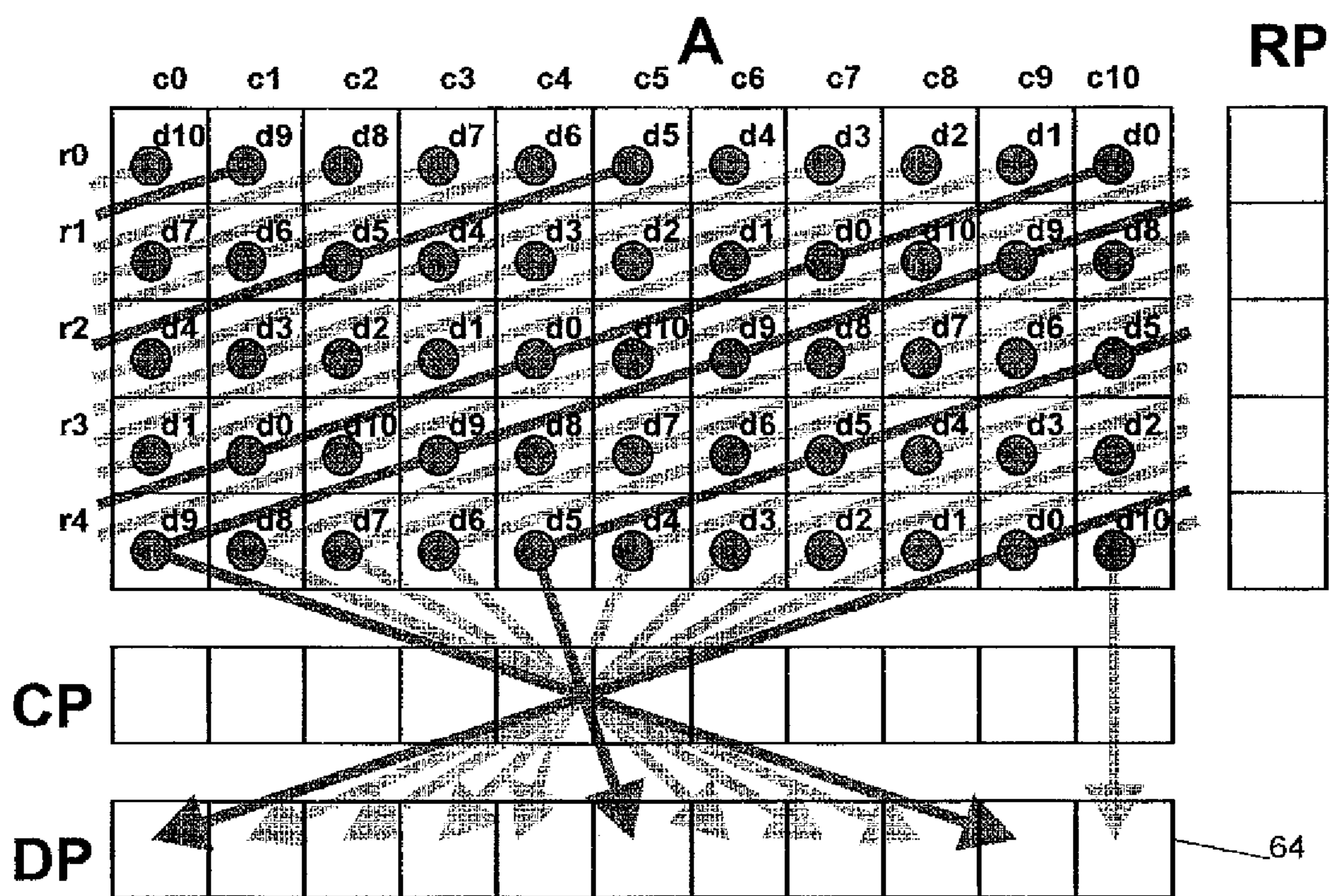
Figure 3C Transmitter Computation of diagonal parity packets
