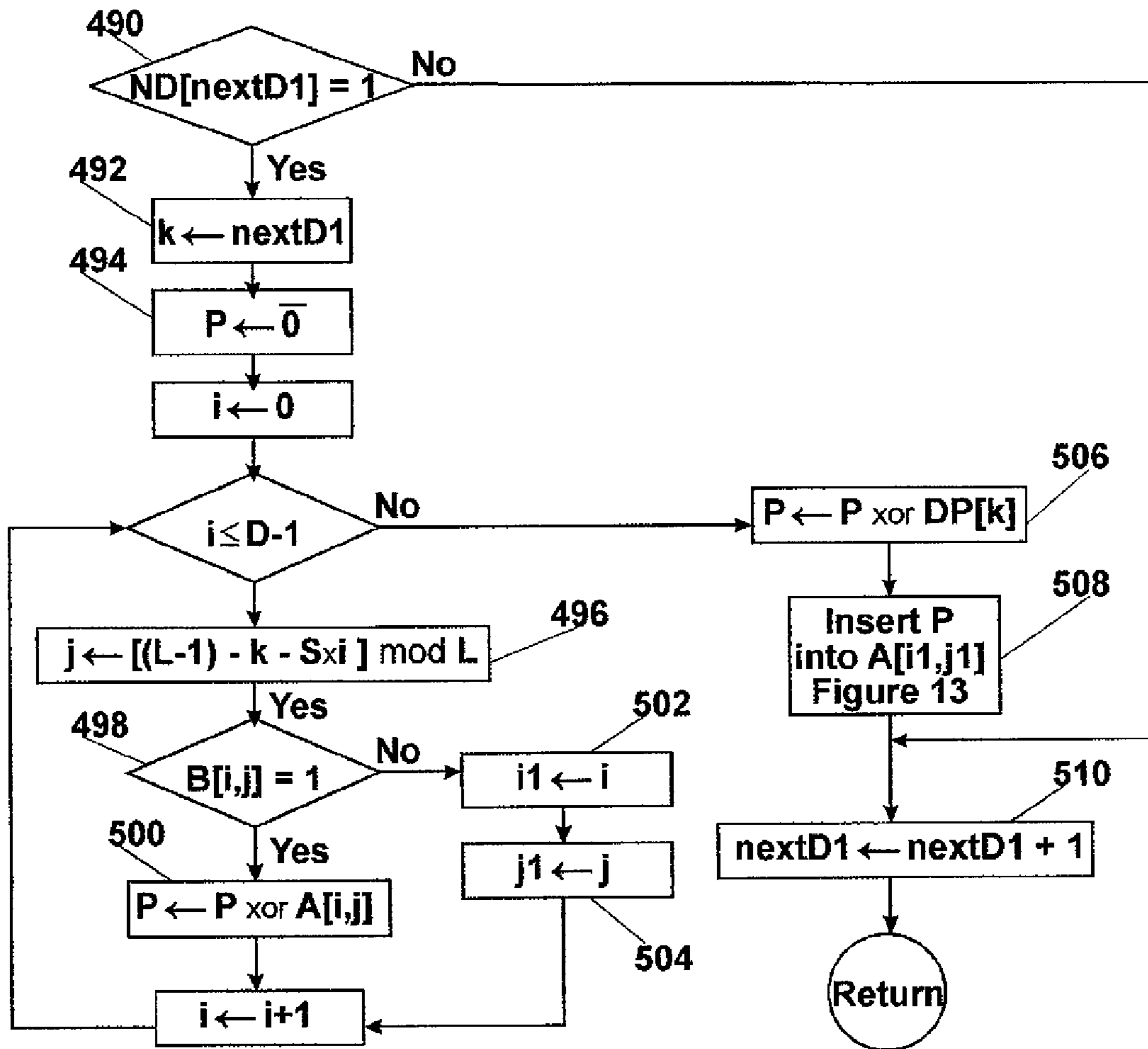
Figure 19C Receiver Correct D1[nextD1]
