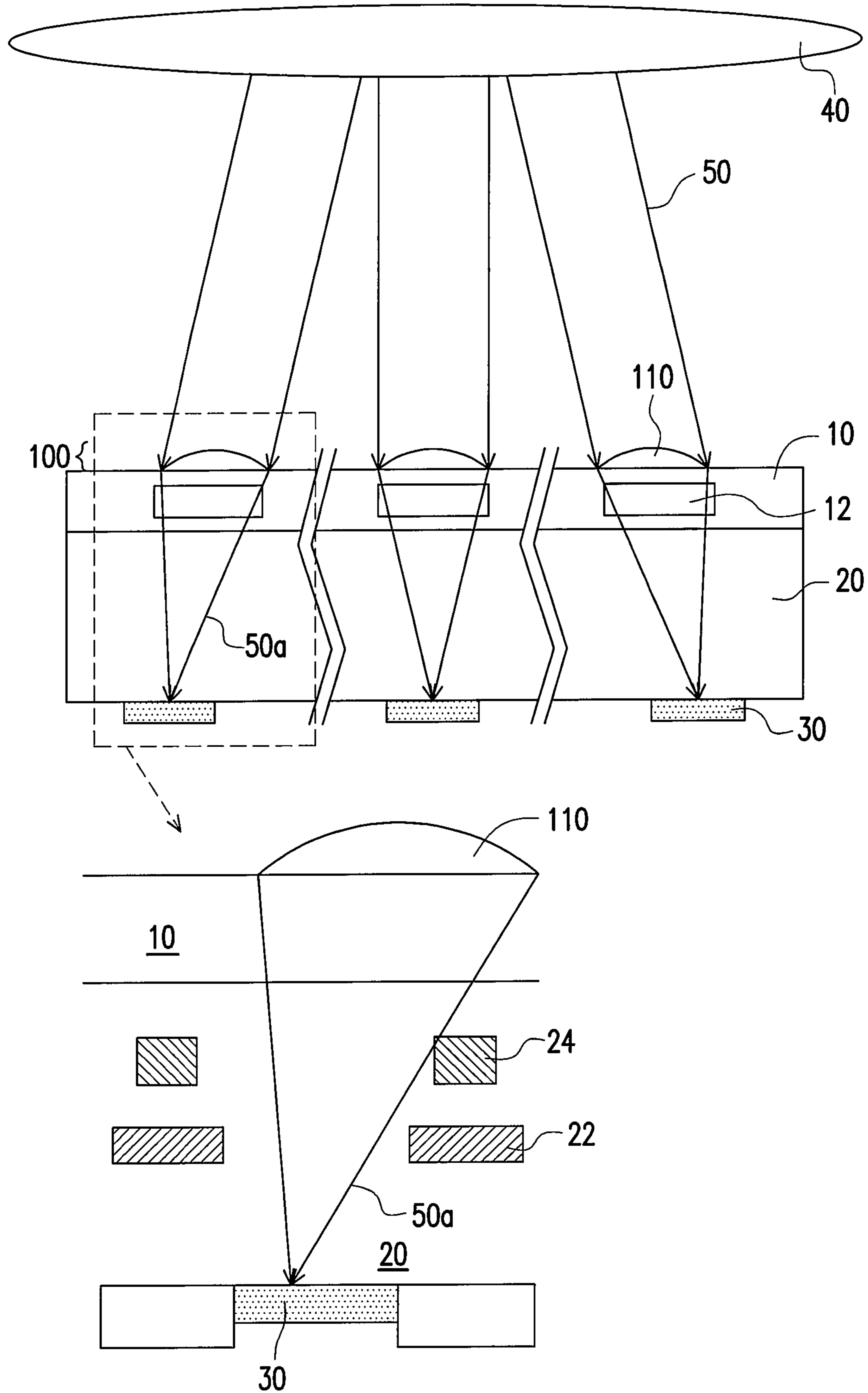
FIG. 2 (PRIOR ART)
