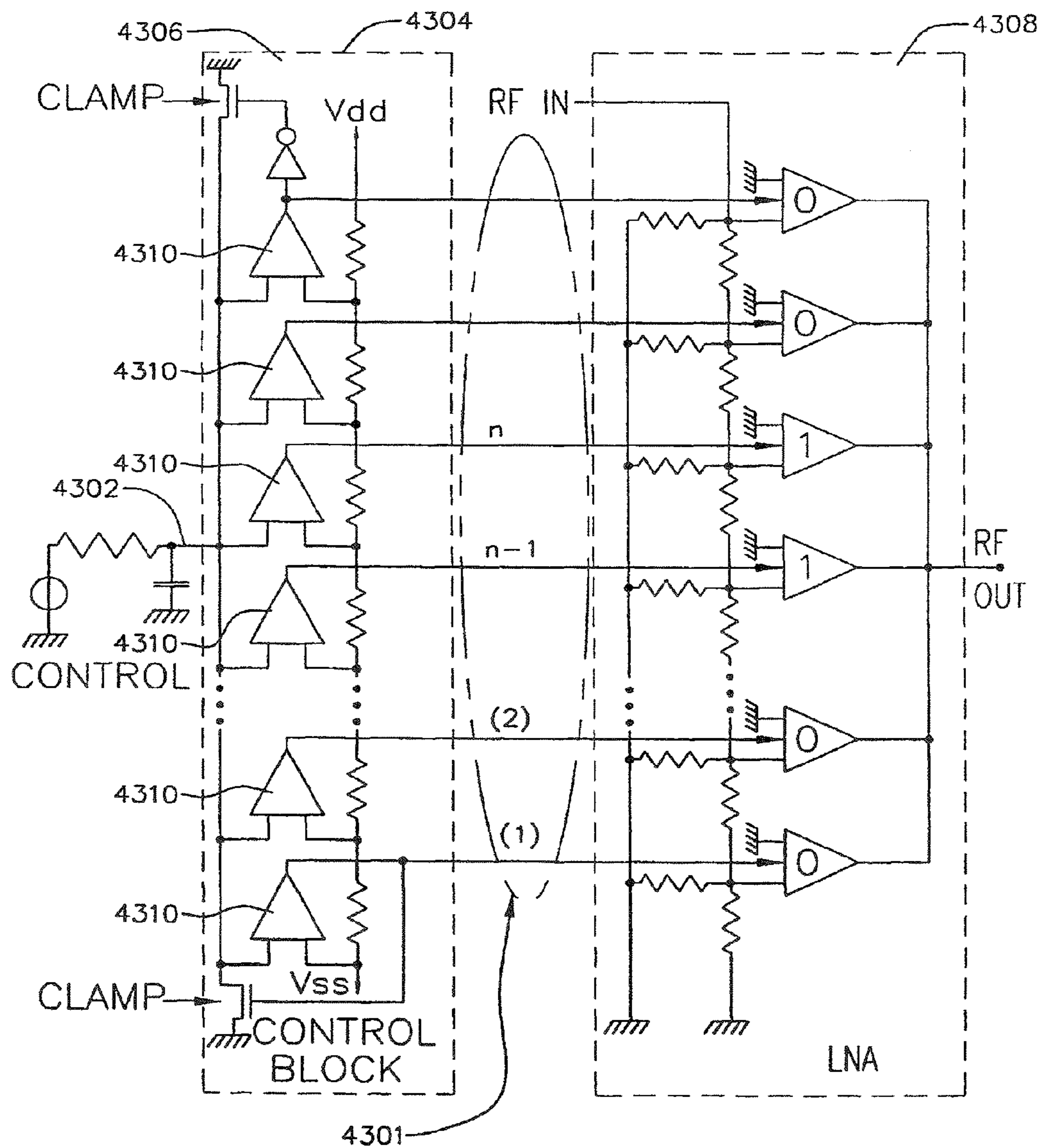
FIG. 43 CLAMPING CONTROL RANGE
