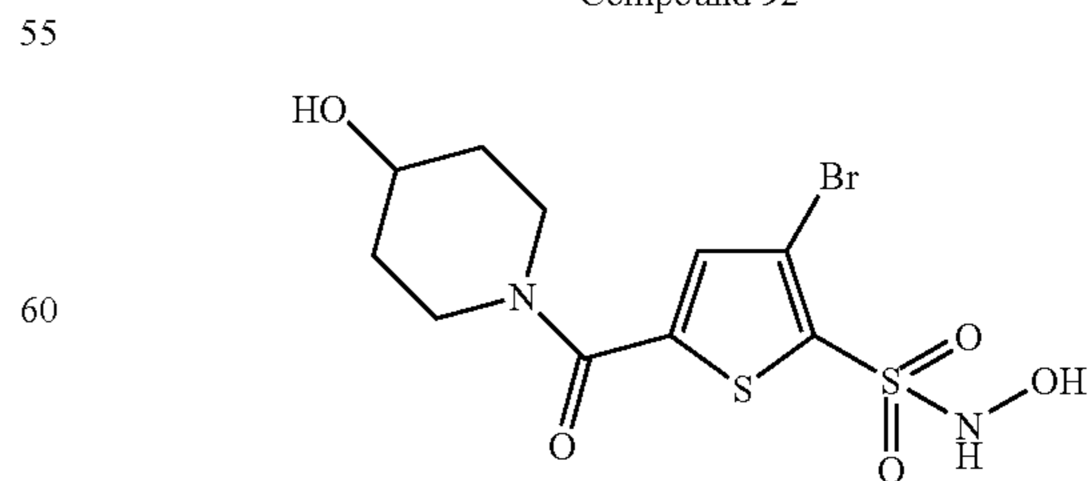
Compound 92
