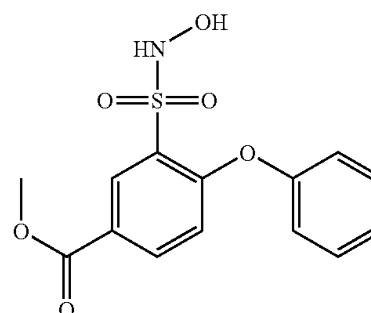
Compound 48
