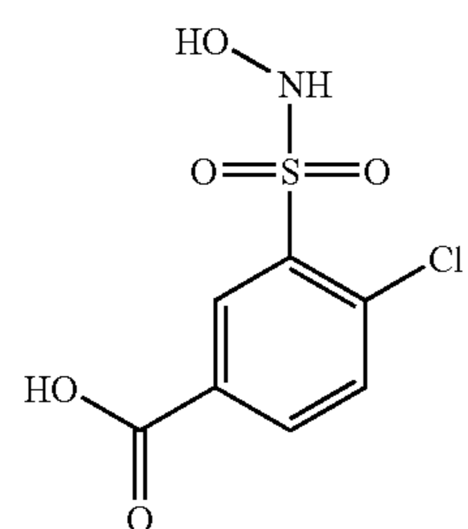
Compound 3
