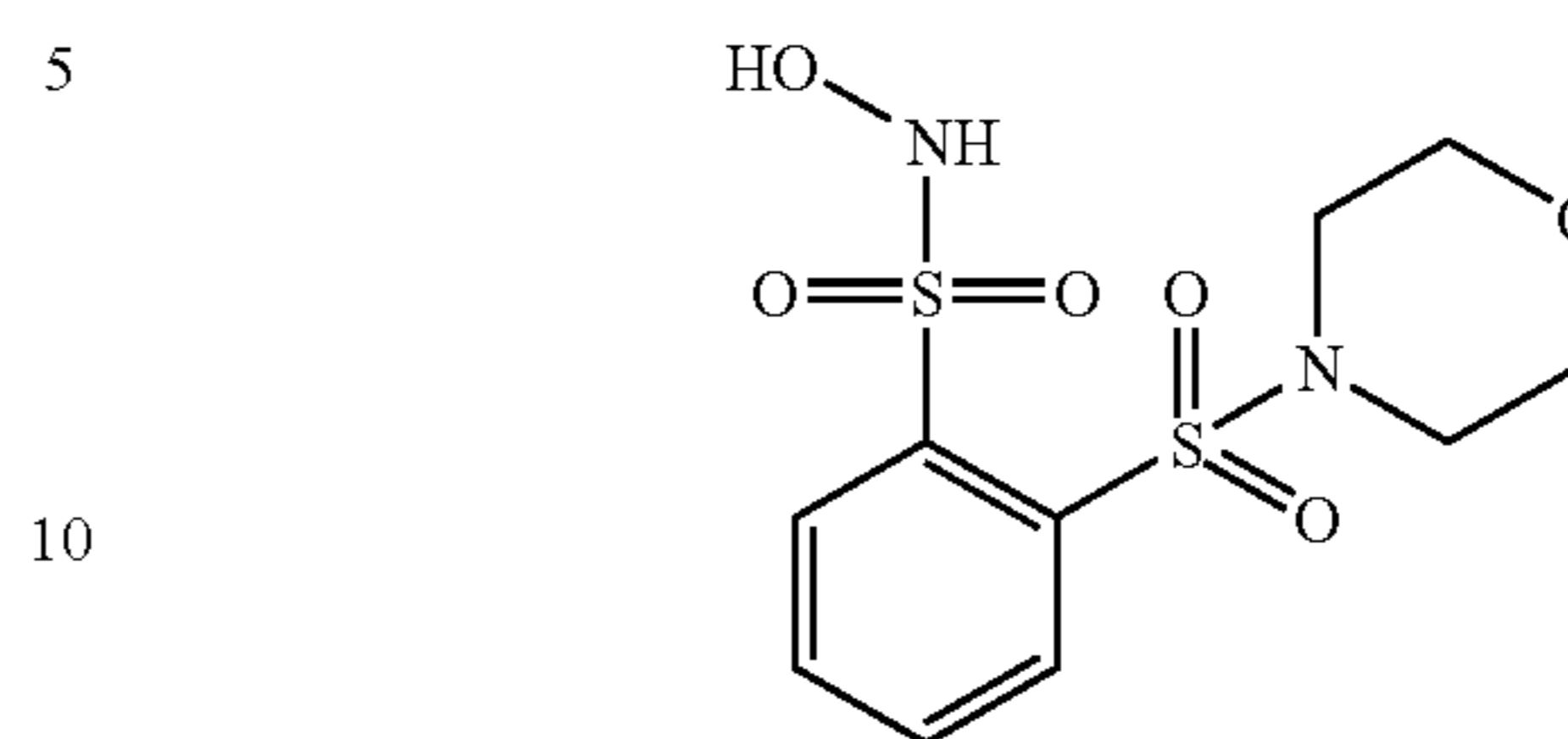
Compound 8
