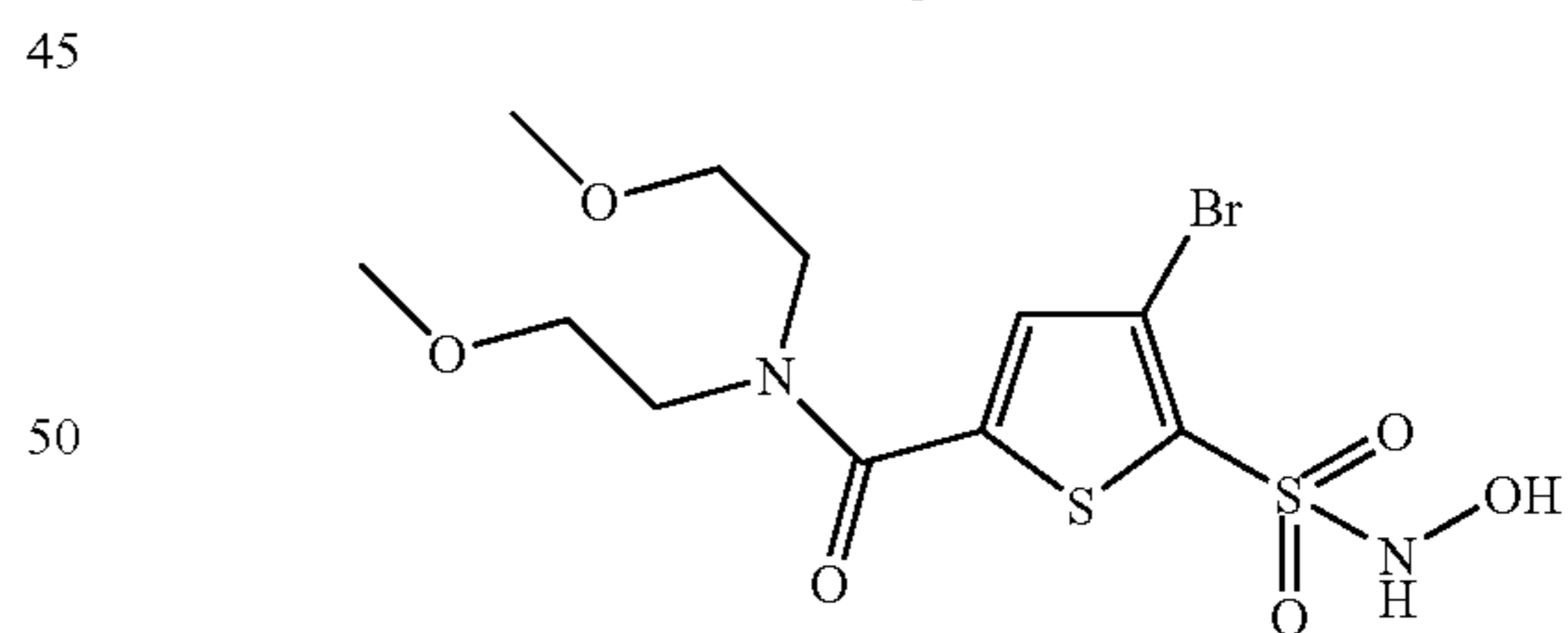
Compound 91
