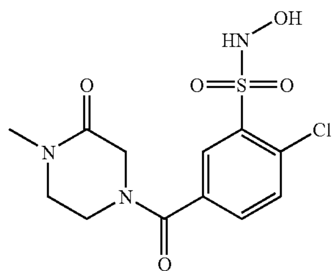
Compound 24
