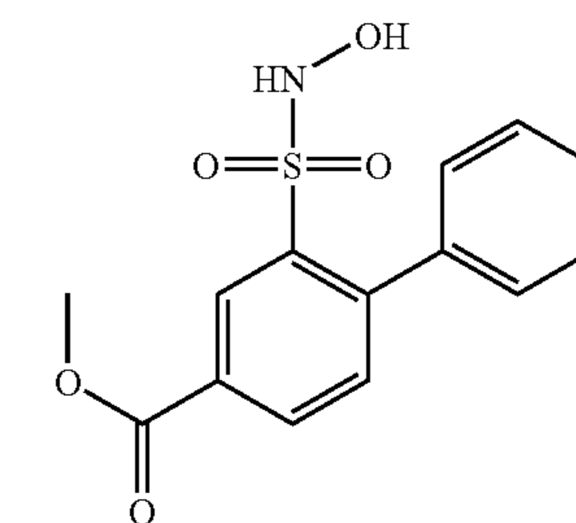
Compound 40
