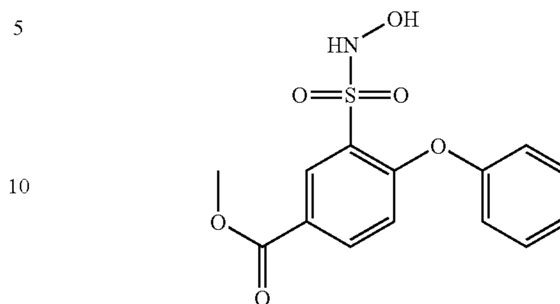
Compound 48
