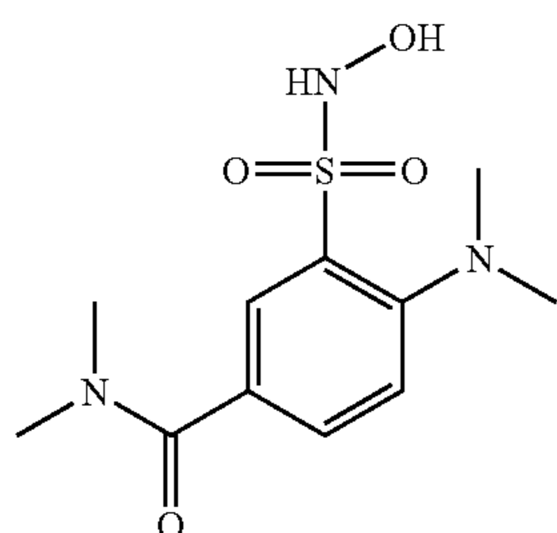
Compound 47
