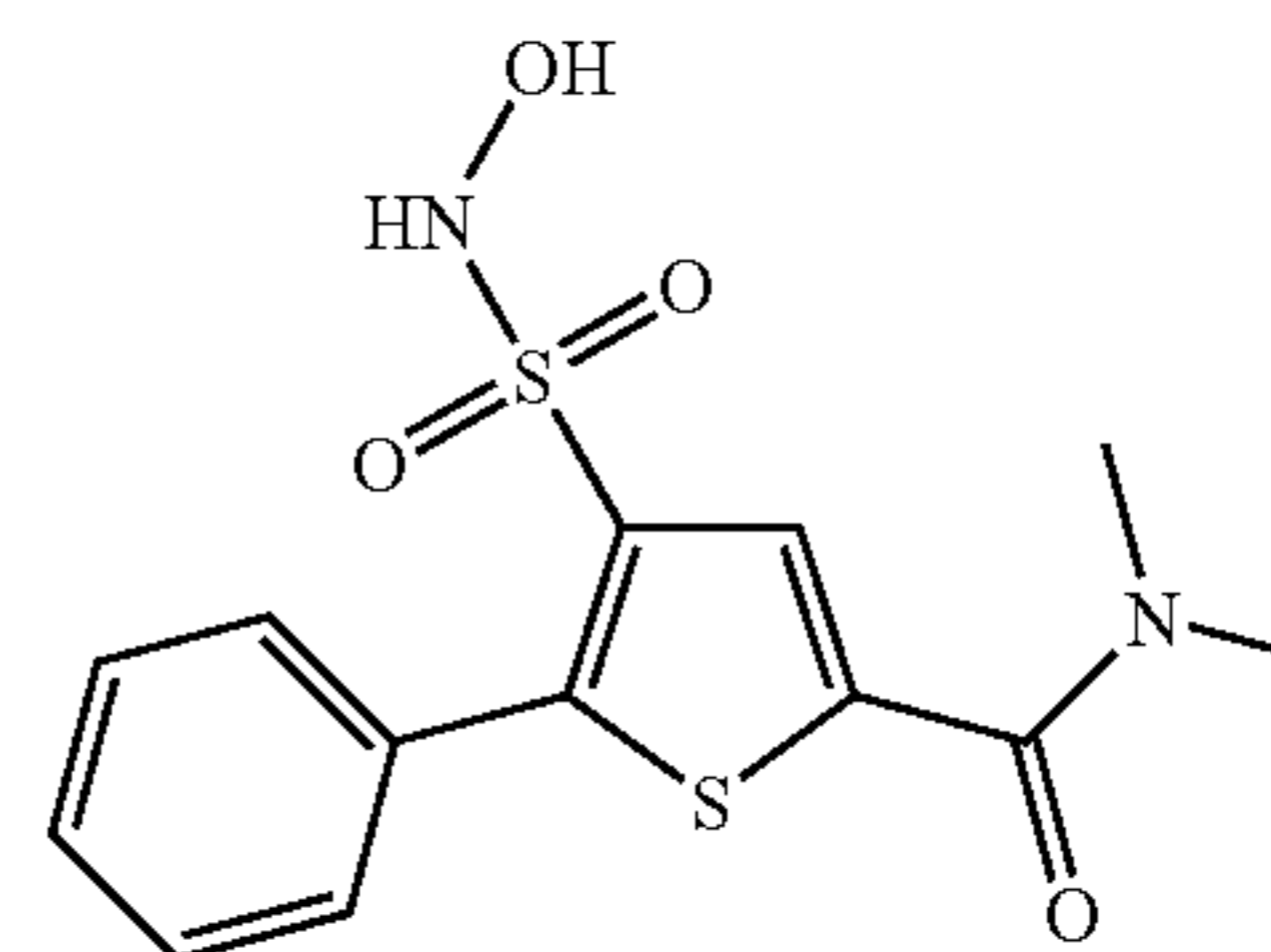
Compound 81
