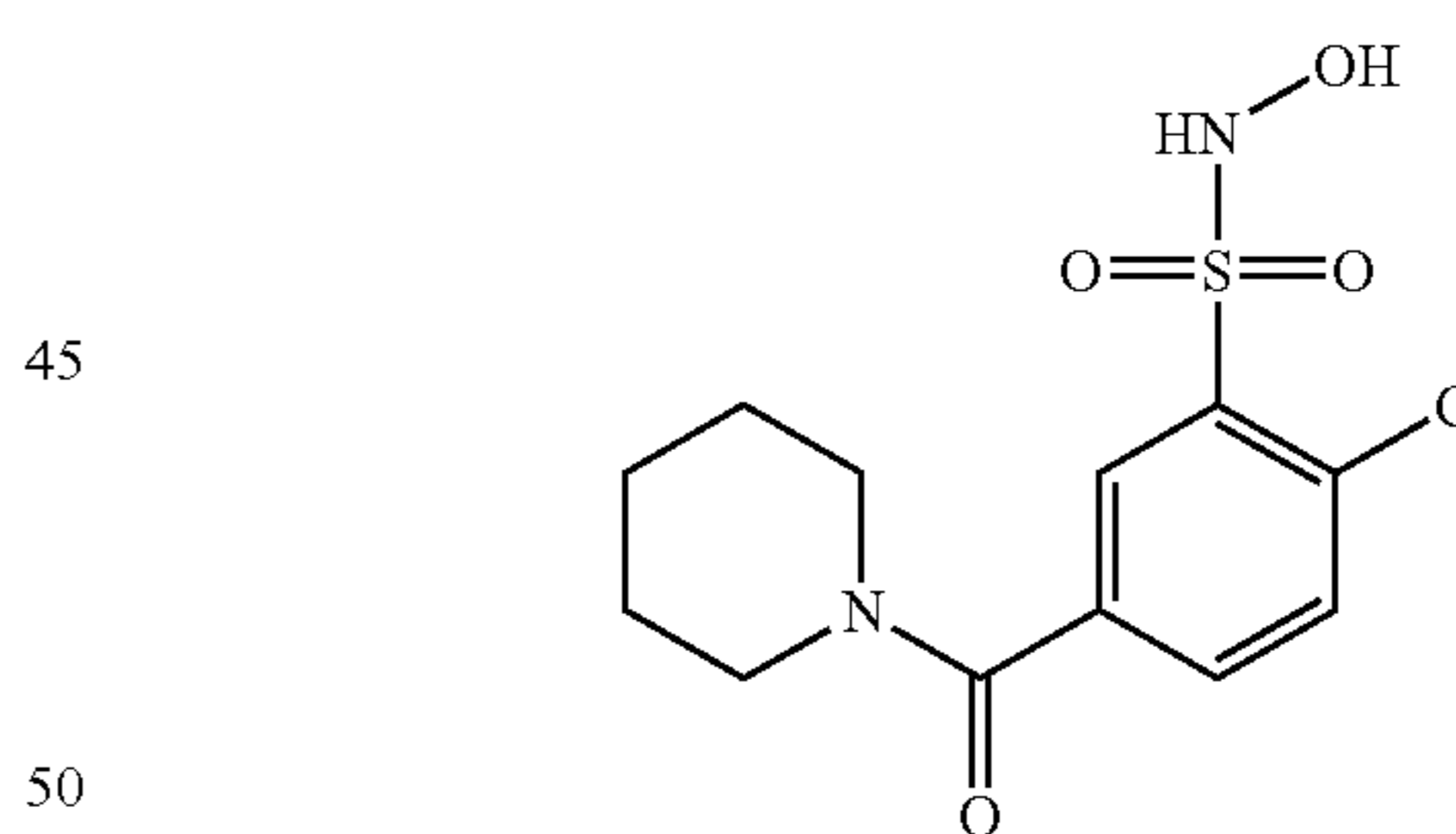
Compound 11
