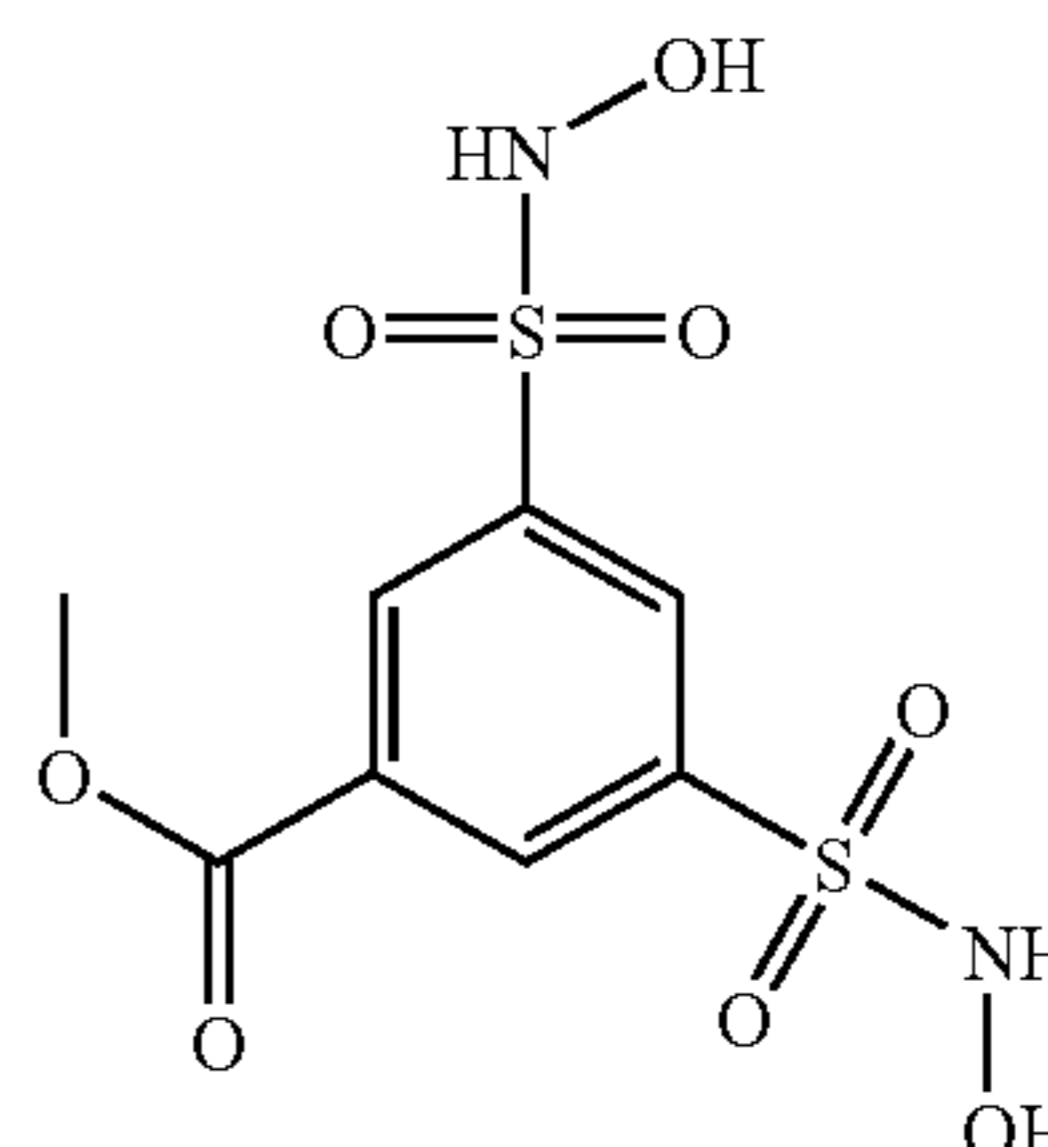
Compound 62
