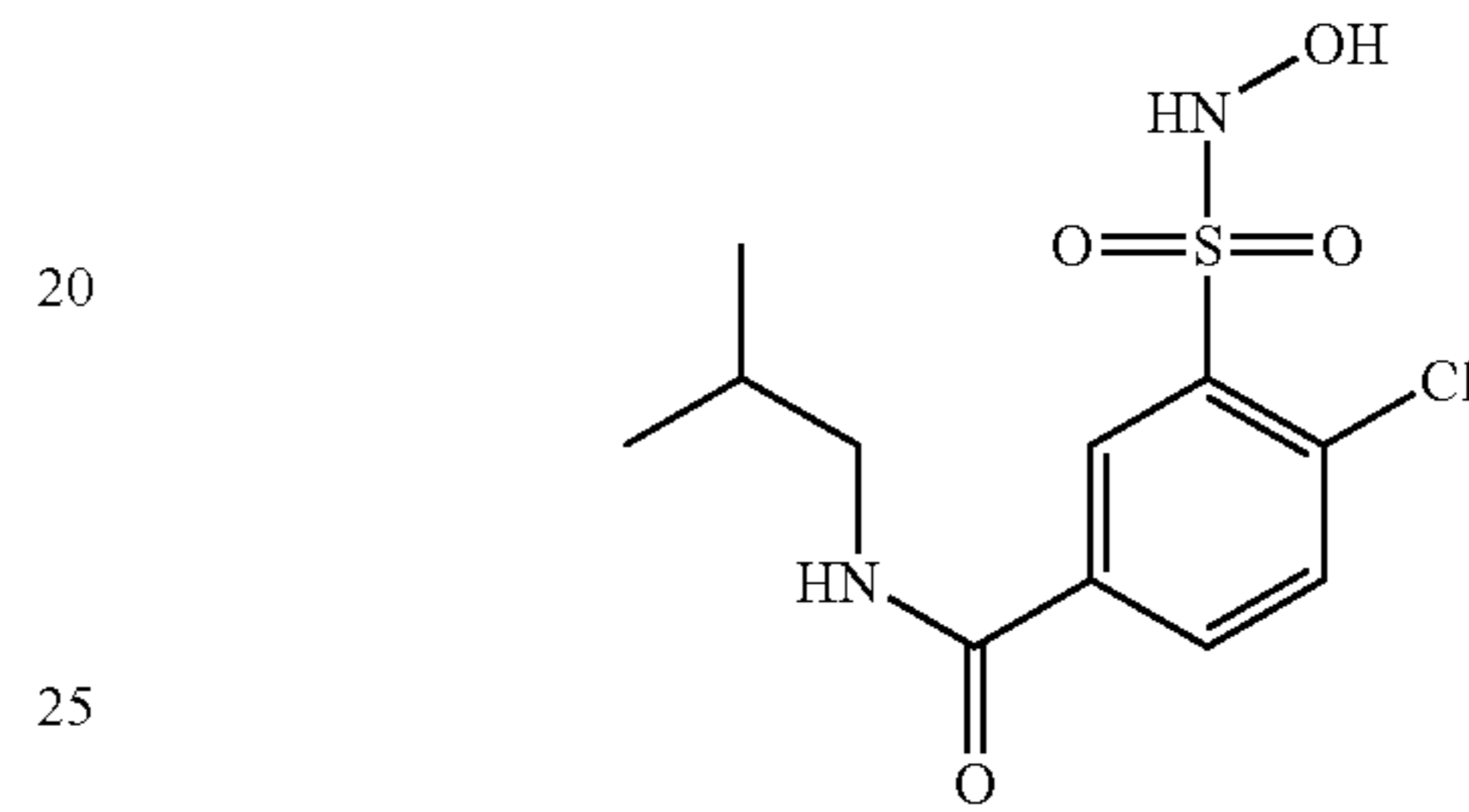
Compound 29
