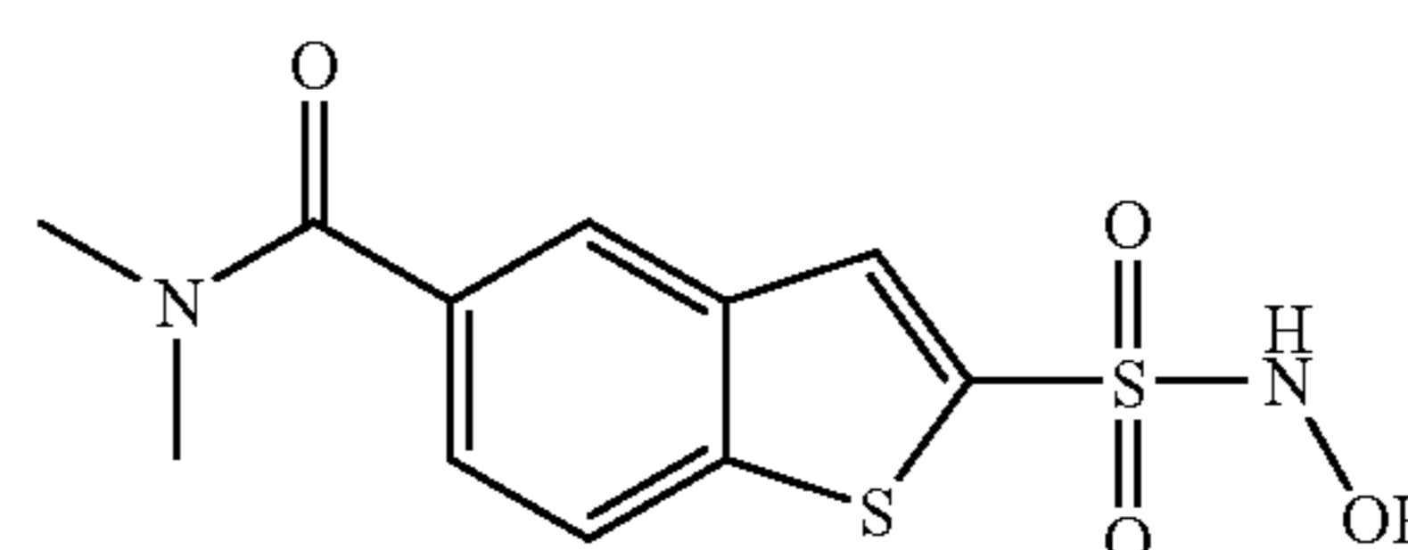
Compound 73
