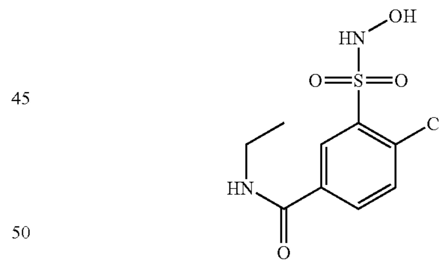
Compound 31
