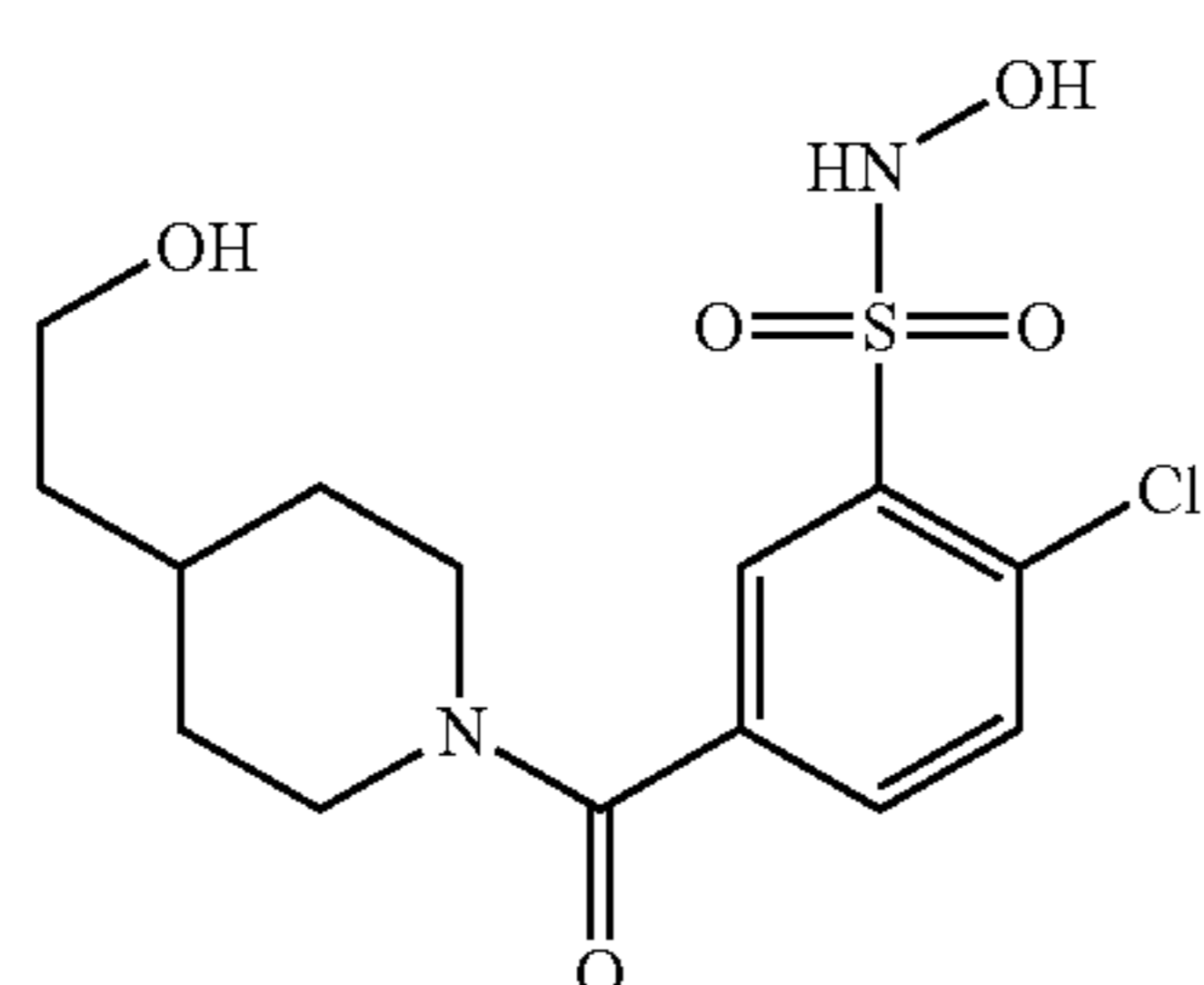
Compound 17
