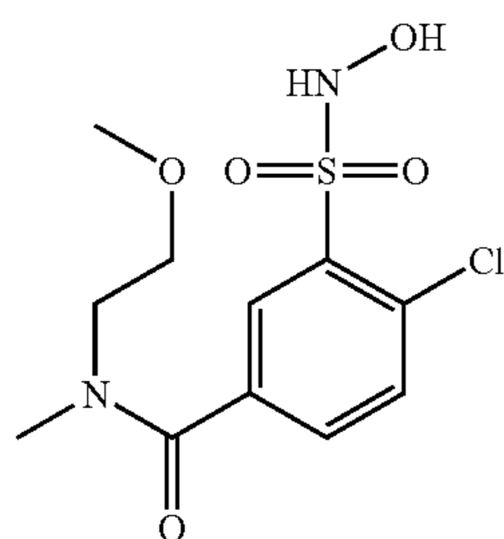
Compound 33
