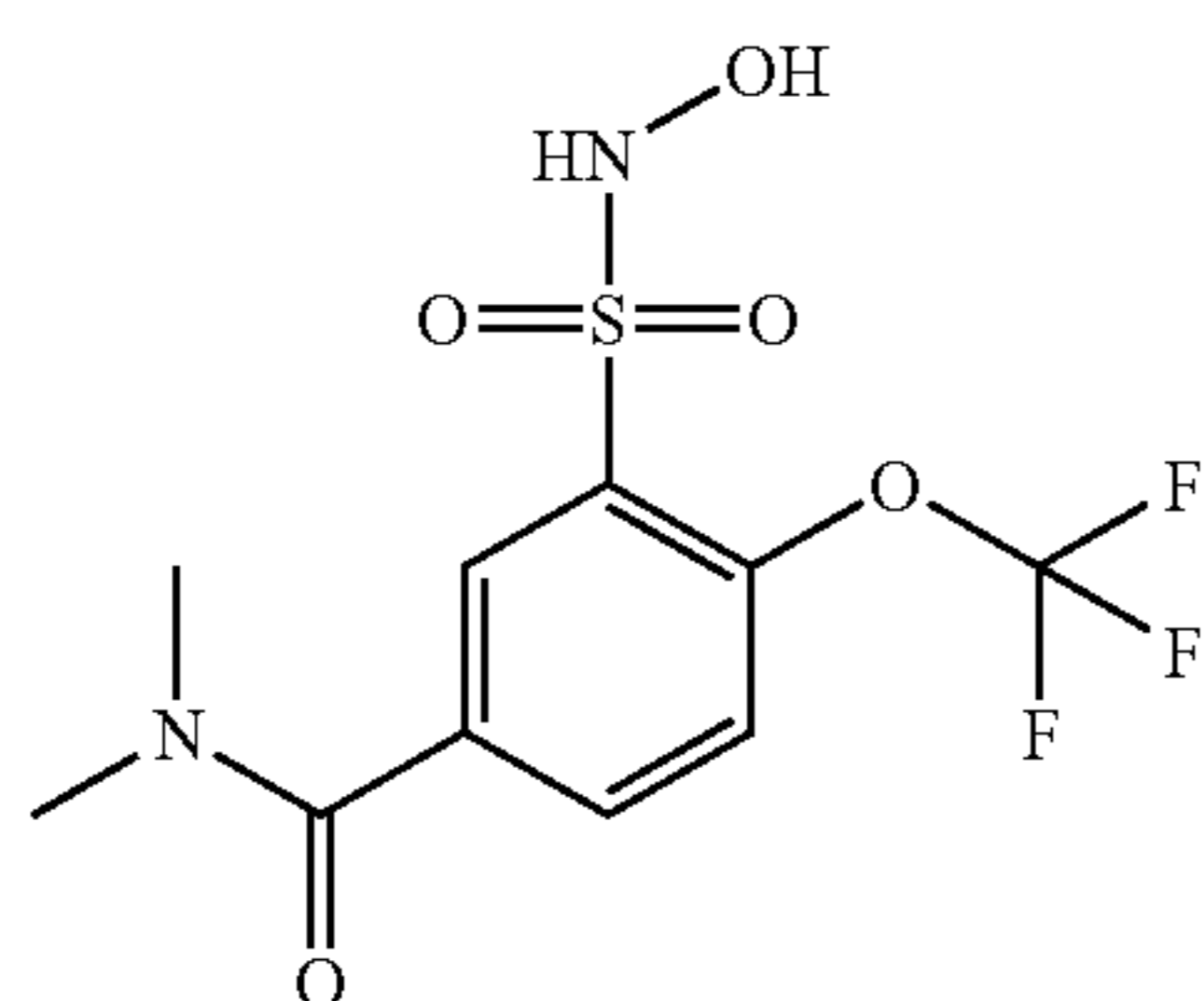
Compound 45
