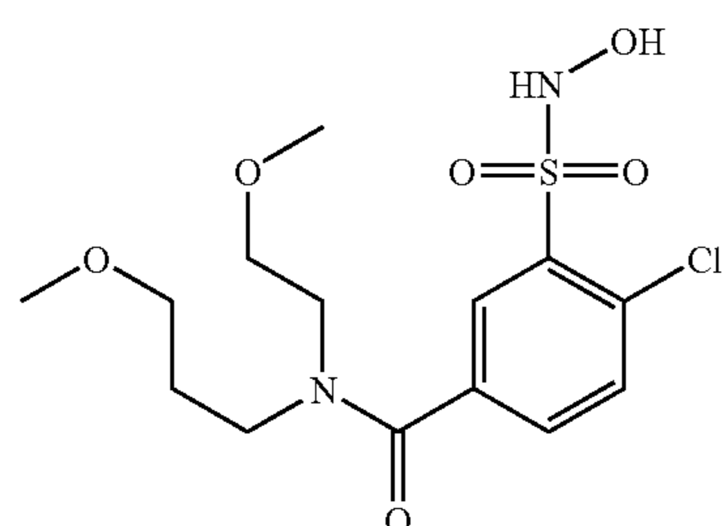
Compound 37
