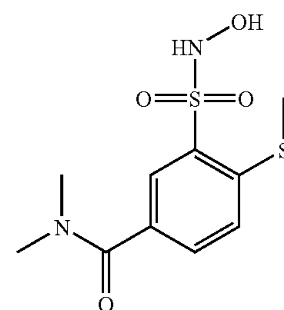
Compound 39
