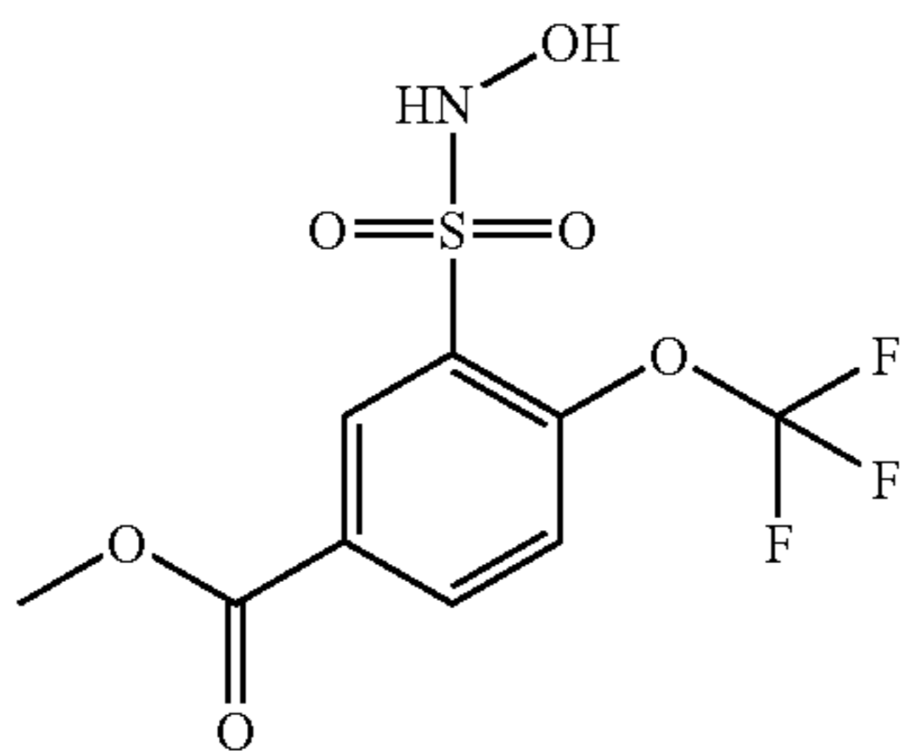
Compound 44
