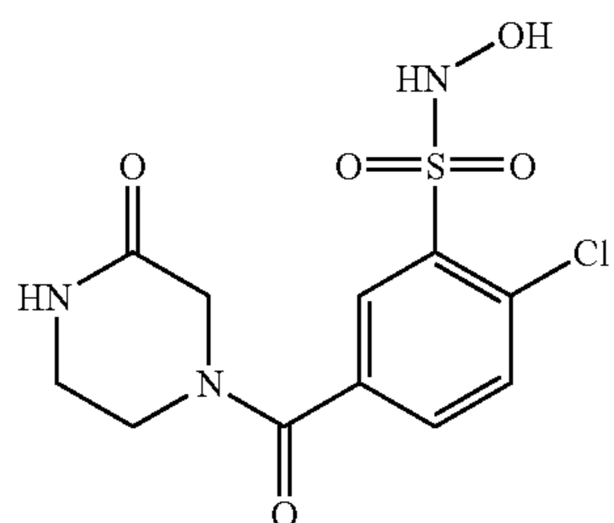
Compound 23
