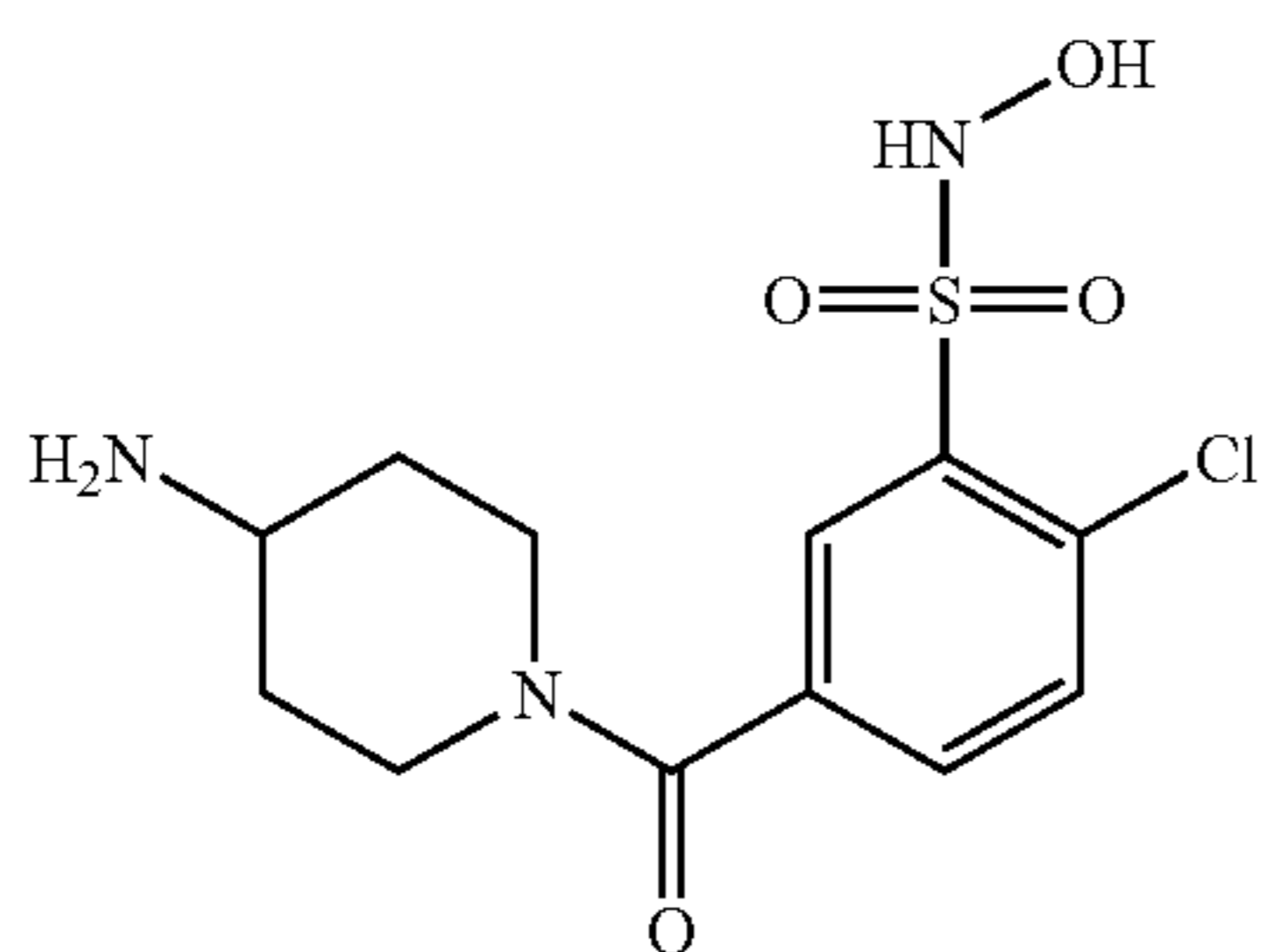
Compound 14
