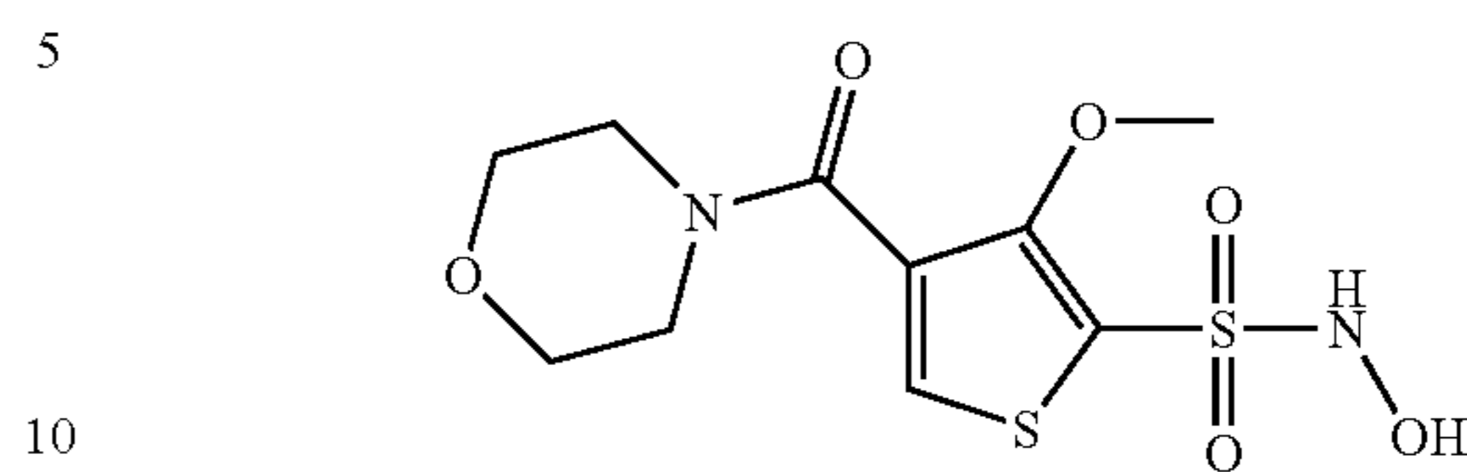
Compound 88
