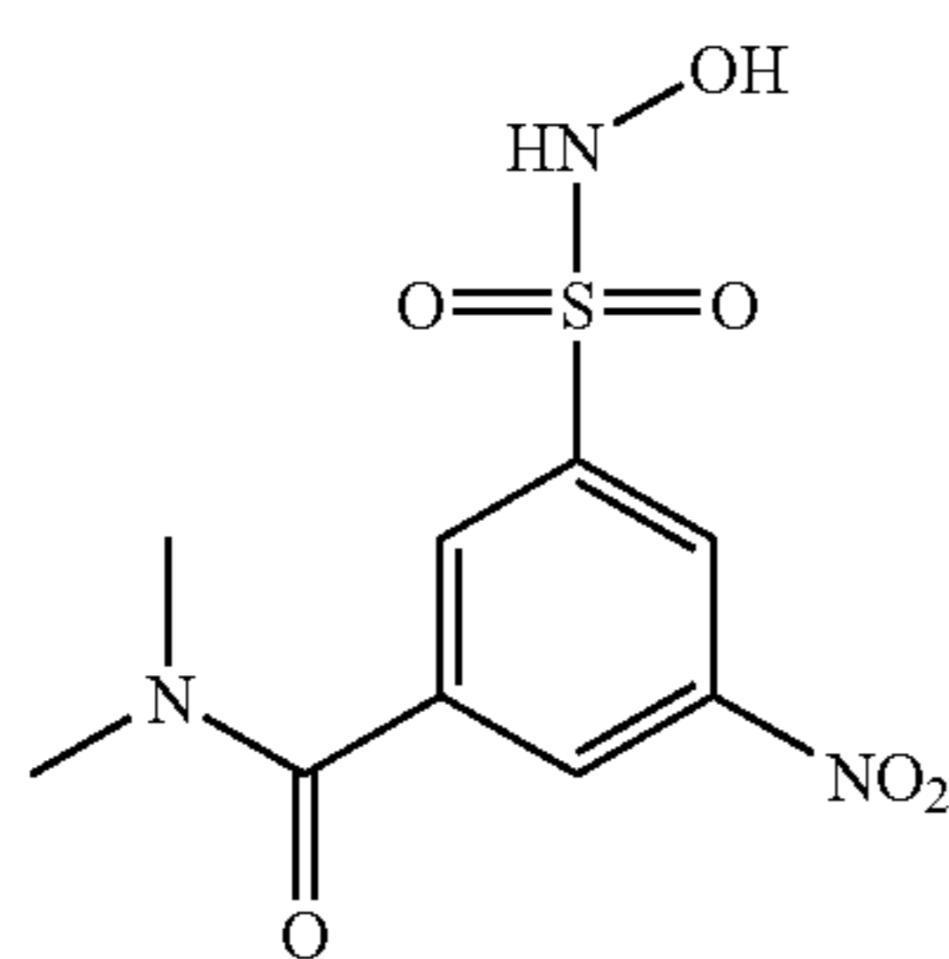
Compound 57
