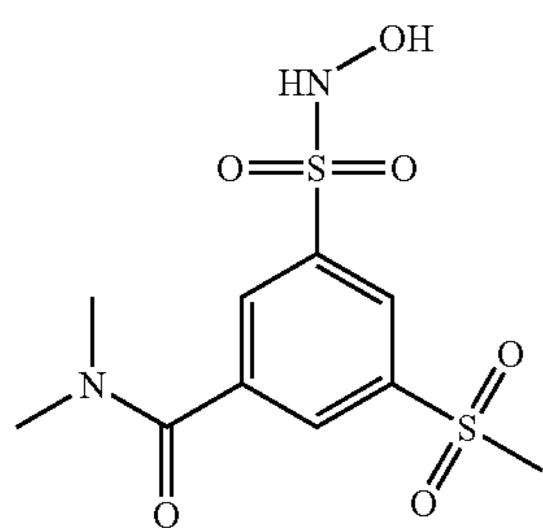
Compound 53
