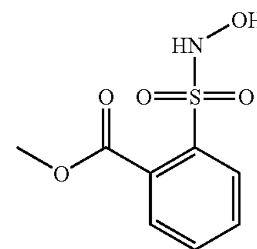
Compound 1
