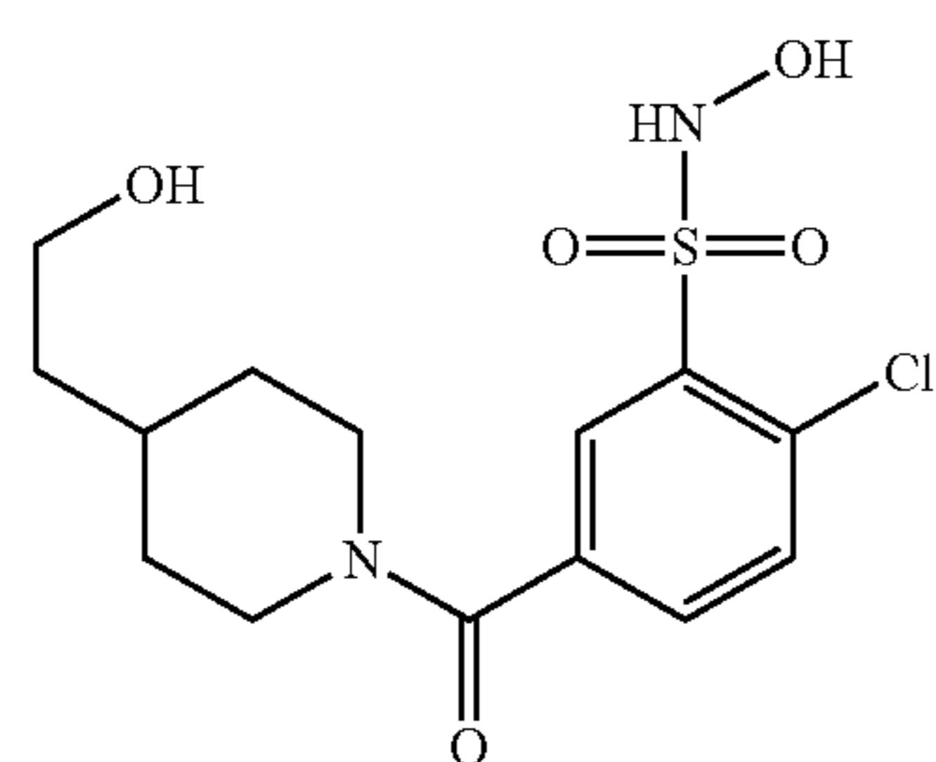
Compound 17
