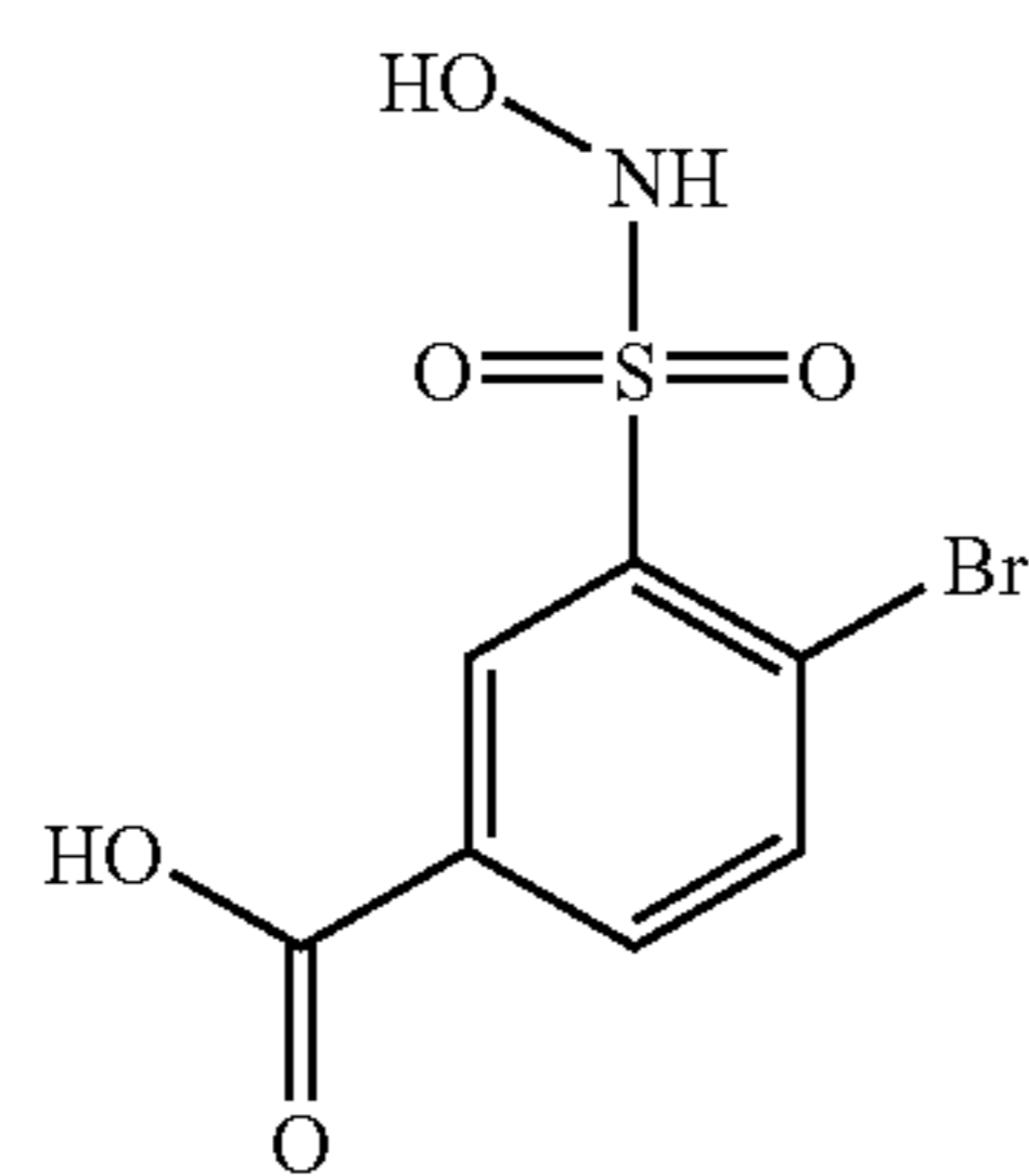
Compound 4
