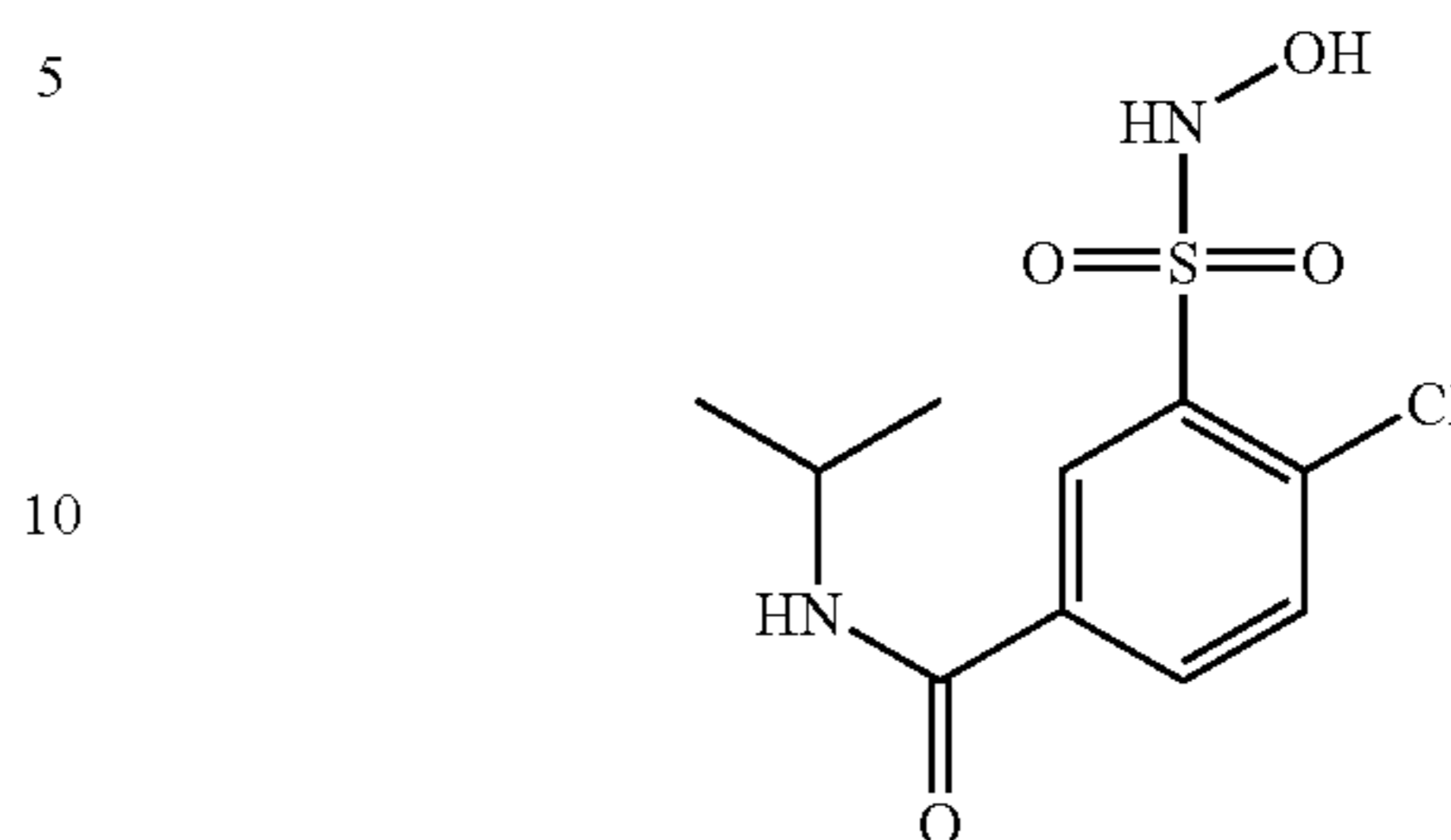
Compound 28
