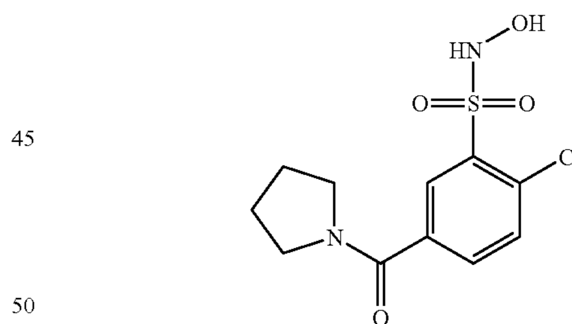
Compound 71
