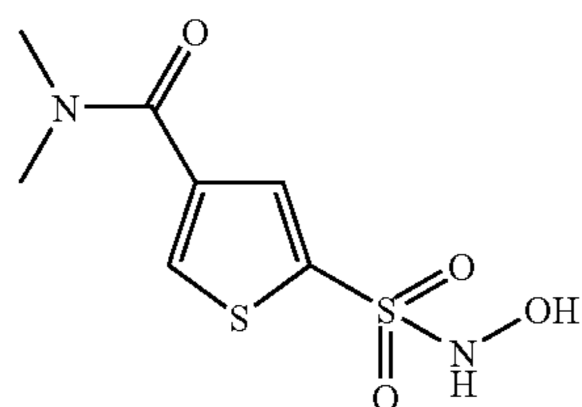
Compound 83
