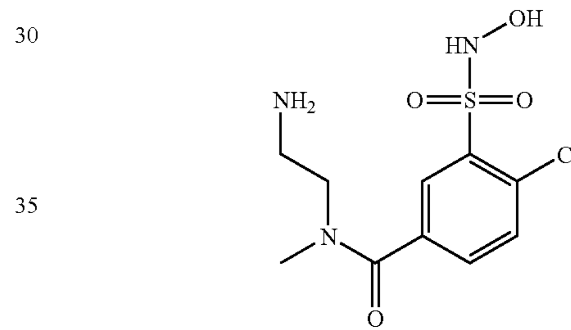
Compound 30
