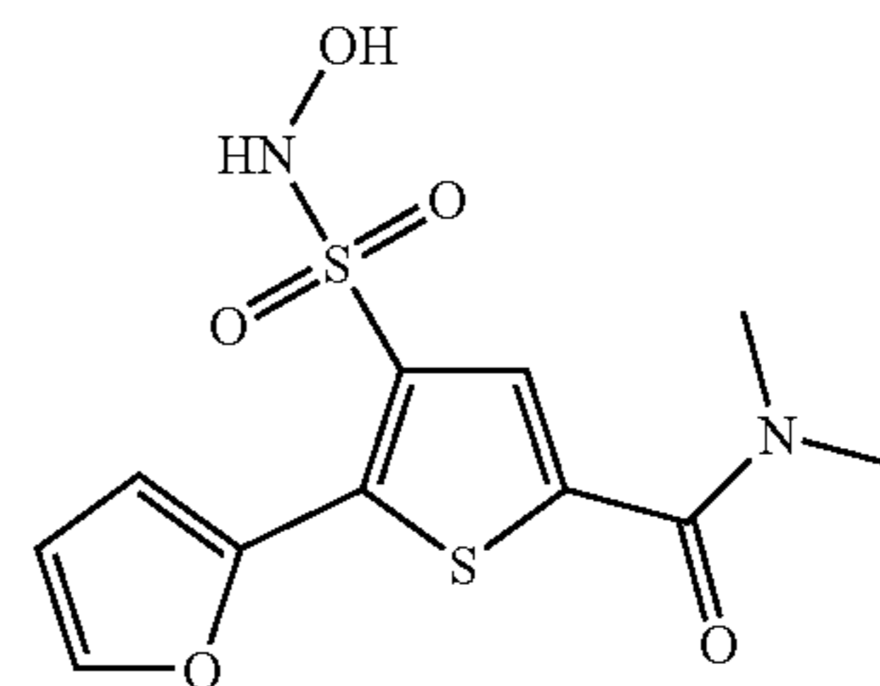
Compound 80
