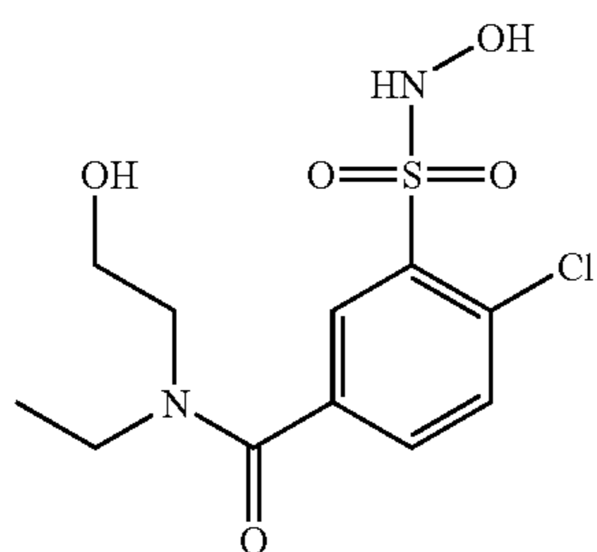
Compound 35
