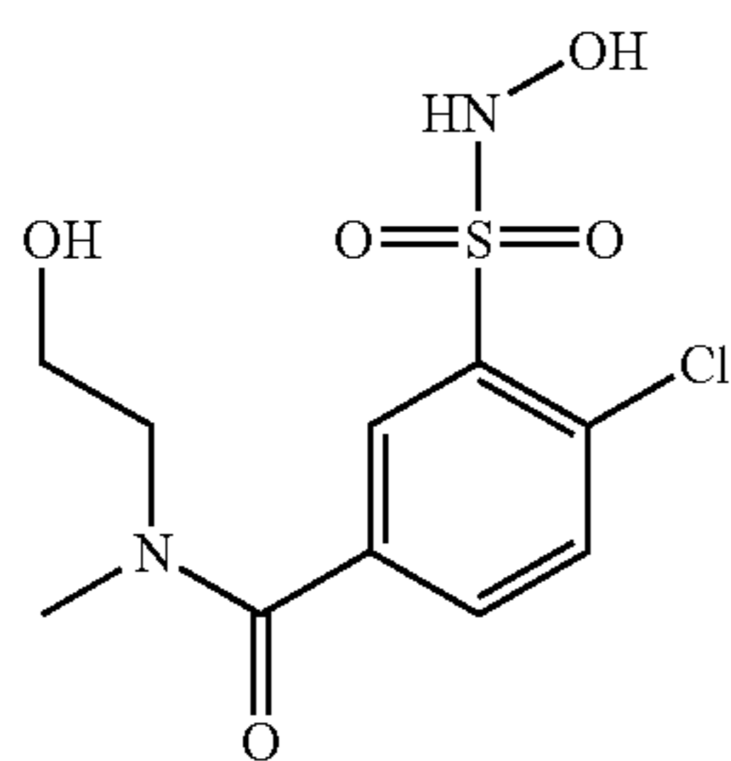
Compound 34
