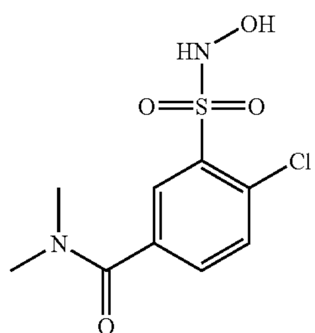
Compound 7
