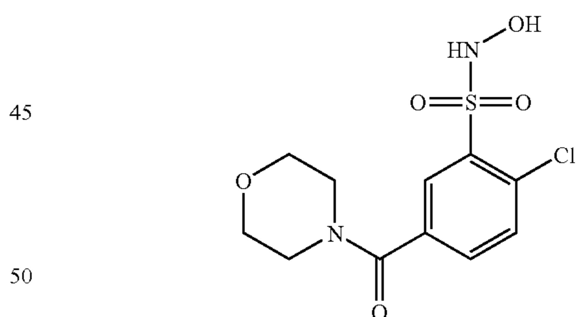
Compound 21
