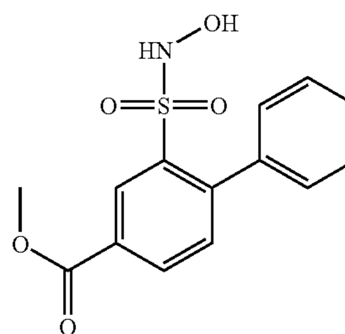
Compound 40
