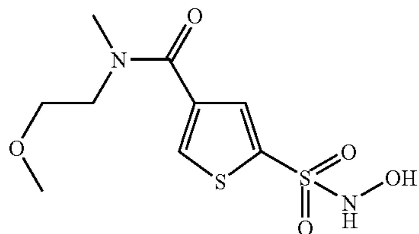
Compound 84
