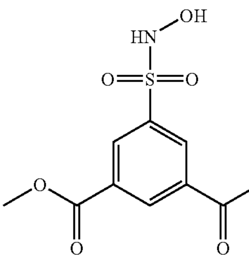
Compound 60
