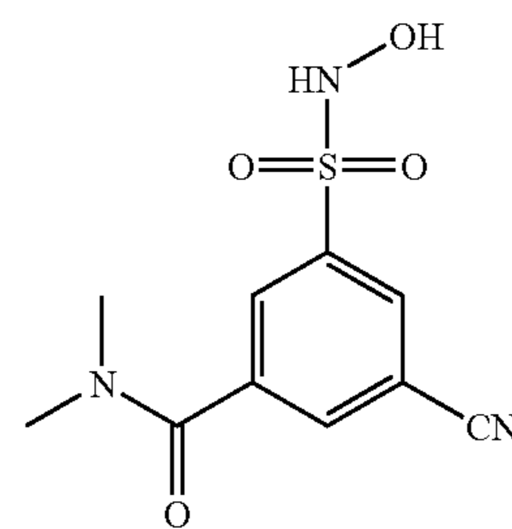
Compound 59
