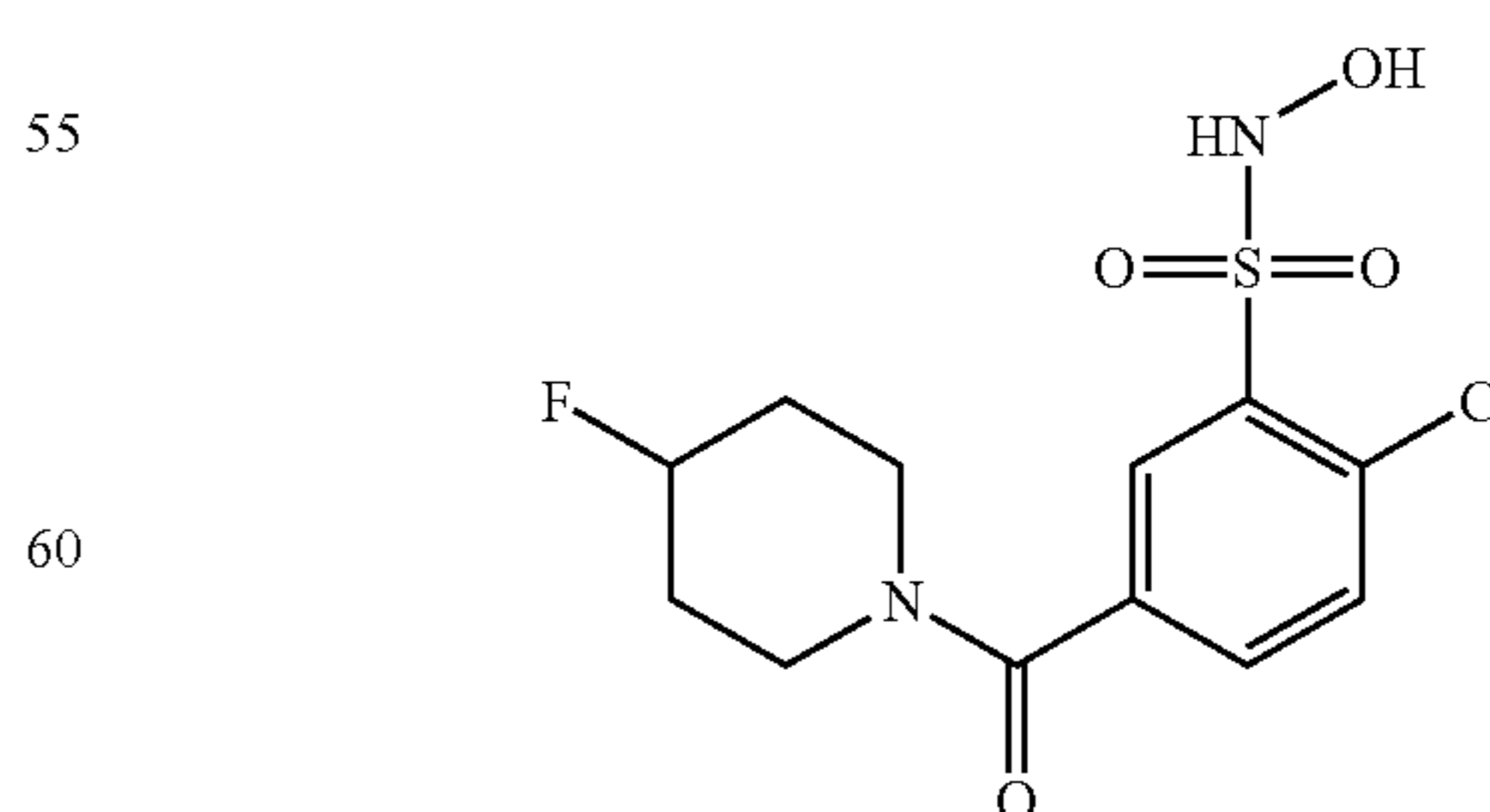
Compound 12
