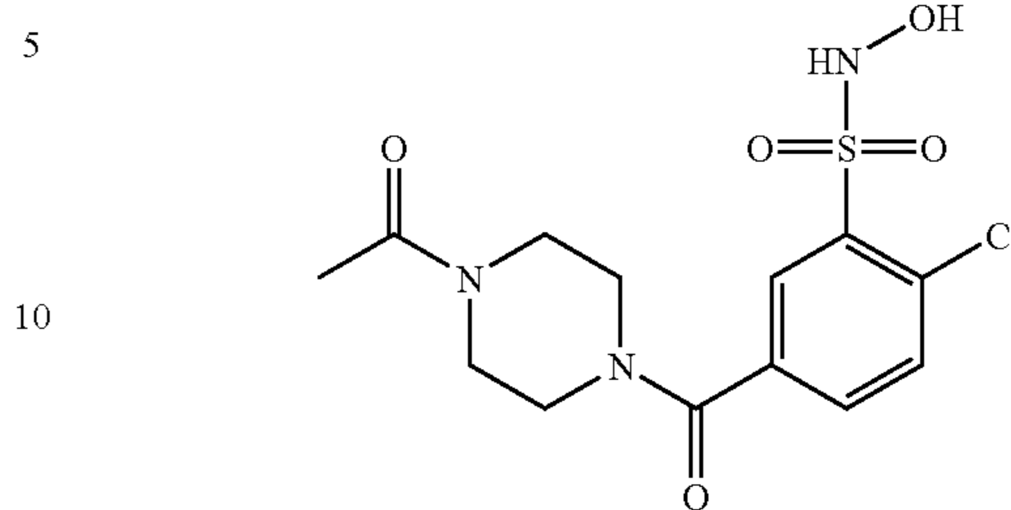
Compound 68
