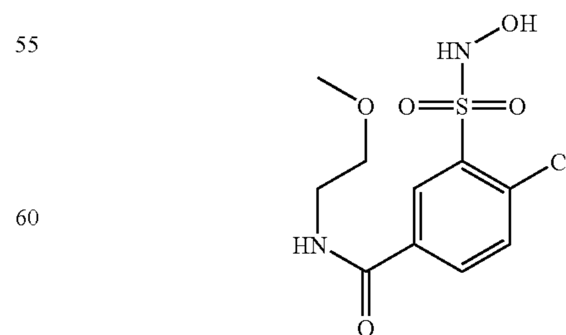
Compound 32
