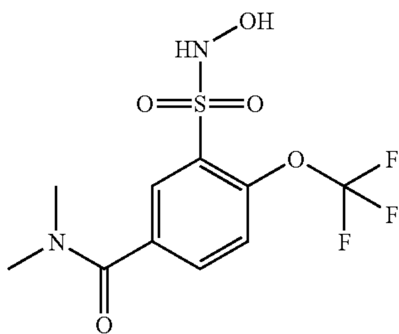
Compound 45
