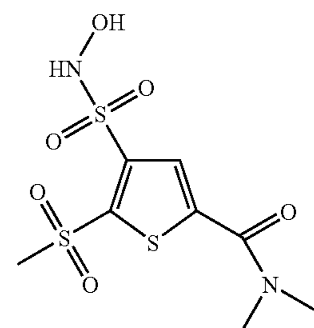
Compound 78
