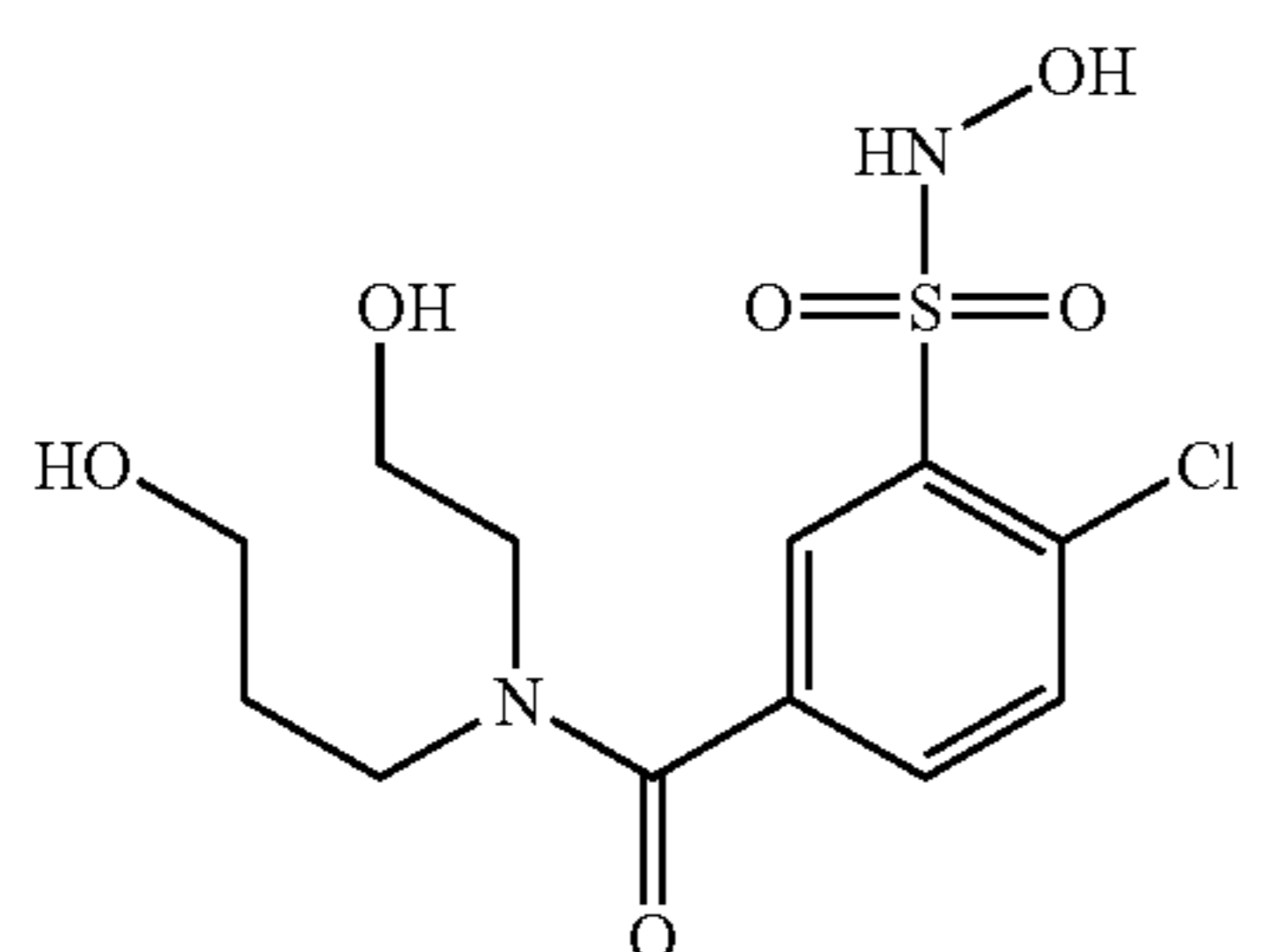
Compound 36
