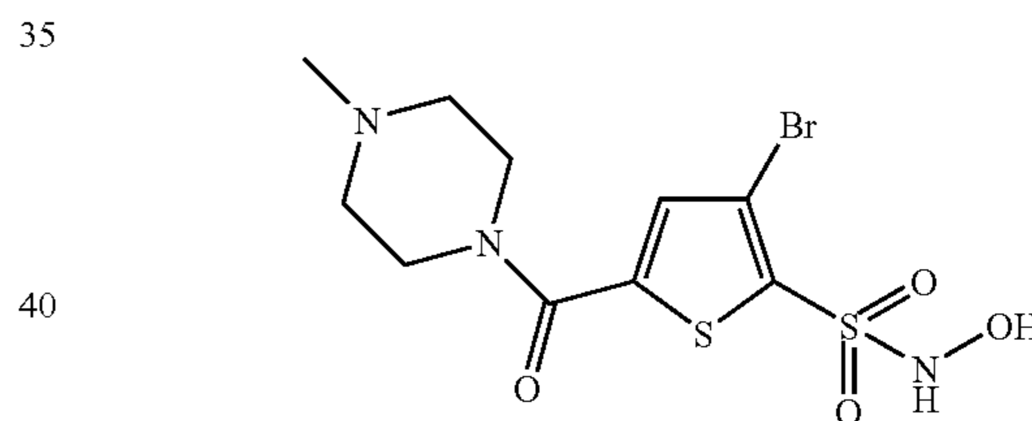
Compound 90
