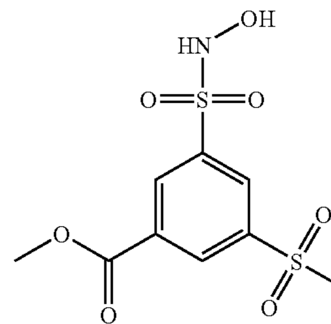
Compound 52
