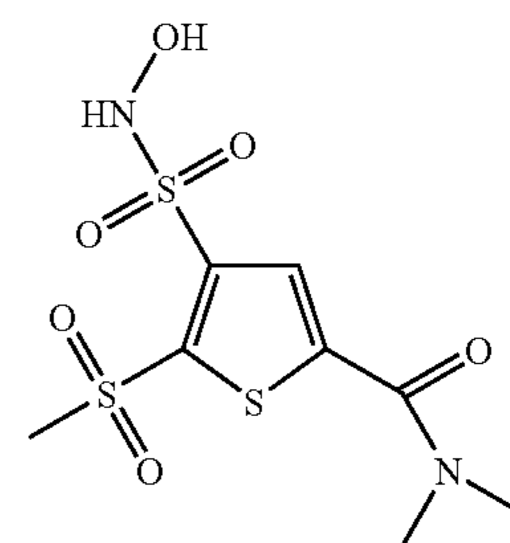
Compound 78
