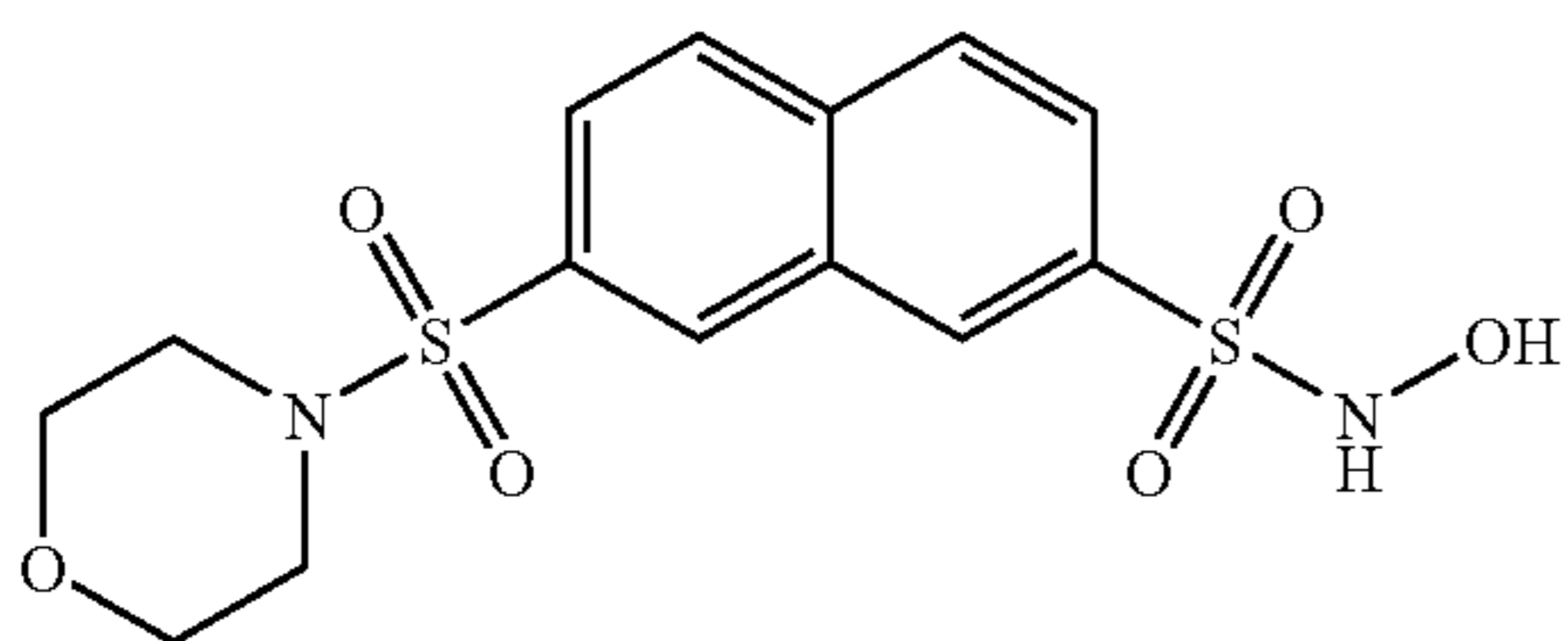
Compound 76
