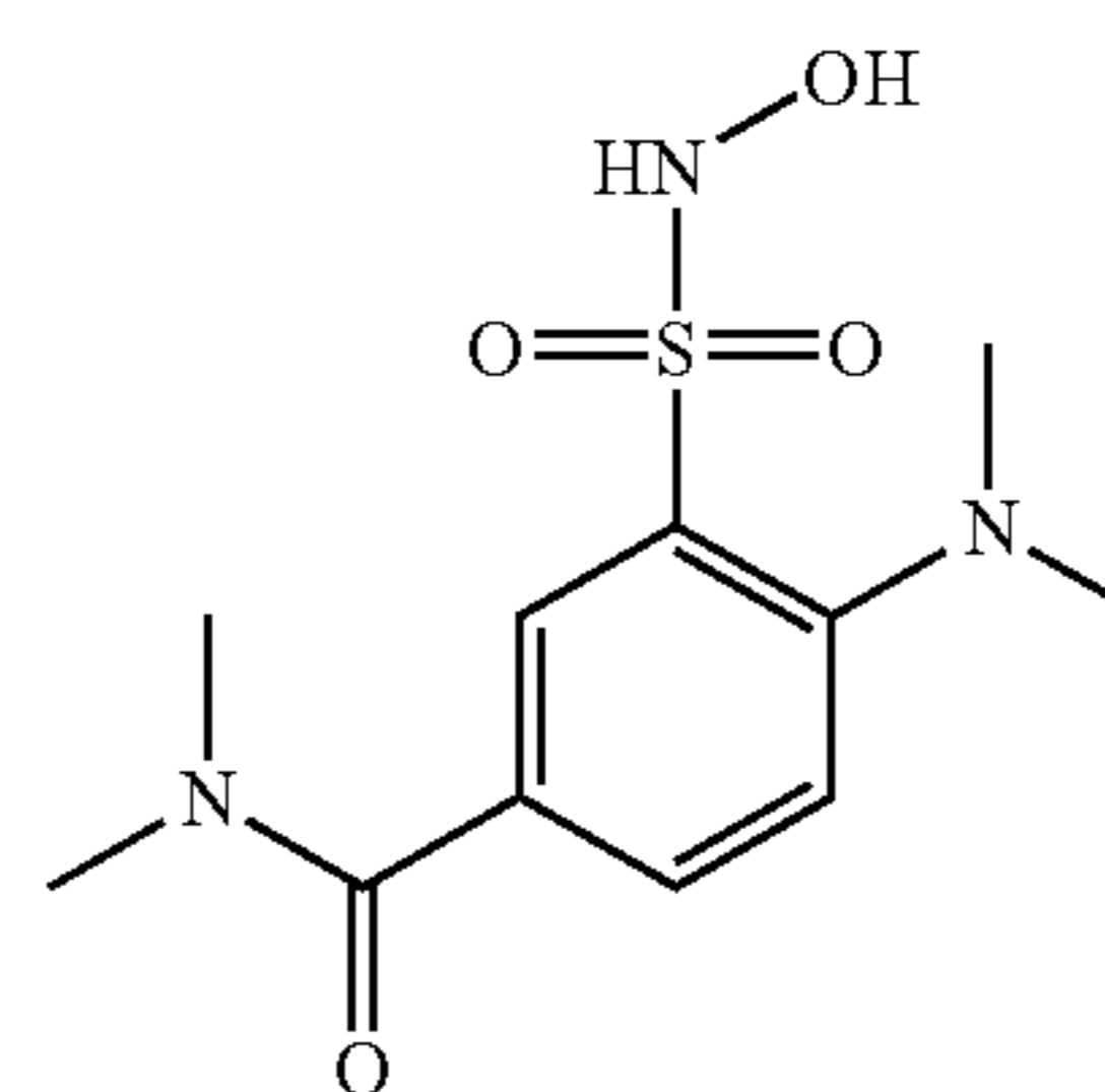
Compound 51
