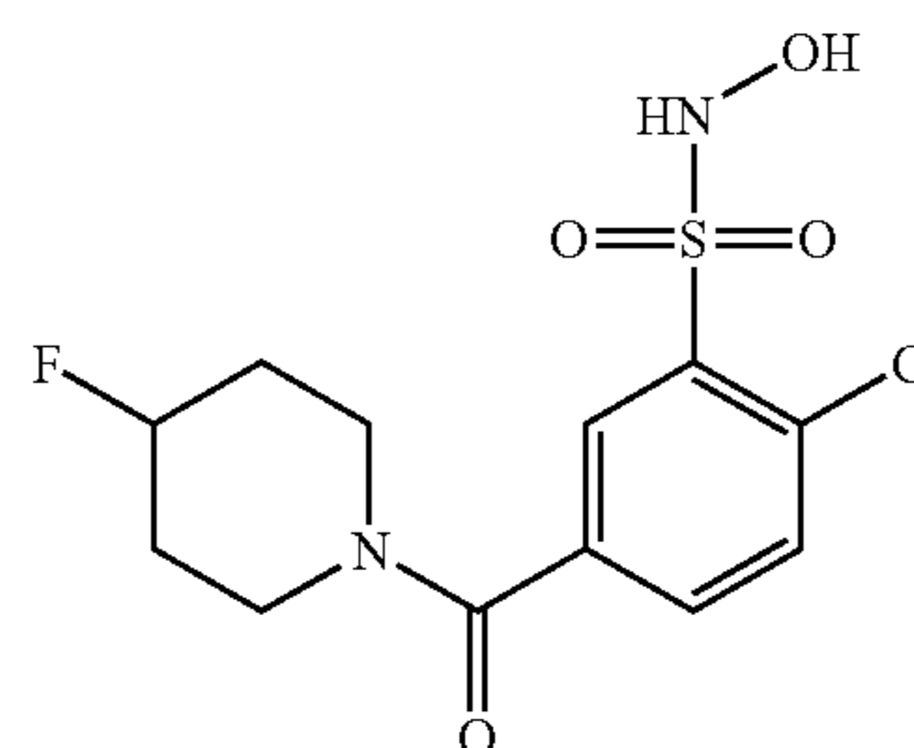
Compound 12
