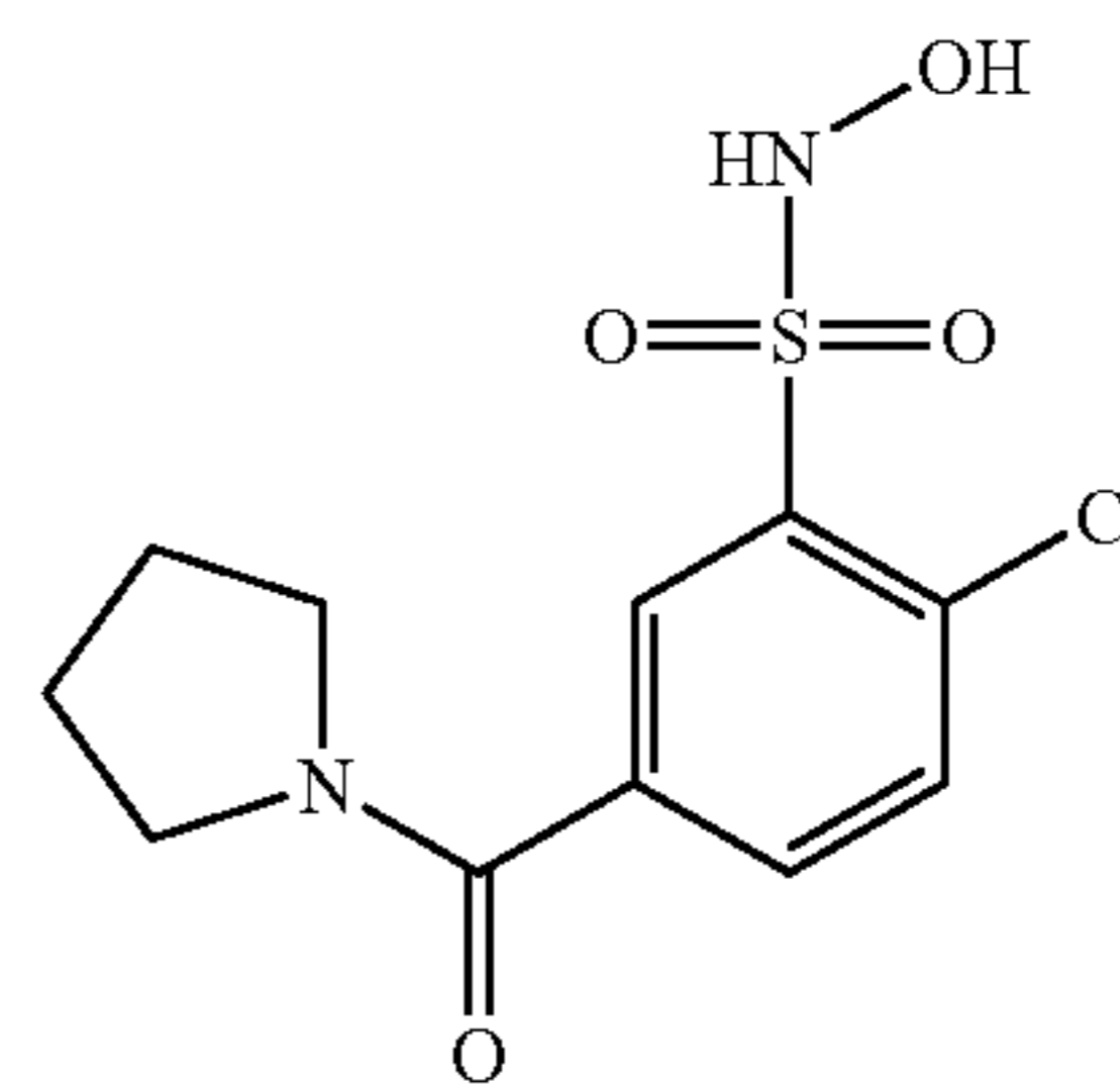
Compound 71
