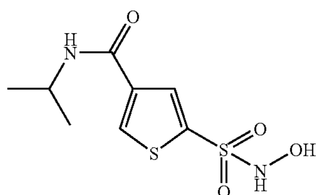
Compound 87
