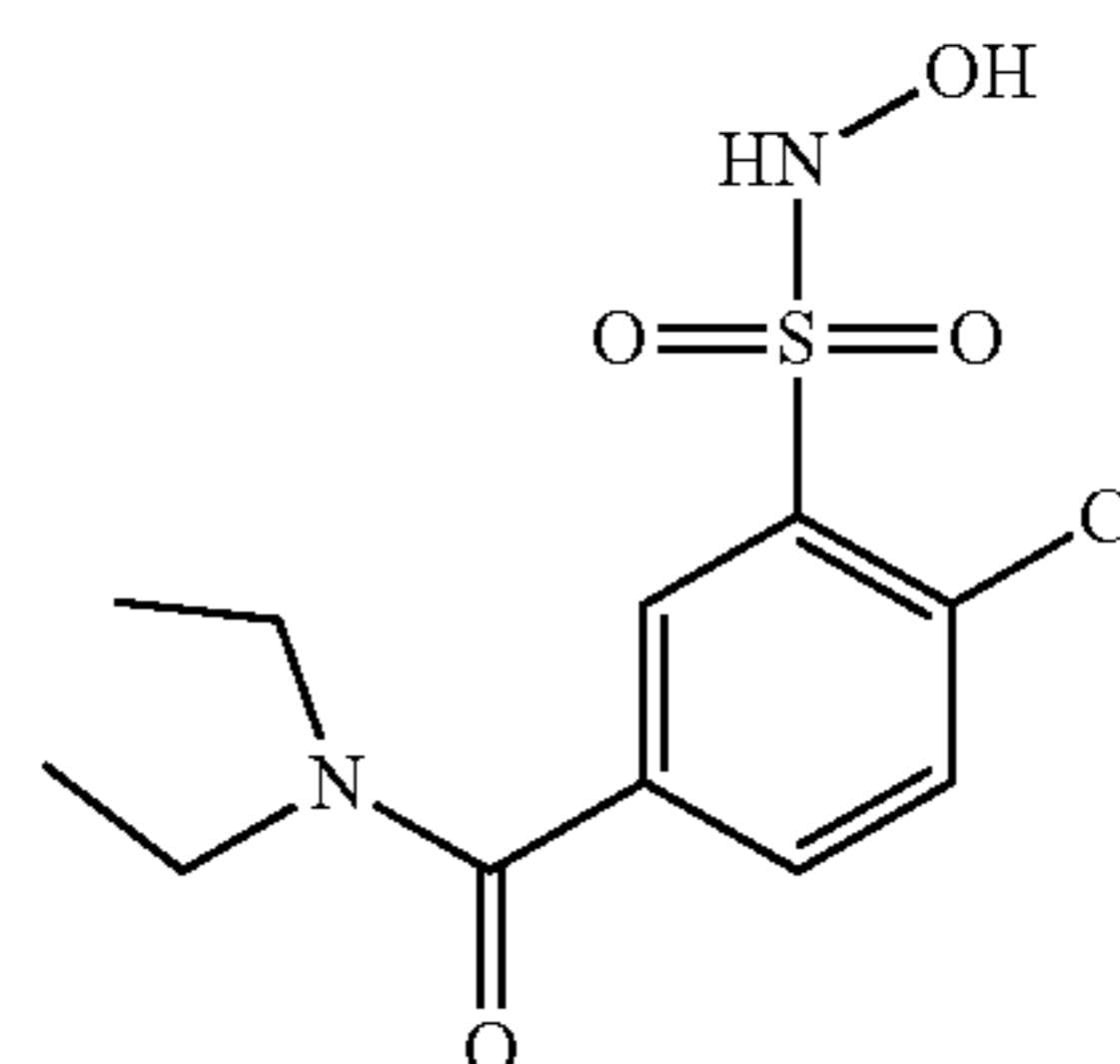
Compound 10
