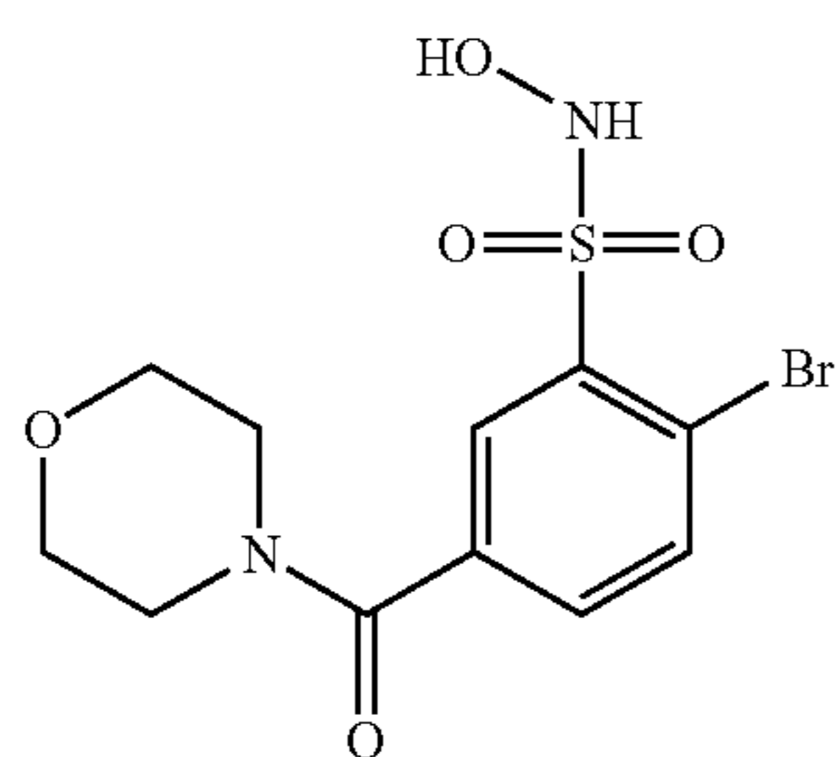
Compound 5
