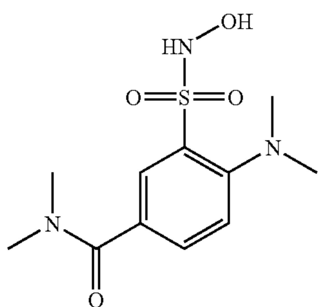
Compound 47
