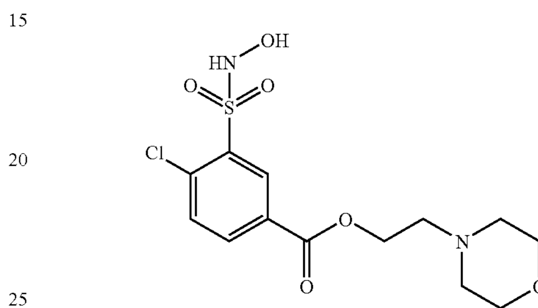
Compound 8
