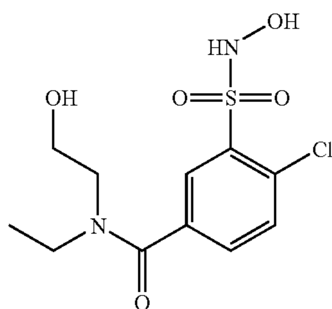
Compound 35
