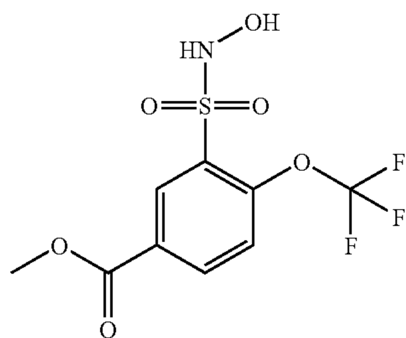
Compound 44
