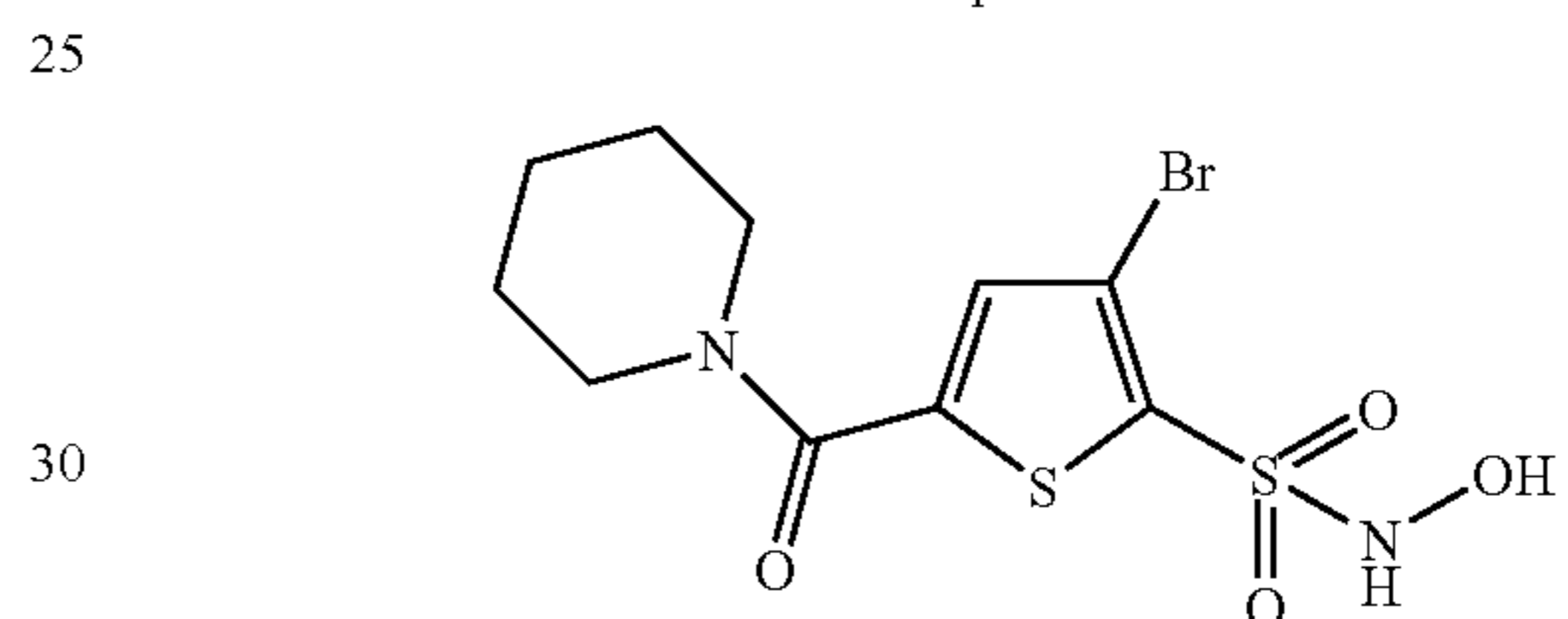
Compound 89
