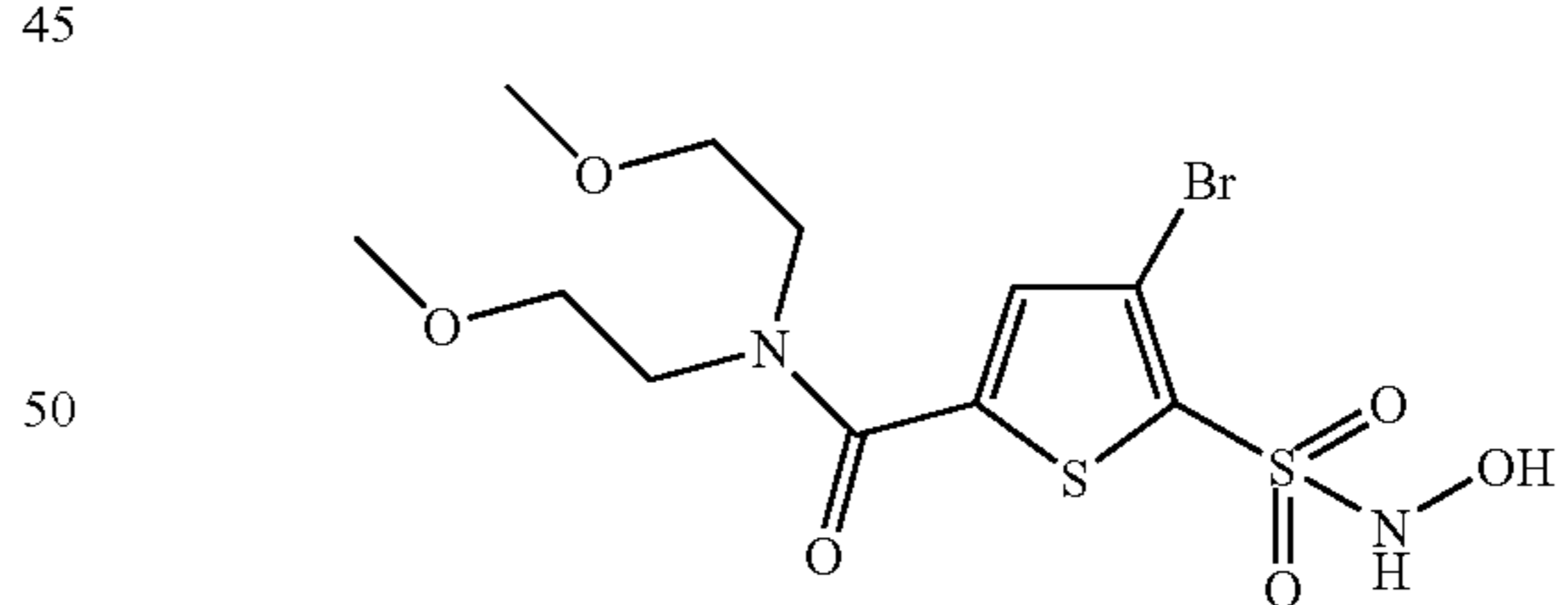
Compound 92
