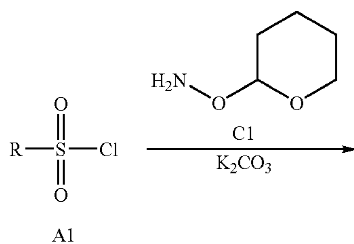
Scheme D. General Synthesis of Intermediate N-(tetrahydro-pyran-2-yloxy)sulfonamides.
