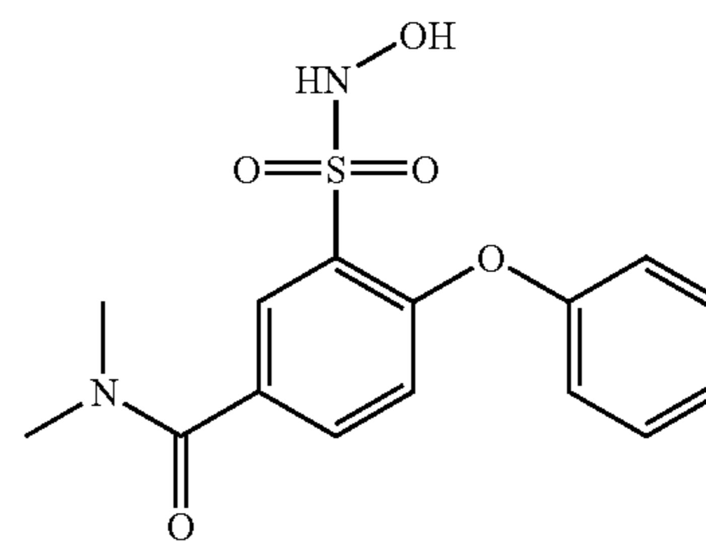
Compound 49
