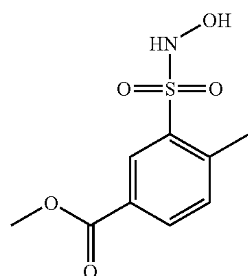
Compound 46
