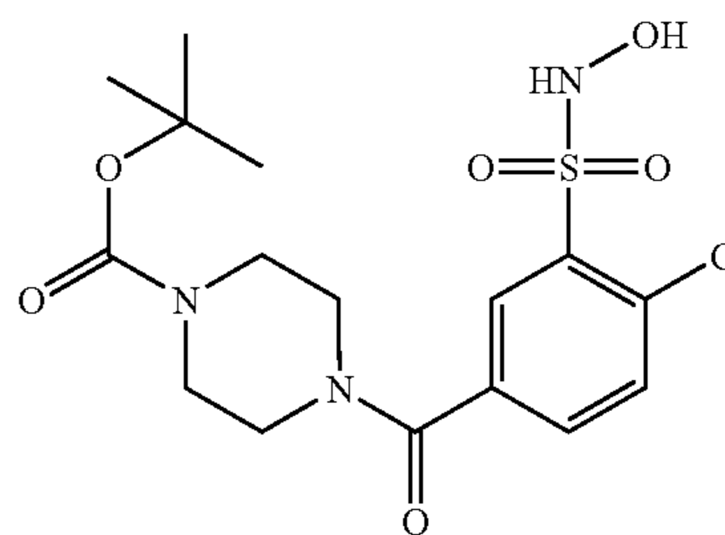
Compound 69
