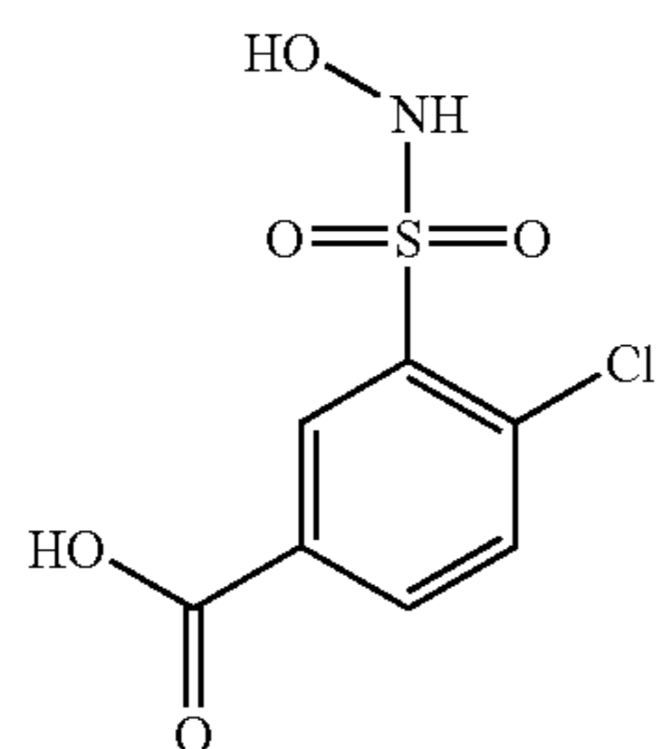
Compound 3
