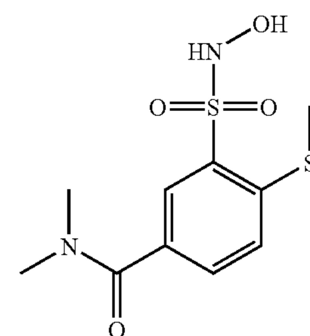
Compound 39
