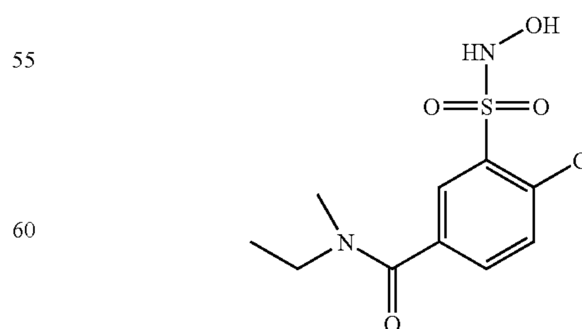
Compound 72
