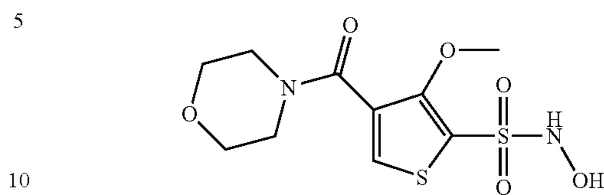
Compound 88
