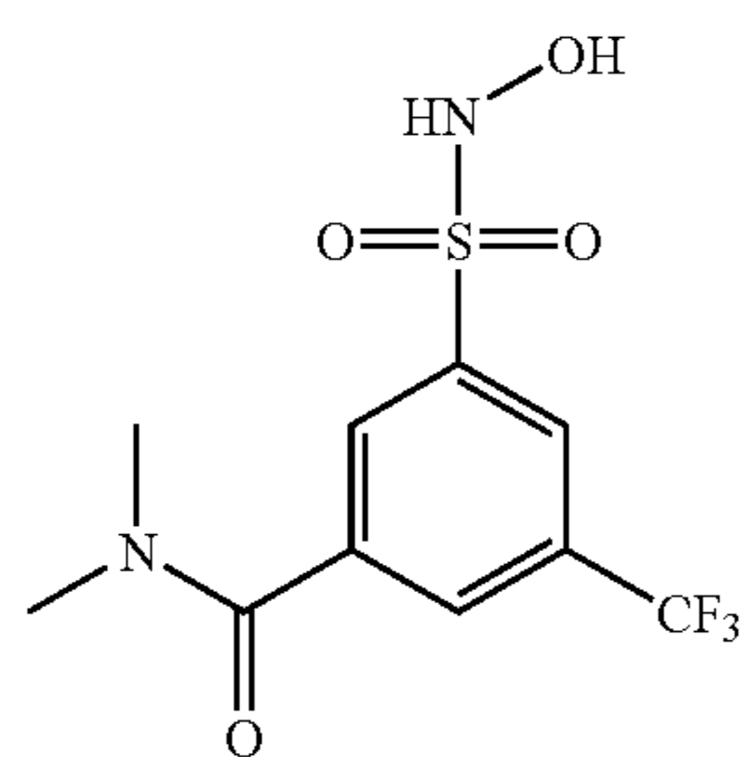
Compound 55
