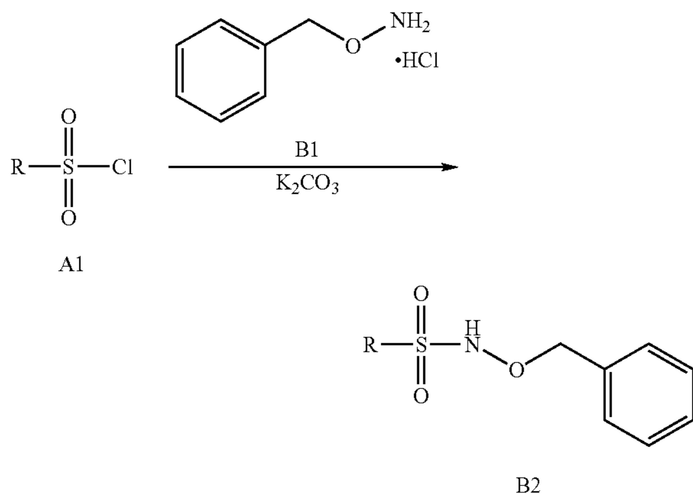
Scheme C. General Synthesis of Intermediate N-Benzyloxysulfonamides.
