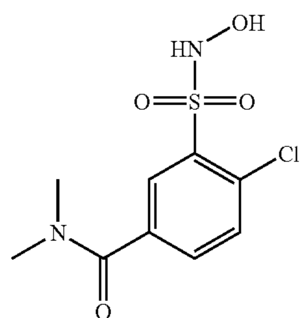
Compound 7
