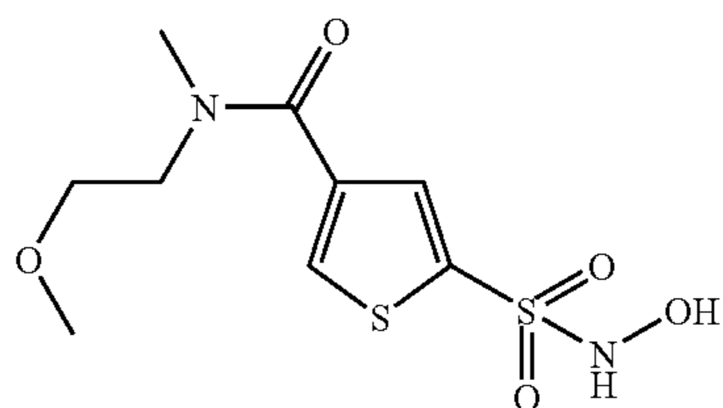
Compound 84
