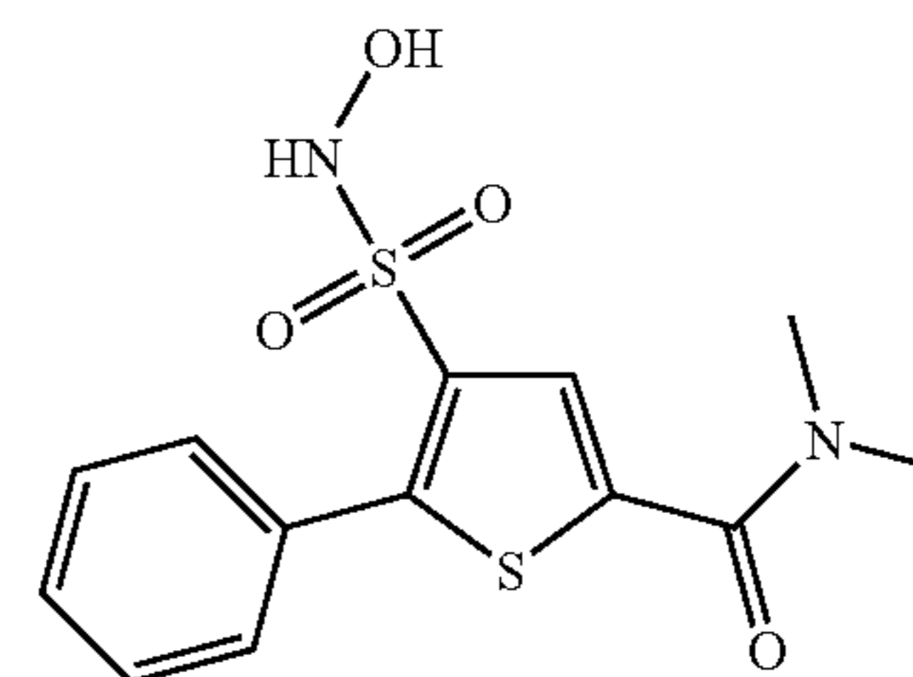
Compound 81
