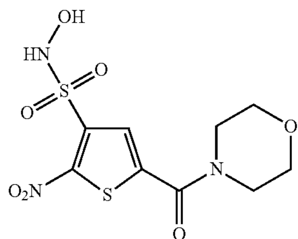
Compound 85
