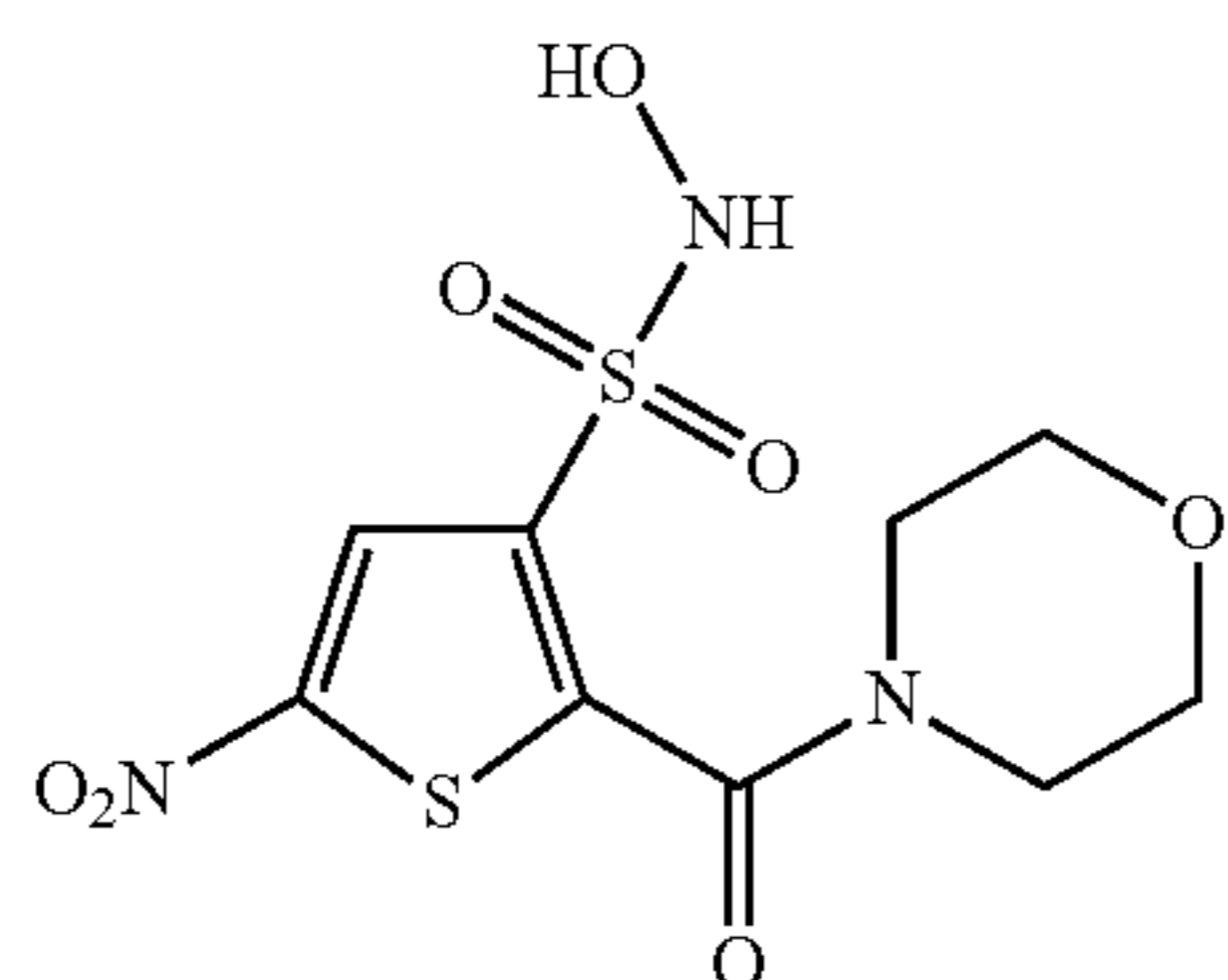
Compound 86
