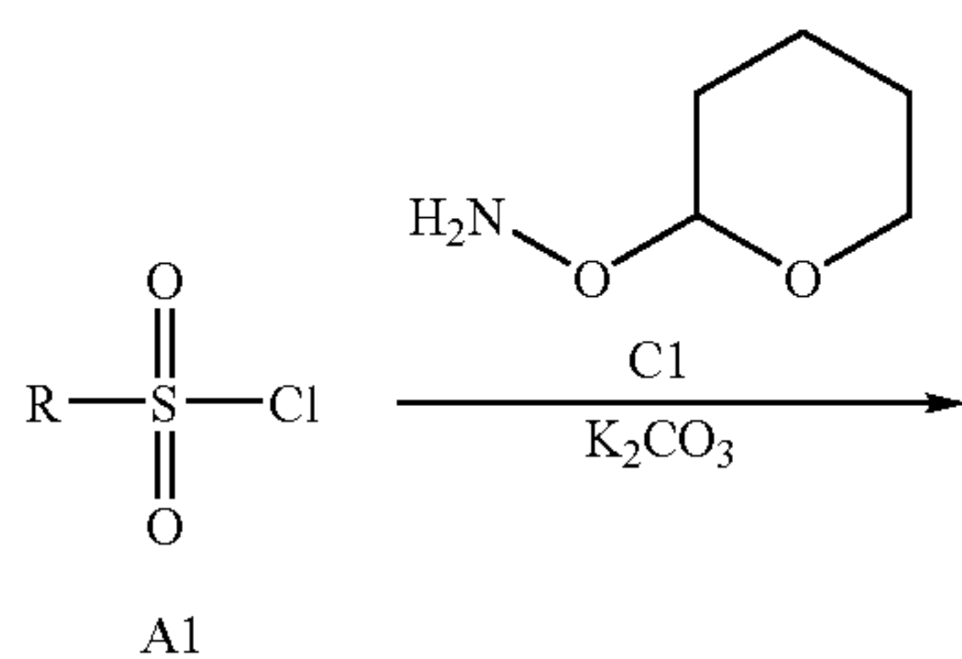
Scheme D. General Synthesis of Intermediate N-(tetrahydro-pyran-2-yloxy)sulfonamides.
