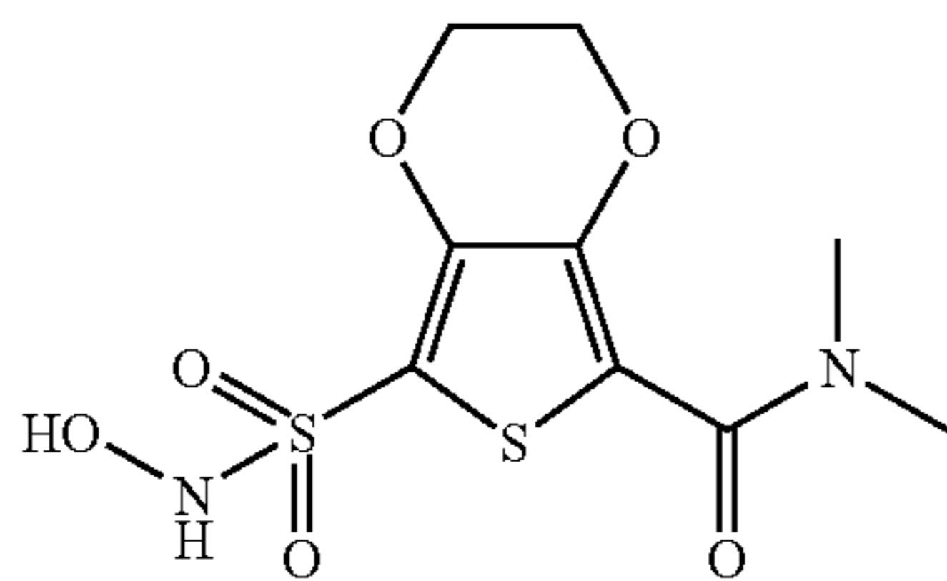
Compound 74
