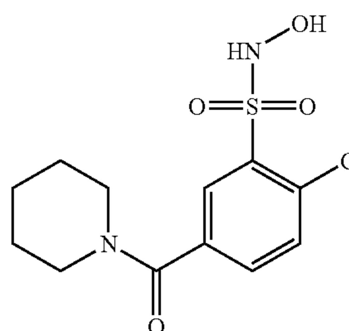
Compound 11
