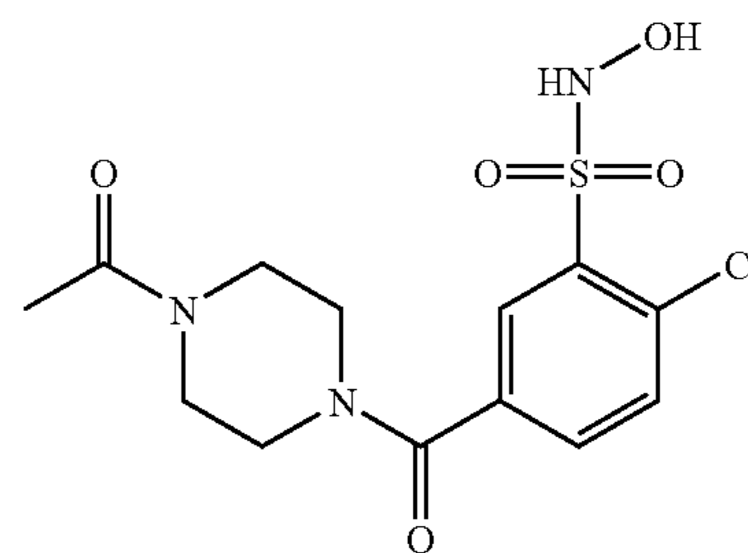
Compound 68
