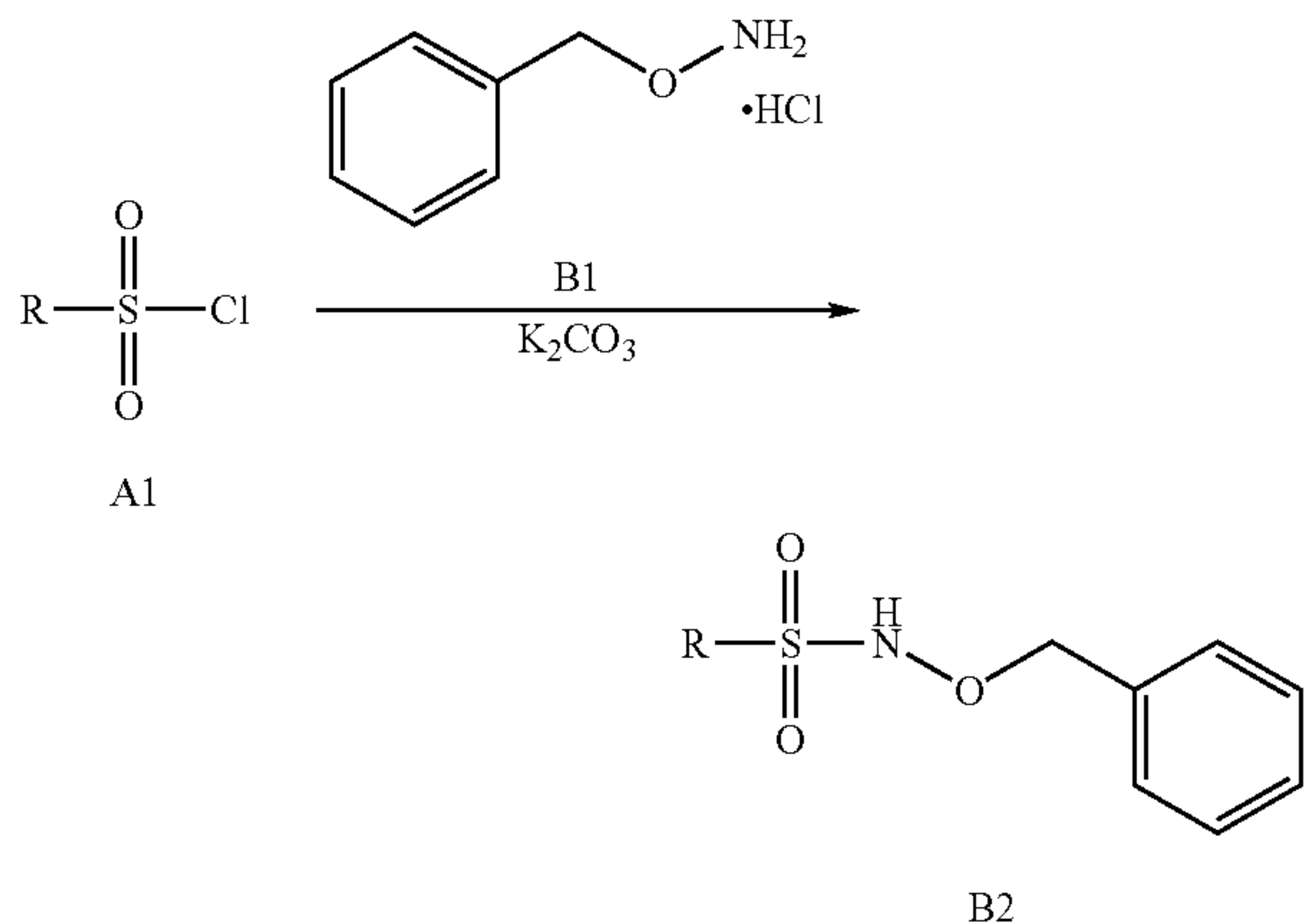
Scheme C. General Synthesis of Intermediate N-Benzyloxysulfonamides.
