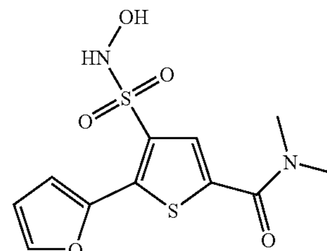
Compound 80
