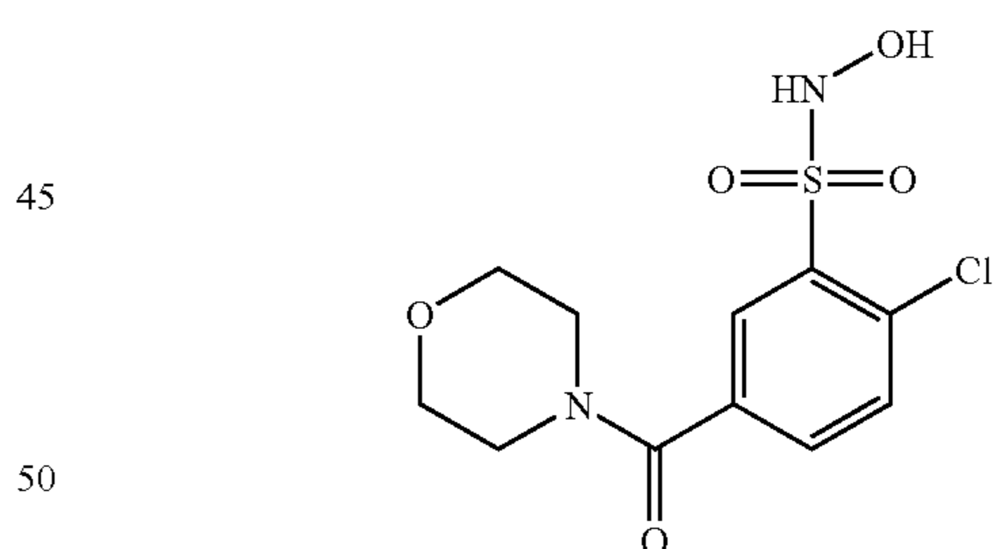
Compound 21
