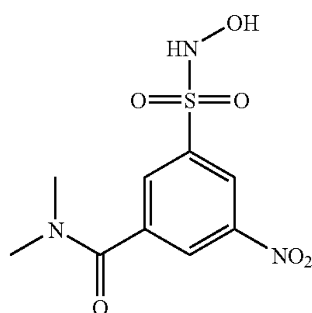
Compound 57
