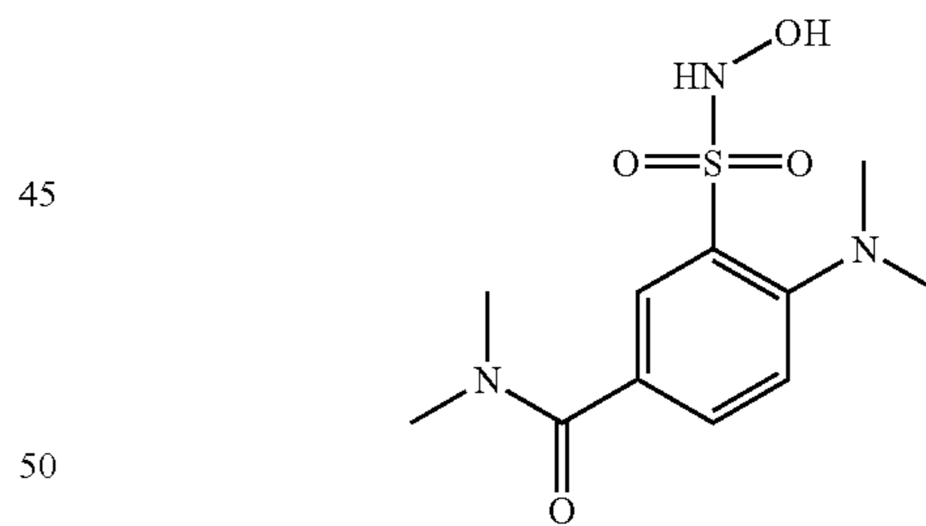
Compound 51
