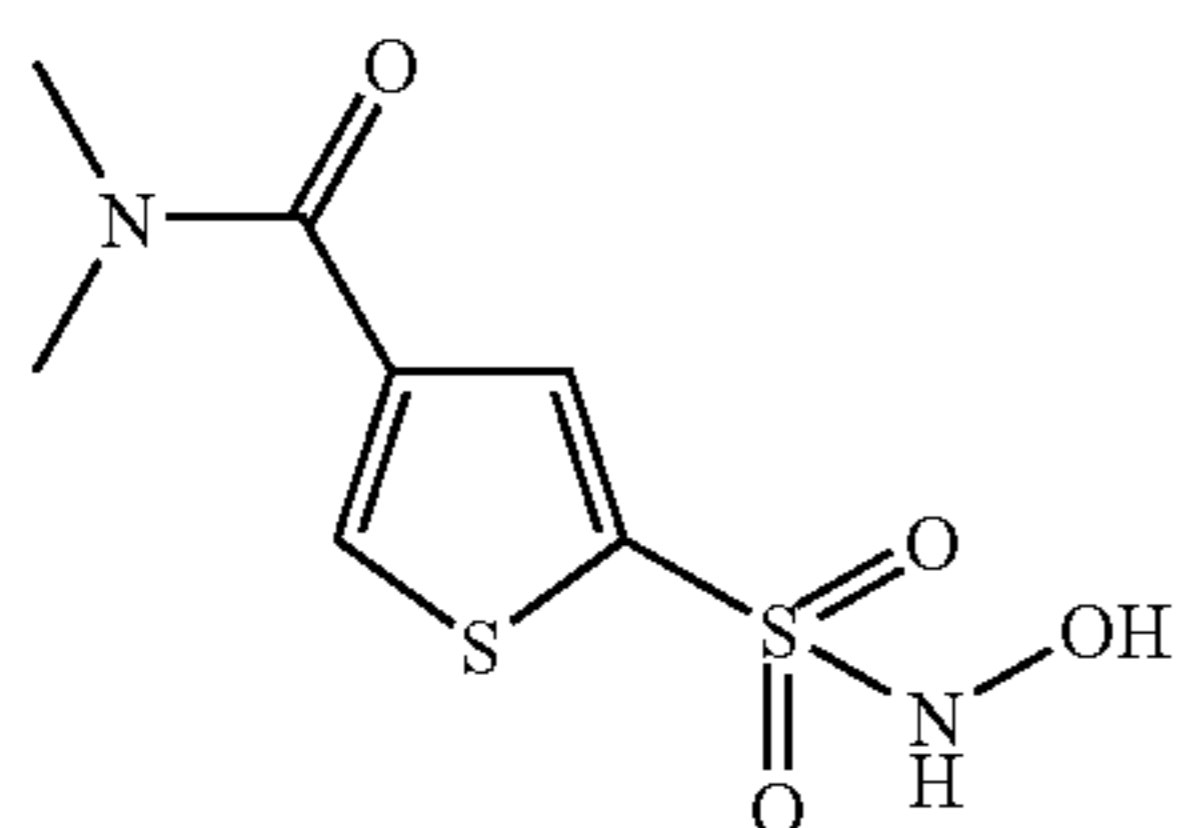
Compound 83
