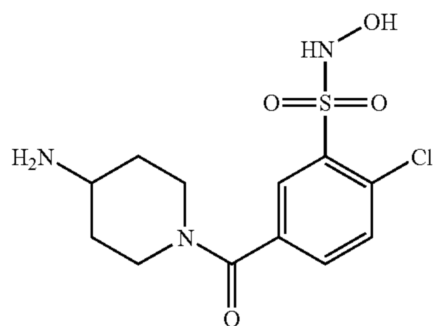
Compound 14
