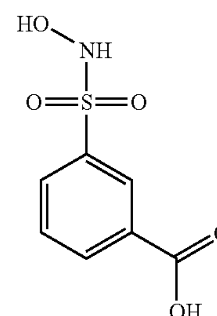
Compound 2
