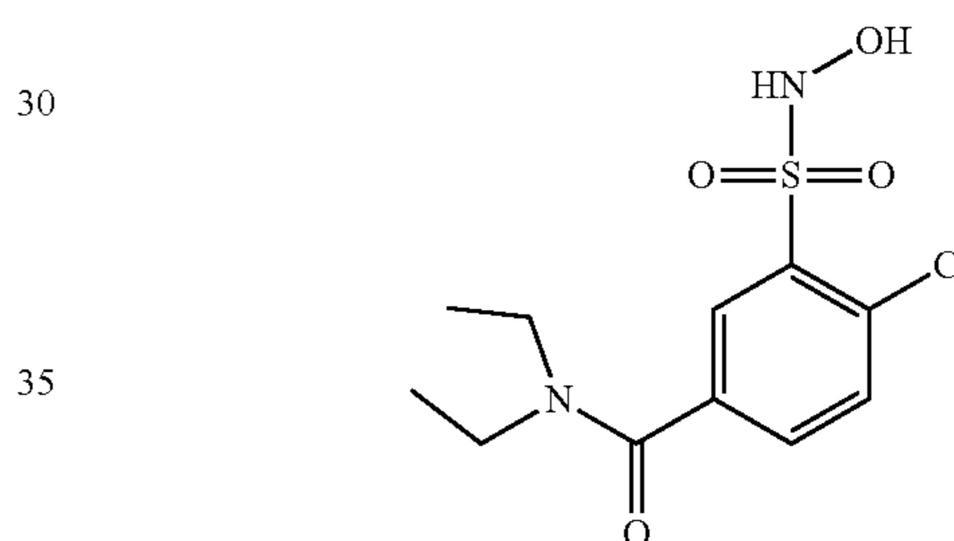
Compound 10
