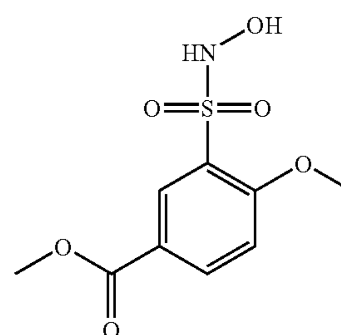
Compound 42
