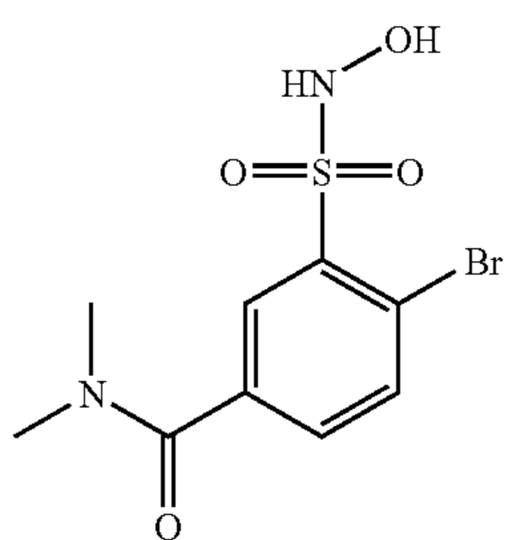
Compound 6
