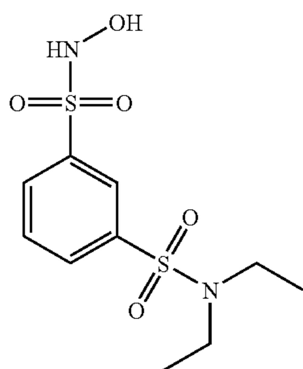
Compound 63
