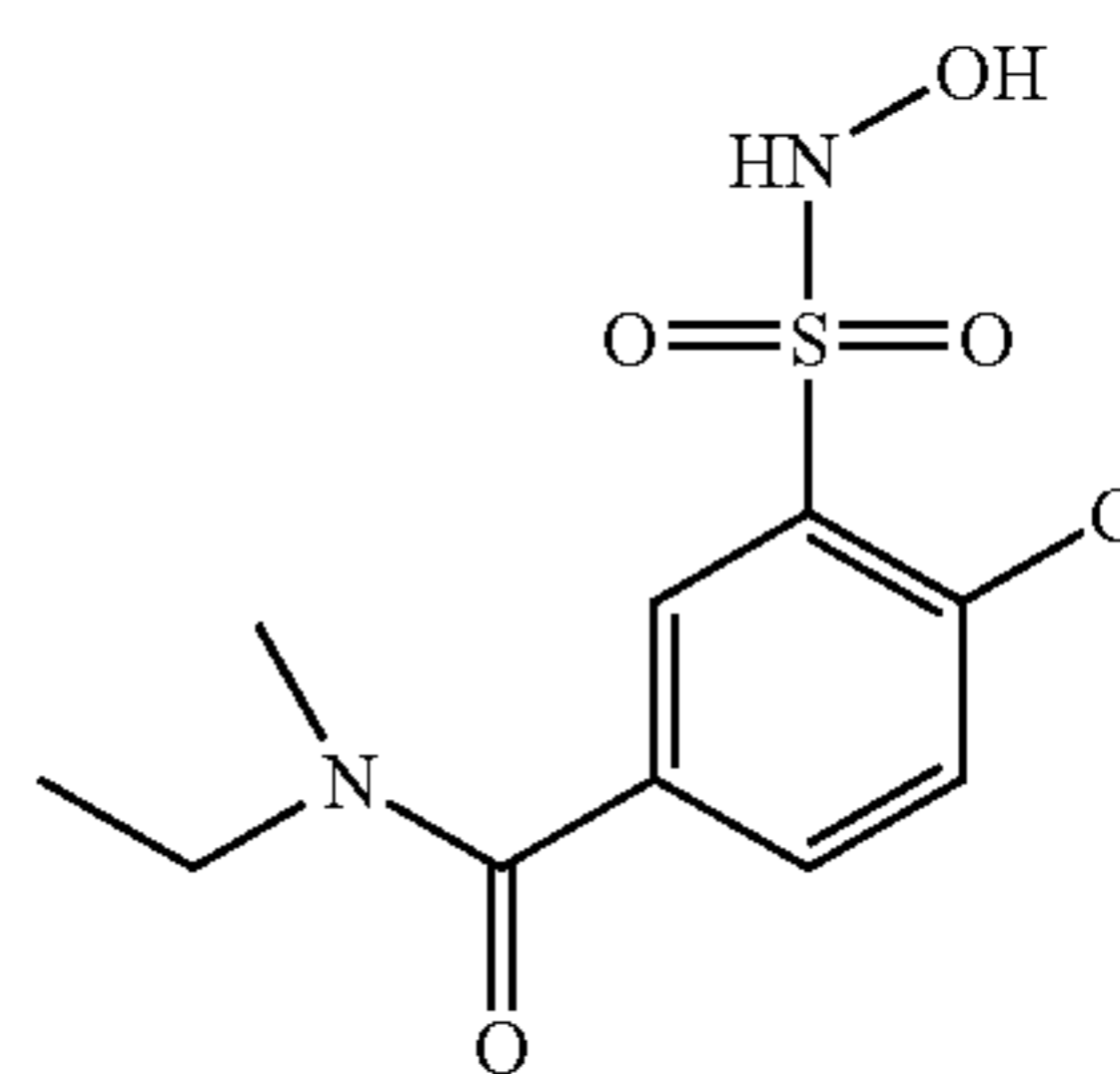
Compound 72
