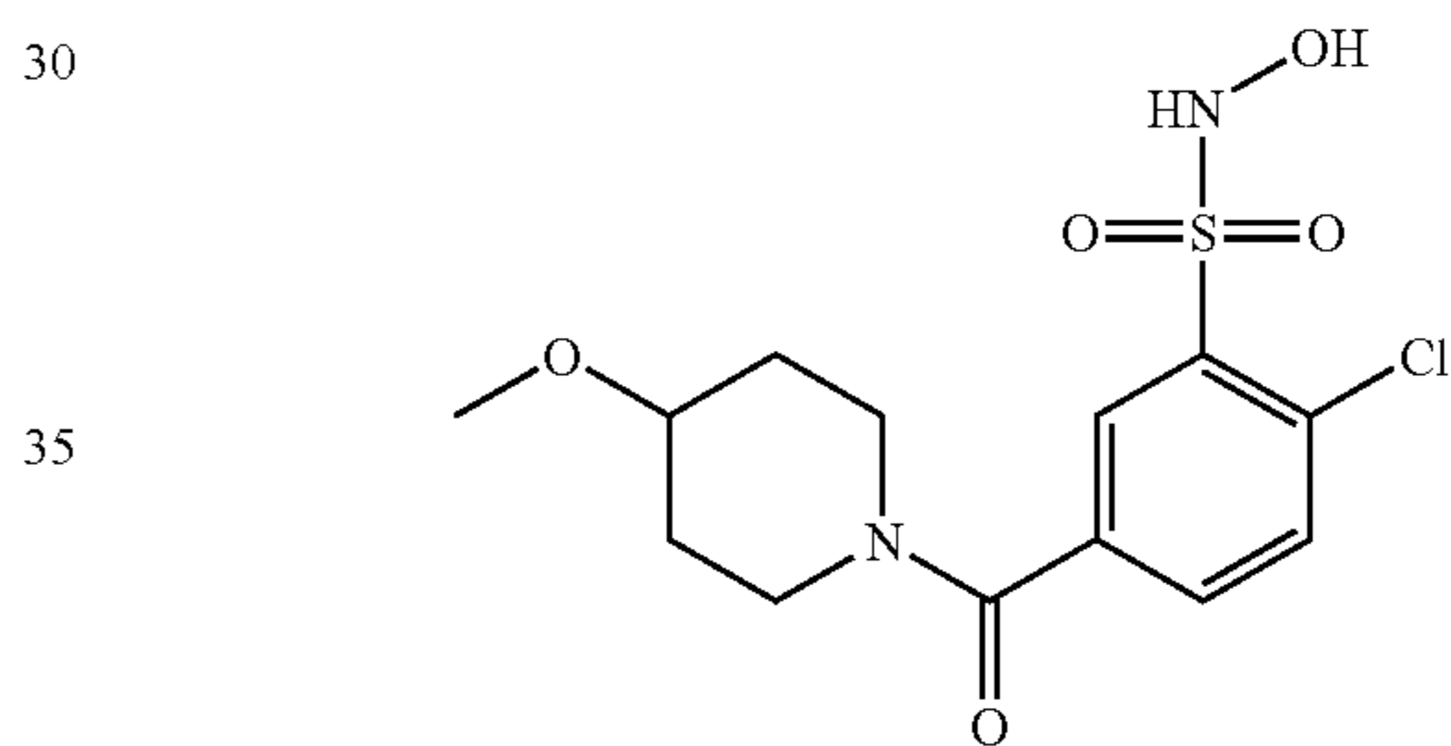
Compound 20
