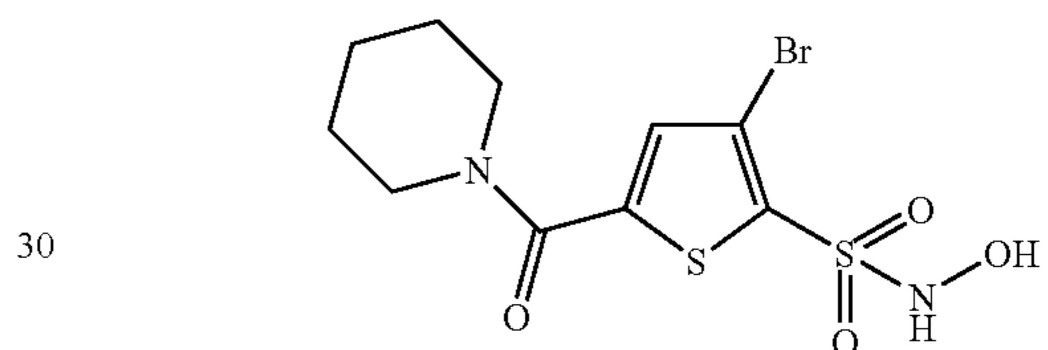
Compound 90
