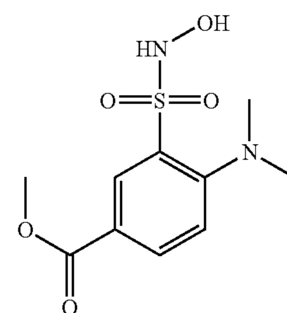
Compound 50
