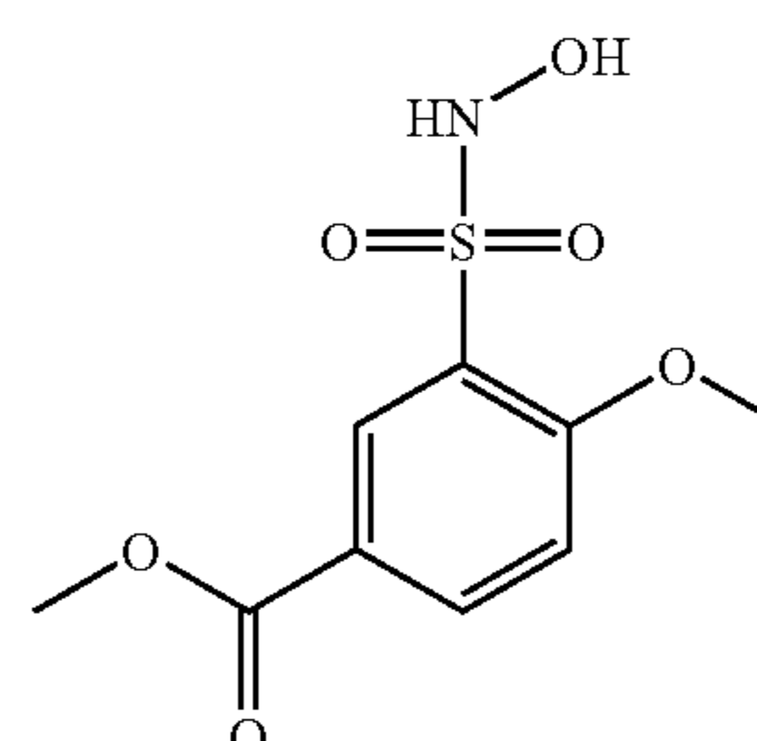
Compound 42
