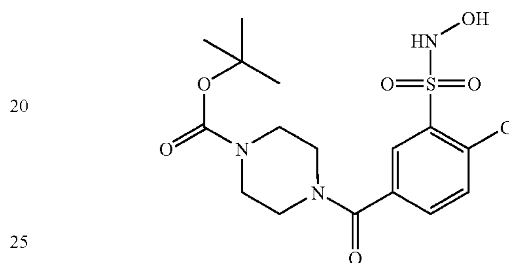
Compound 69
