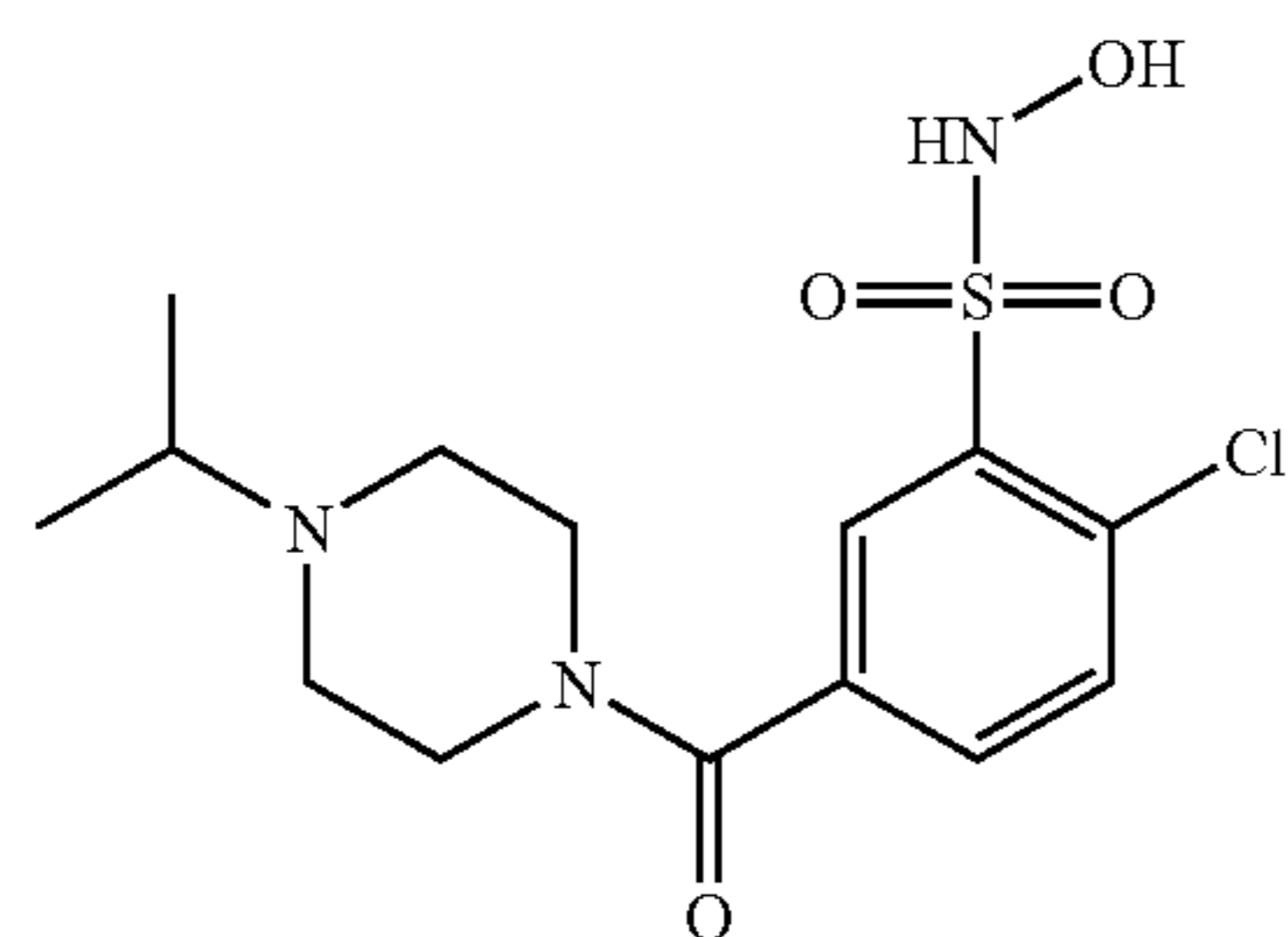
Compound 67
