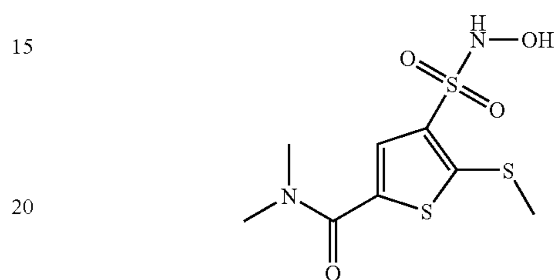
Compound 89
