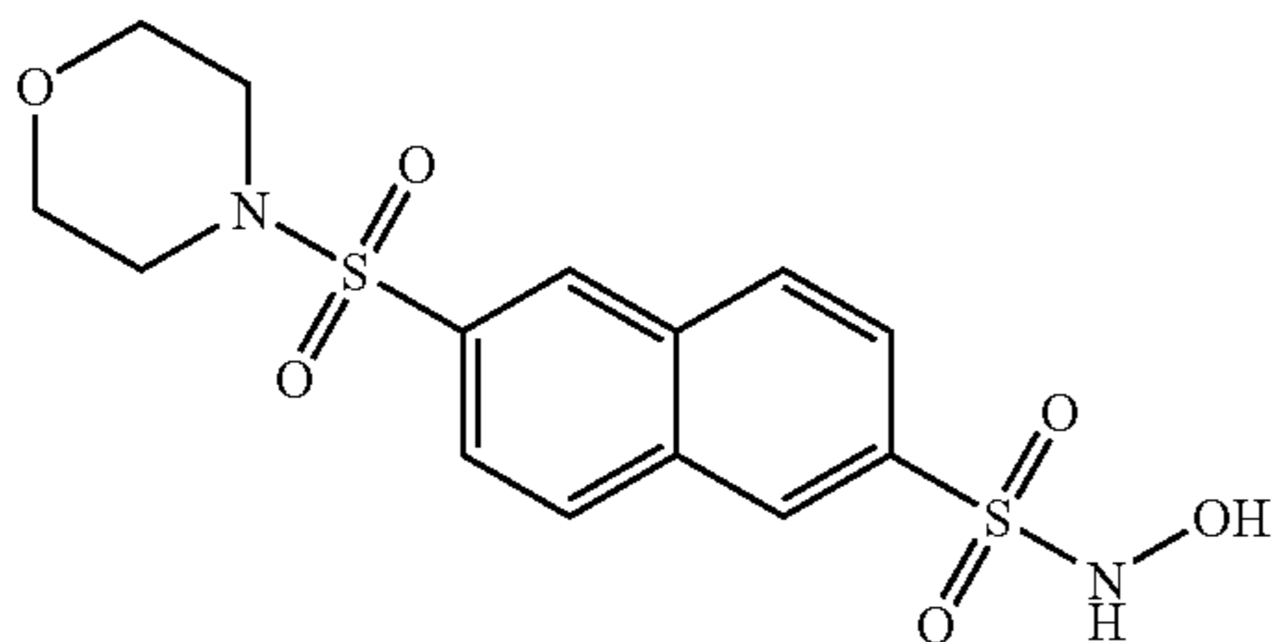
Compound 75
