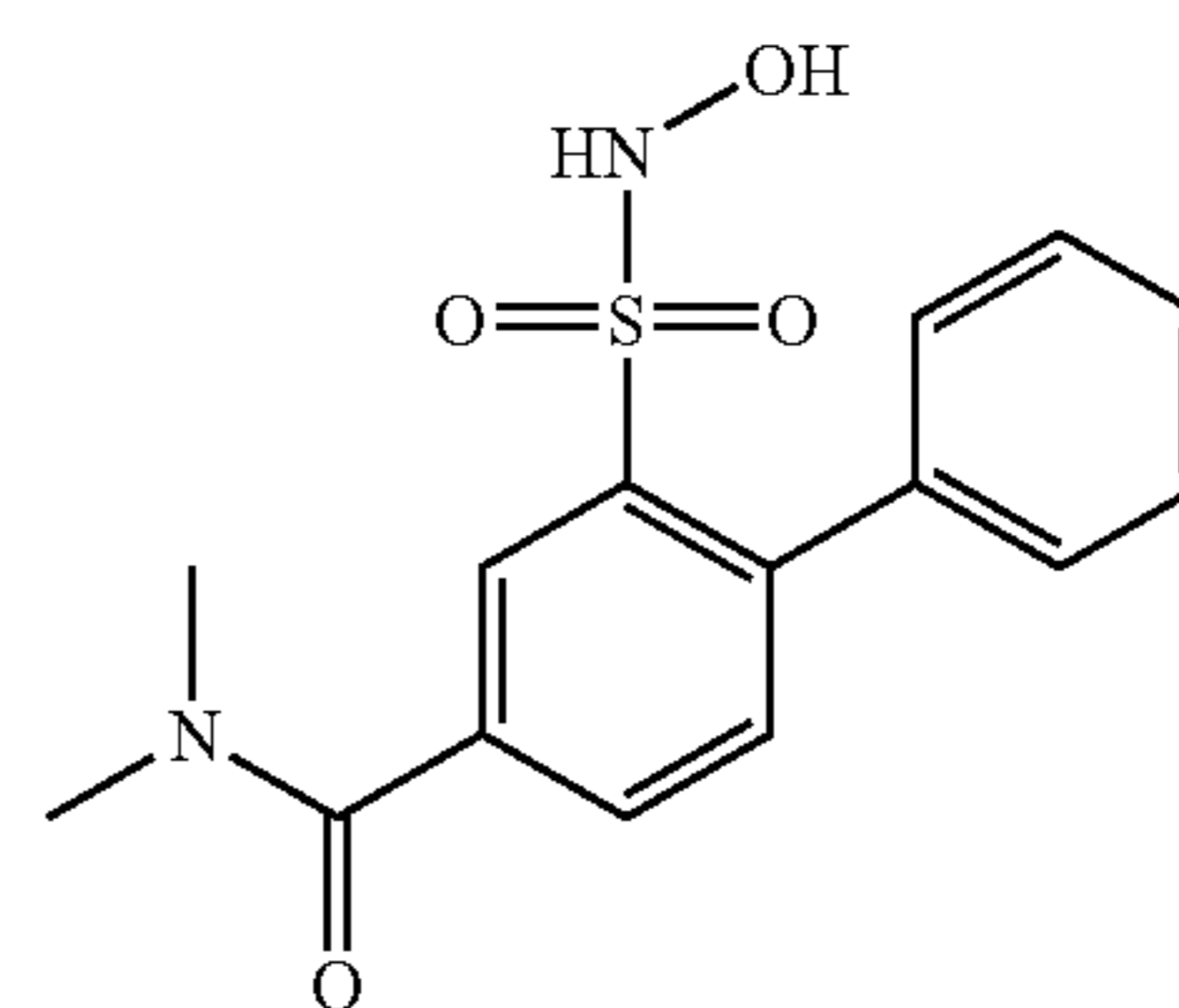
Compound 41
