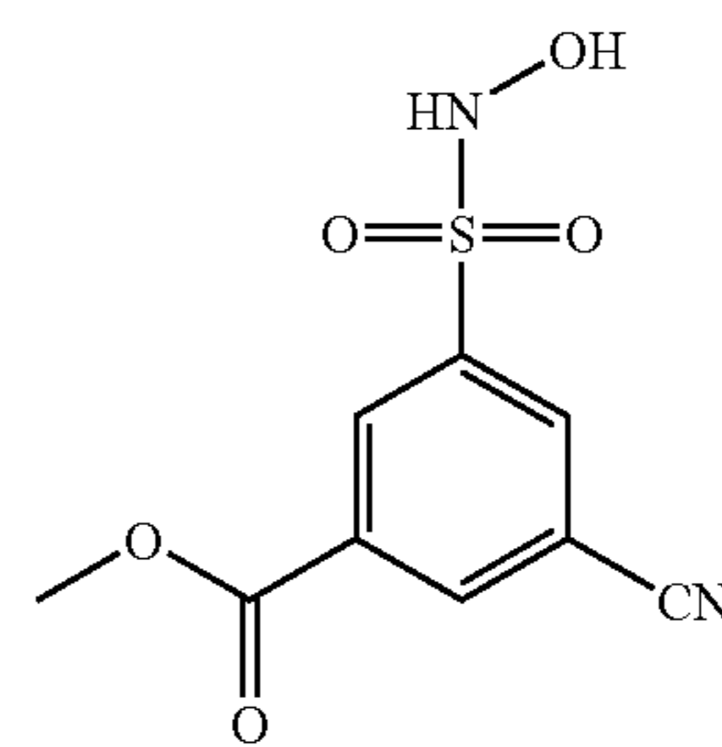
Compound 58
