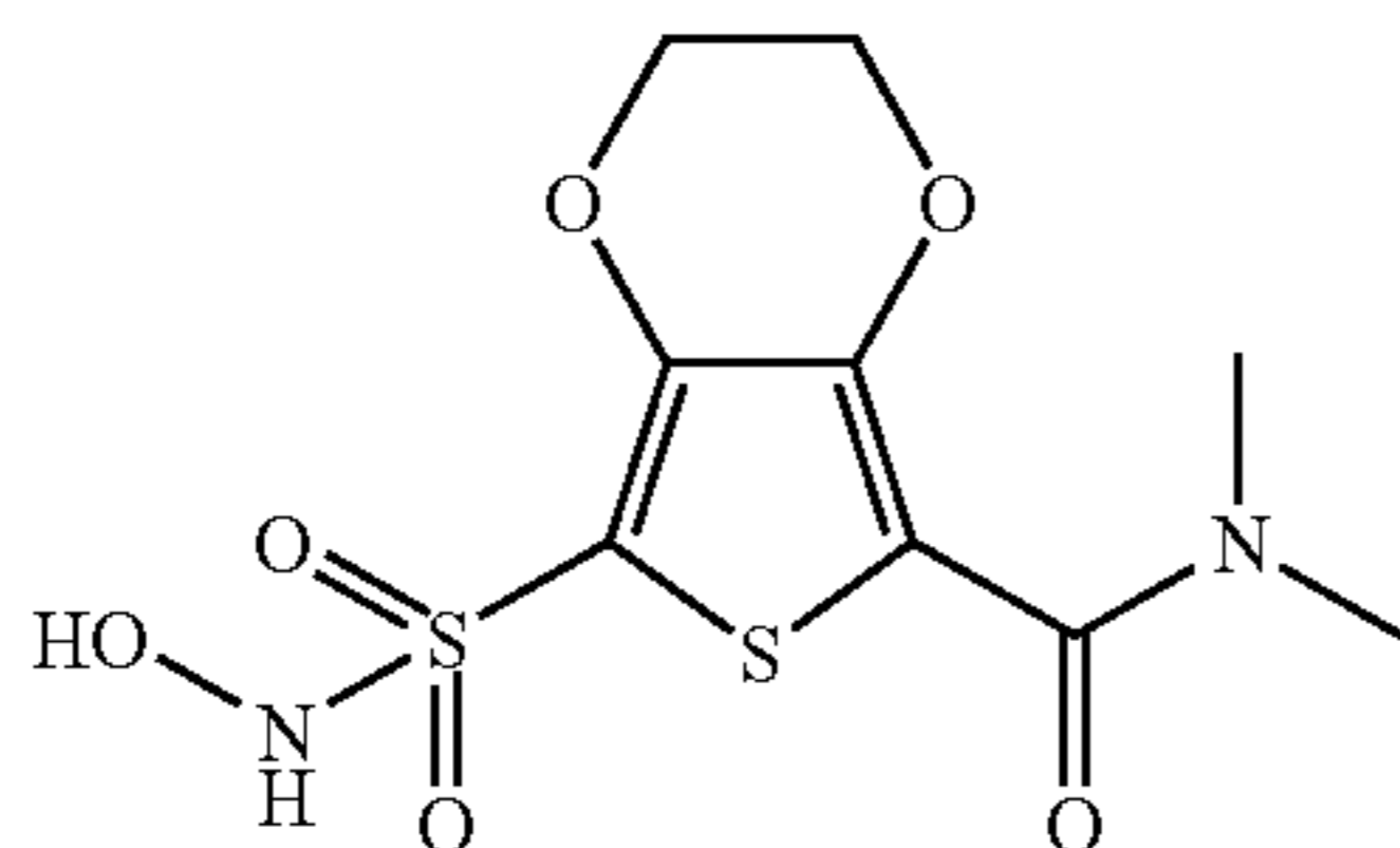
Compound 74
