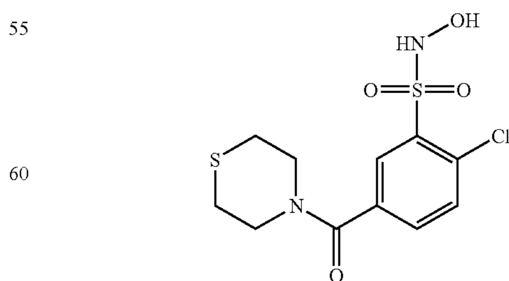
Compound 22
