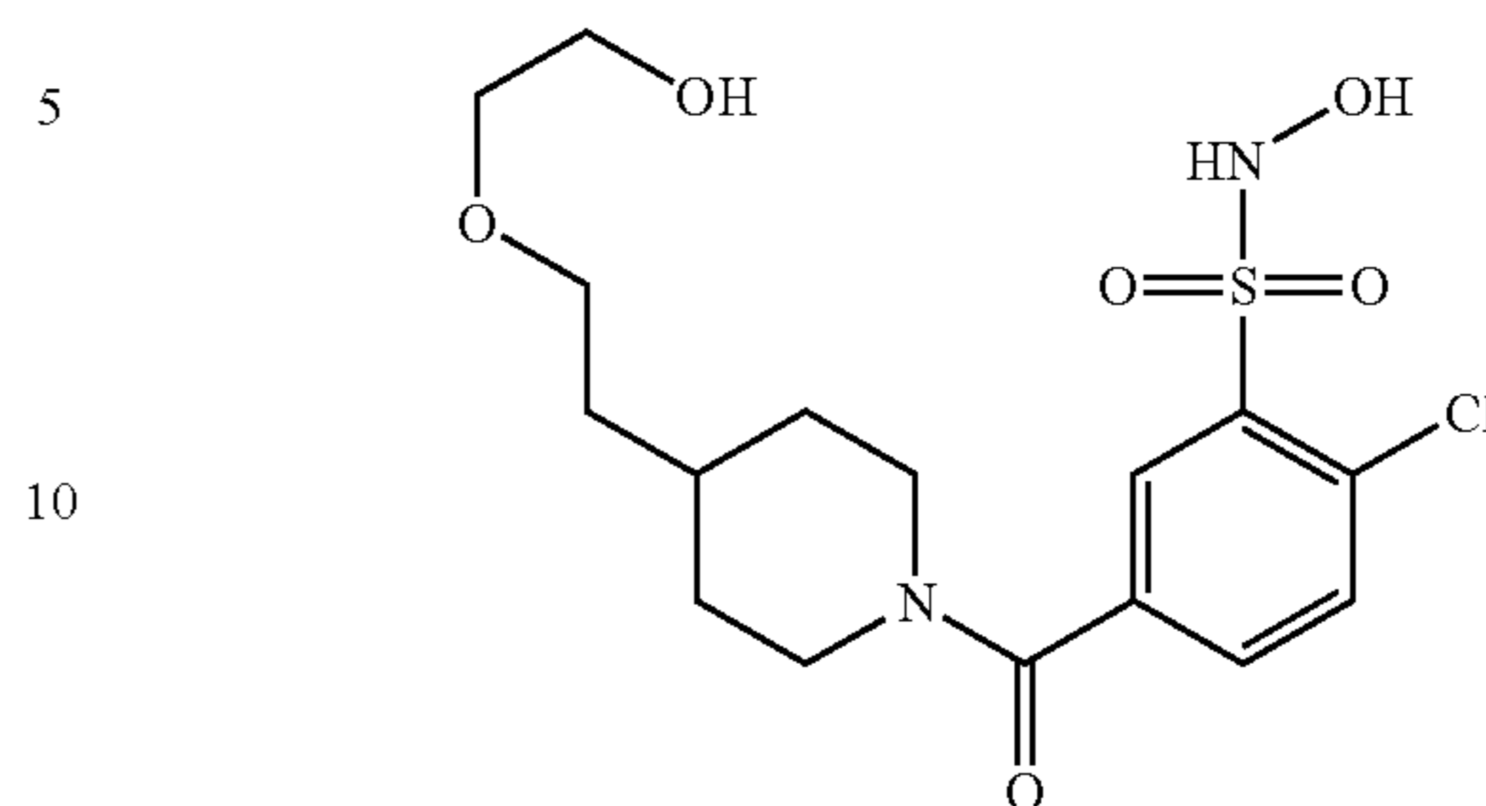
Compound 18
