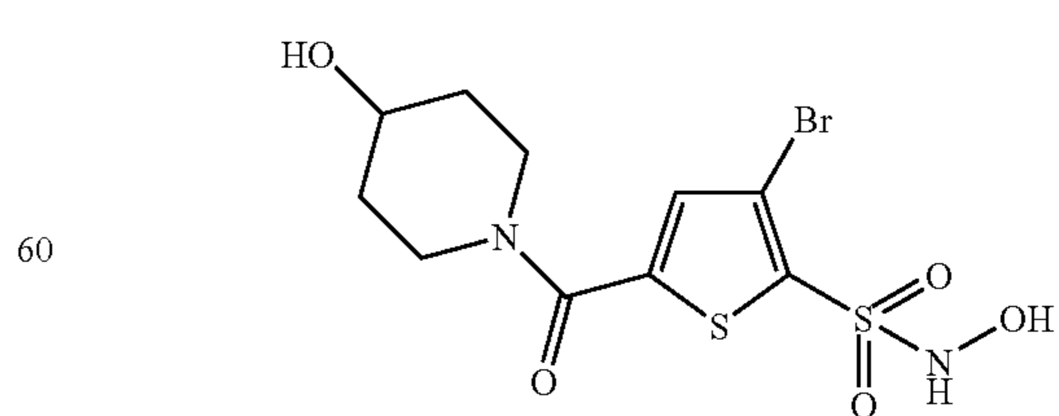
Compound 93
