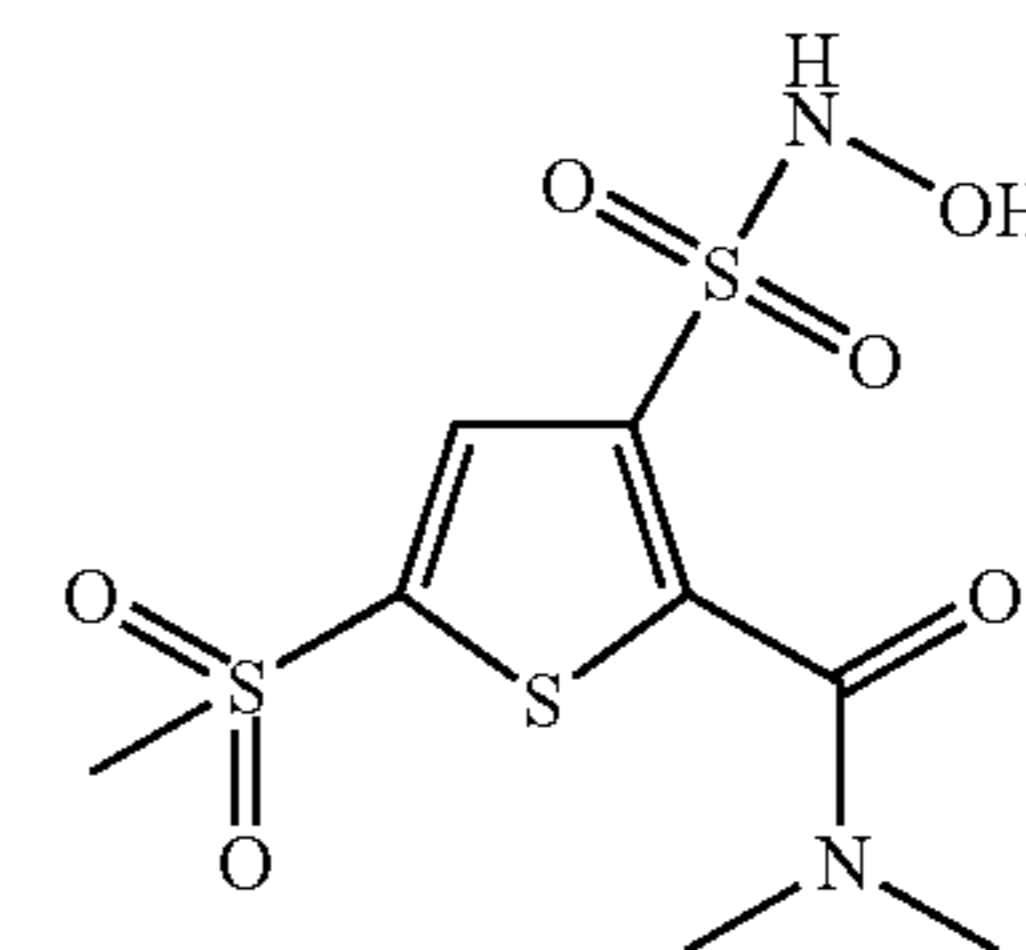
Compound 77
