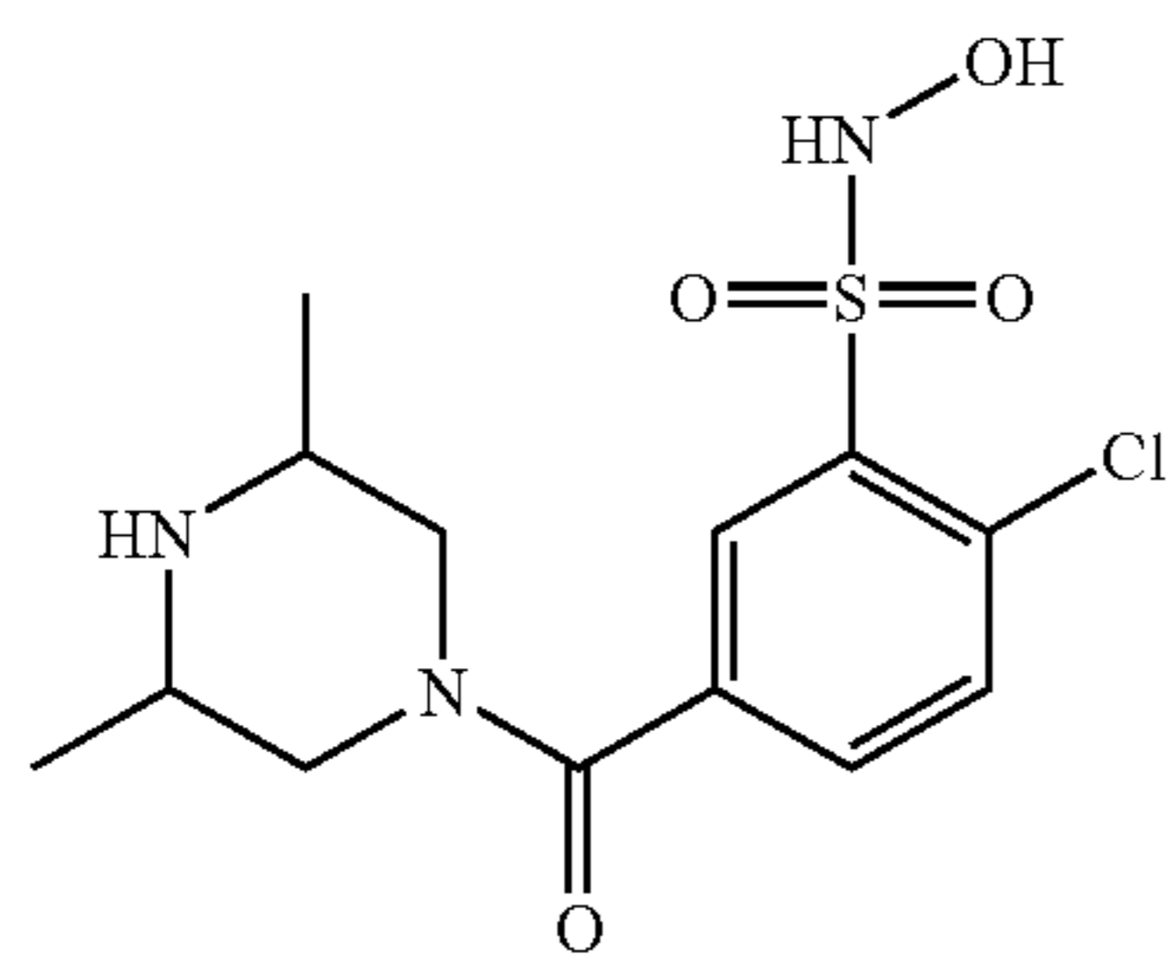
Compound 65
