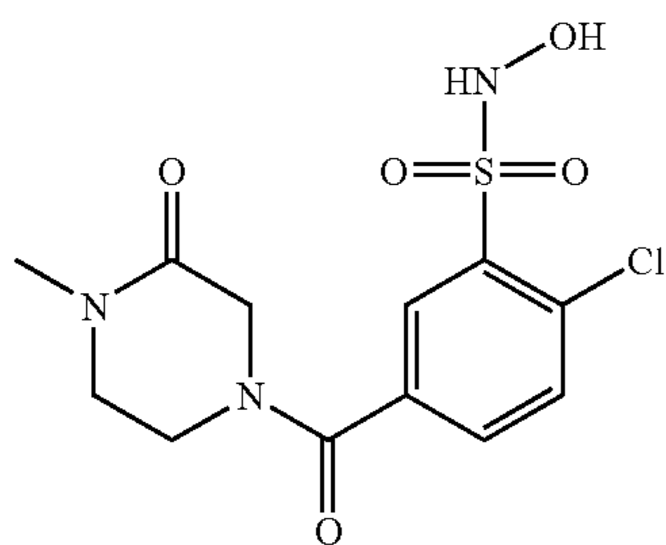
Compound 24
