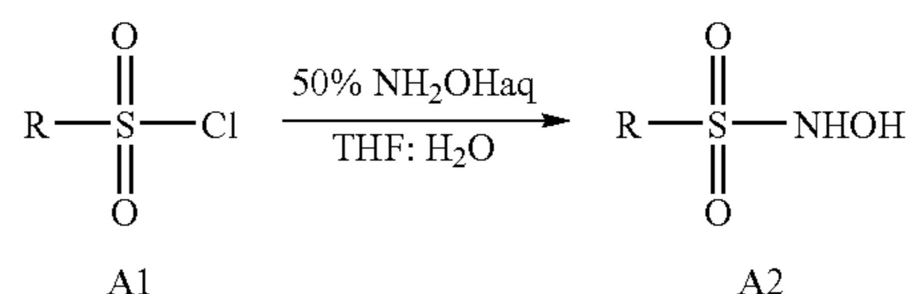
Scheme B. General Synthesis of N-Hydroxysulfonamides (Method 2).
