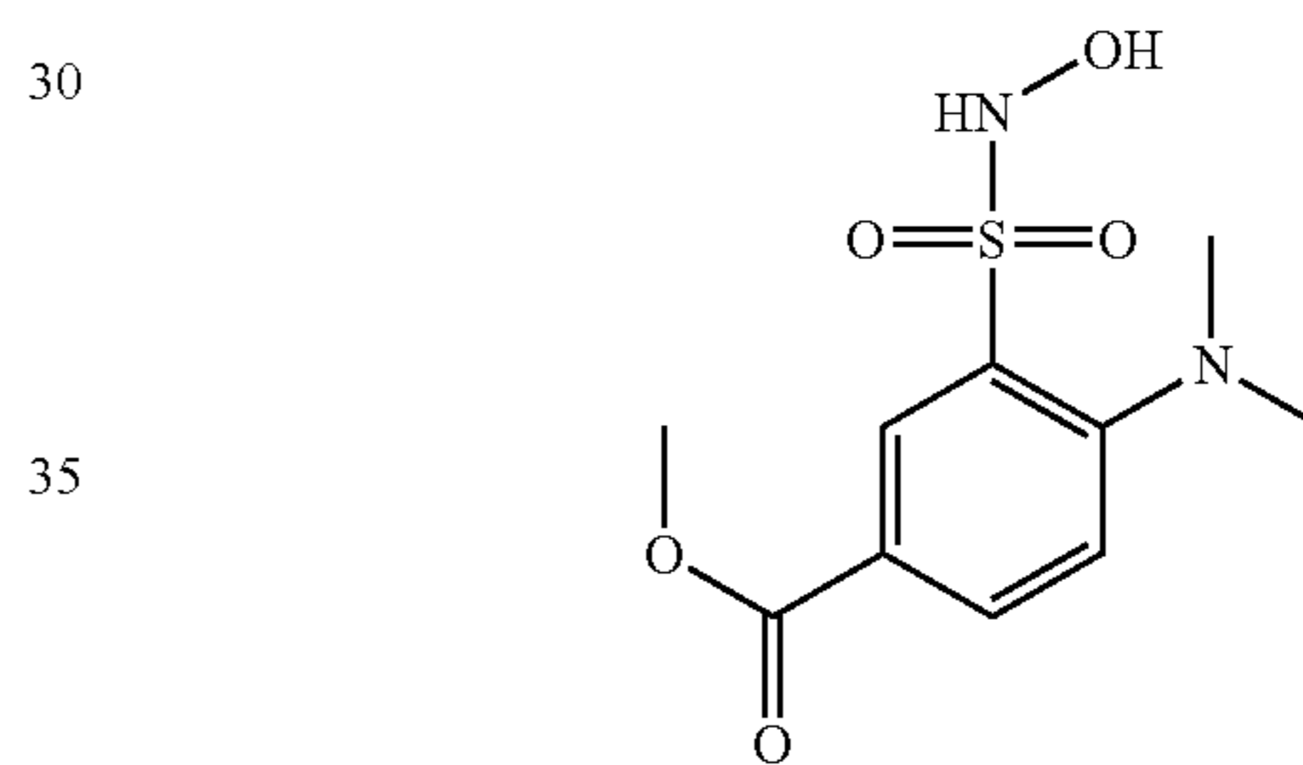
Compound 50
