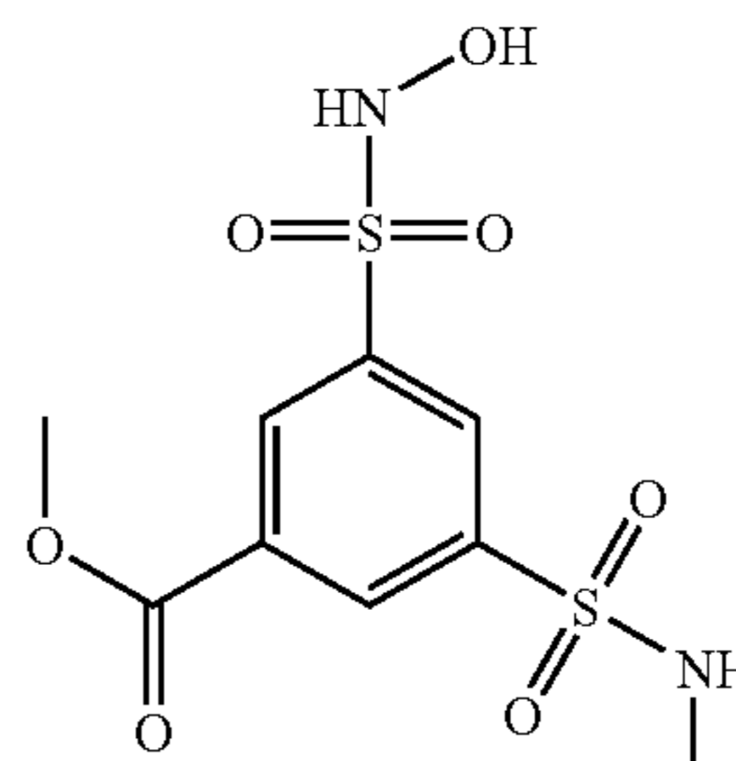
Compound 62
