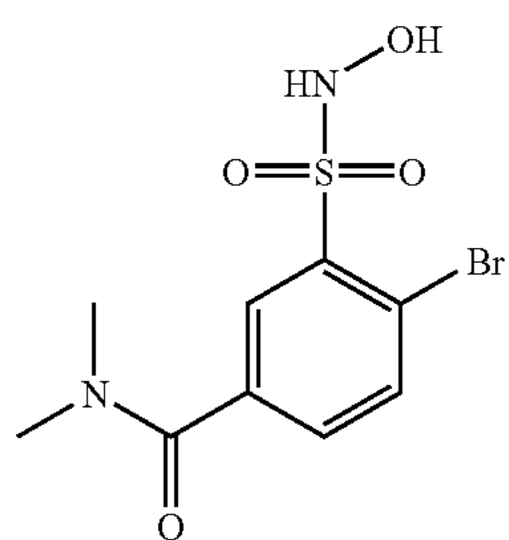
Compound 6
