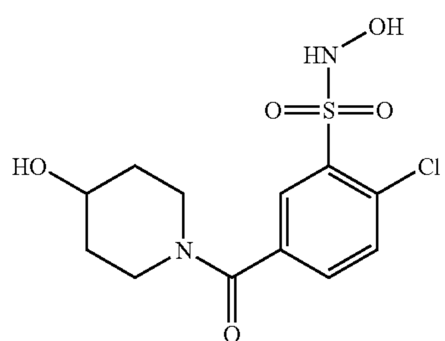
Compound 16
