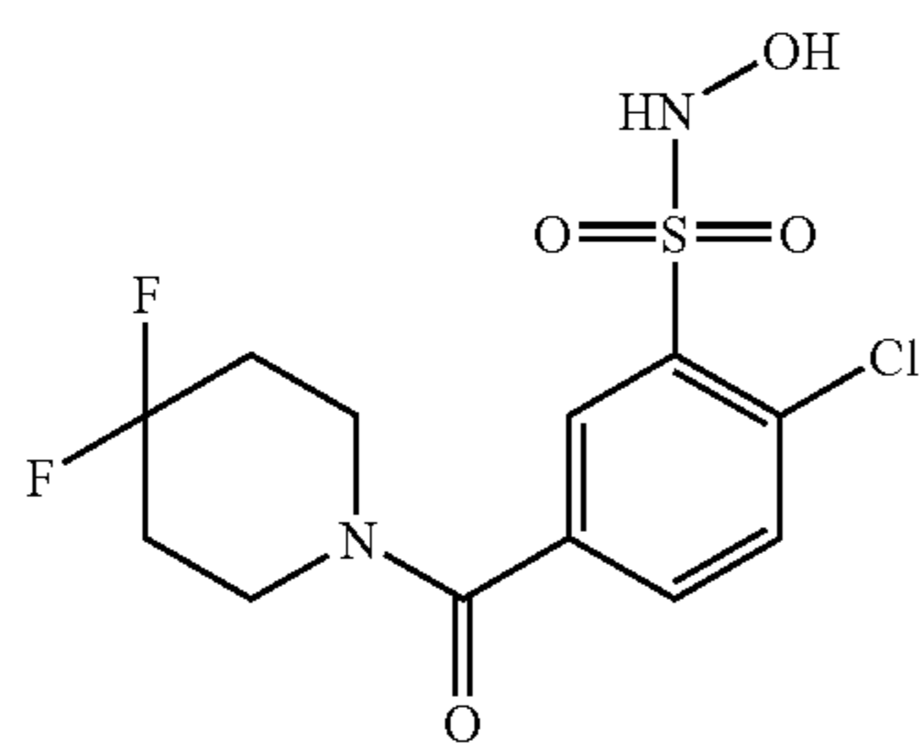
Compound 13
