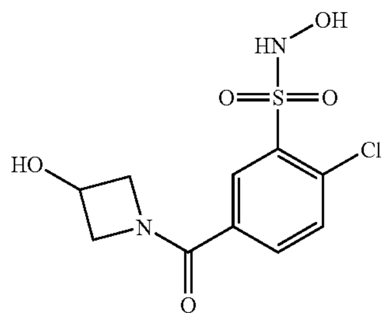
Compound 15
