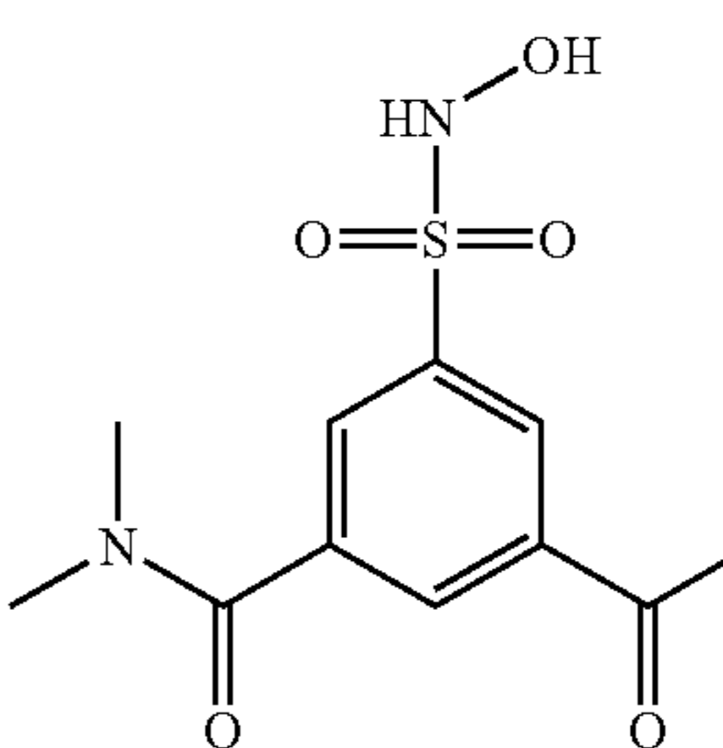
Compound 61
