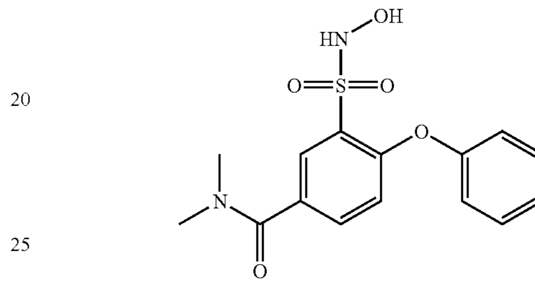
Compound 49
