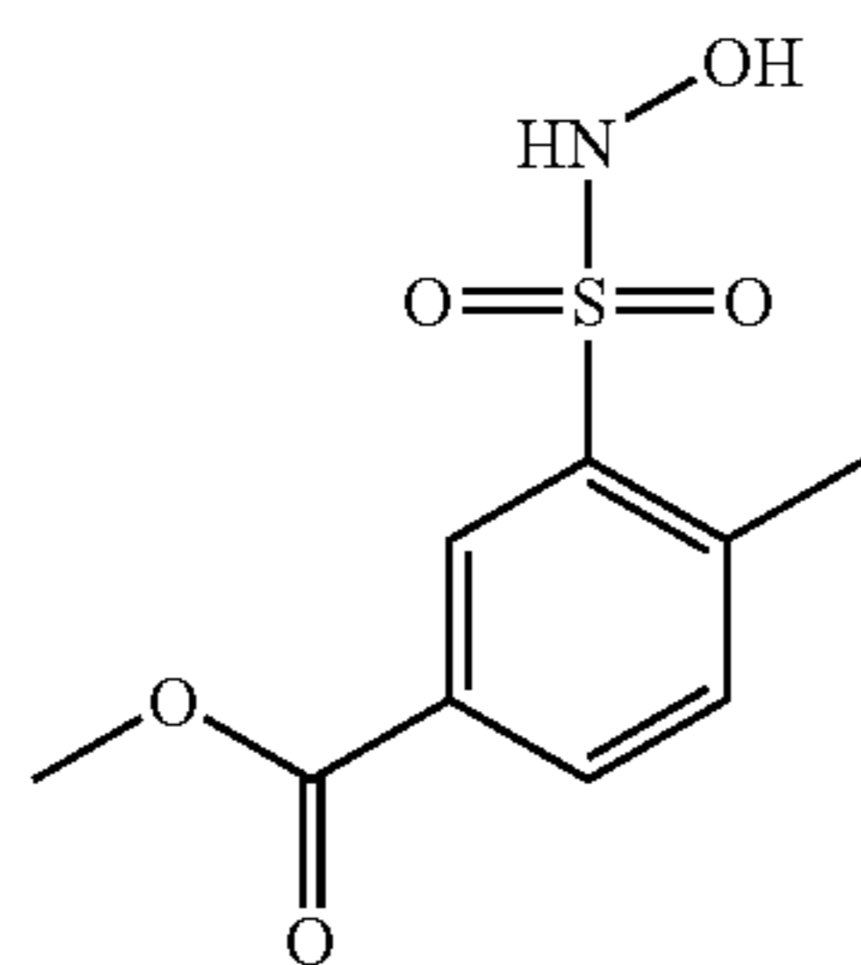
Compound 46
