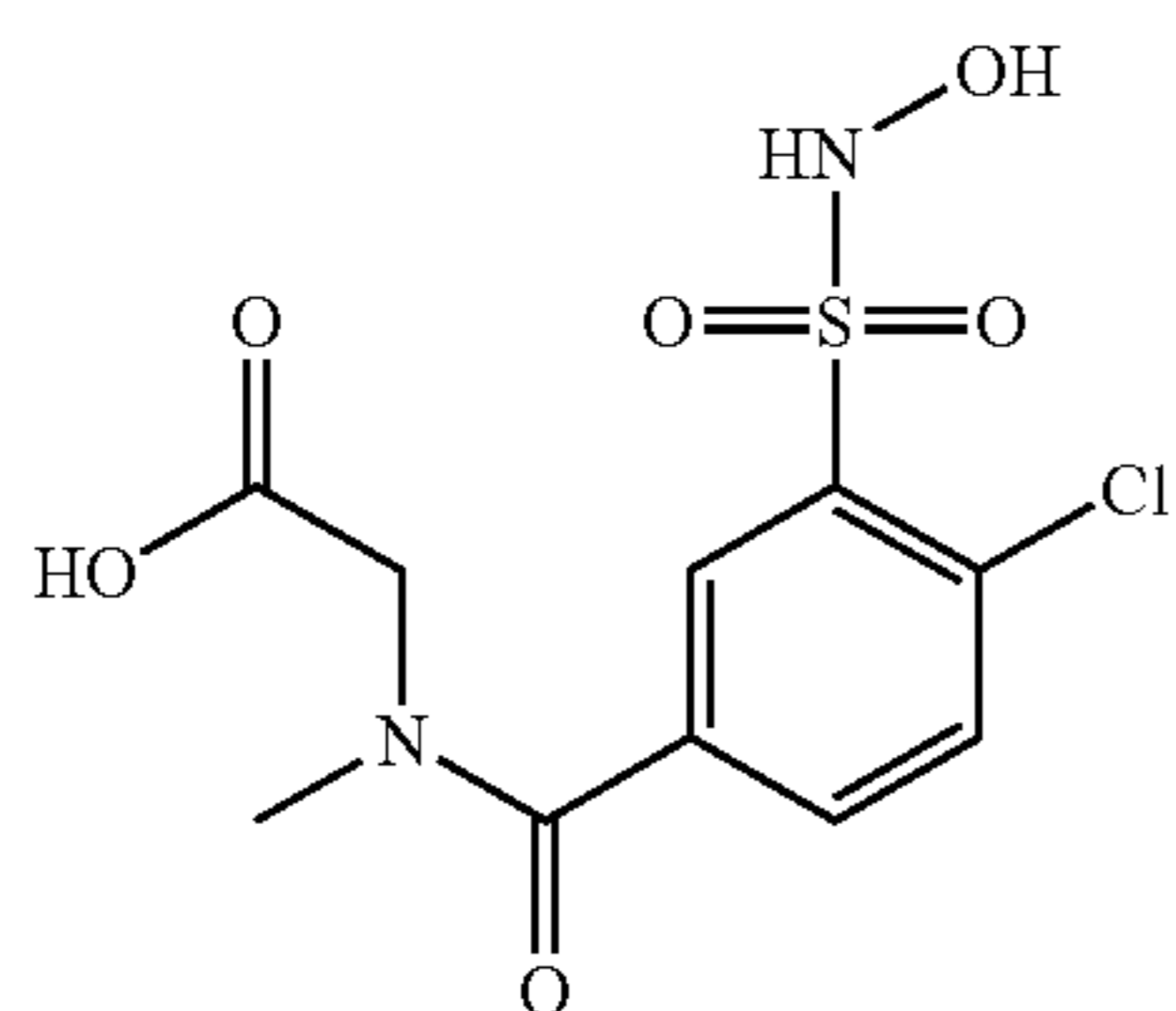
Compound 25
