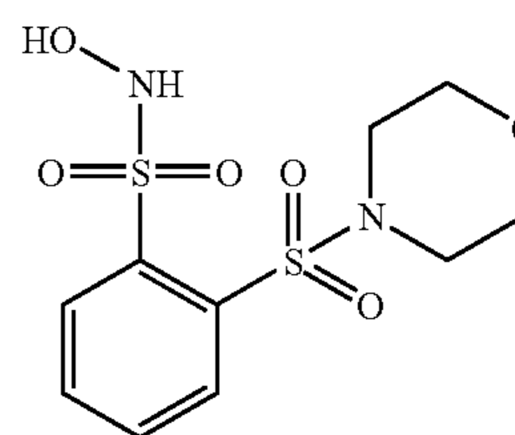
Compound 8
