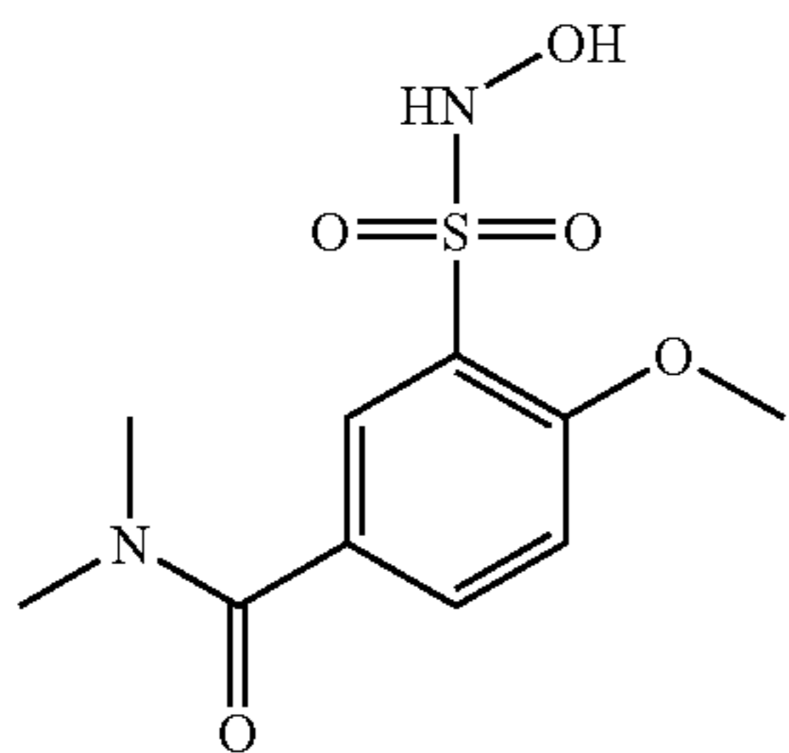
Compound 43
