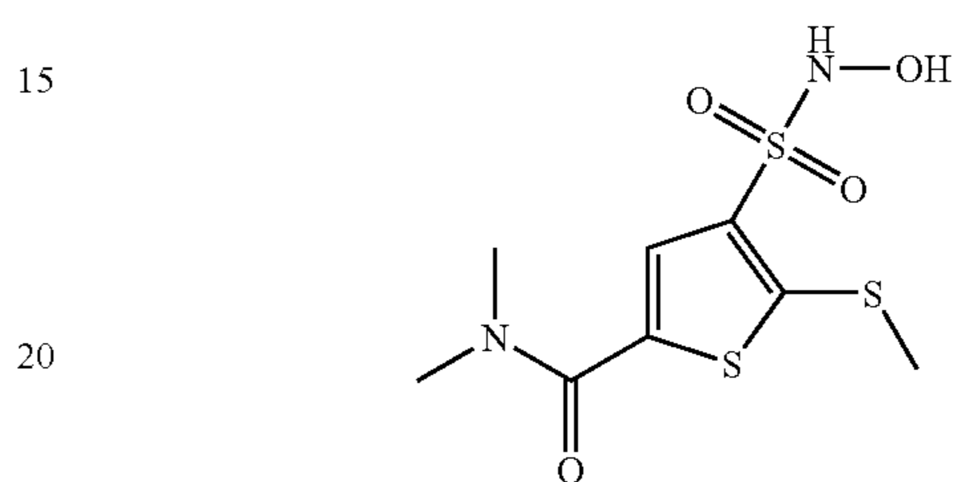
Compound 89
