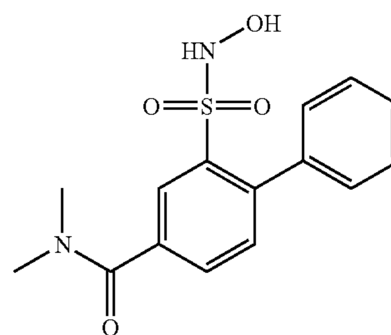
Compound 41
