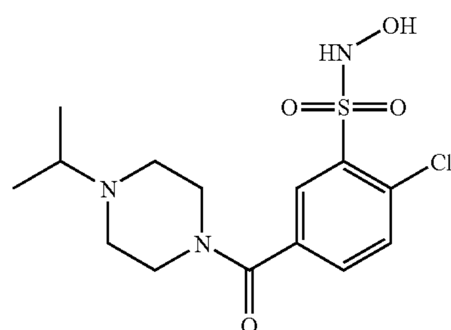
Compound 67
