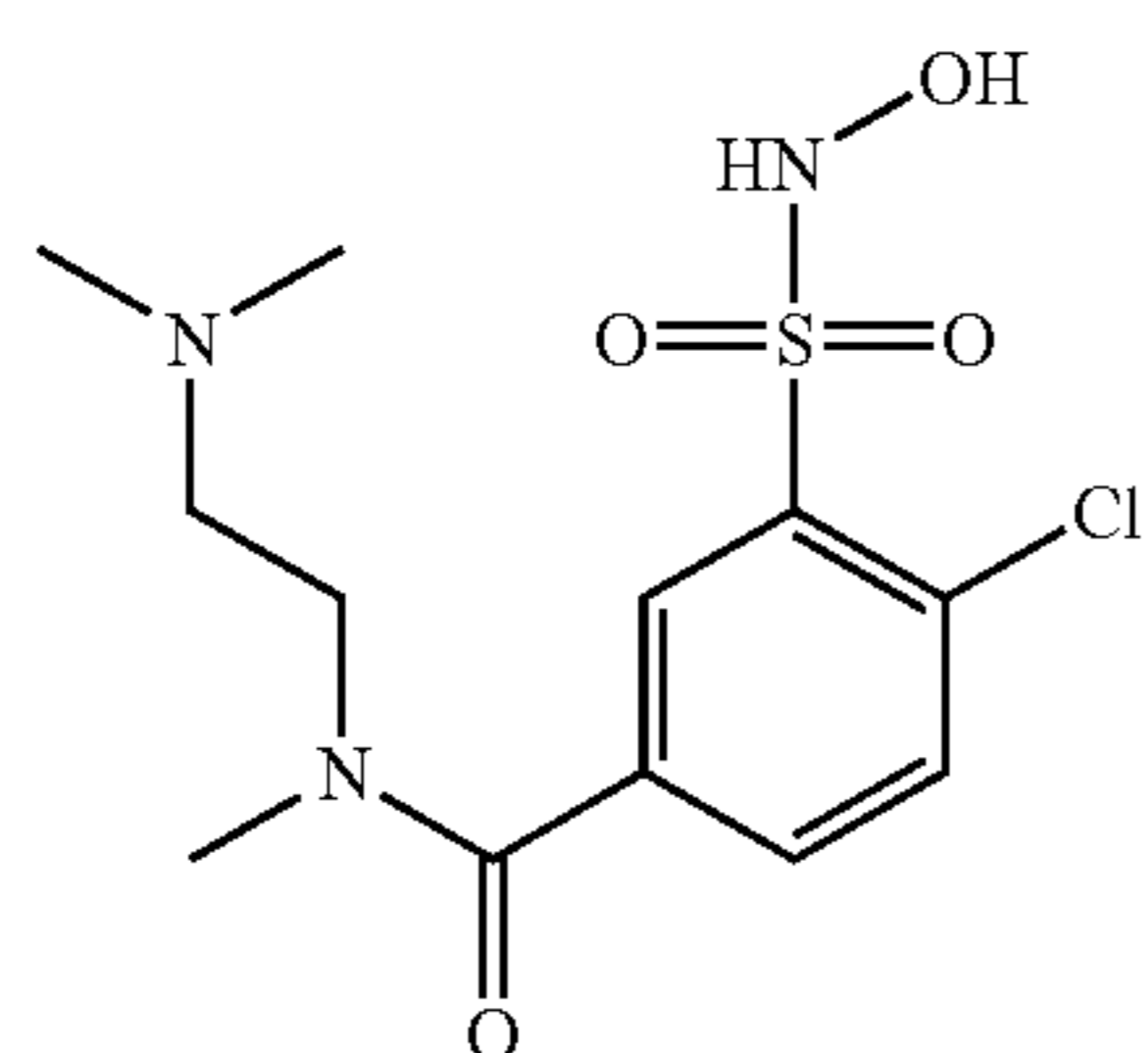
Compound 27
