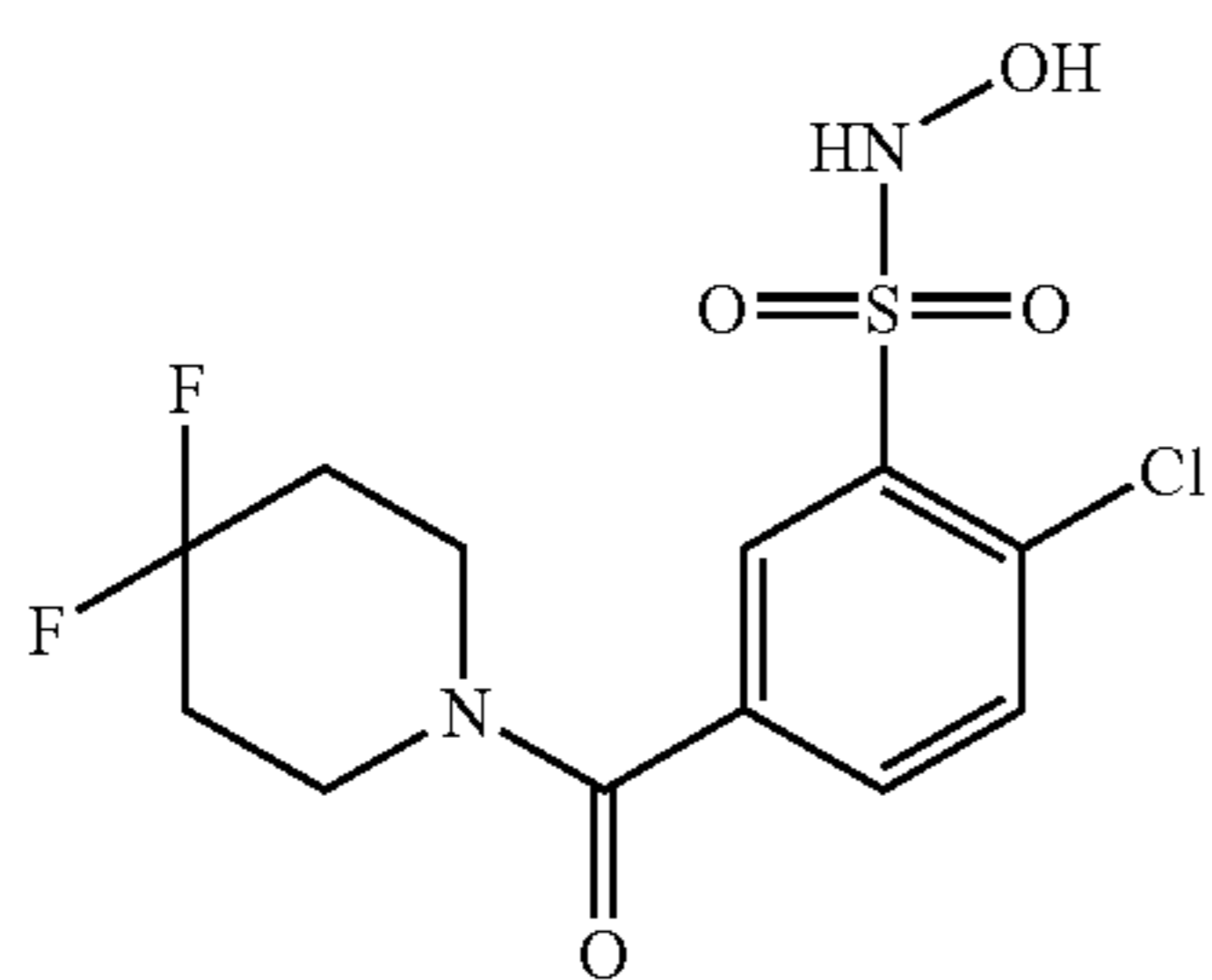
Compound 13
