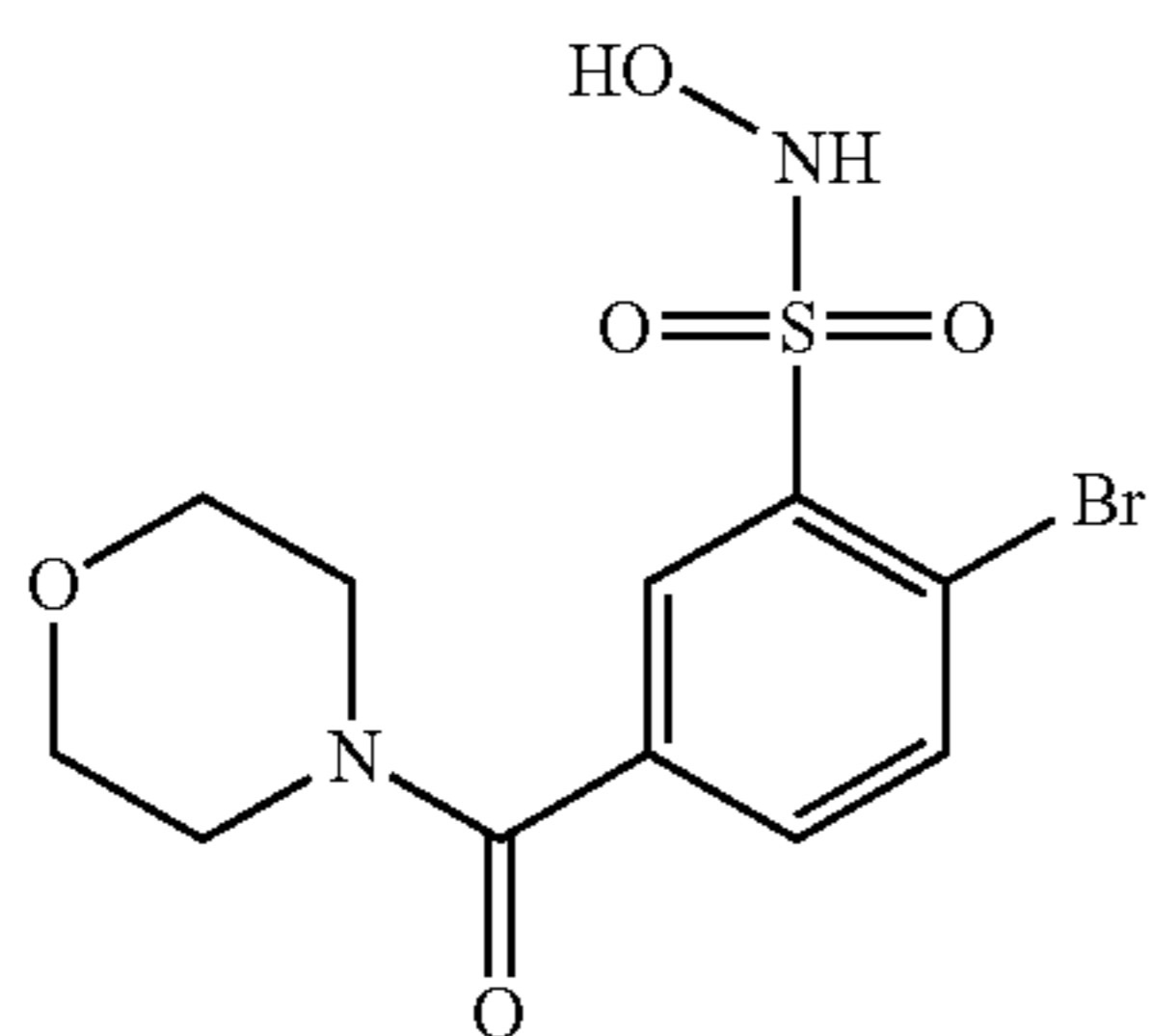
Compound 5
