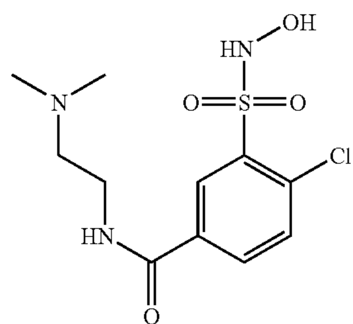
Compound 26
