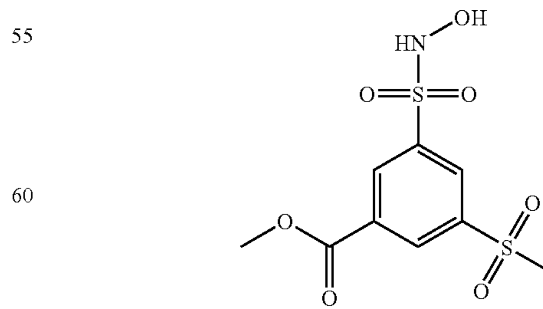
Compound 52
