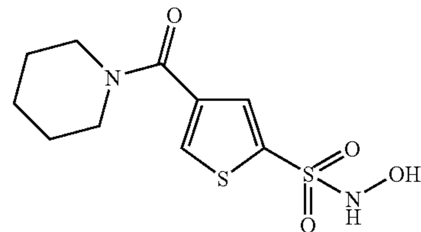
Compound 79
