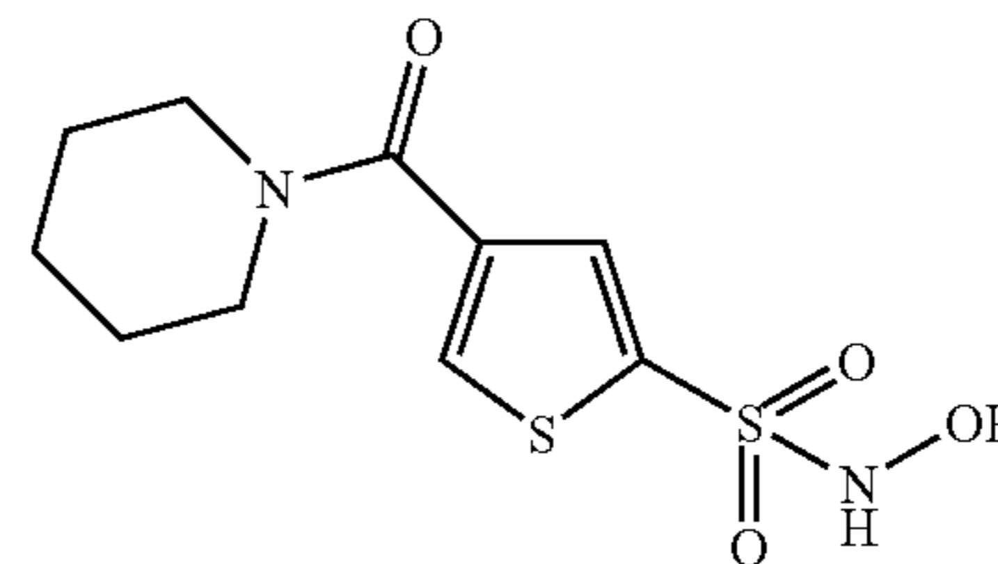
Compound 79
