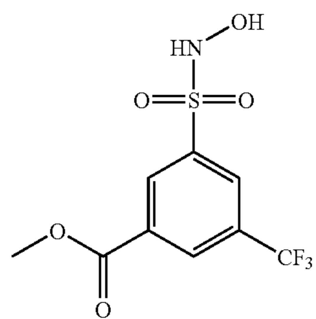
Compound 54
