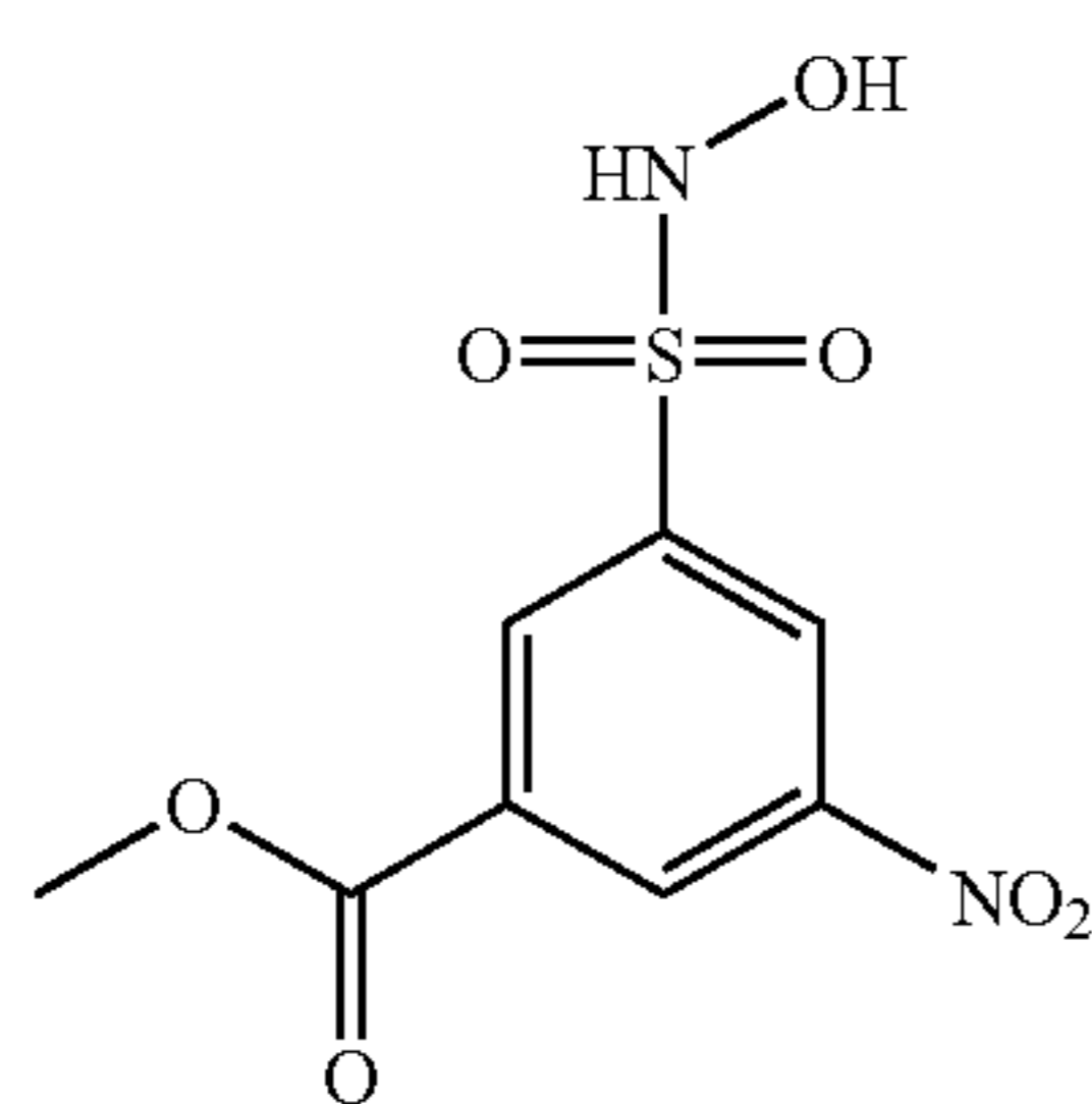
Compound 56
