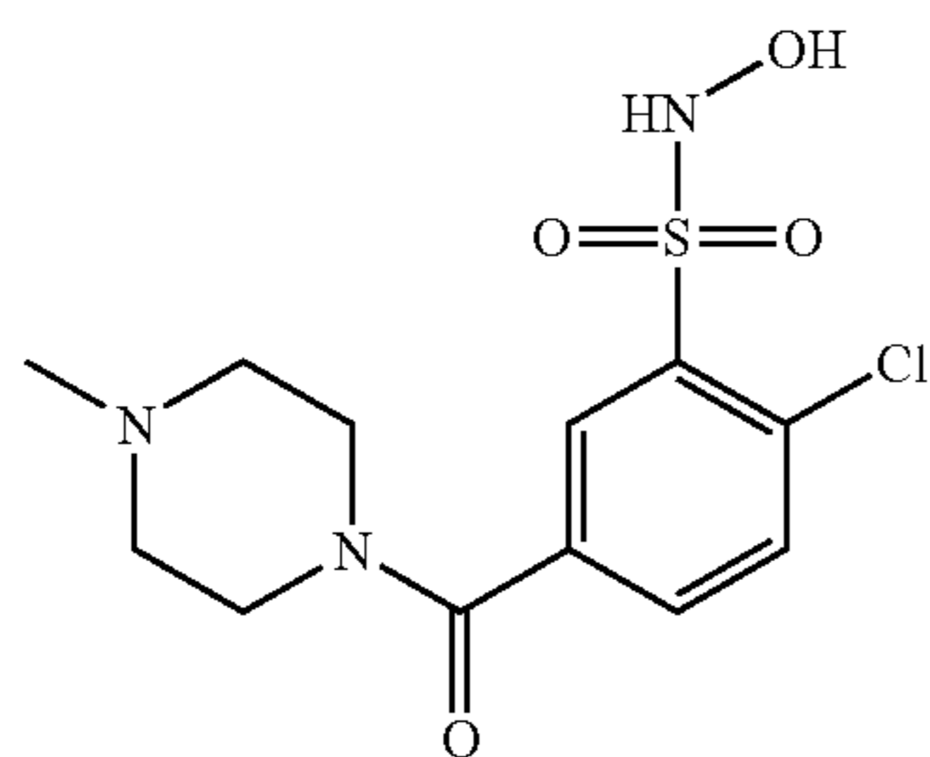
Compound 66
