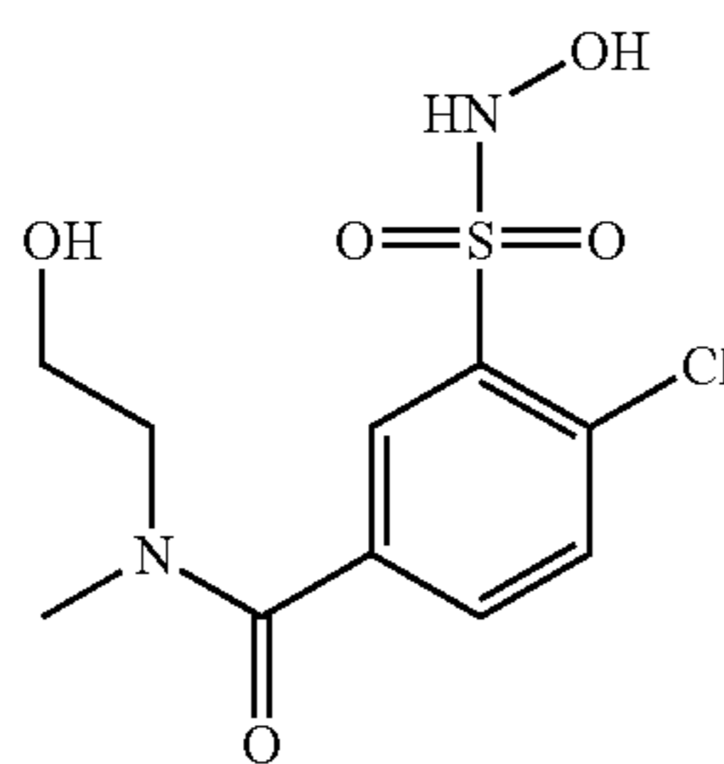
Compound 34
