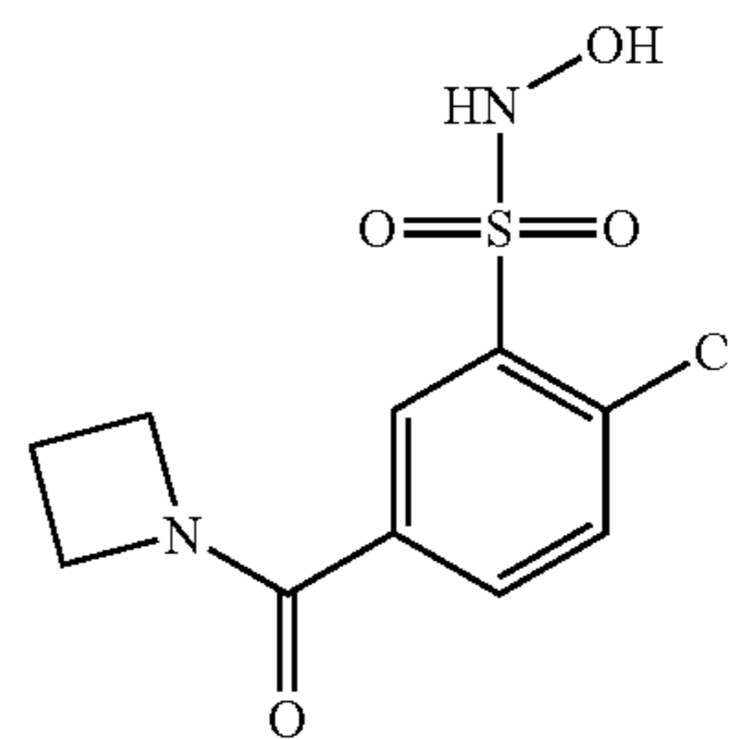
Compound 70
