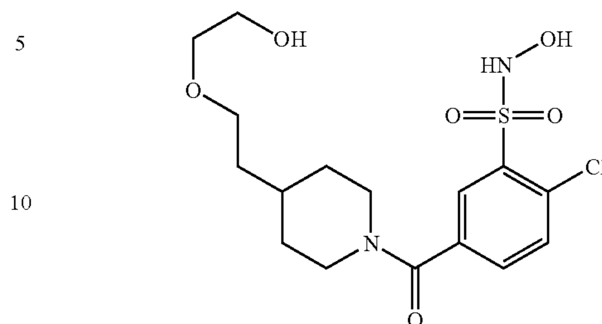
Compound 18
