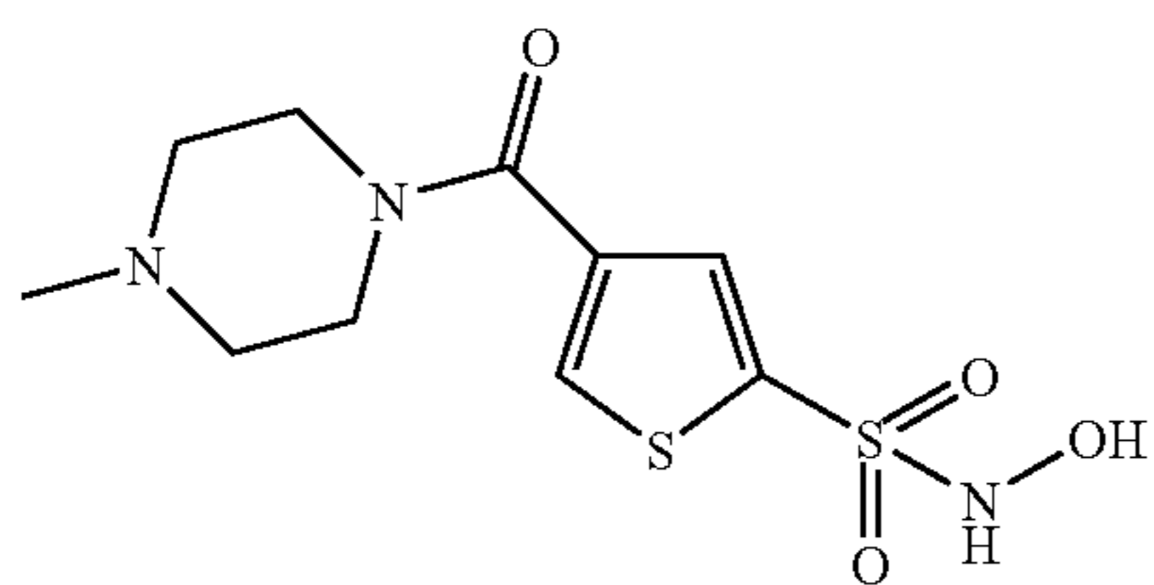
Compound 82
