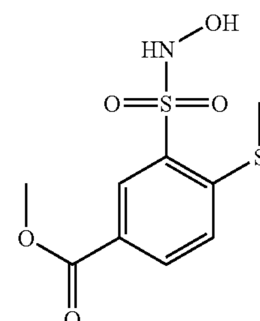
Compound 38
