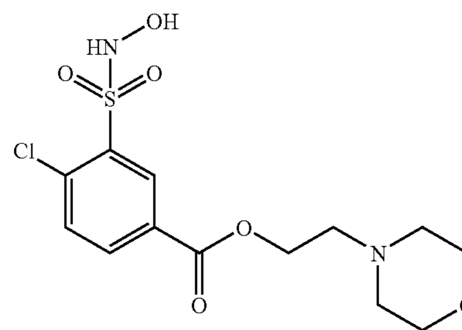
Compound 9
