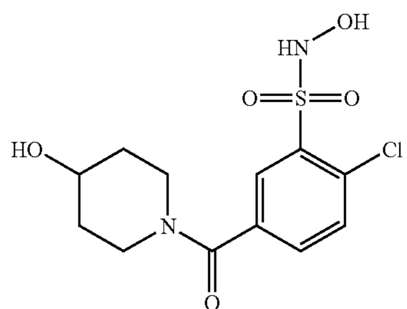
Compound 16
