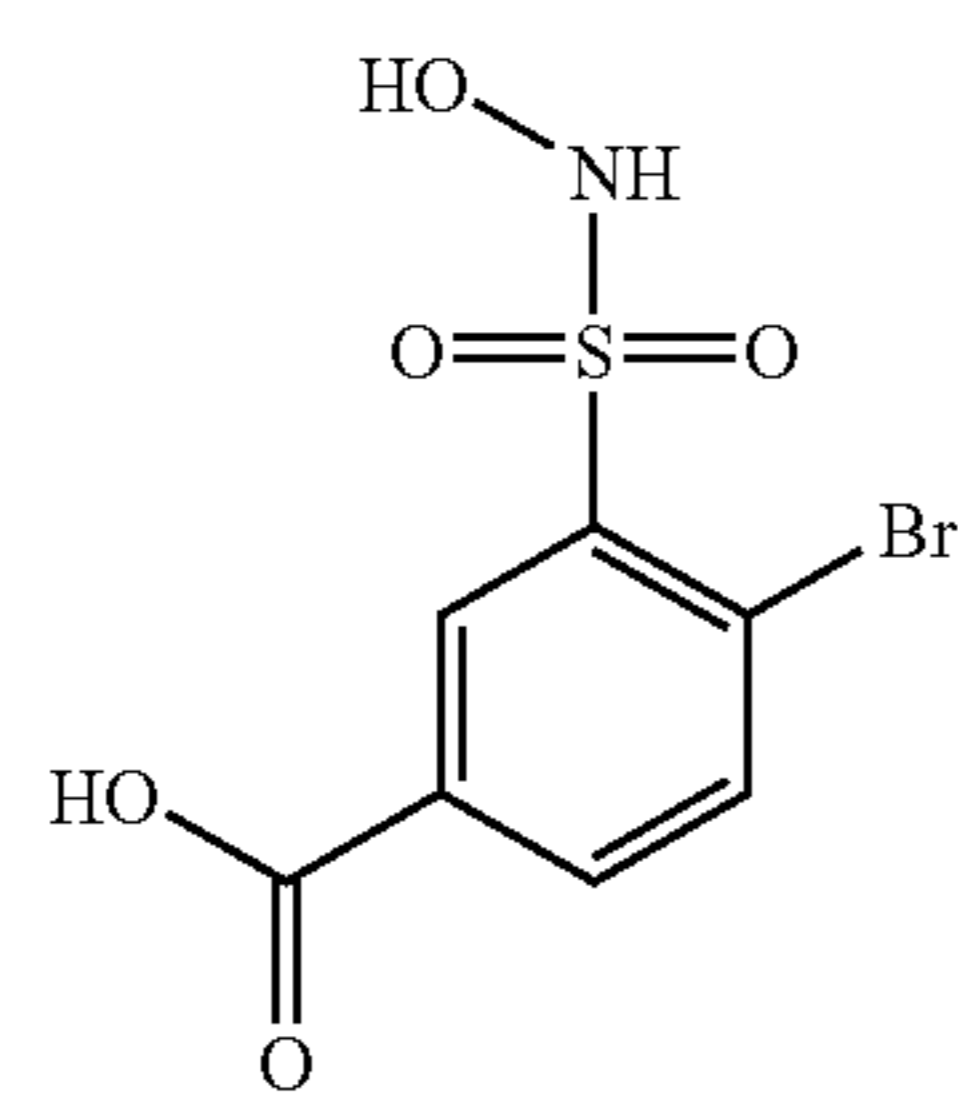
Compound 4
