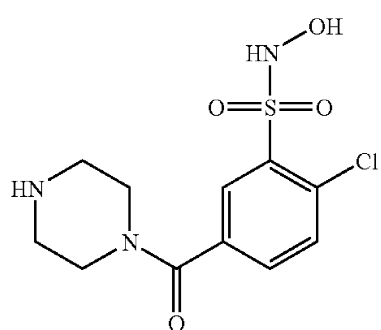
Compound 64
