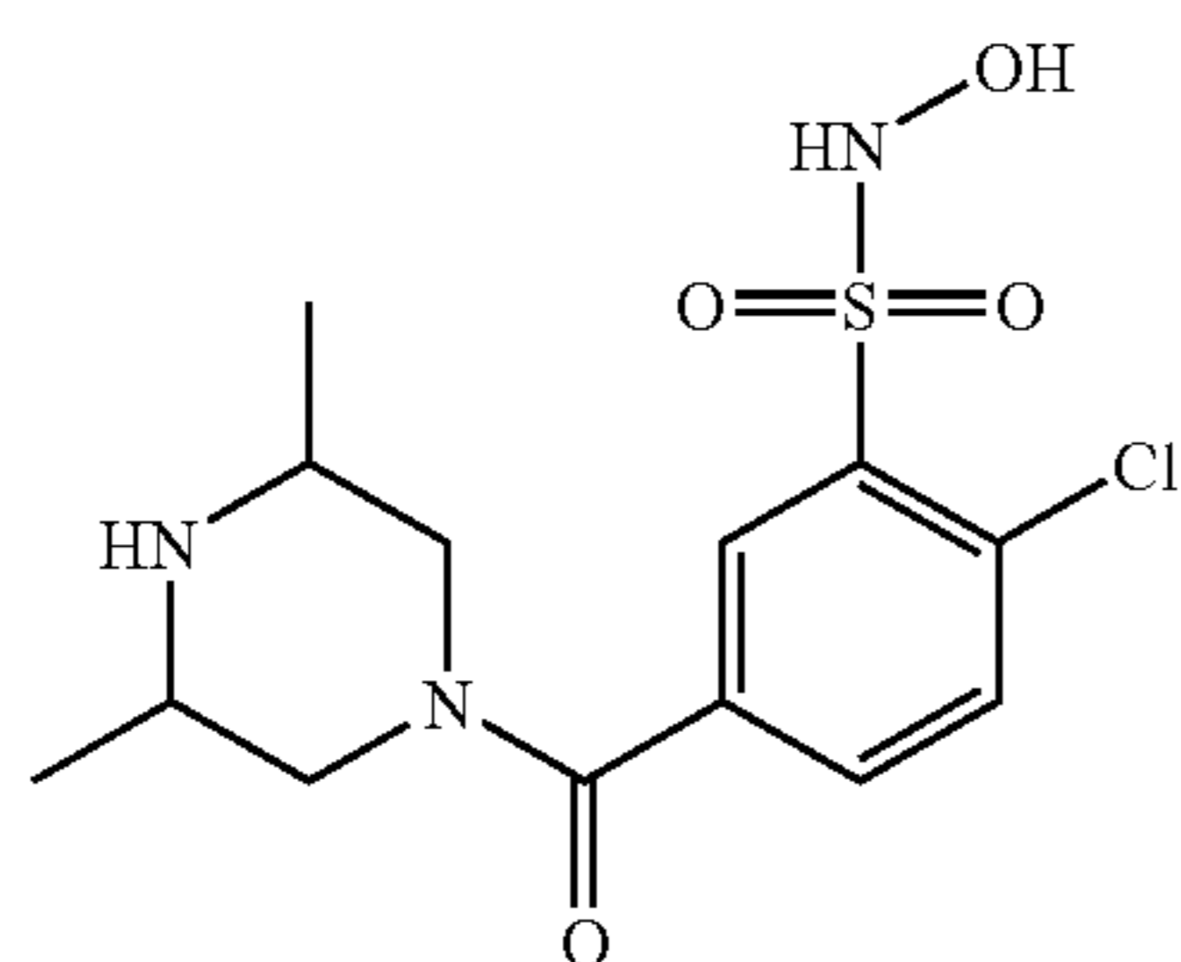
Compound 65
