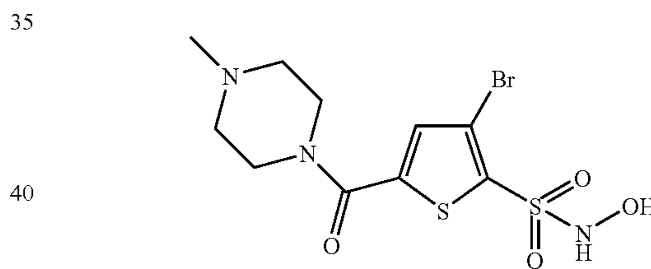
Compound 90
