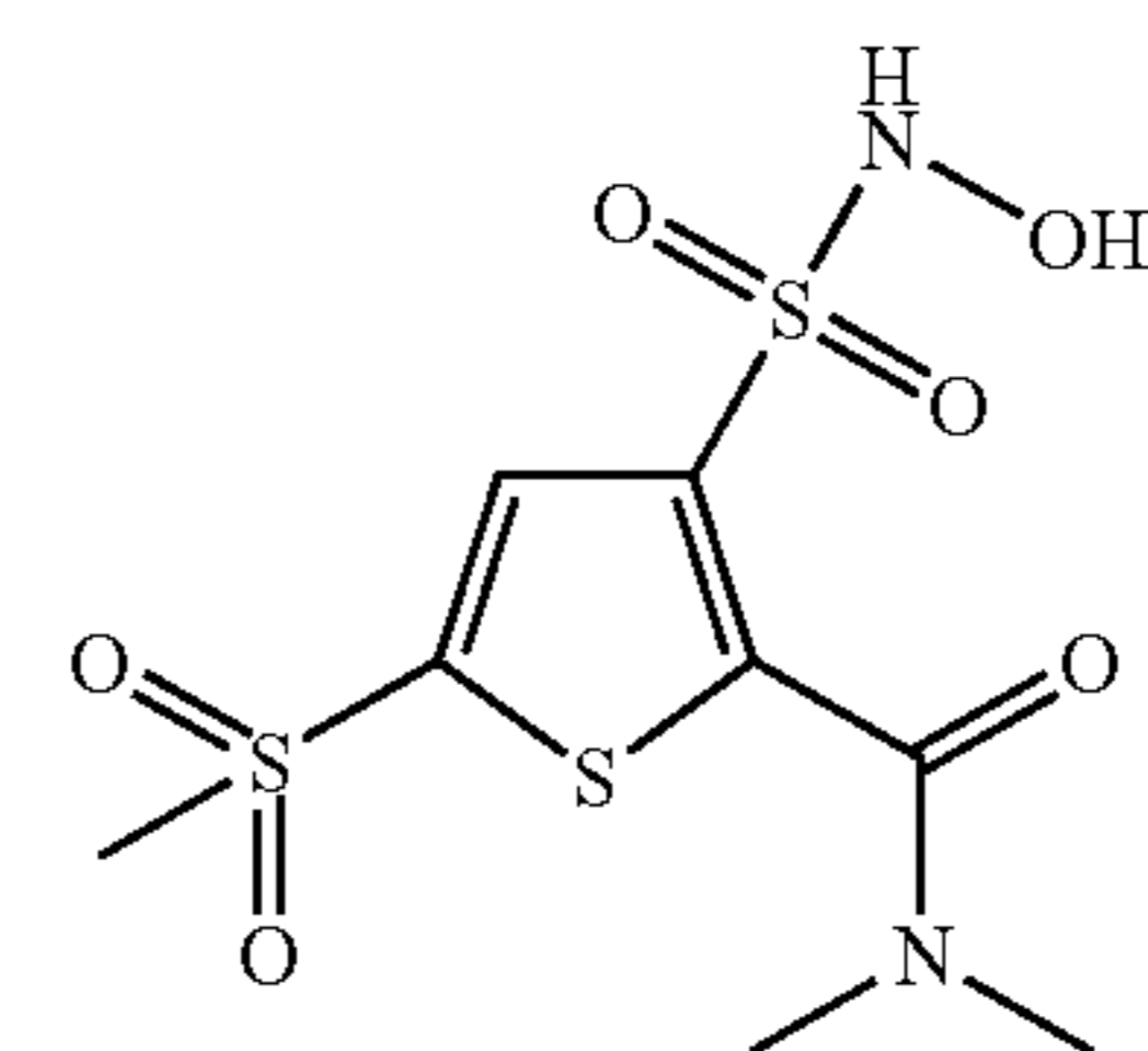
Compound 77
