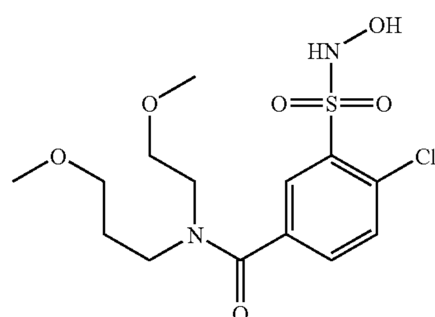
Compound 37
