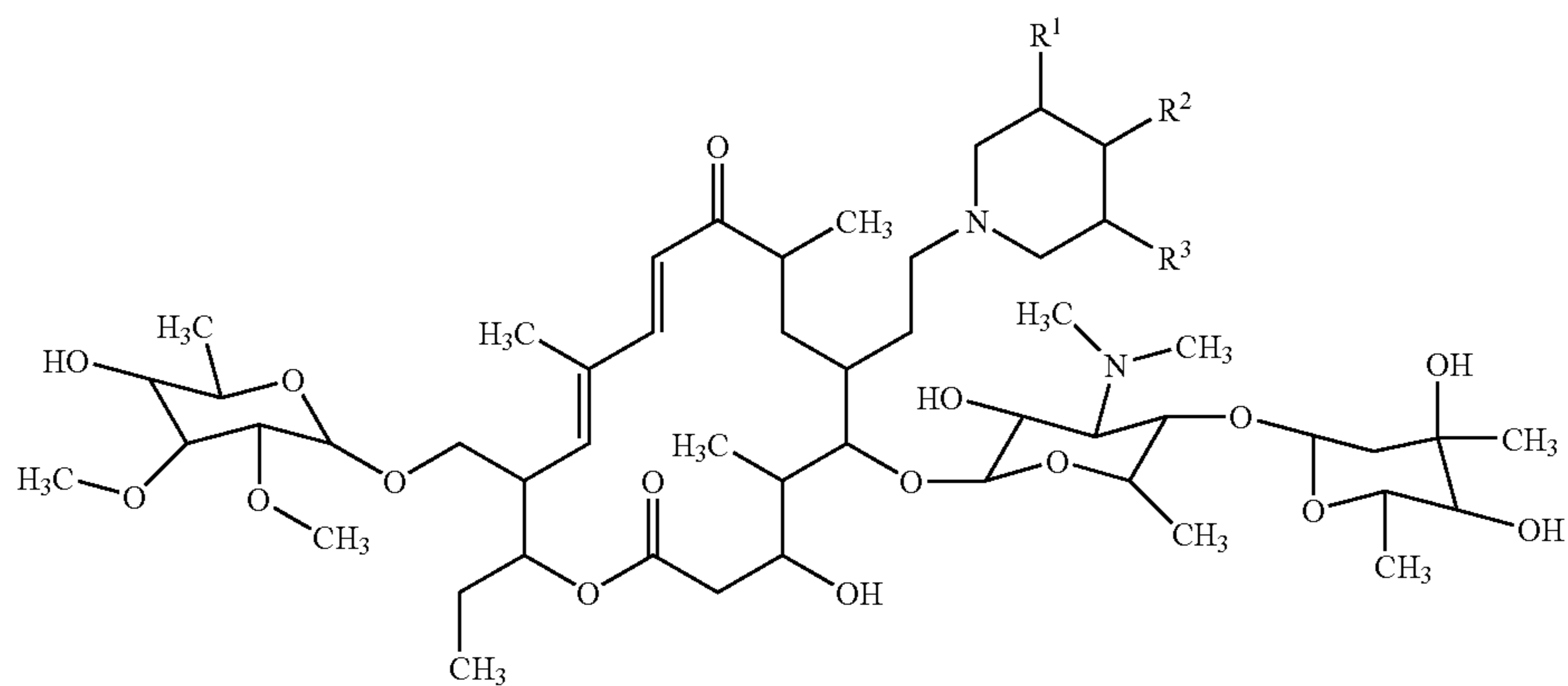
20-piperidinyl-tylosin compound
