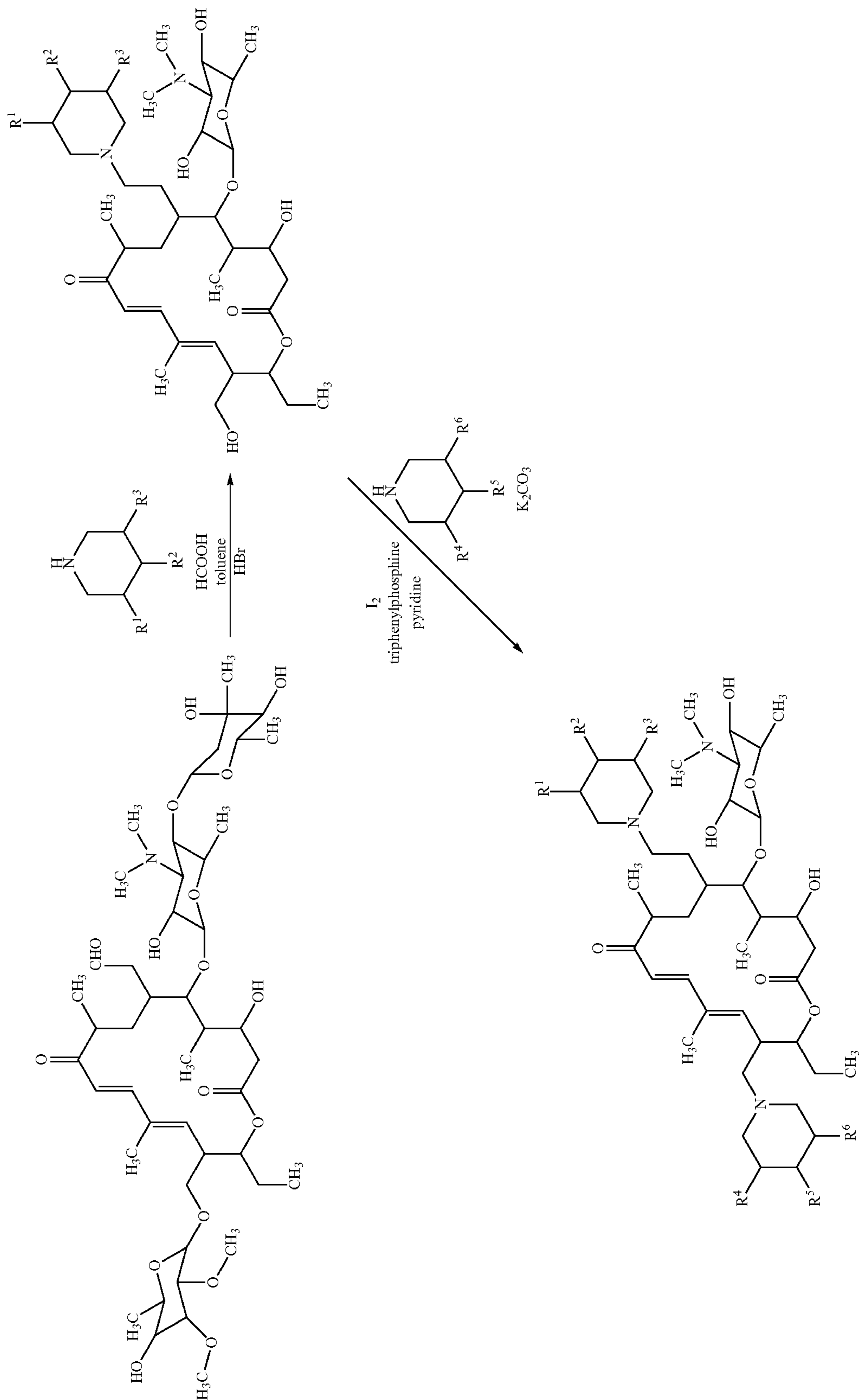
Scheme V
