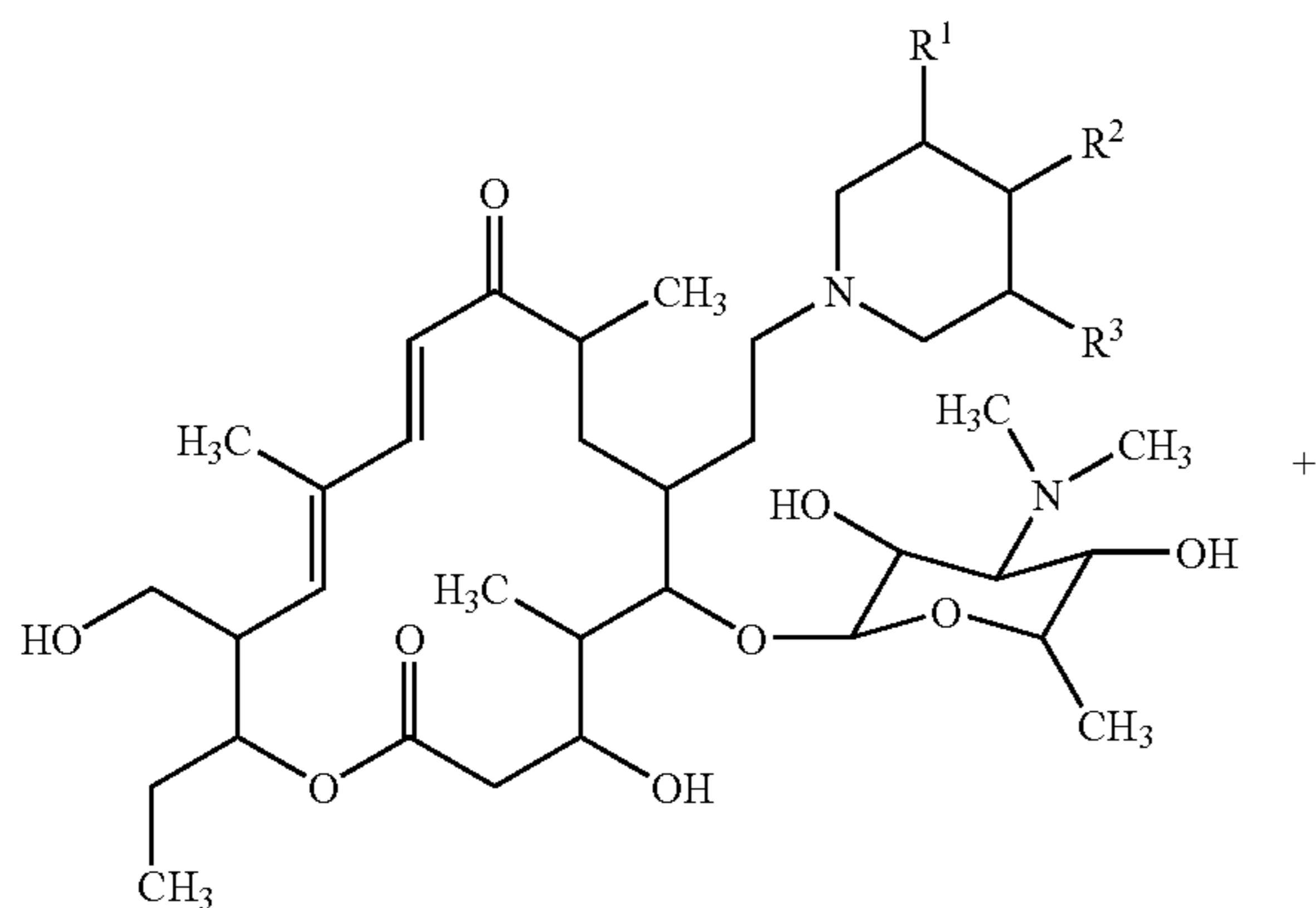
23-hydroxyl-20-piperidinyl-5-O-mycaminosyl-tylonolide compound
