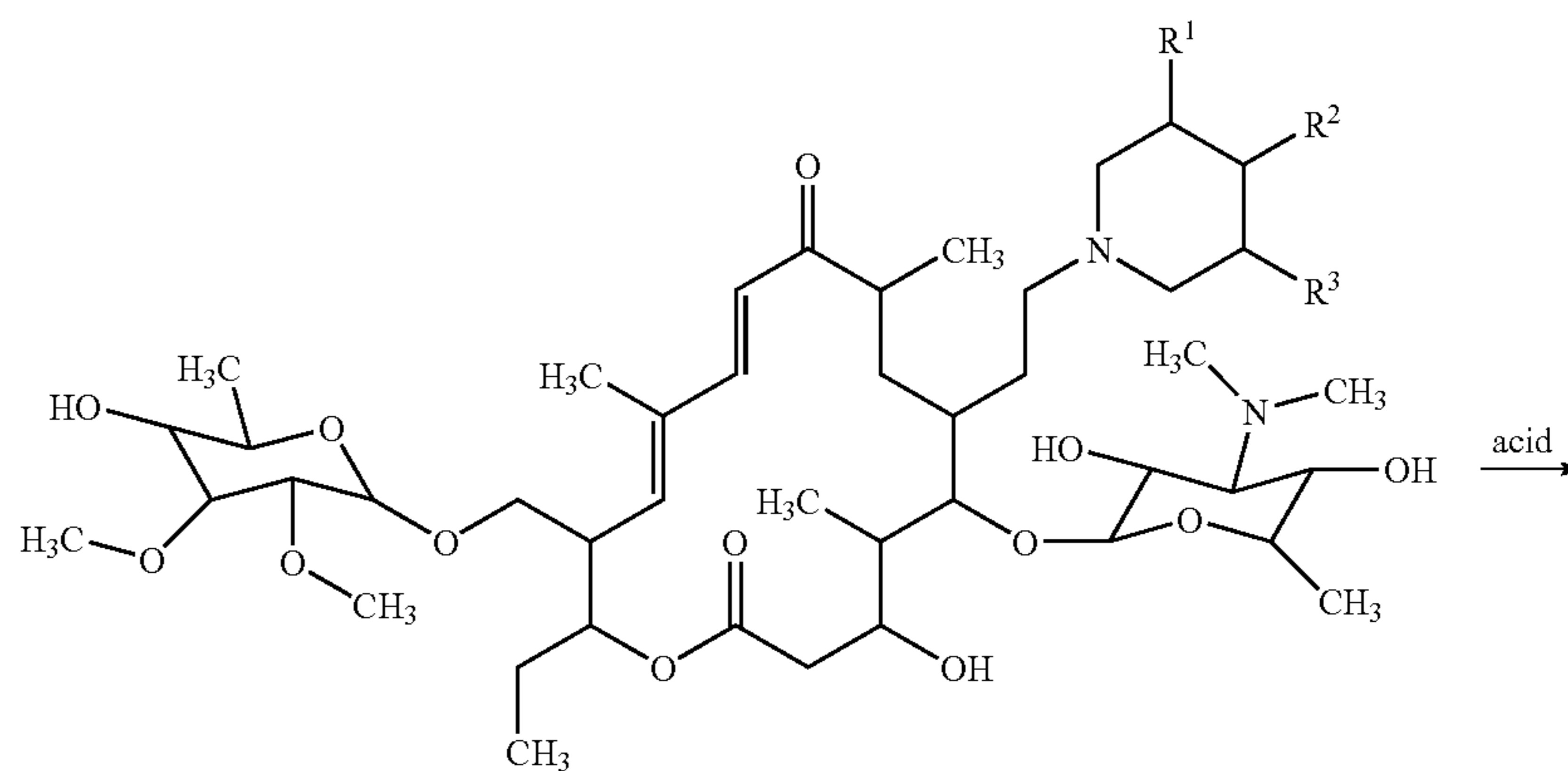
23-O-mycinosyl-20-piperidinyl-5-O-mycaminosyl-tylonolide compound
