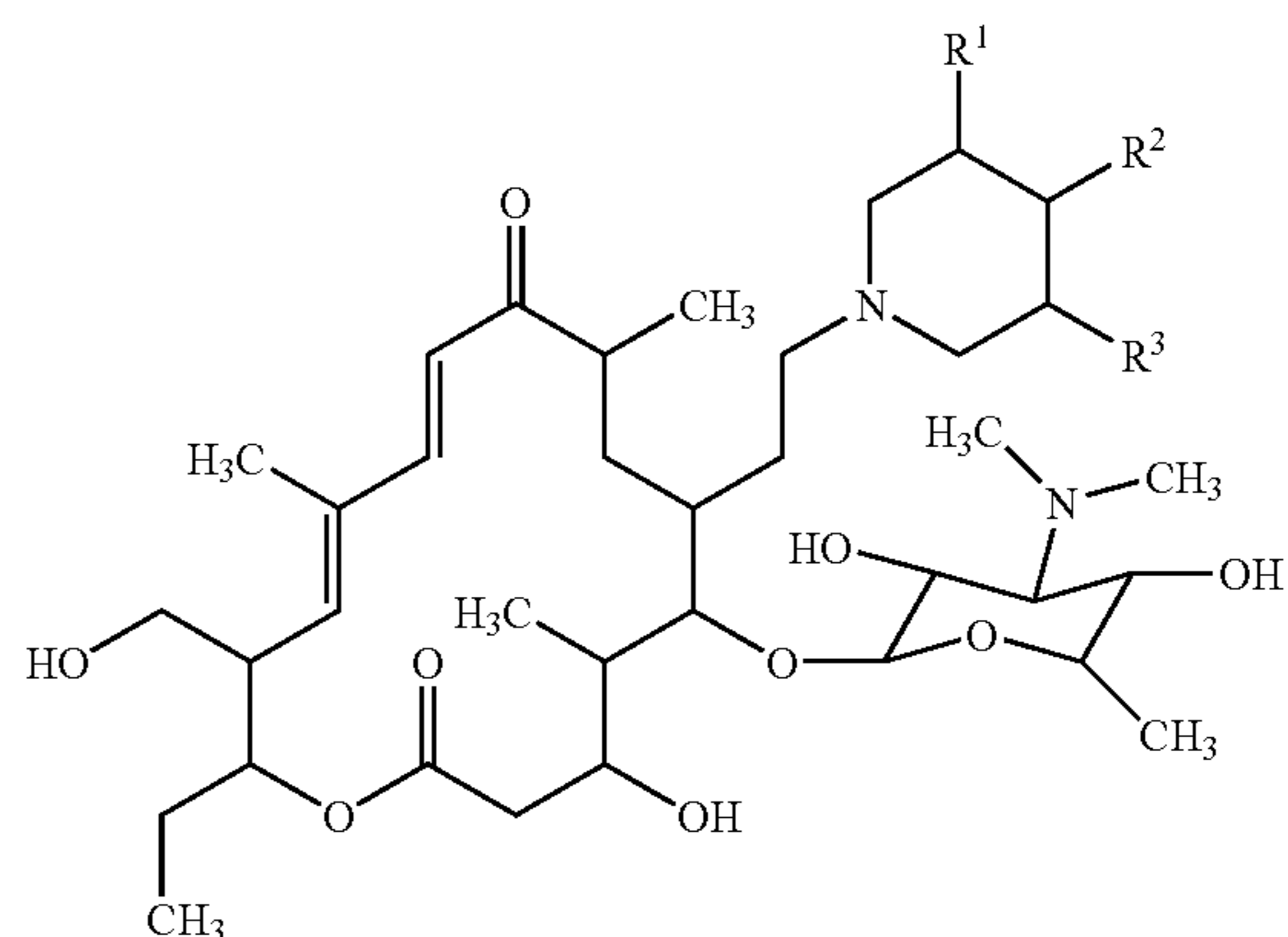
23-hydroxy-20-piperidinyl-5-O-mycaminosyl-tylonolide compound
