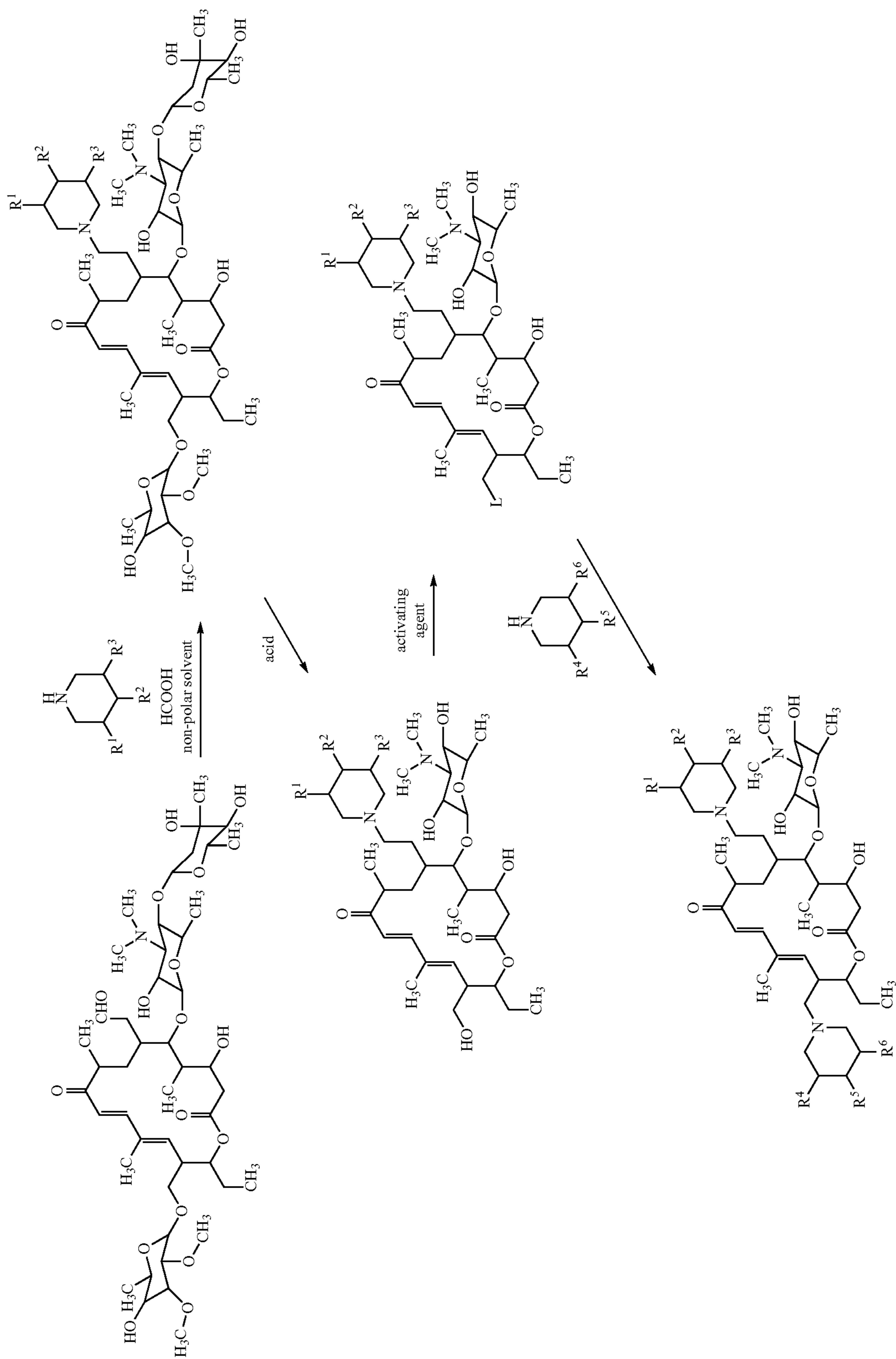
Scheme III
