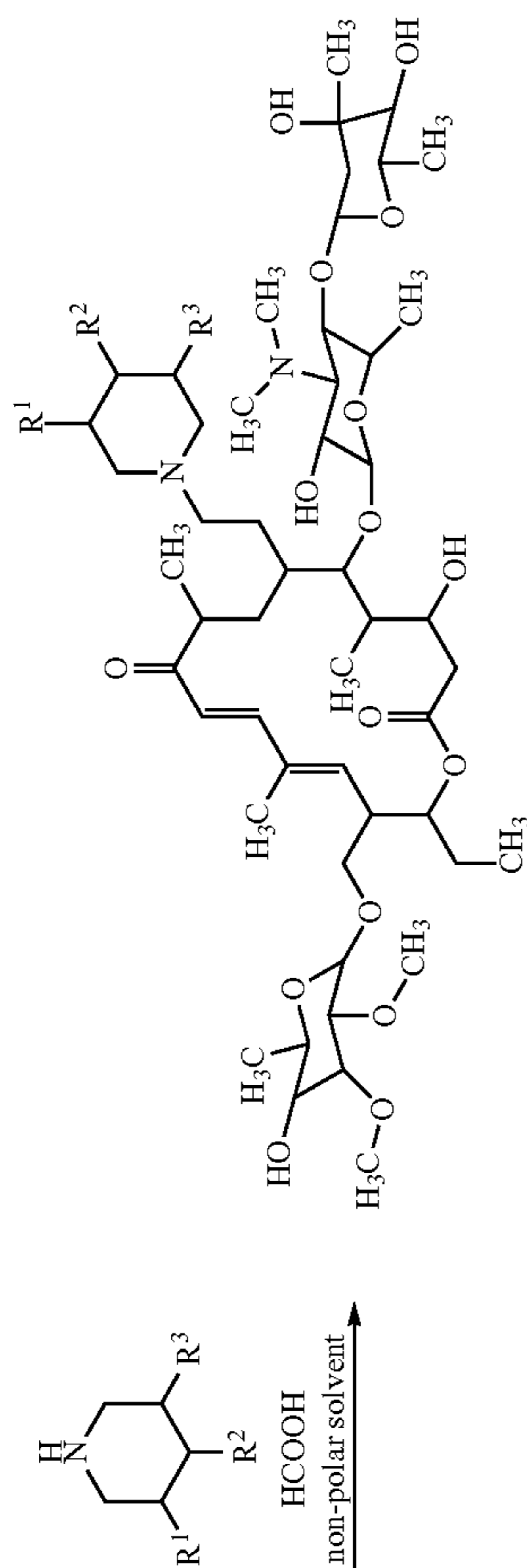
Scheme I
