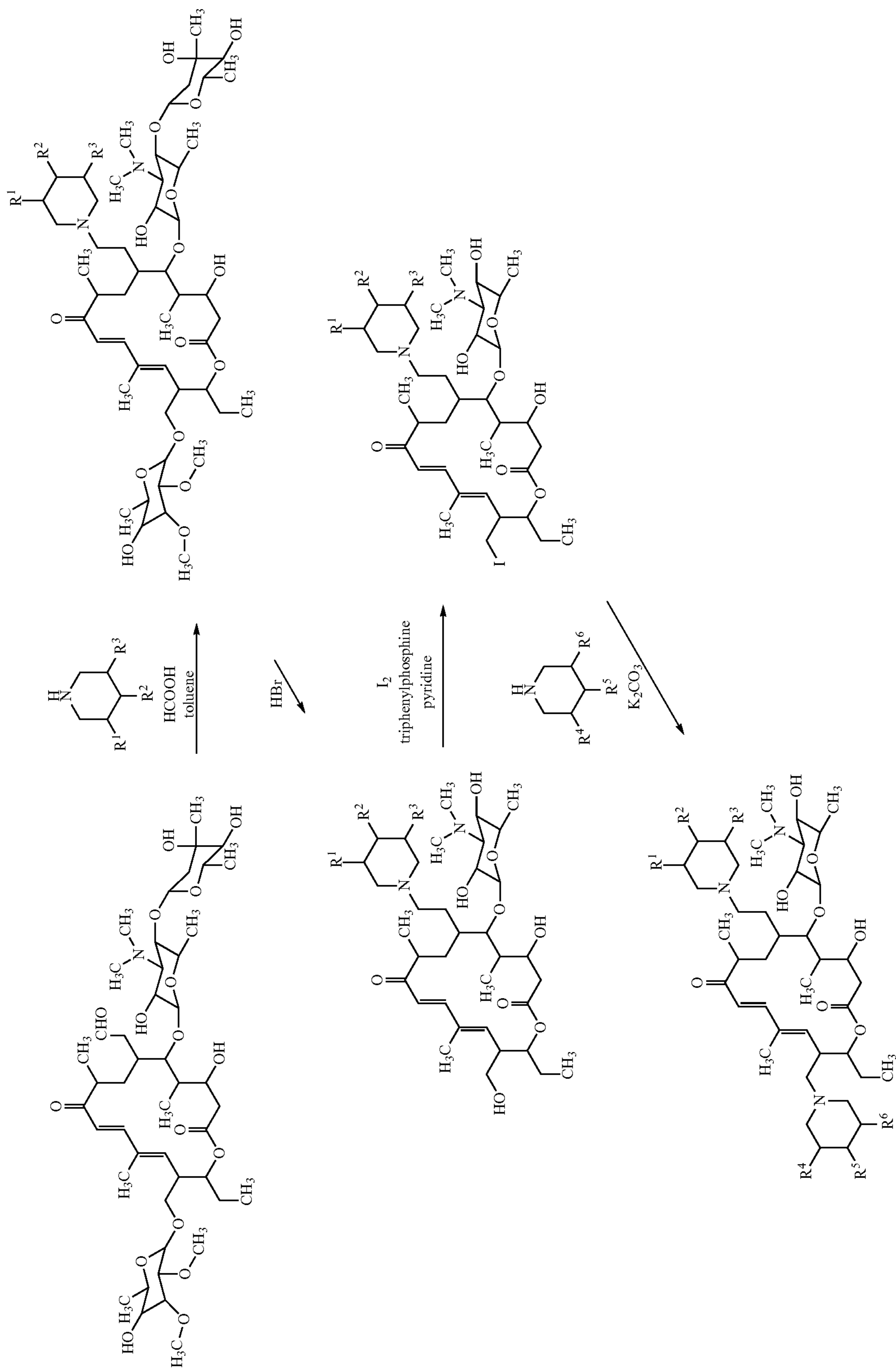
Scheme IV
