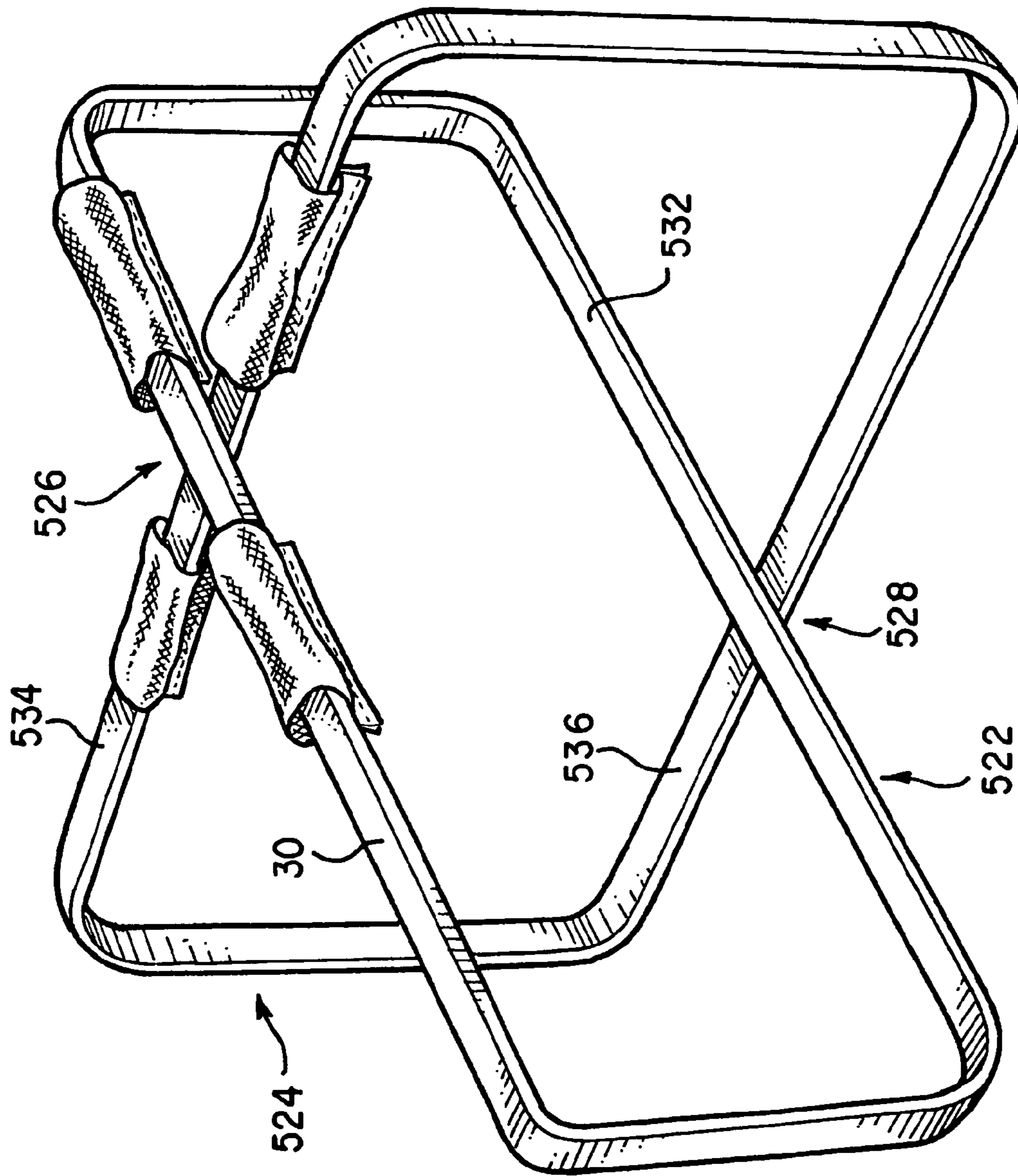
FIG. 21C (PRIOR ART)
