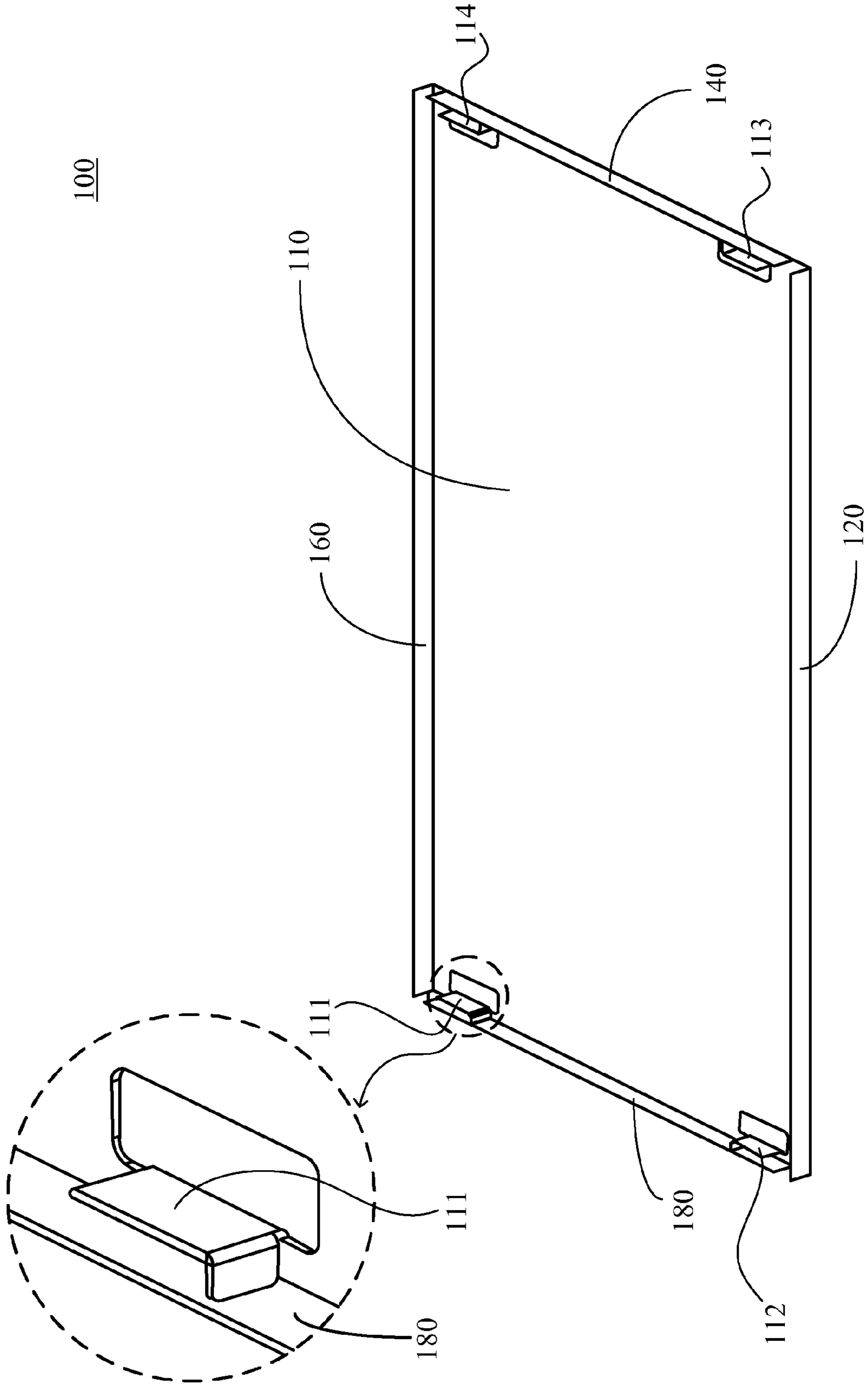
FIG. 1 (prior art)
