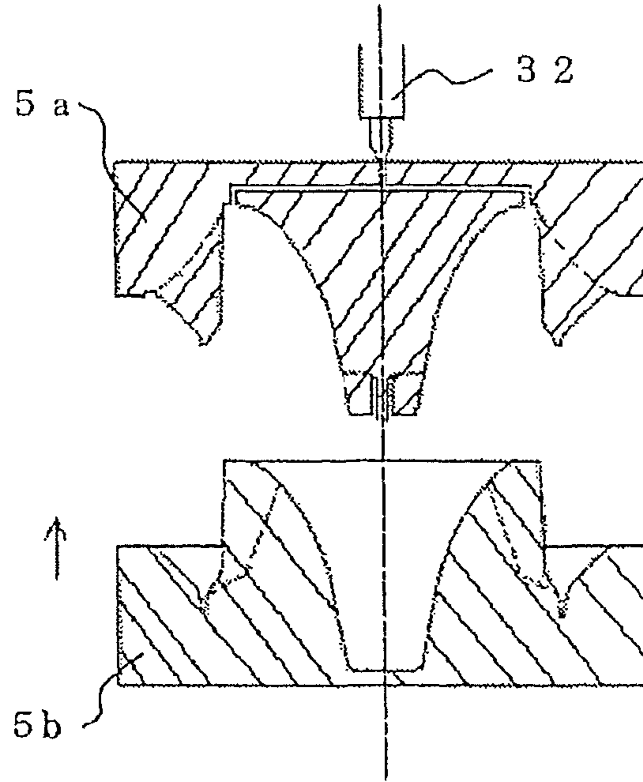
(b) RESIN INFUSION STEP
