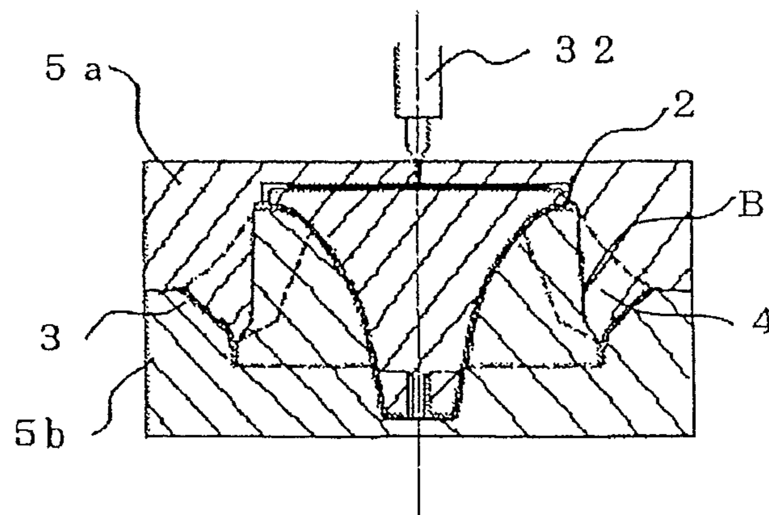
(c) RESIN COOLING STEP
