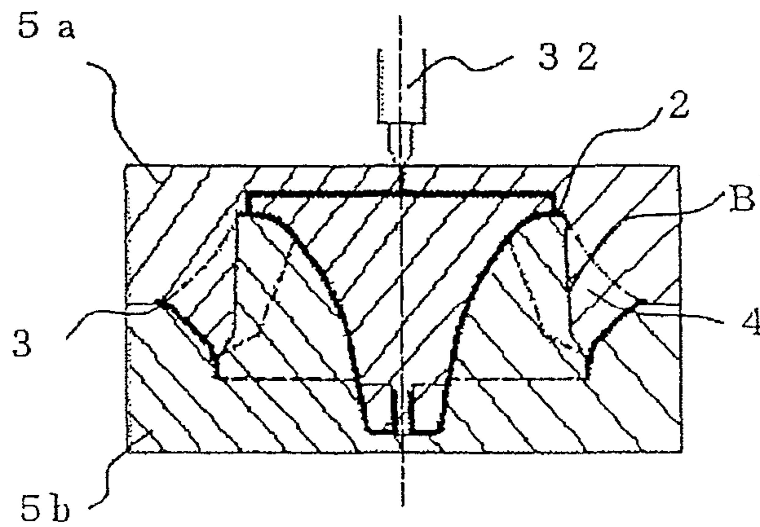
(c) RESIN COOLING STEP
