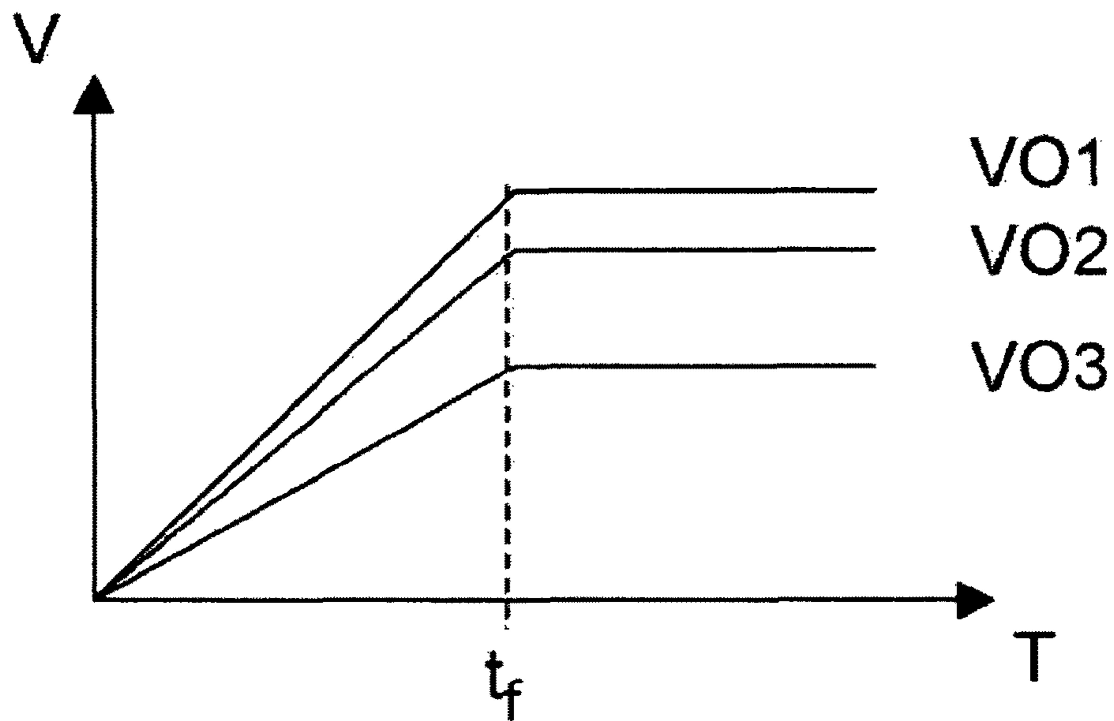
(a) Ratiometric tracking
