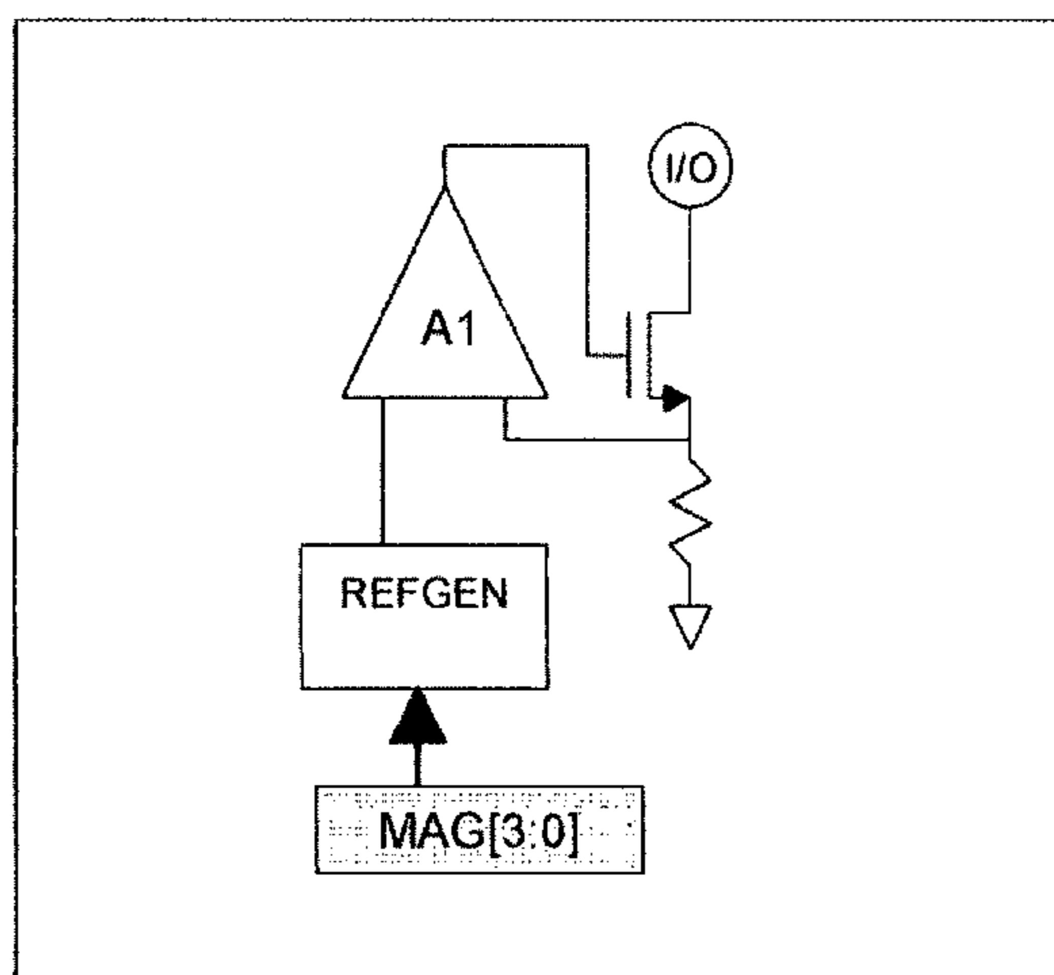
(a) Current-regulated output.
