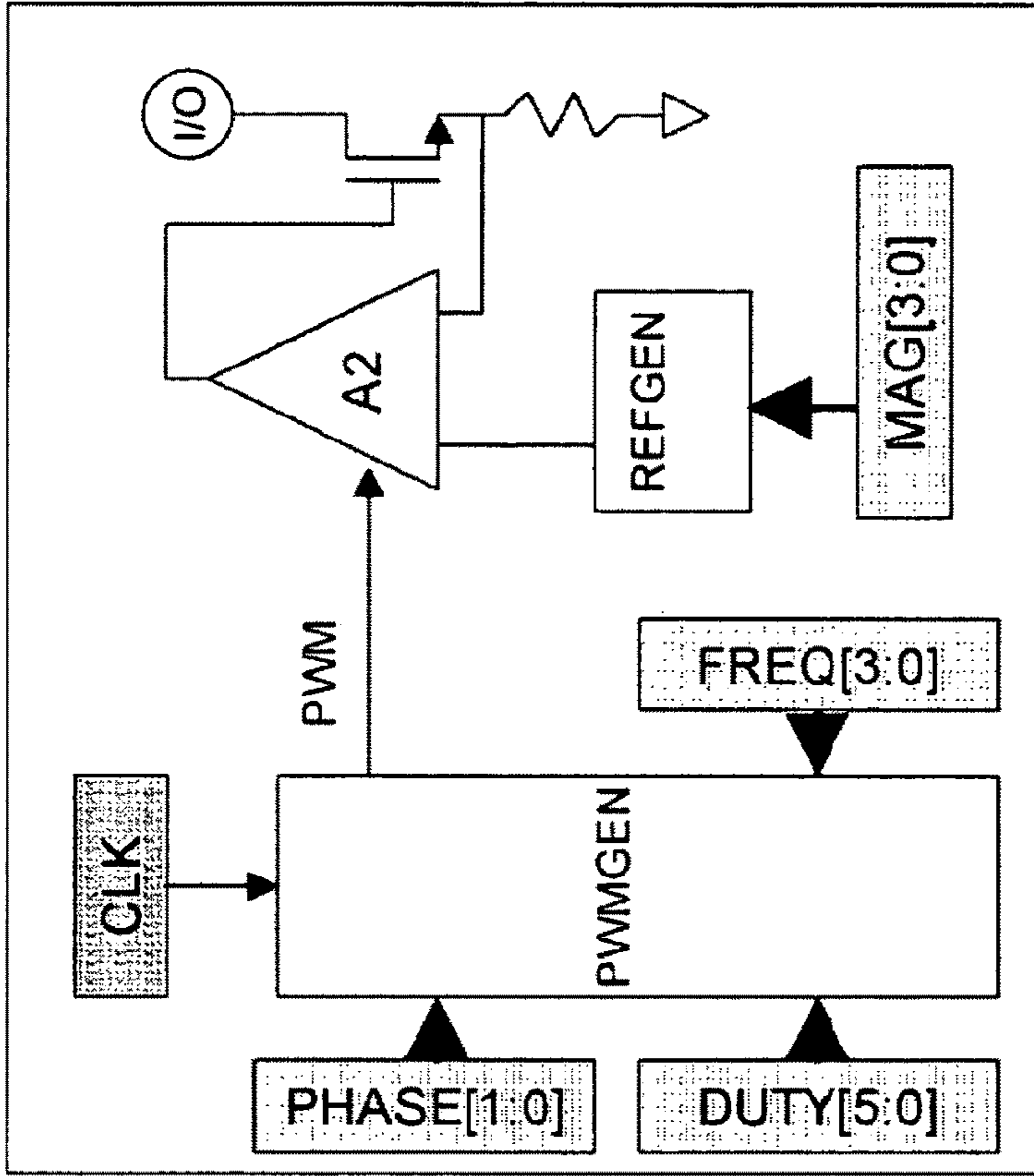
(b) Pulse Width Modulated (PWM) current-regulated output.
