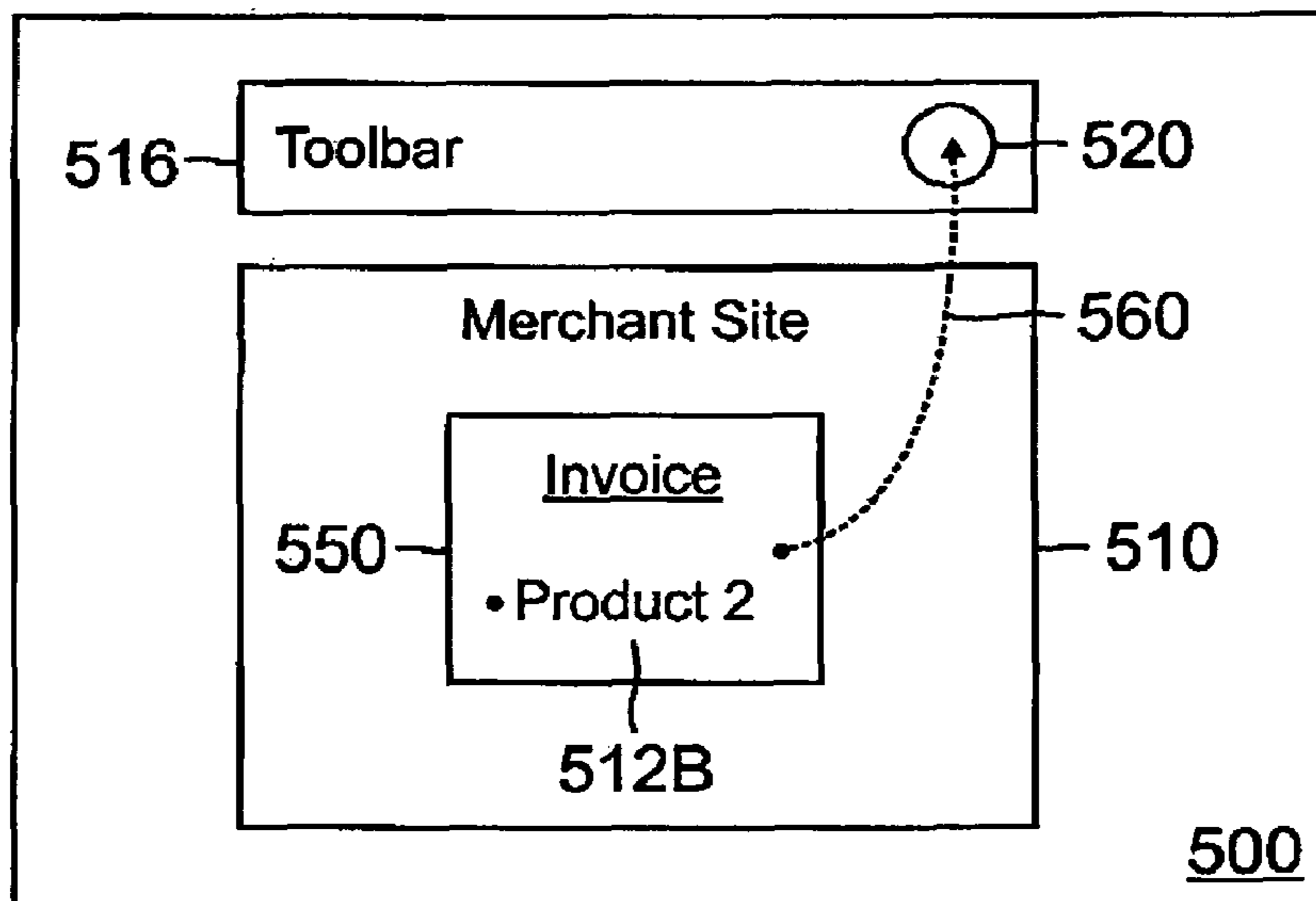
Drag-and-Drop Invoice Icon in Desktop Toolbar
