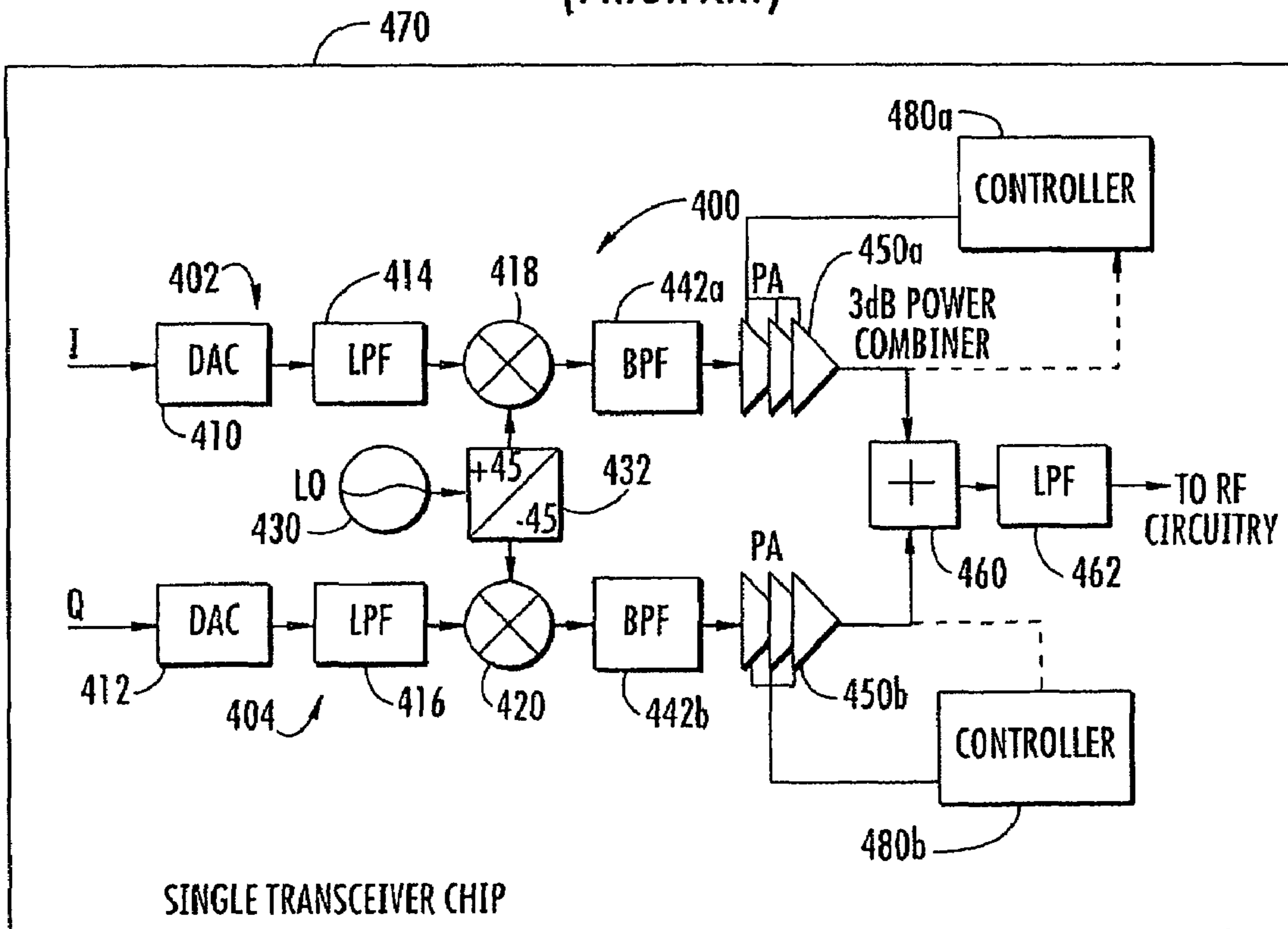
FIG. 4 (PRIOR ART)
