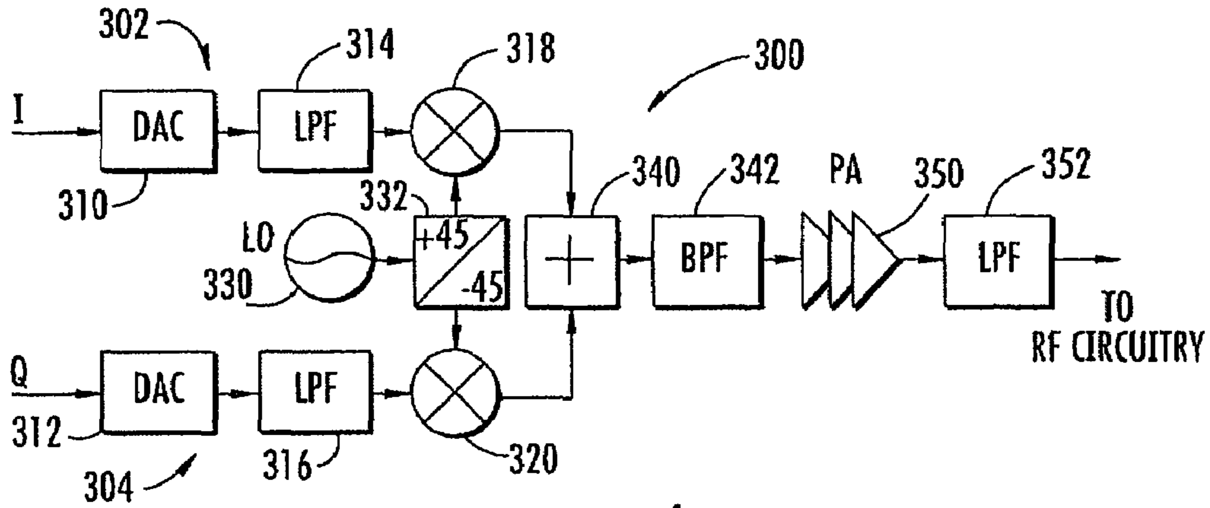
FIG. 4 (PRIOR ART)
