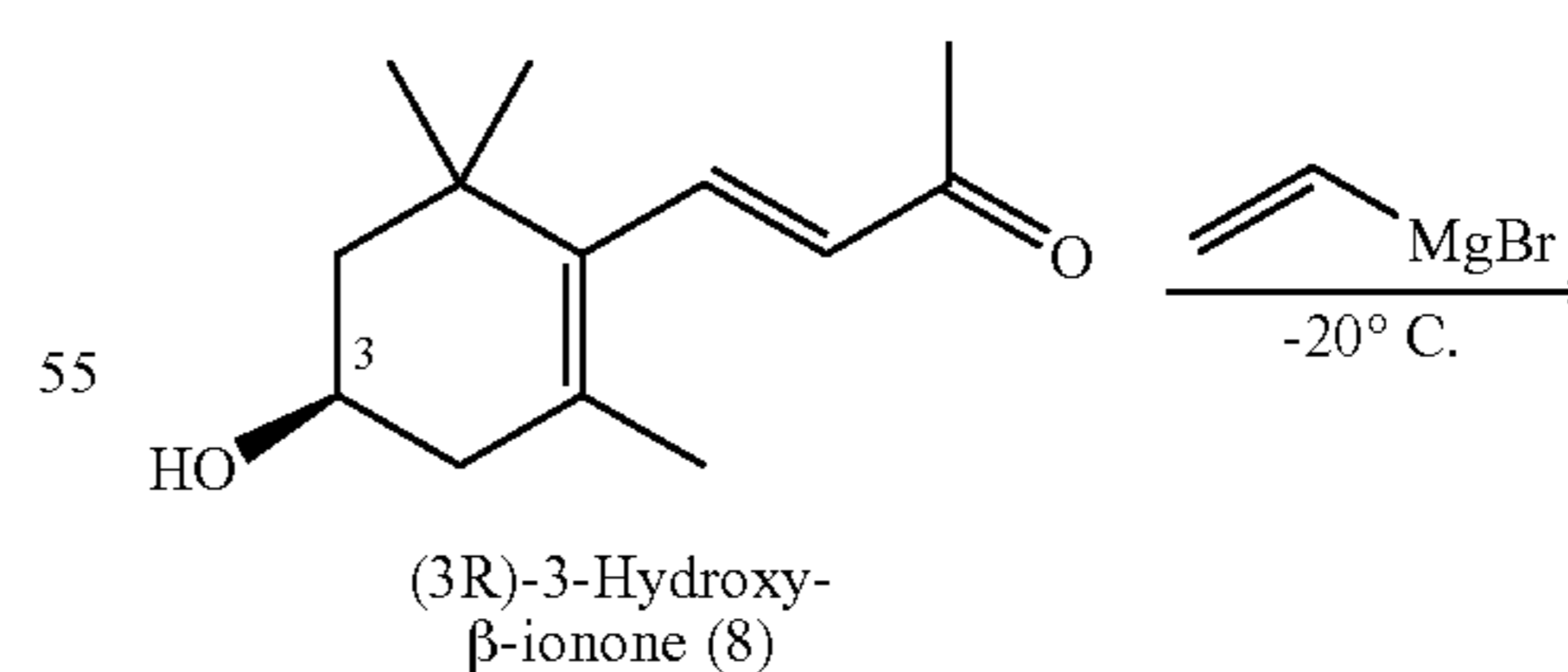
Scheme 9. Transformation of (3R)-3-hydroxy- \beta -ionone (8) and its 3S-isomer (9) to Wittig salts 12 and 13 according to published procedures.*
