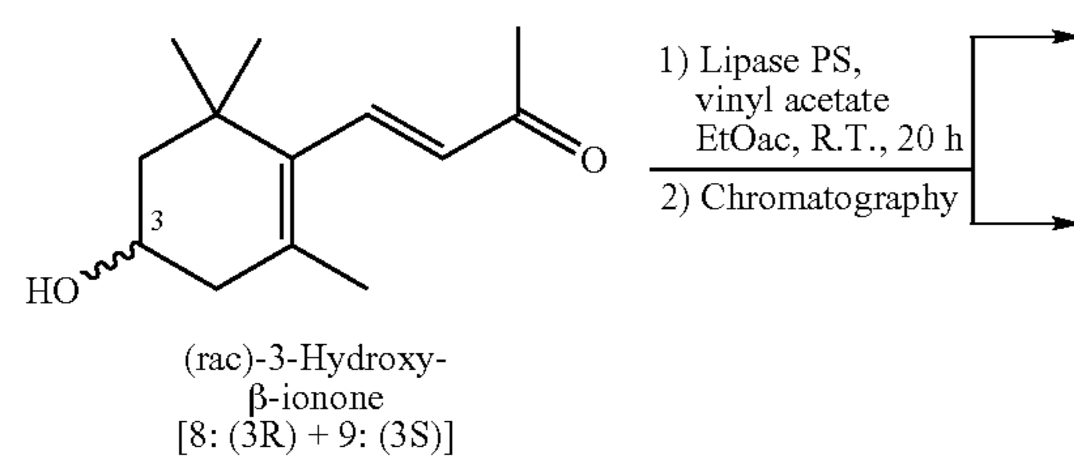
Scheme 8. Separation of (3R)-3-hydroxy- \beta -ionone (8) from its 3S-isomer (9) by enzyme-mediated acylation.*
