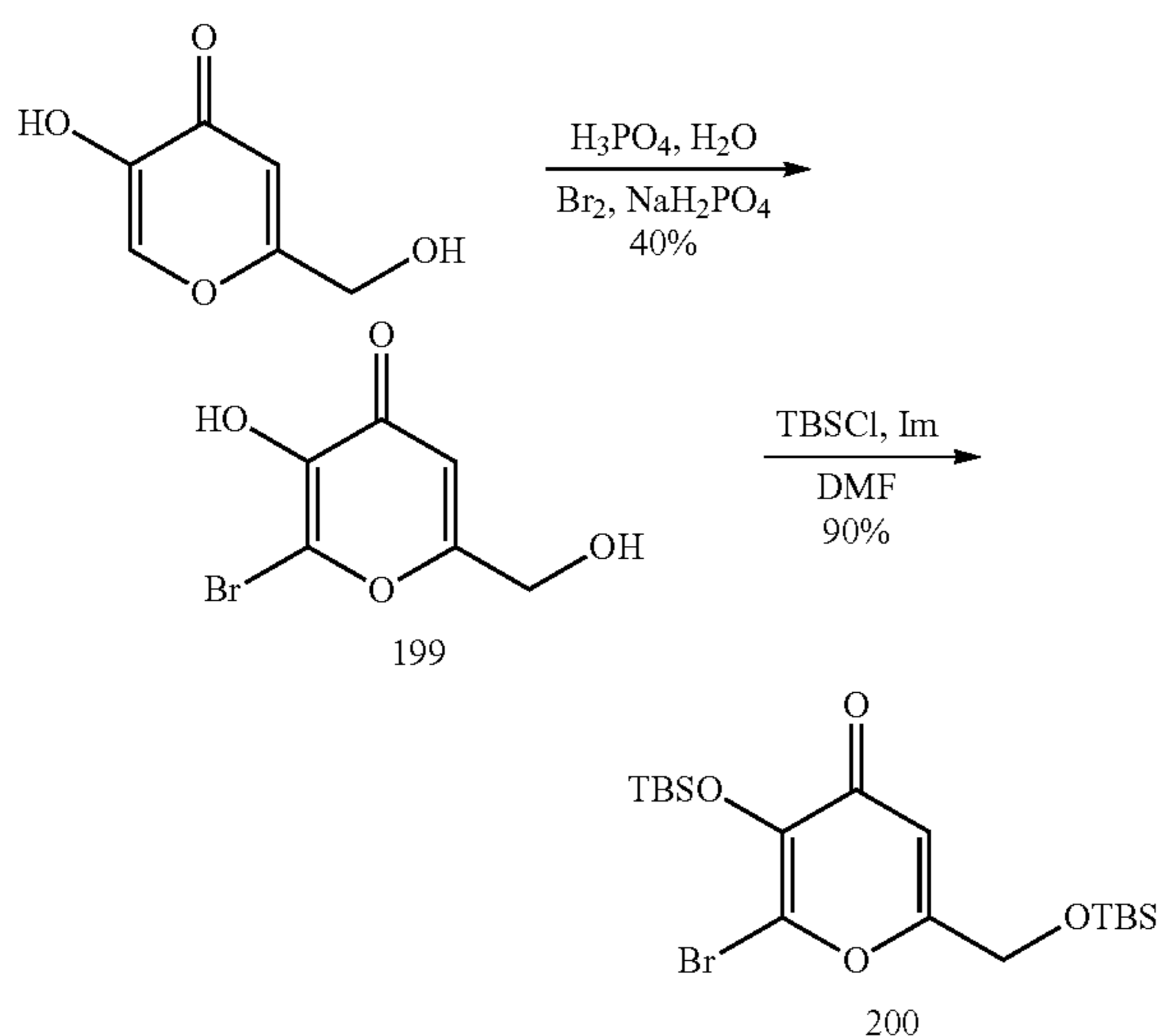
Scheme 4 Bromination and protection of kojic acid.
