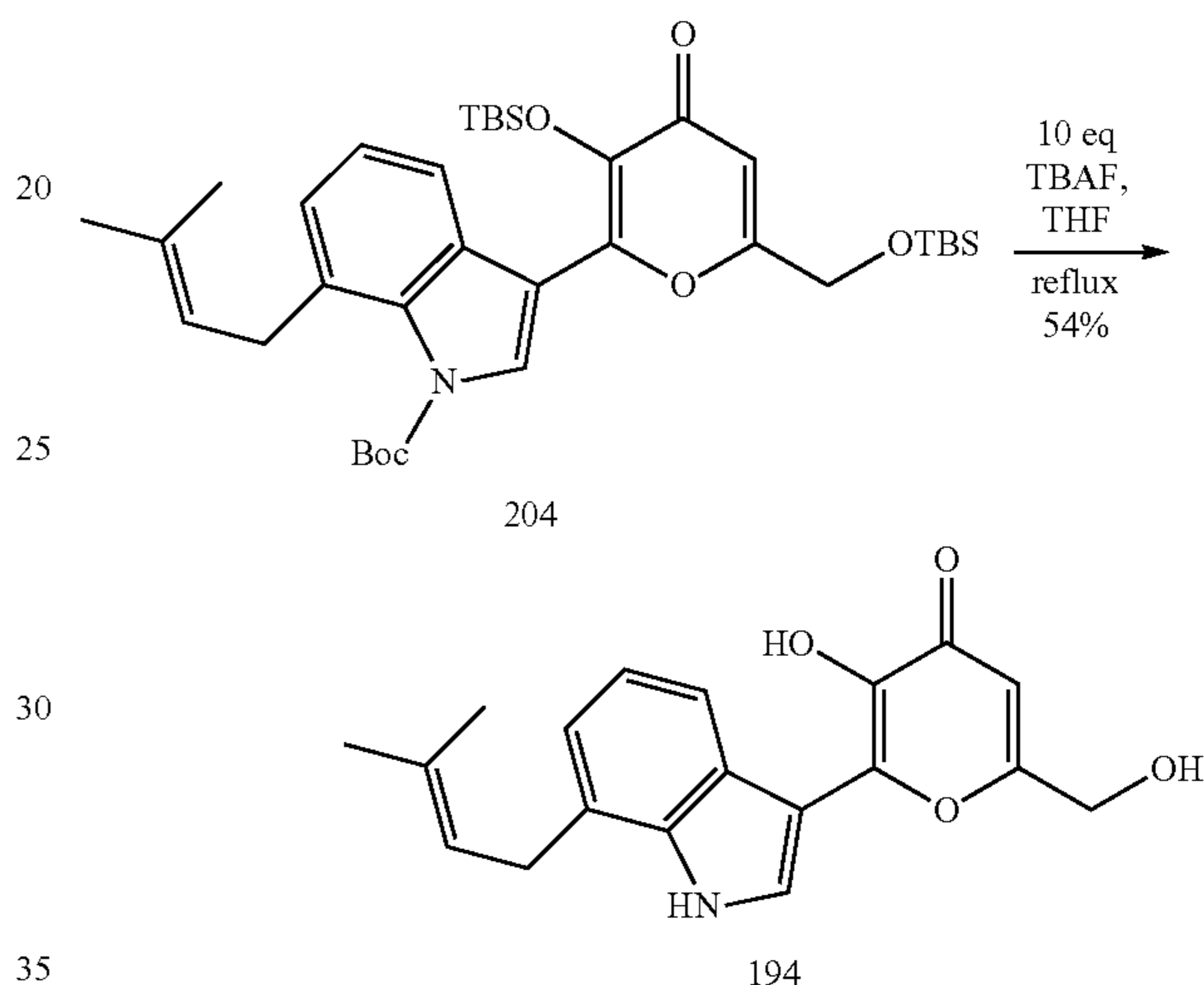
Scheme 8. Deprotection of Boc group and TBS ether by TBAF.
