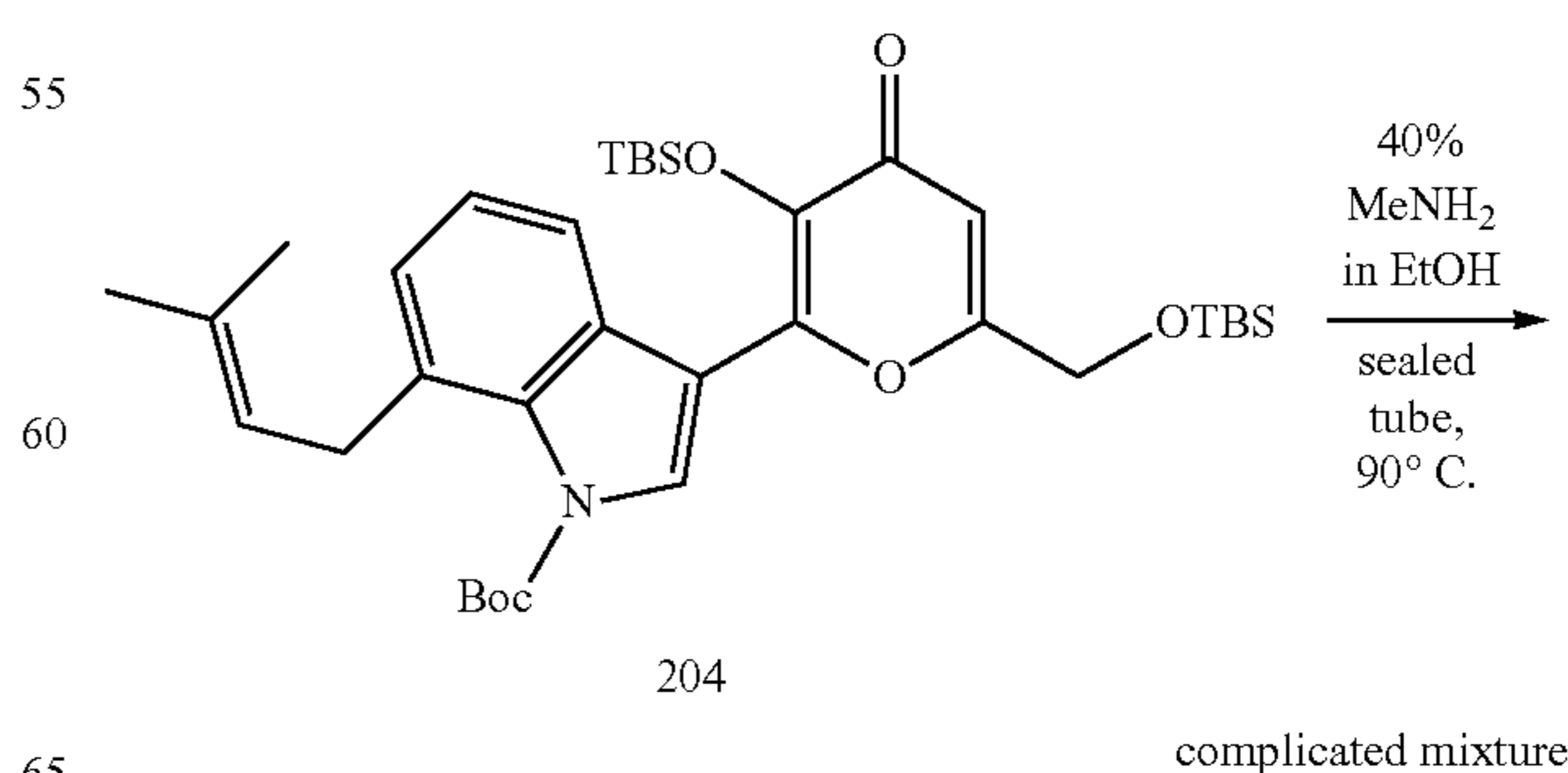
Scheme 9. Unsuccessful conversion of 204 to its pyridone.
