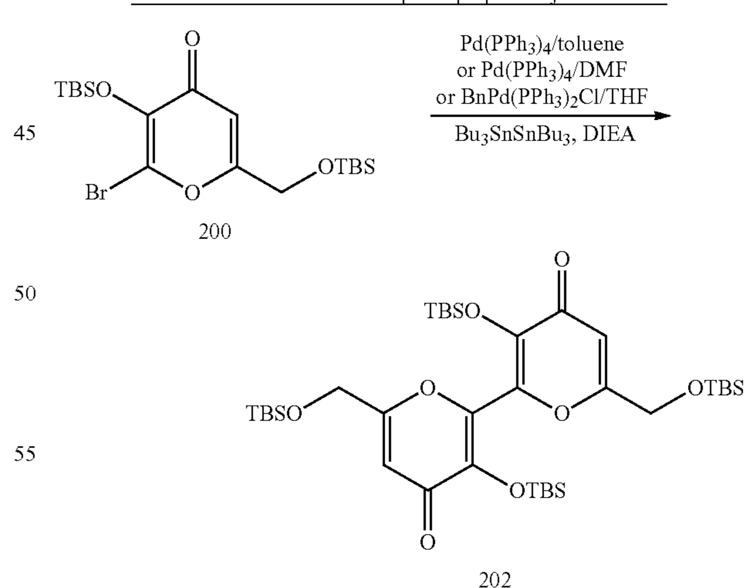
Scheme 6 Unsuccessful attempts to prepare kojic-stannane.
