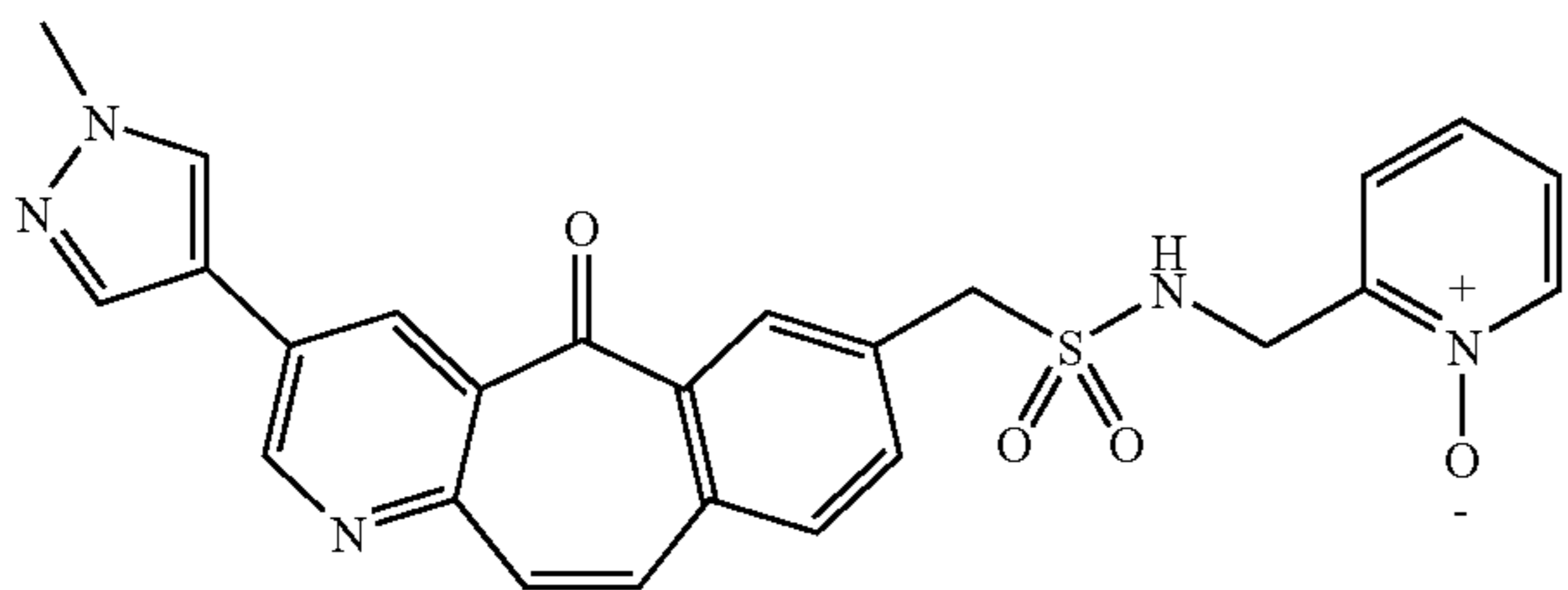
1-[3-(1-methyl-1H-pyrazol-4-yl)-5-oxo-5H-benzo[4,5]cyclohepta[1,2-b]pyridin-7-yl]-N-[(1-oxidopyridin-2-yl)methyl]methanesulfonamide (Compound 10-1)
