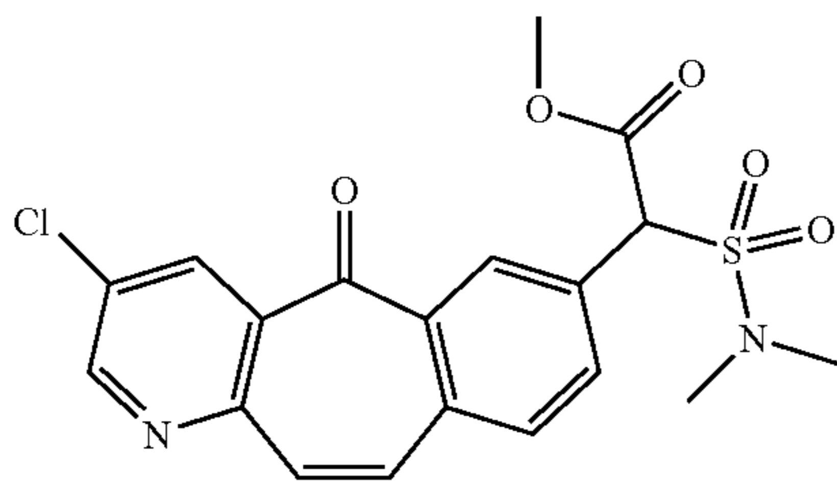
Step 2: Methyl (3-chloro-5-oxo-5H-benzo[4,5]cyclohepta[1,2-b]pyridin-7-yl)[(dimethylamino)sulfonyl]acetate (Compound 2-2)
