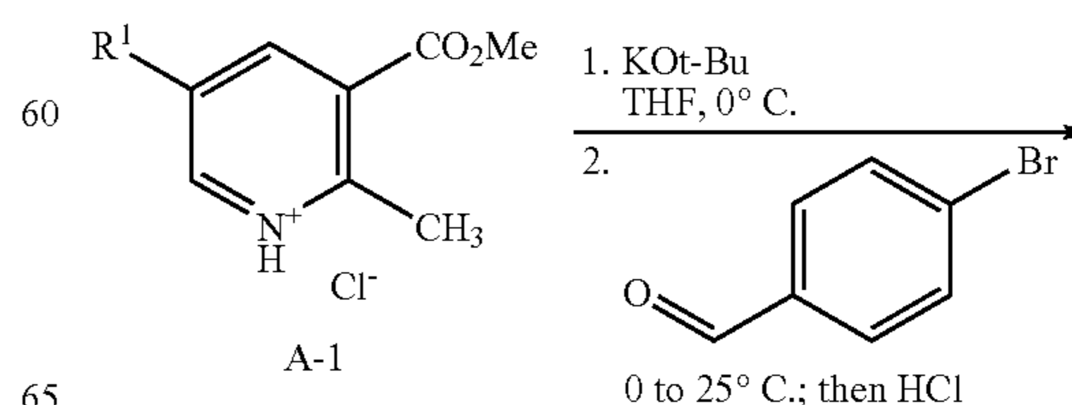
SCHEME A
