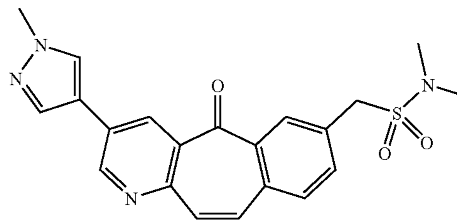
Step 4: N,N-Dimethyl-1-[3-(1-methyl-1H-pyrazol-4-yl)-5-oxo-5H-benzo[4,5]cyclohepta[1,2-b]pyridin-7-yl]methanesulfonamide (Compound 2-4)
