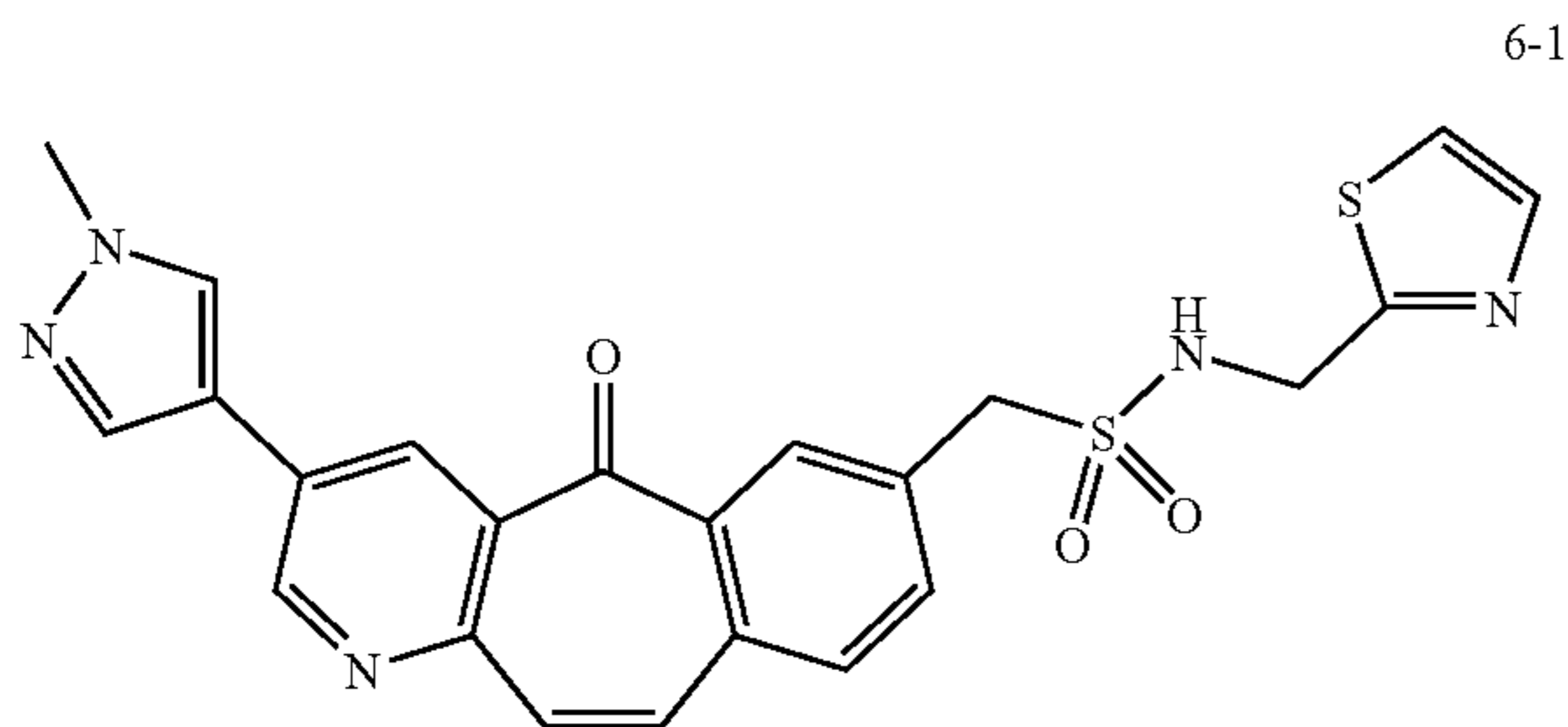
1-[3-(1-methyl-1H-pyrazol-4-yl)-5-oxo-5H-benzo[4,5]cyclohepta[1,2-b]pyridin-7-yl]-N-(1,3-thiazol-2-ylmethyl)methanesulfonamide (Compound 6-1)
