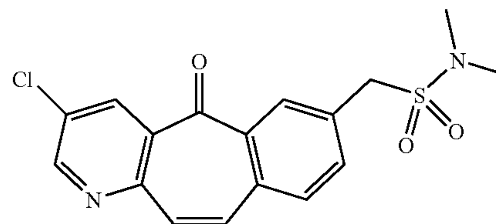
Step 3: 1-(3-Chloro-5-oxo-5H-benzo[4,5]cyclohepta[1,2-b]pyridin-7-yl)-N,N-dimethylmethanesulfonamide (Compound 2-3)
