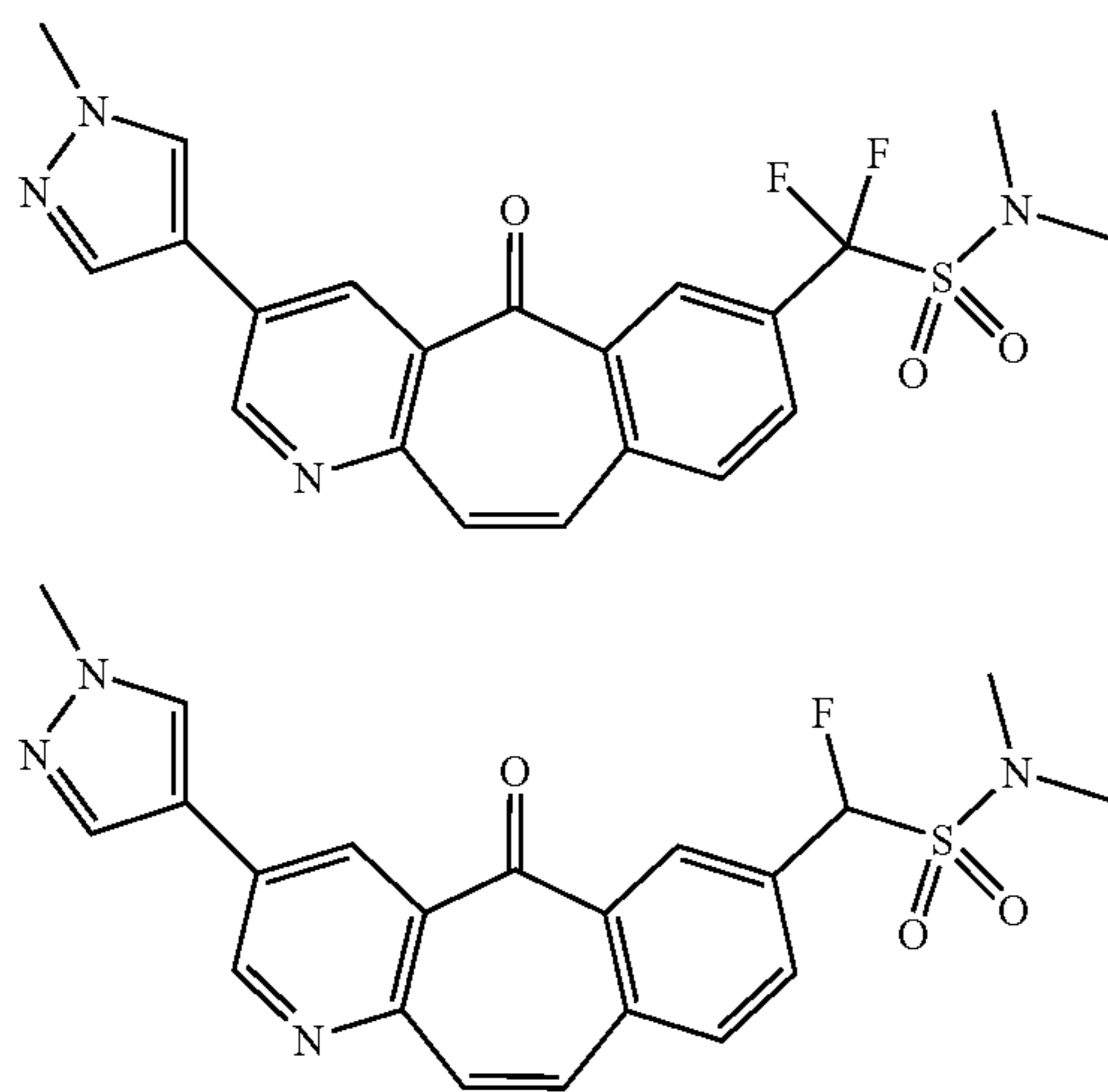
1,1-Difluoro-N,N-dimethyl-1-[3-(1-methyl-1H-pyrazol-4-yl)-5-oxo-5H-benzo[4,5]cyclohepta[1,2-b]pyridin-7-yl]methanesulfonamide (Compound 4-1) and 1-Fluoro-N,N-dimethyl-1-[3-(1-methyl-1H-pyrazol-4-yl)-5-oxo-5H-benzo[4,5]cyclohepta[1,2-b]pyridin-7-yl]methanesulfonamide (Compound 4-2)
