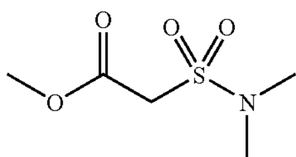
Step 1: Methyl [(dimethylamino)sulfonyl]acetate (Compound 2-1)
