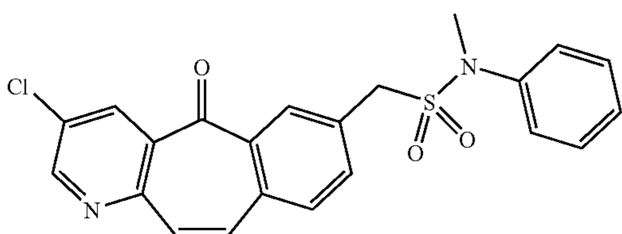
Step 3: 1-(3-Chloro-5-oxo-5H-benzo[4,5]cyclohepta[1,2-b]pyridin-7-yl)-N-methyl-N-phenylmethanesulfonamide (Compound 5-3)
