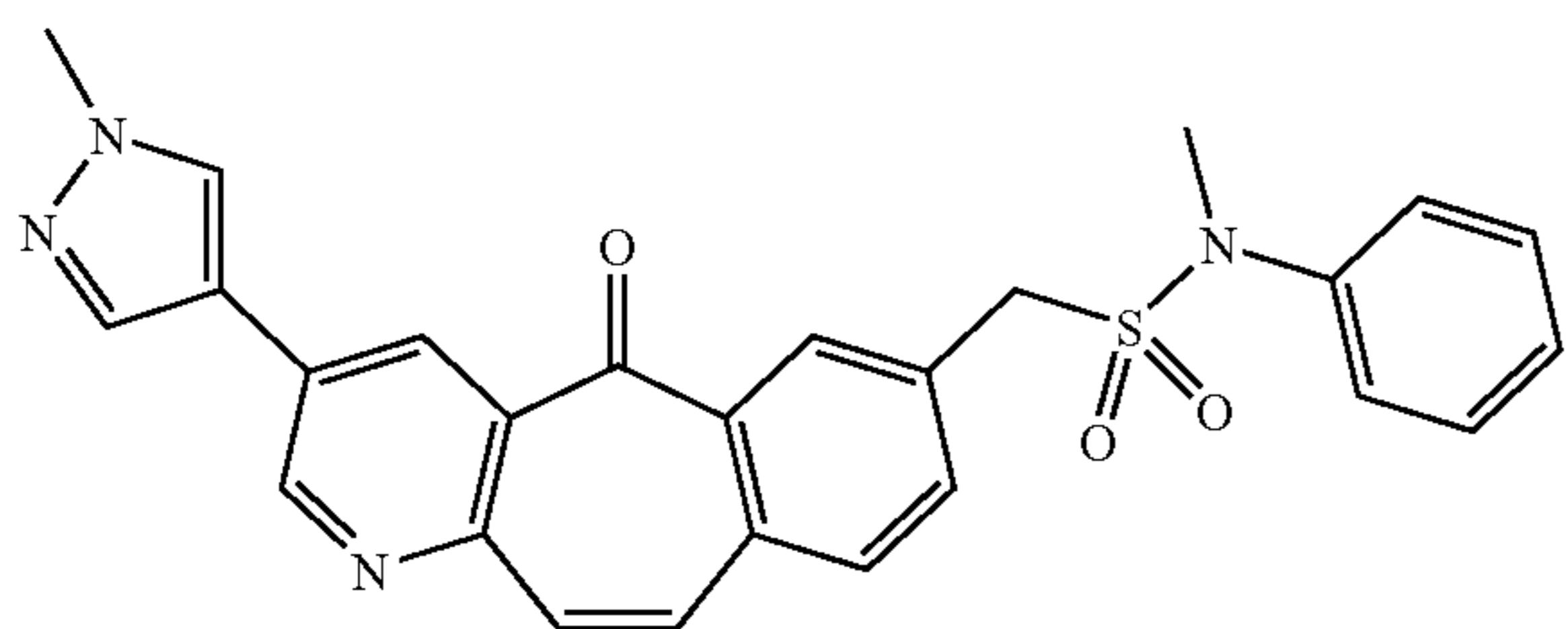
Step 4: N-methyl-1-[3-(1-methyl-1H-pyrazol-4-yl)-5-oxo-5H-benzo[4,5]cyclohepta[1,2-b]pyridin-7-yl]-N-phenylmethanesulfonamide (Compound 5-4)
