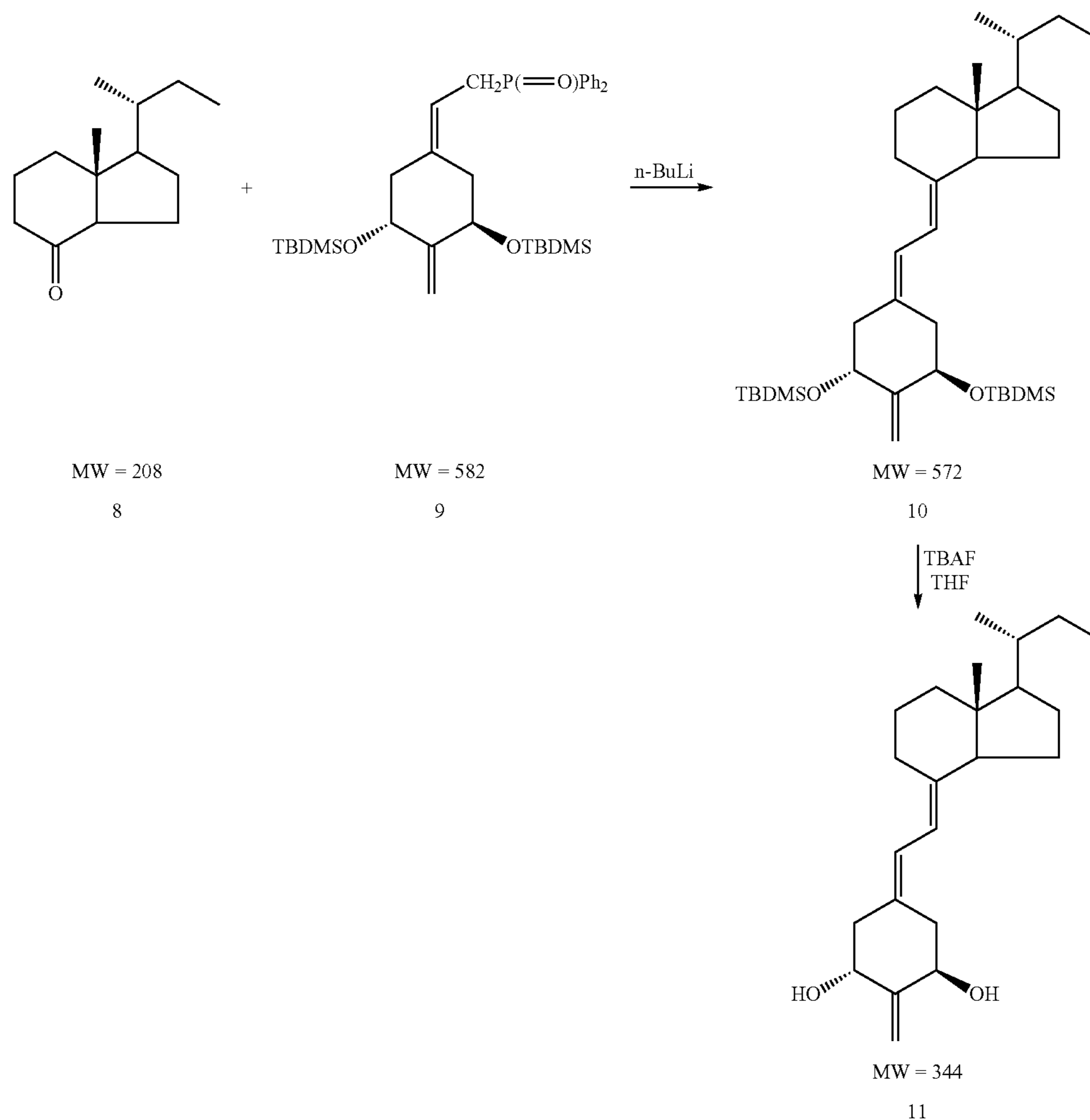
Scheme IIB
