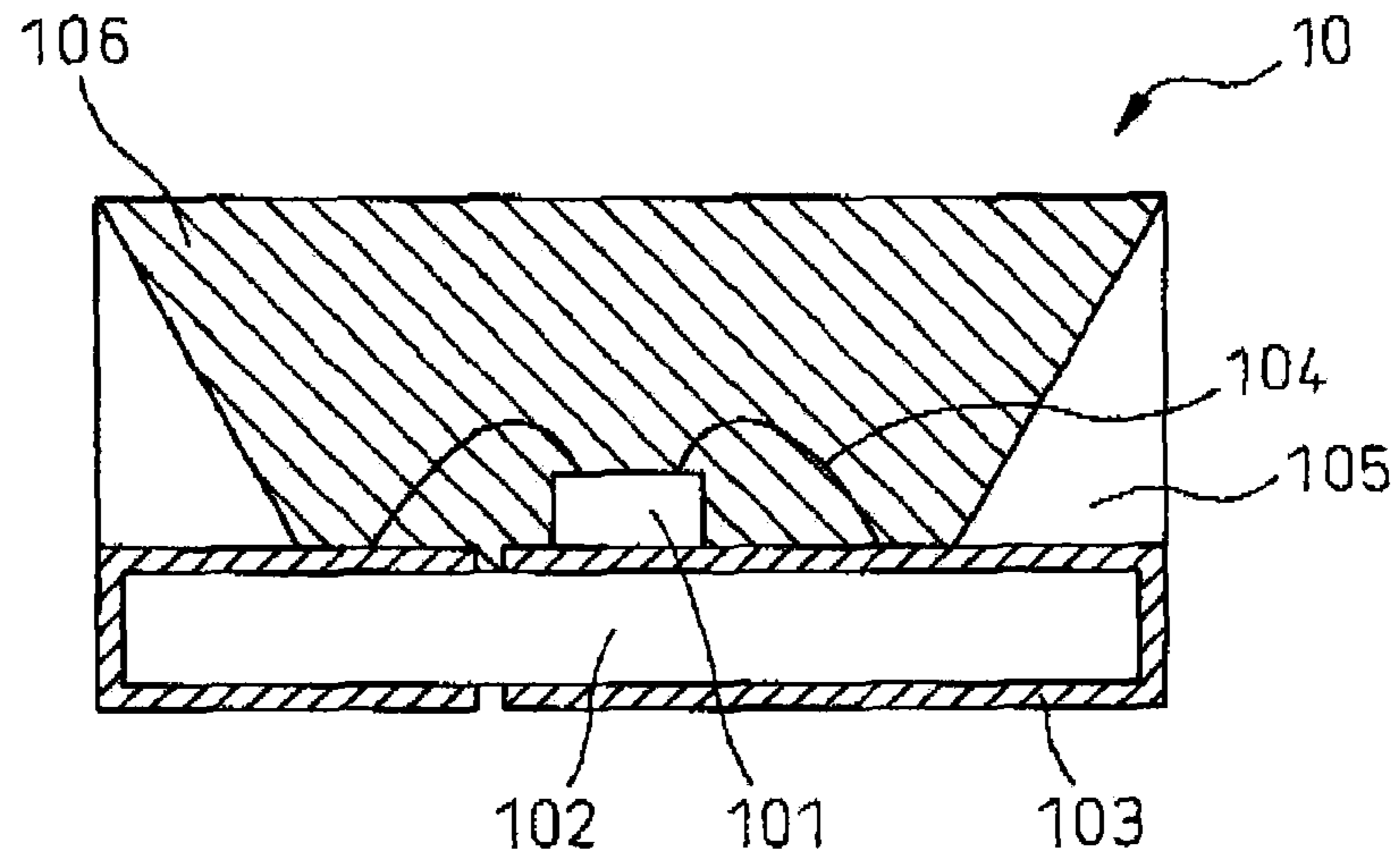
Fig.18 PRIOR ART
