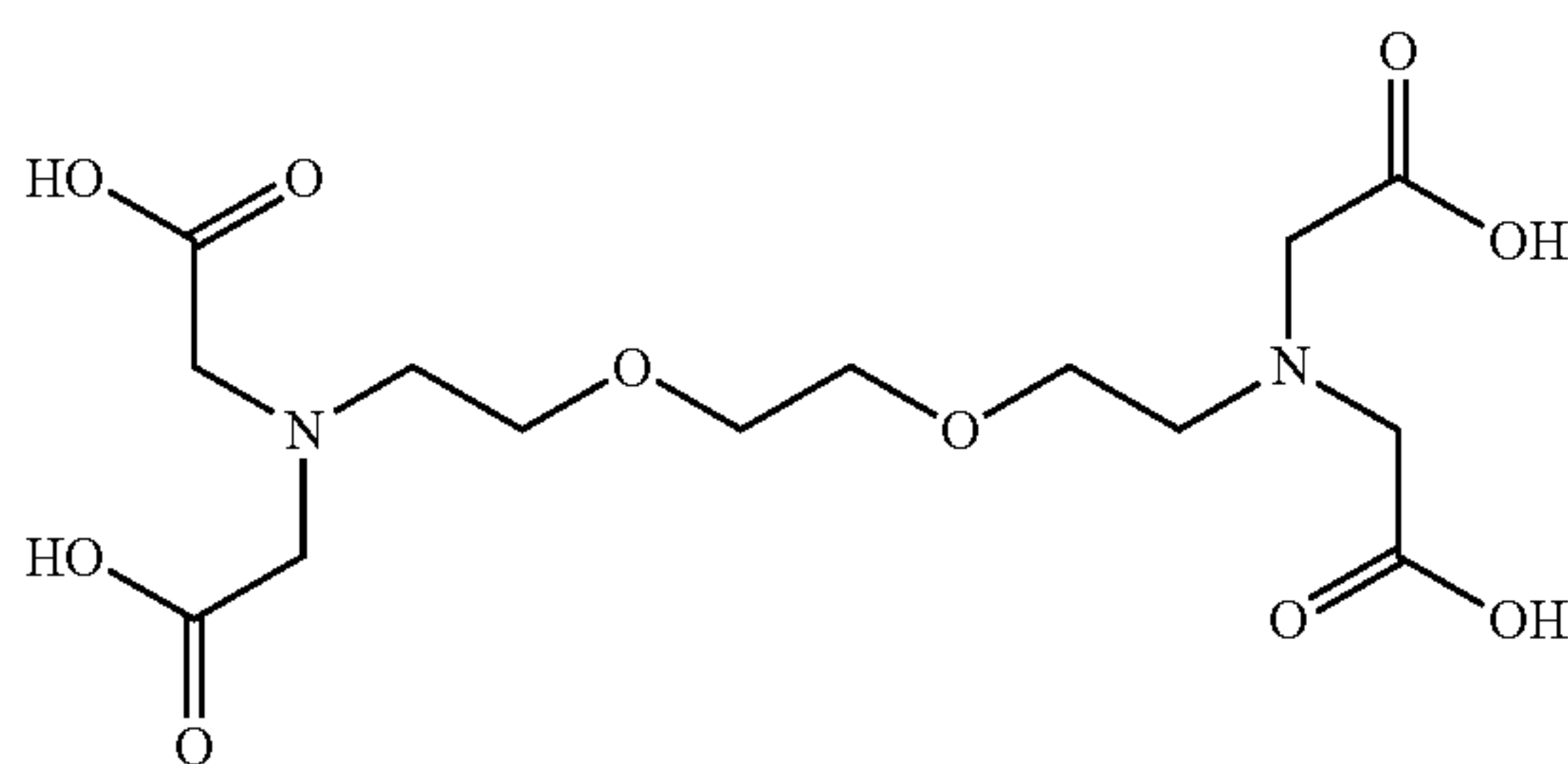
EGTA Formula
