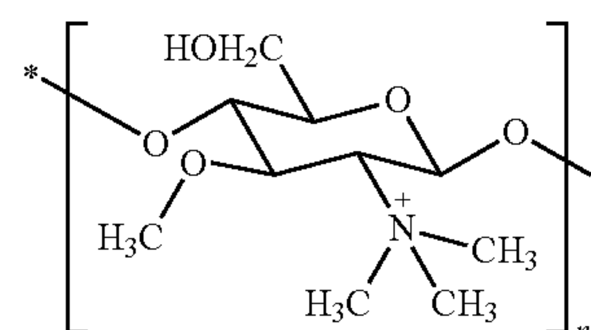
Chitosan
