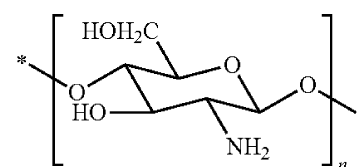
Chitosan
