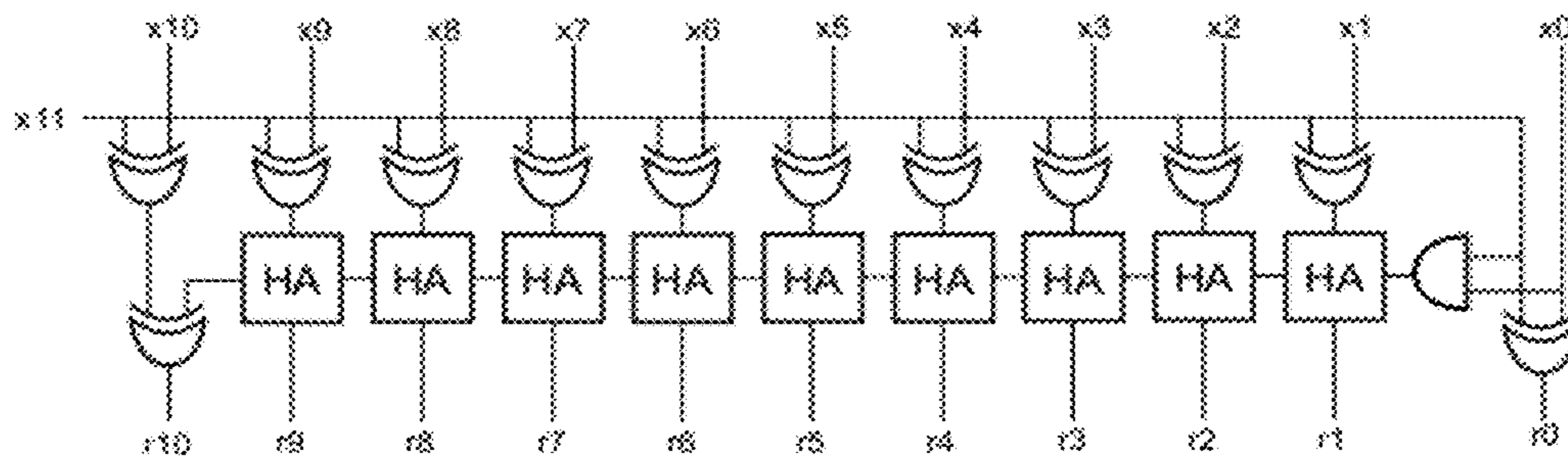
12-Bit Modulus
