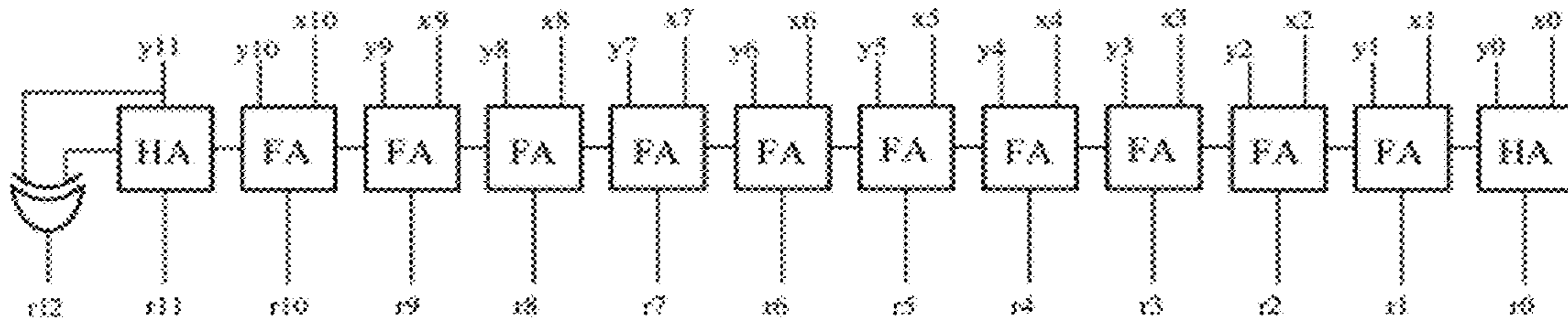
Unsigned/Signed Add
