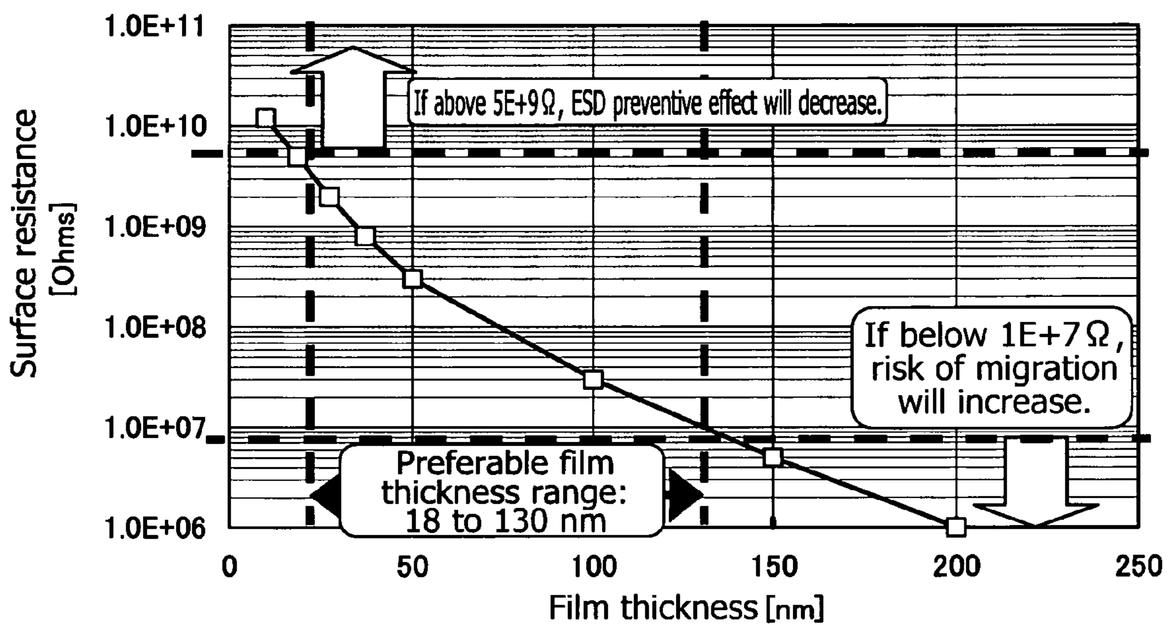
Film thickness vs. wiring-substrate surface resistance
