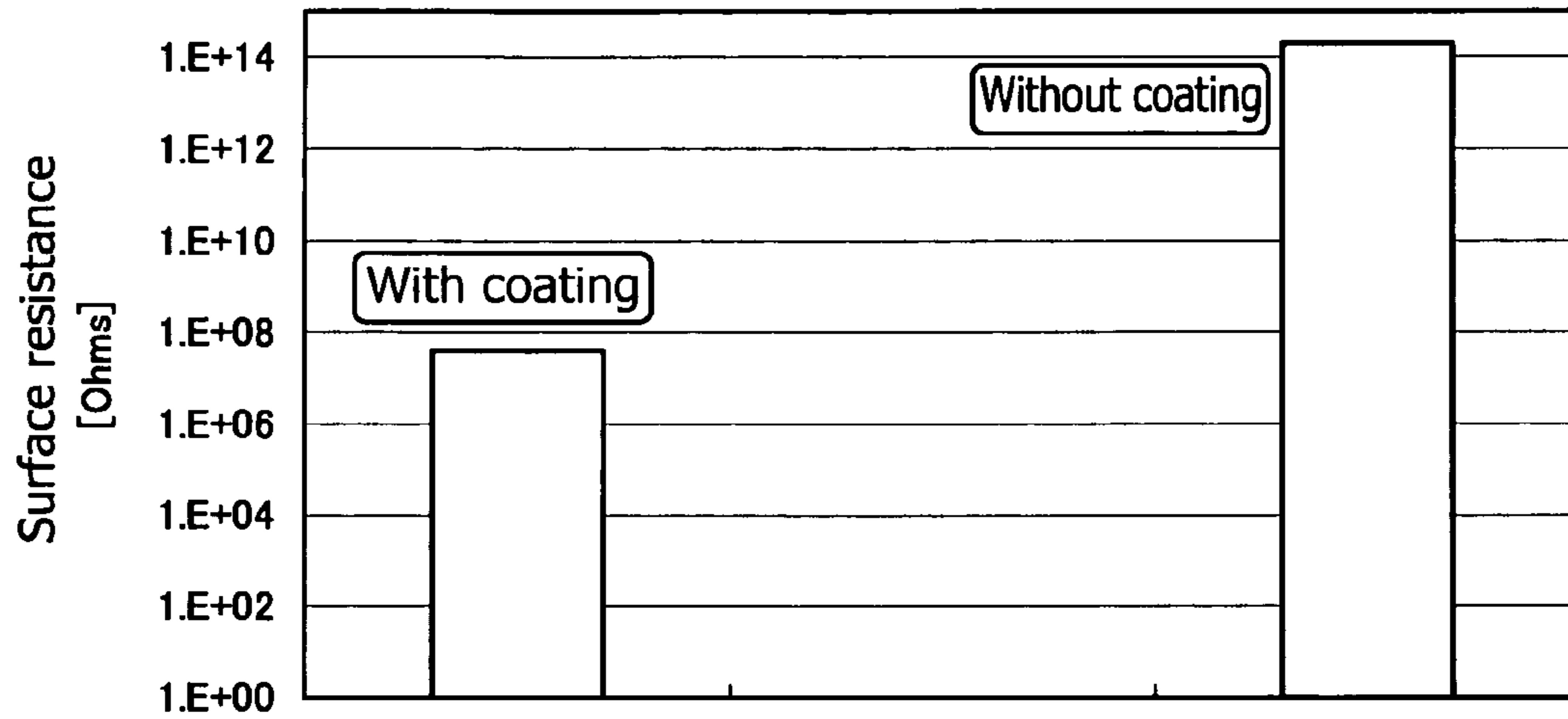
Surface resistance with/without conductive polymer coating
