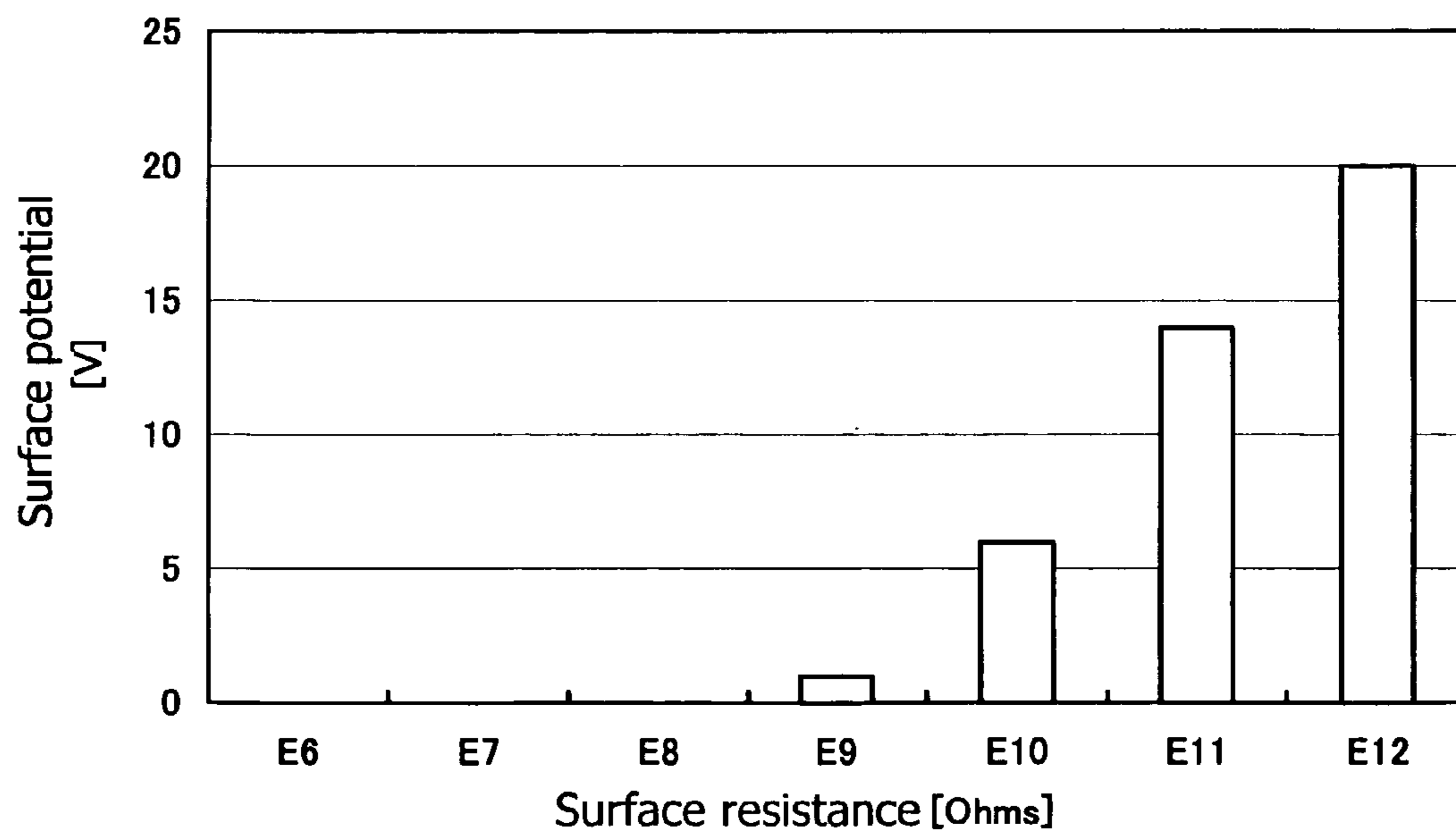
Surface resistance vs. surface potential
