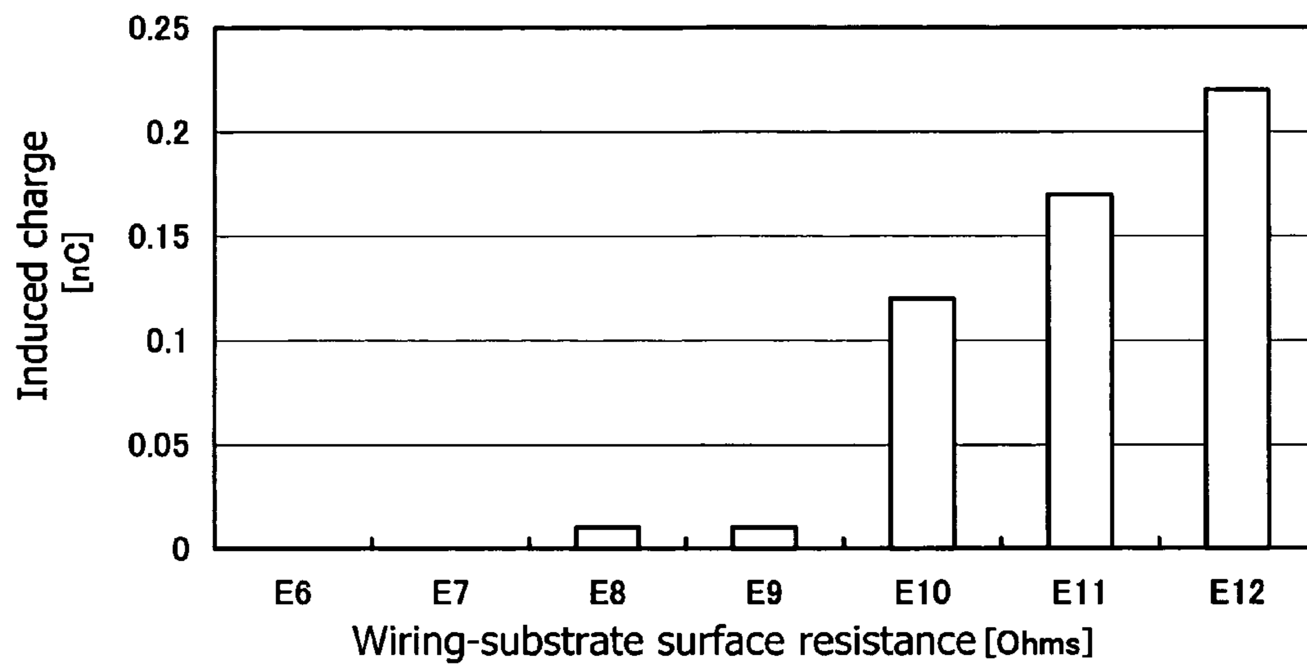
Wiring-substrate surface resistance and induced charge
