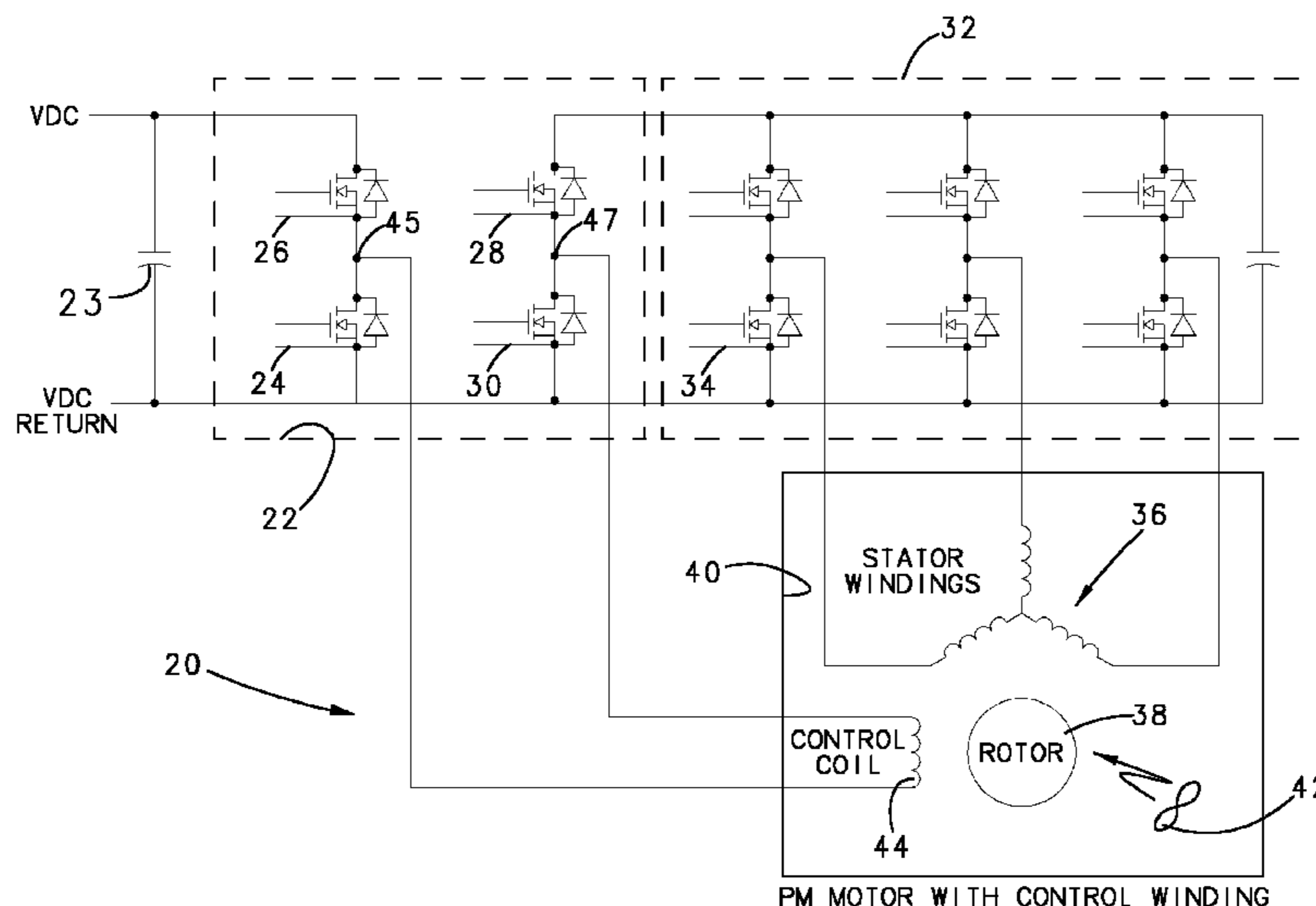
PM MOTOR WITH CONTROL WINDING
