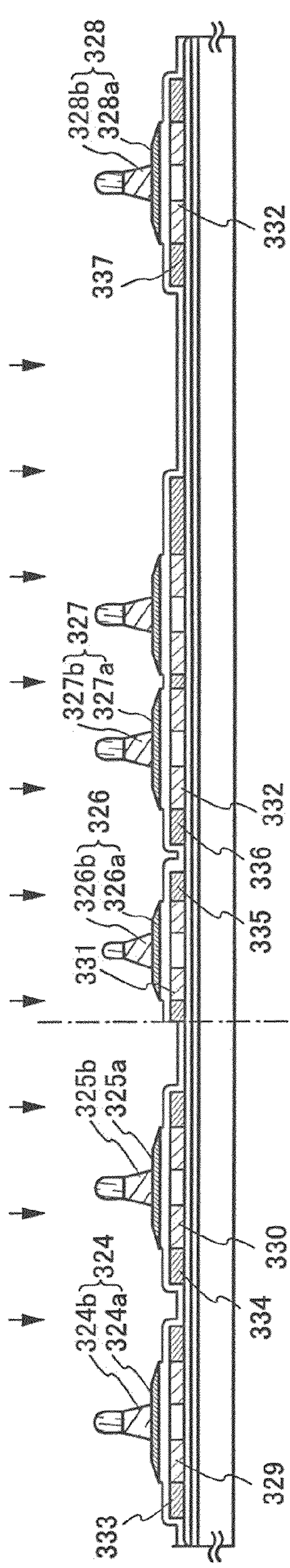
Fig. 22A second doping process
