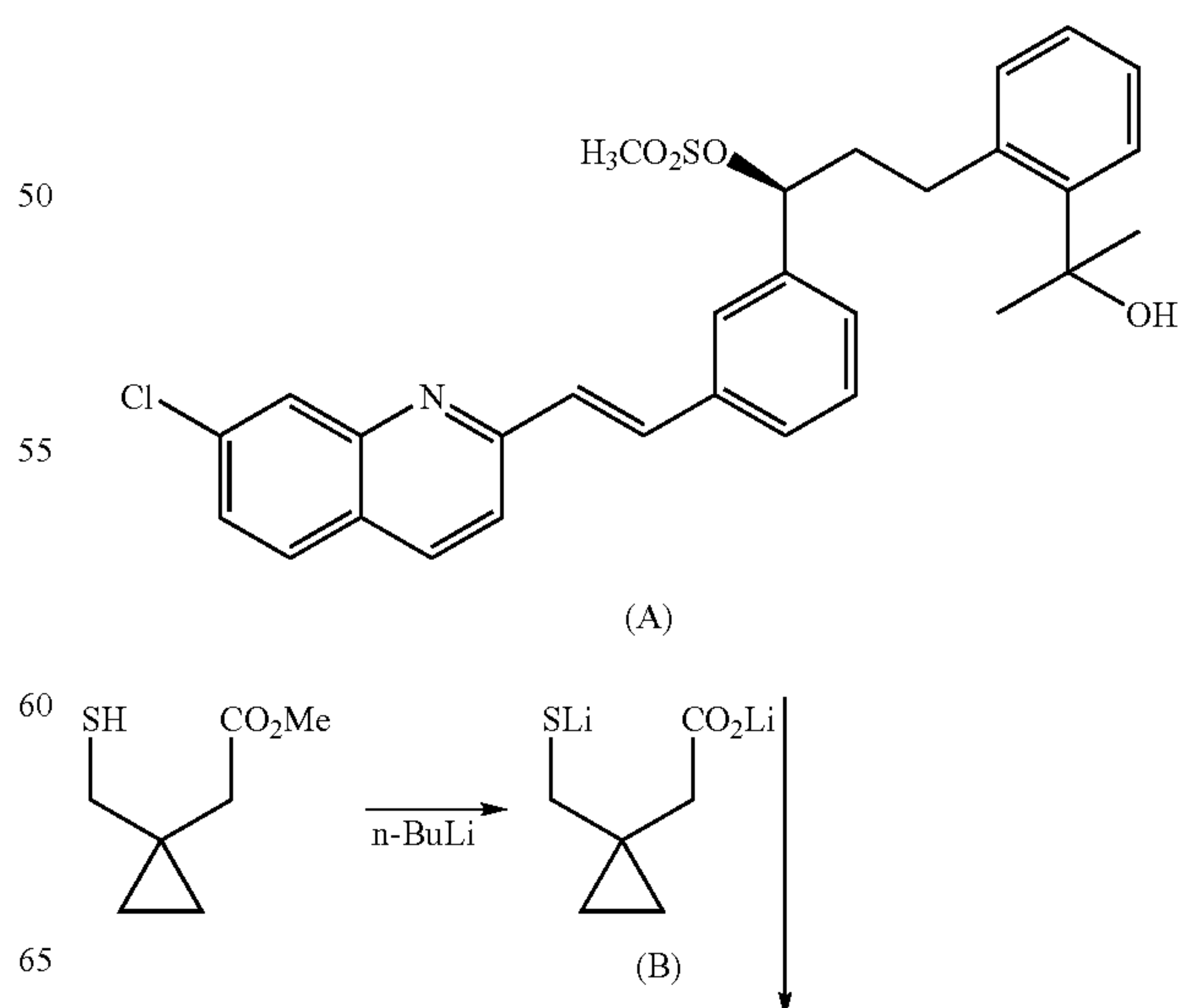
Reaction Scheme 2
