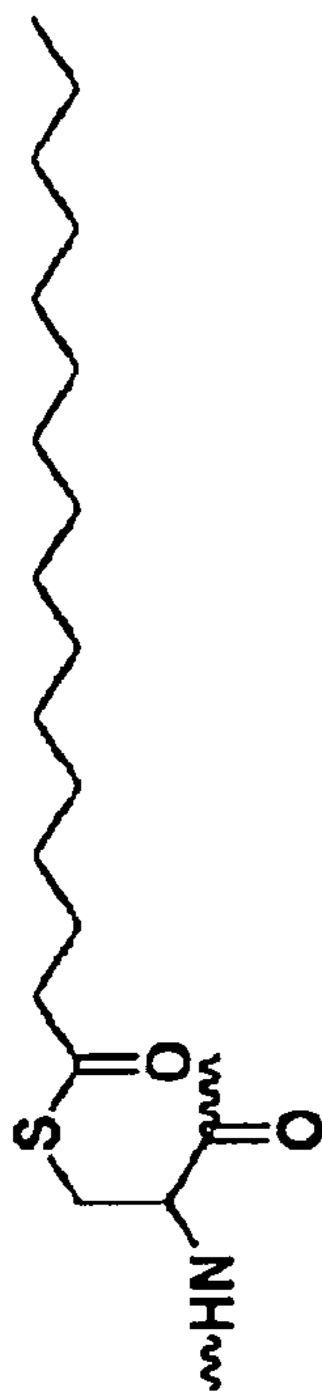
palmitoylcysteine (3)
