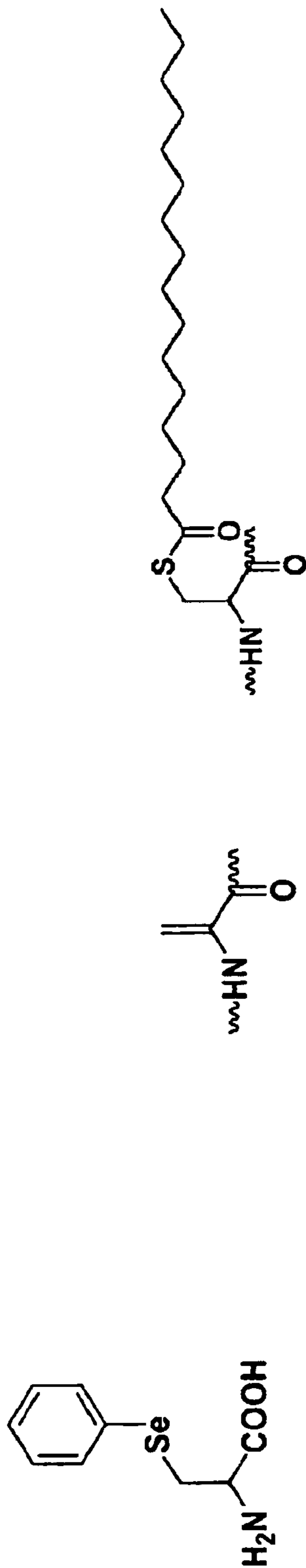
palmitoylcysteine (3)
