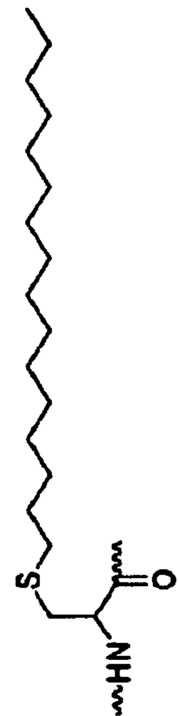
S-hexadecylcysteine (5)
