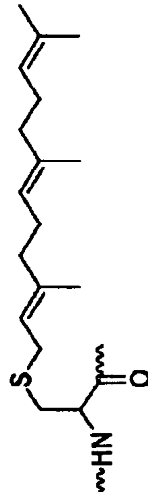
farnesylcysteine (4)
