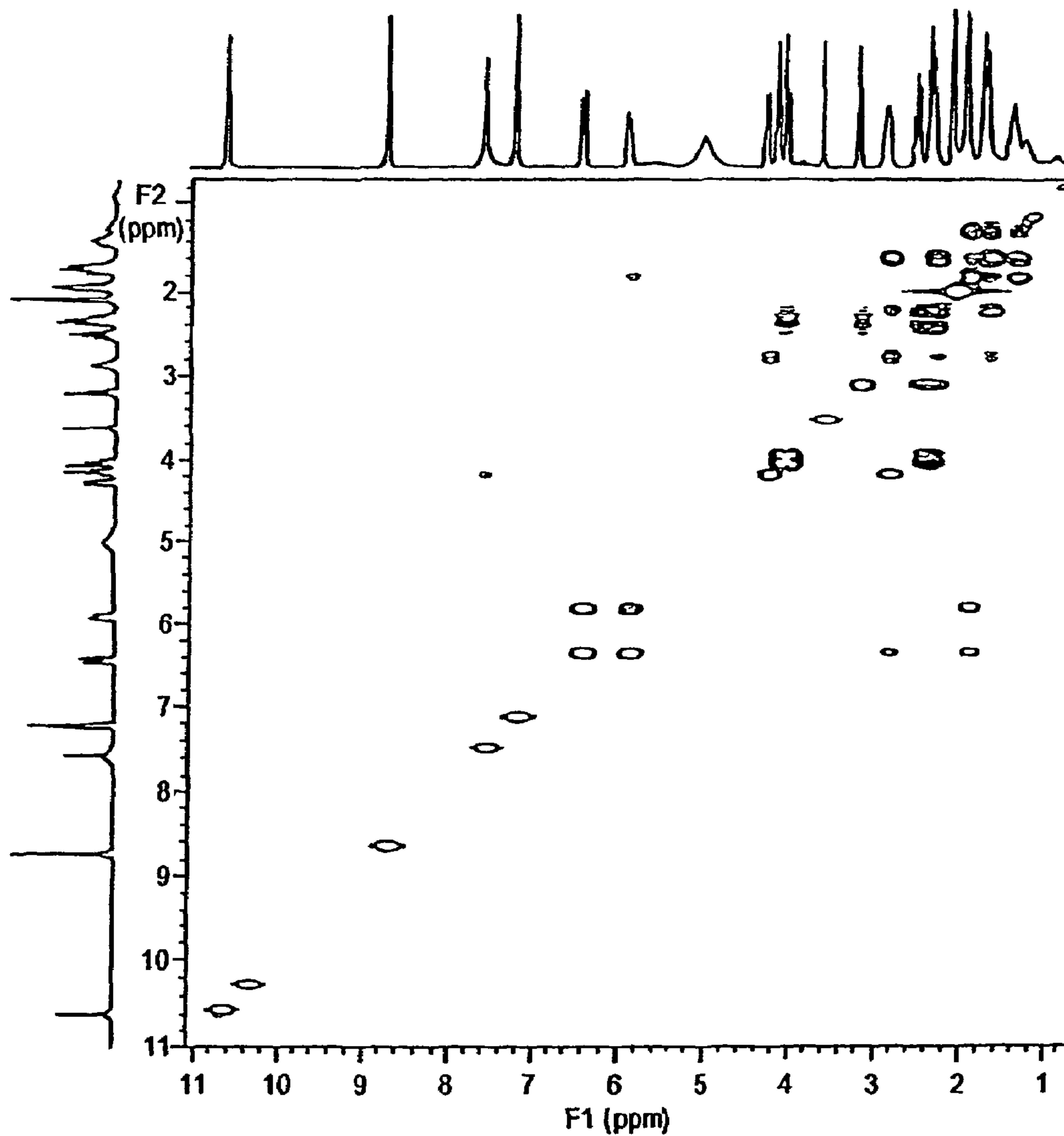
H,H-COSY of salinosporamide A (1), 300 MHz, d 5 -pyridine
