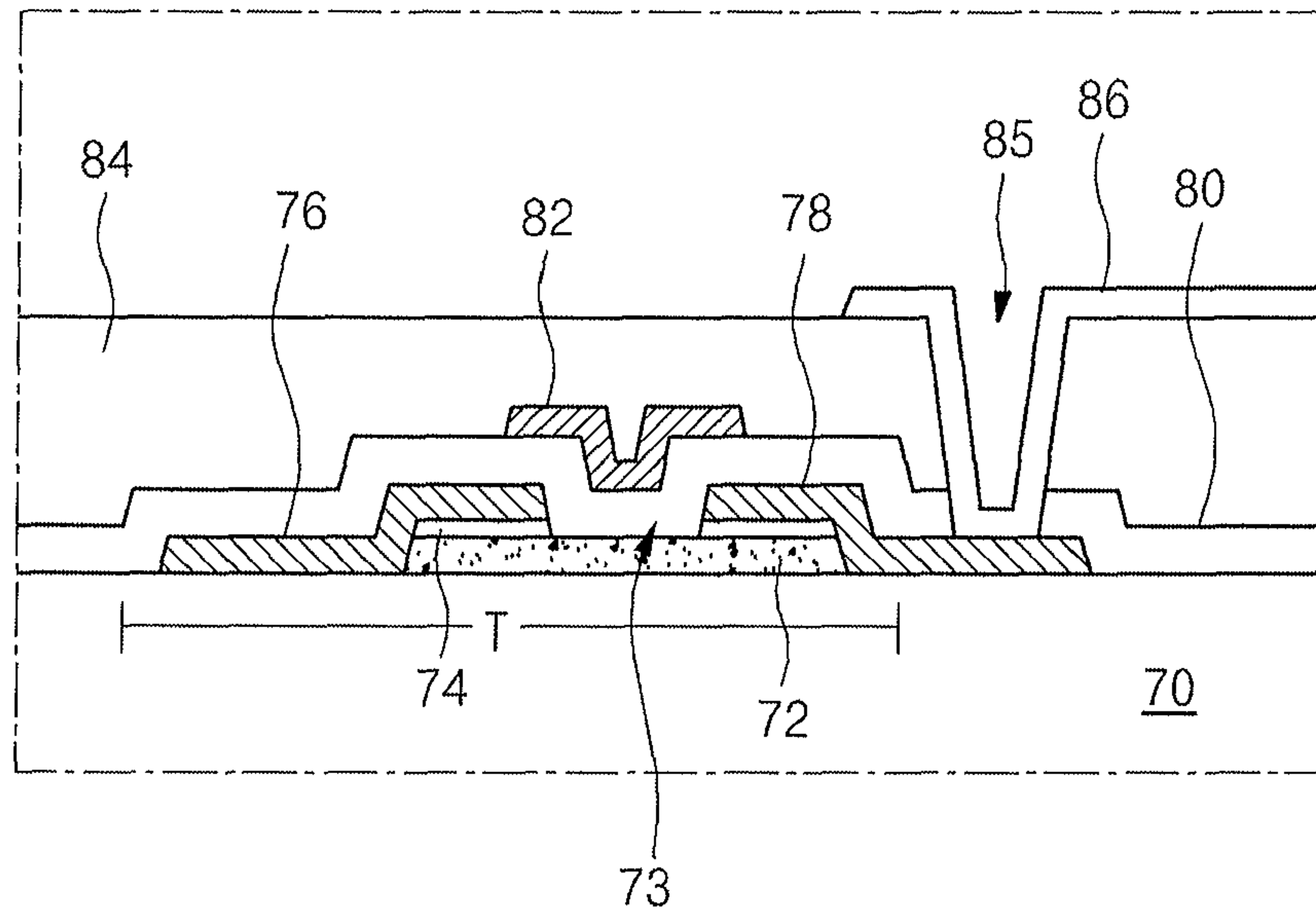
FIG. 4 (related art)
