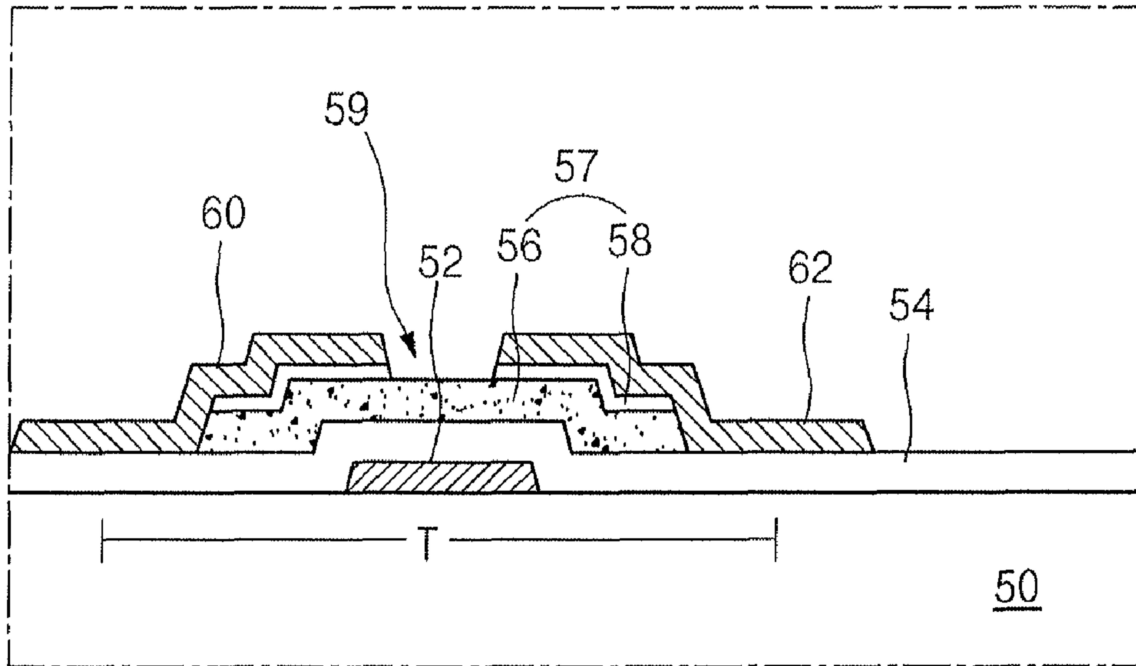
FIG. 3C (related art)
