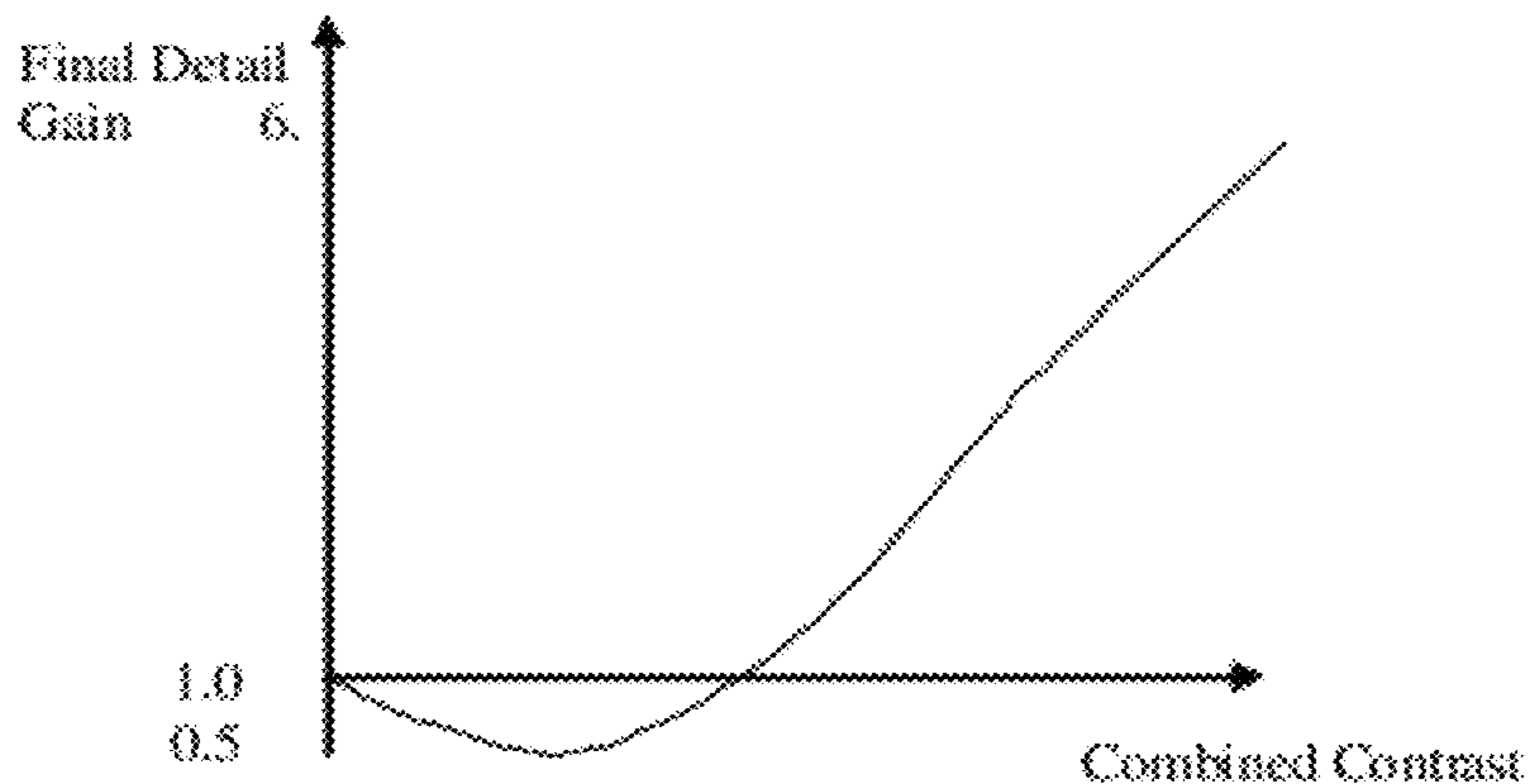
Fig. 6 (Combined Contrast to Watermark Gain Mapping Function)
