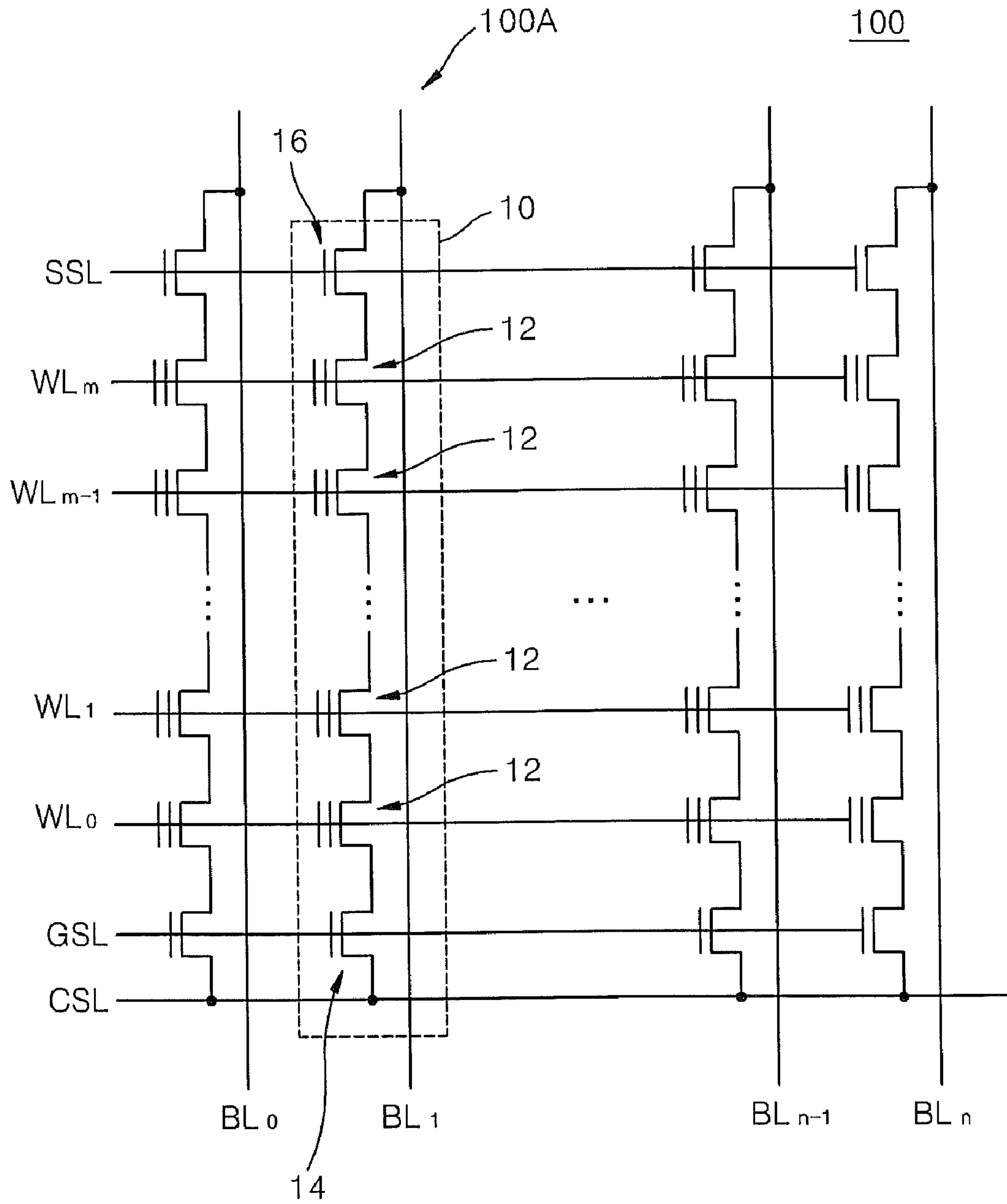
FIG. 2 (PRIOR ART)
