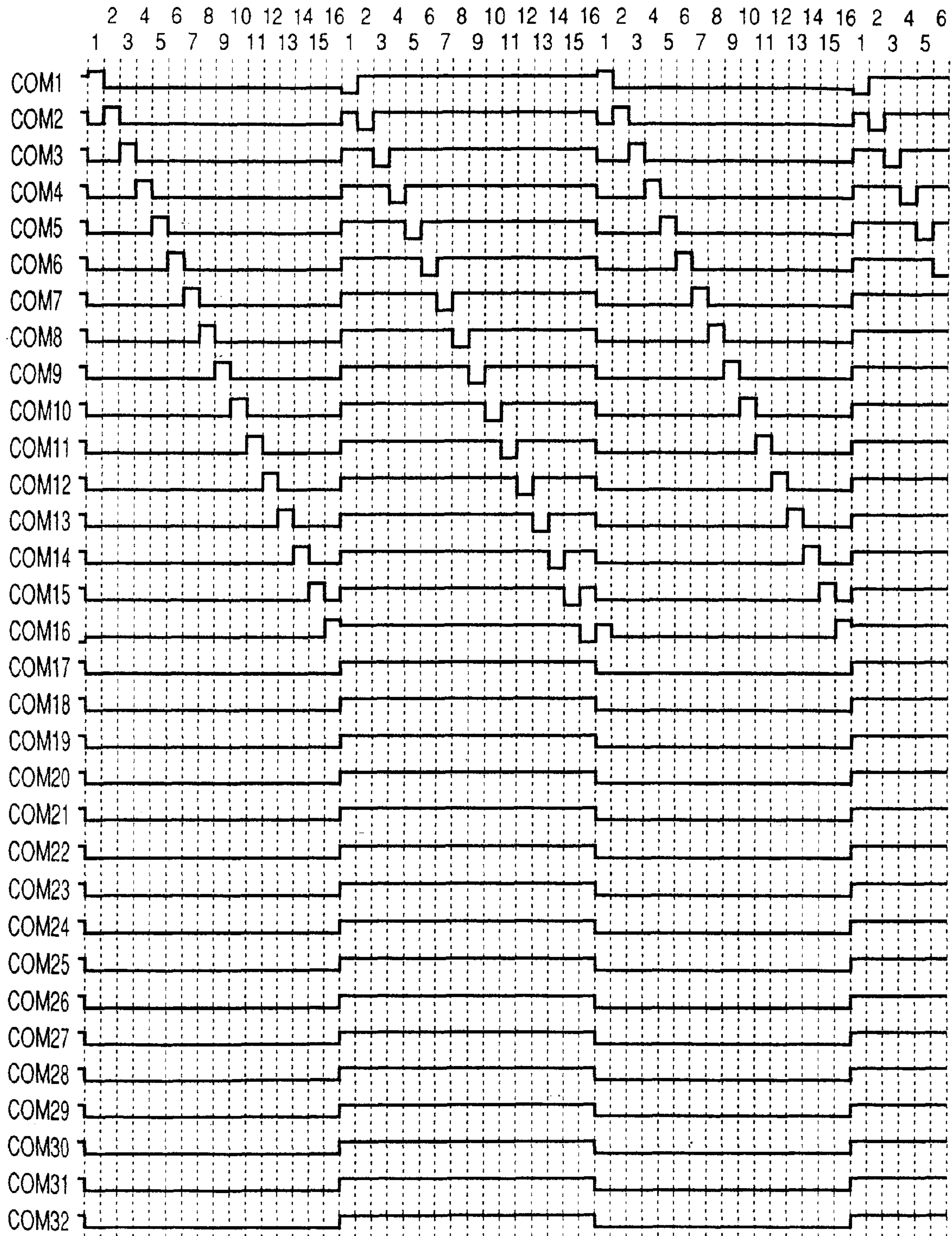
1/16 DUTY DRIVE (COM1~COM16)
