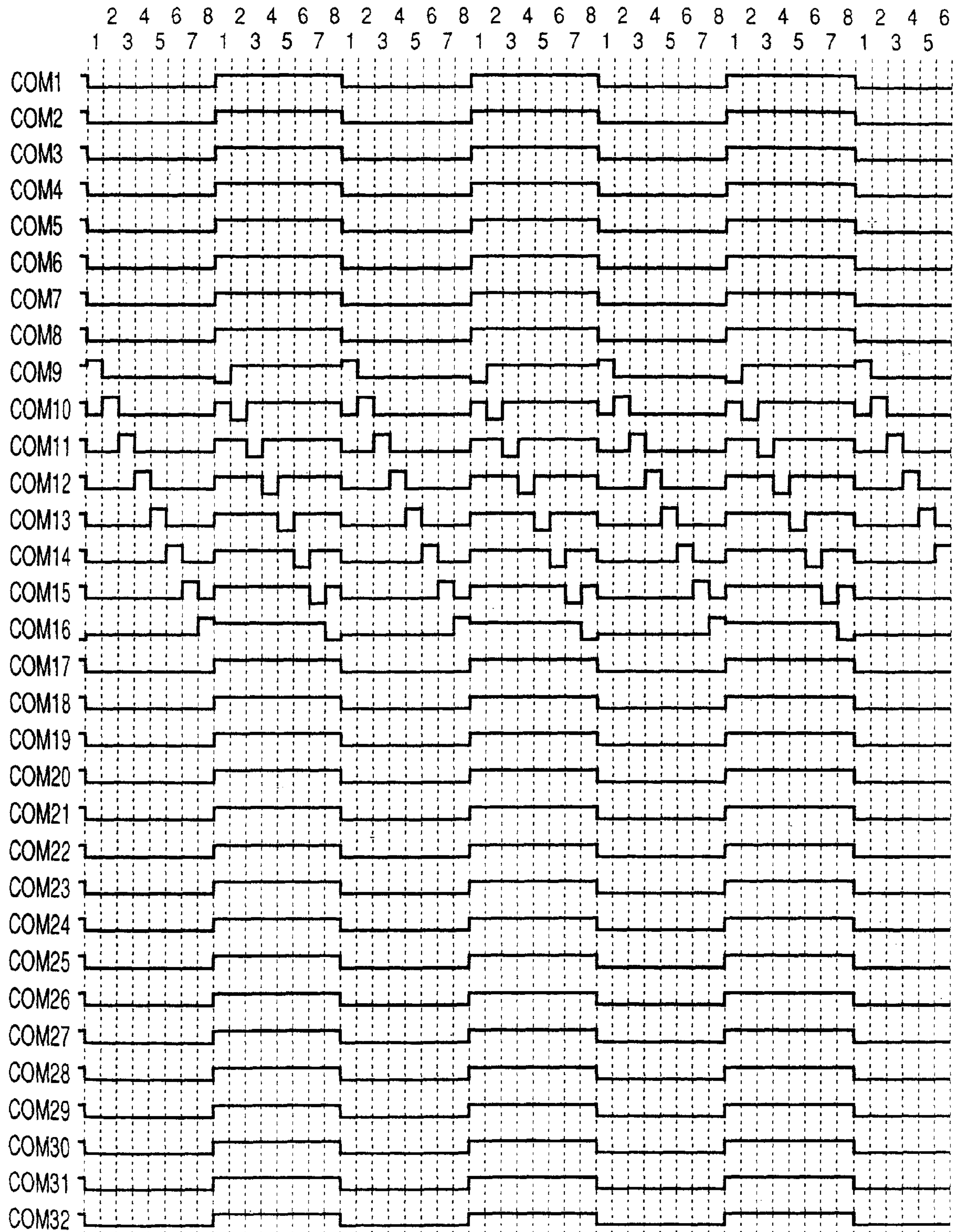
1/8 DUTY DRIVE (COM9~COM16)
