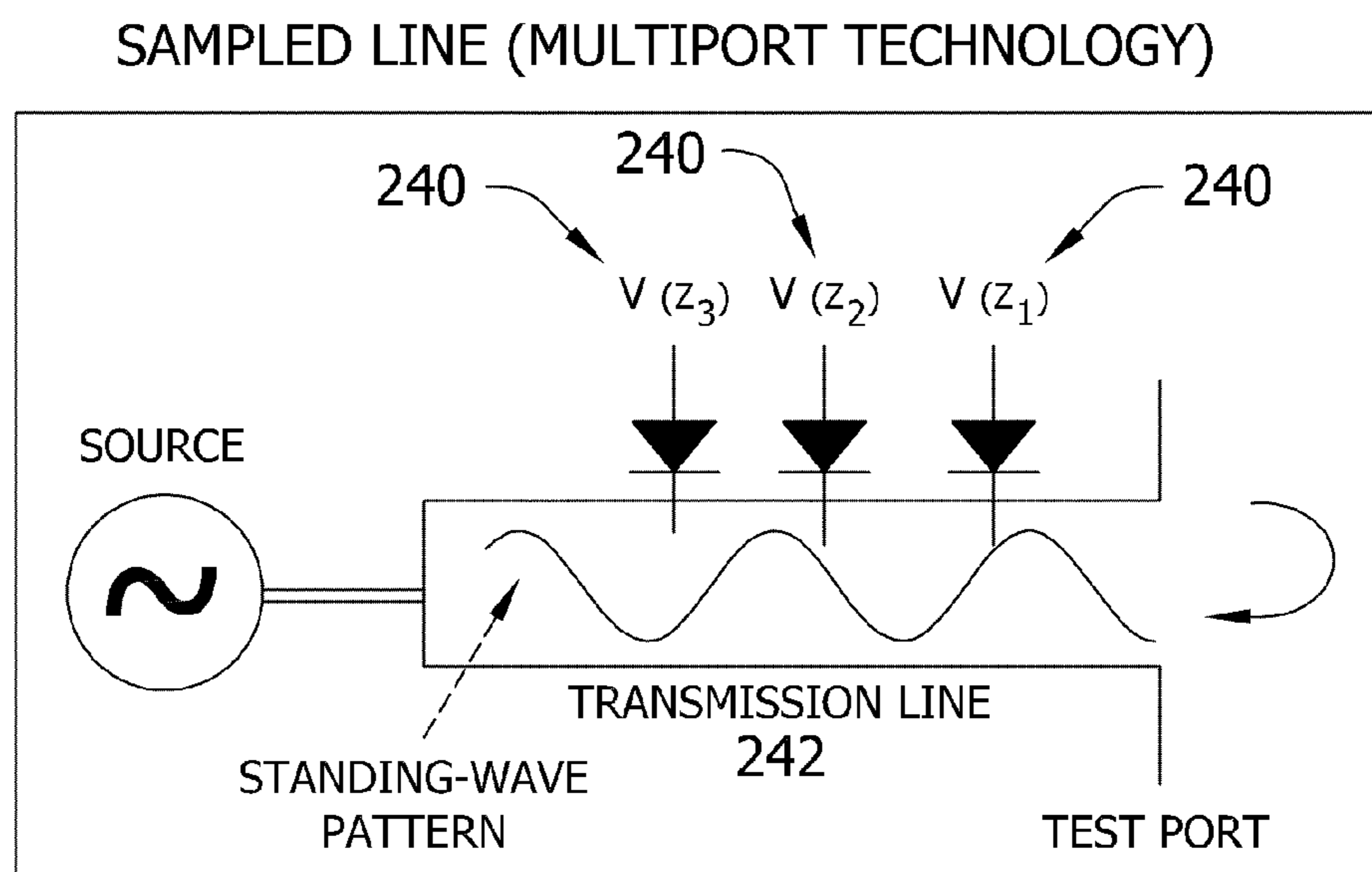
FIG. 2C PRIOR ART
