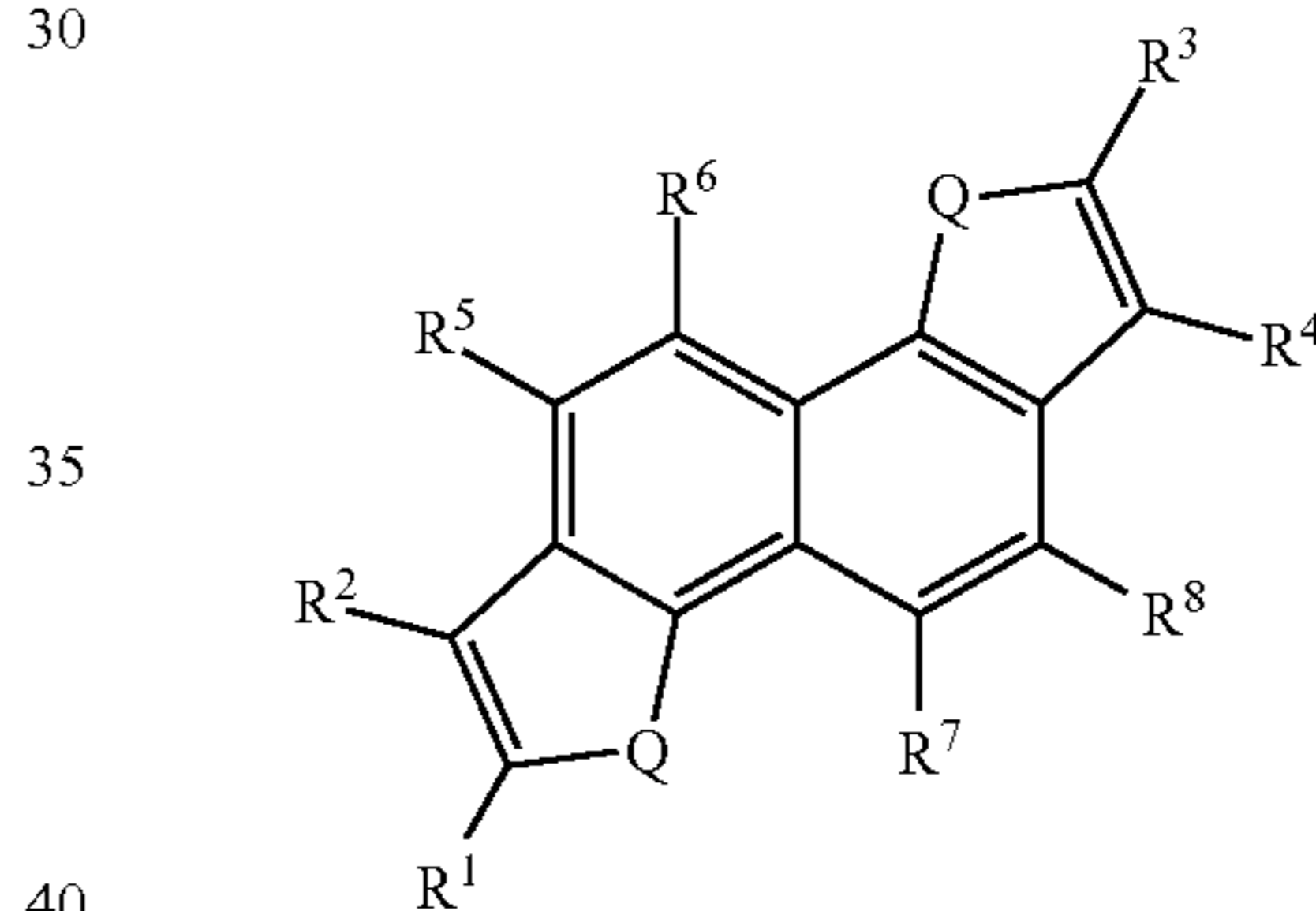
Compound 39
