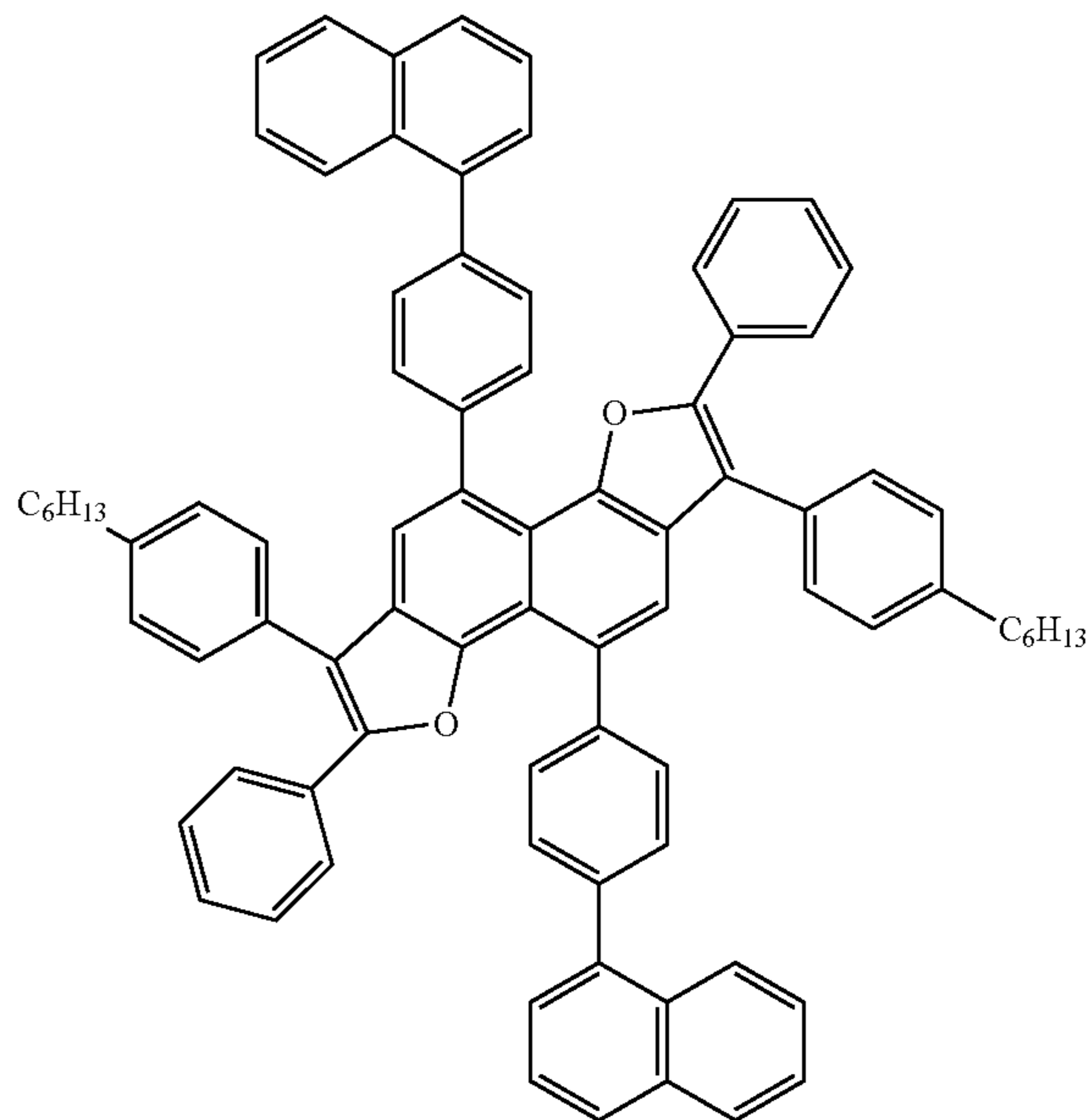
Compound 36
