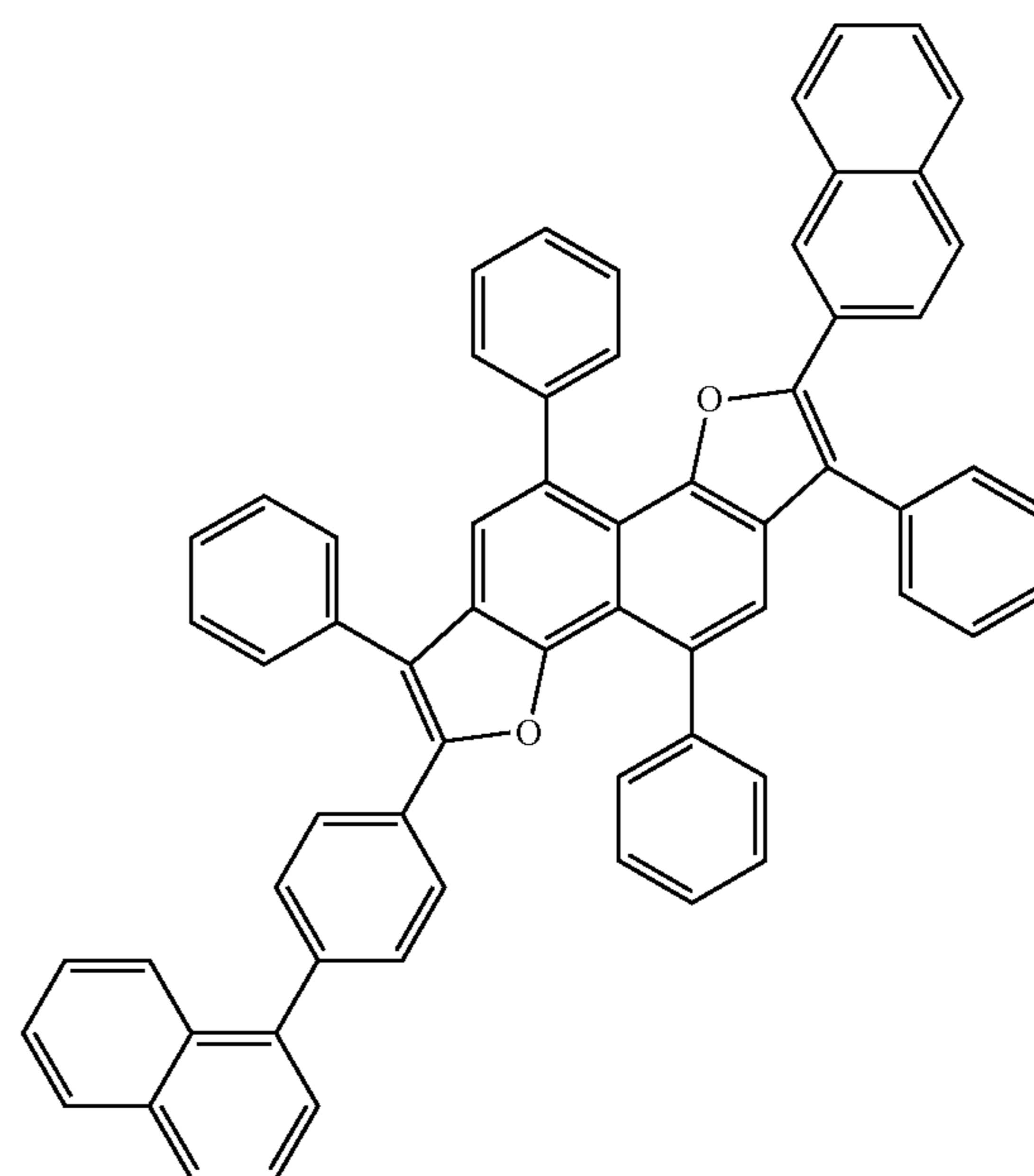
Compound 14
