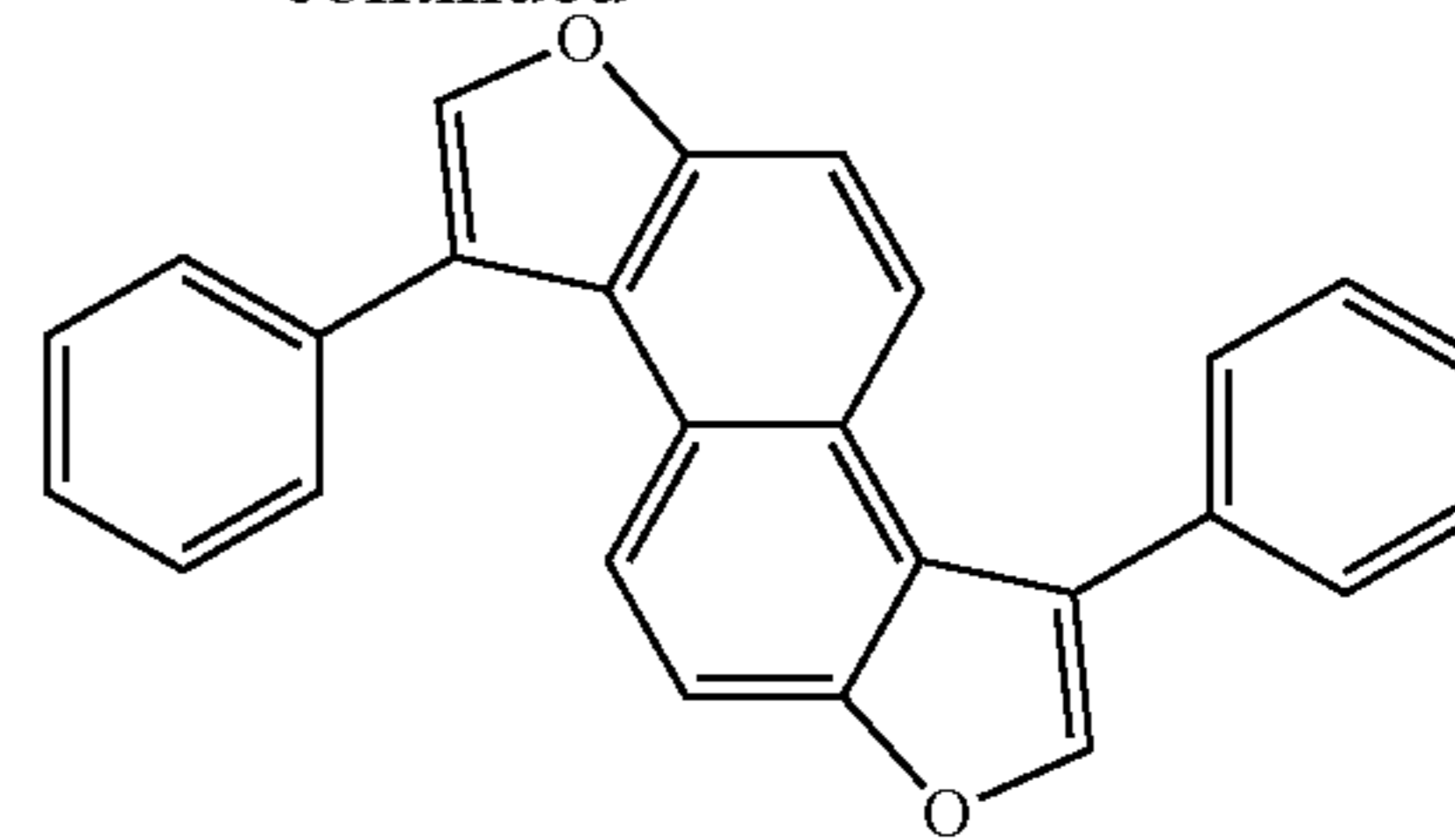
Compound 1
