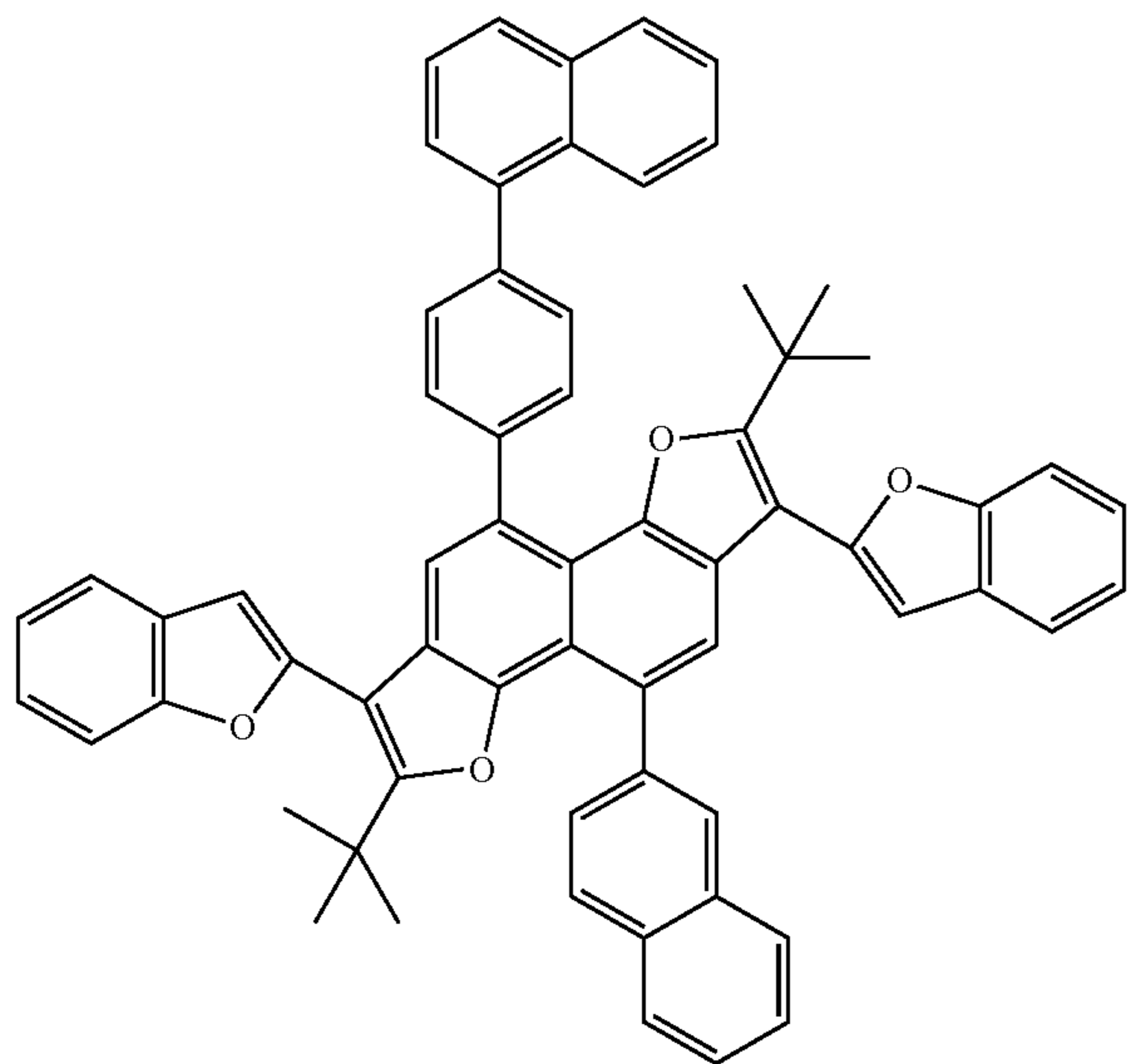
Compound 24
