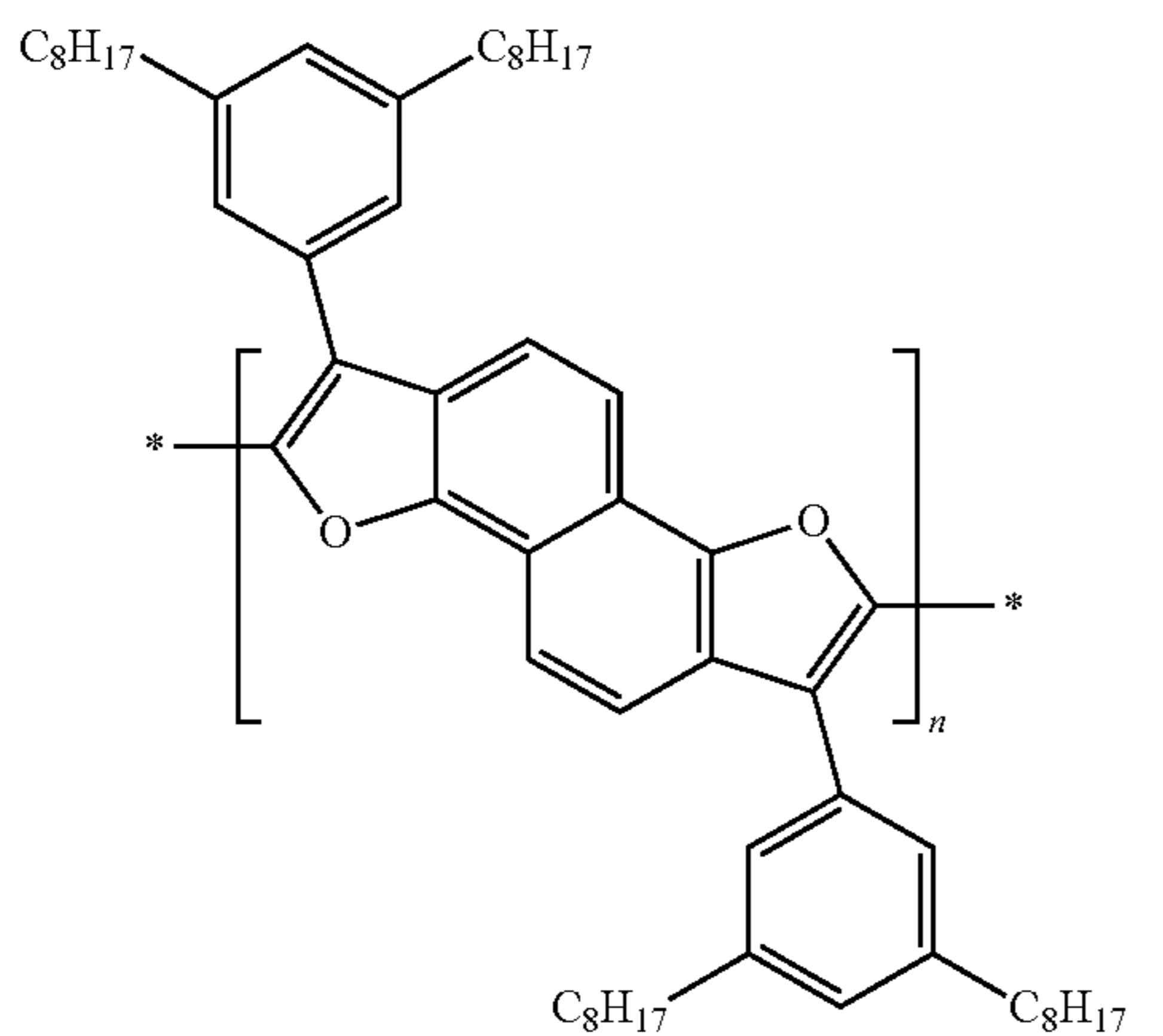
Compound 40
