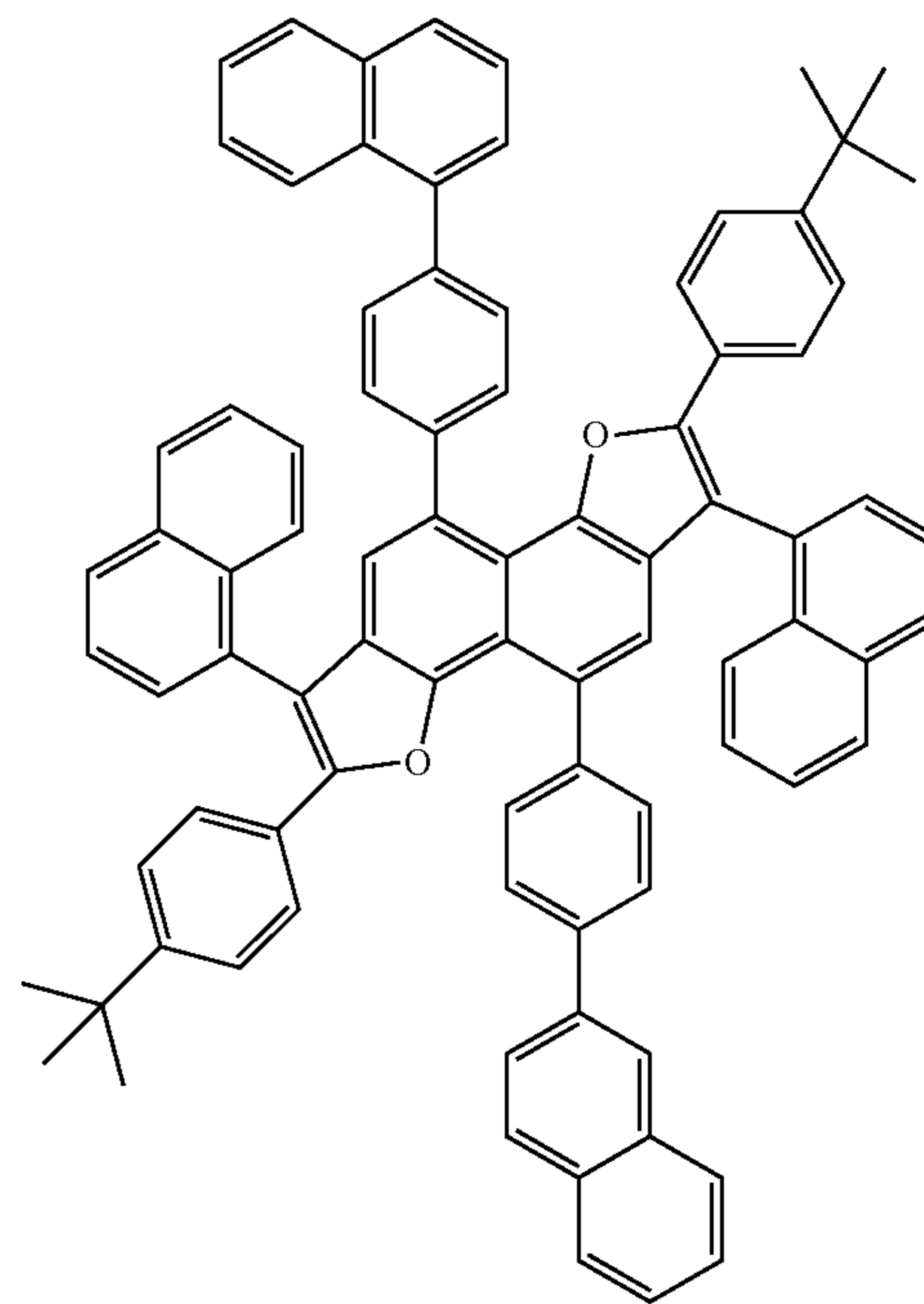
Compound 33
