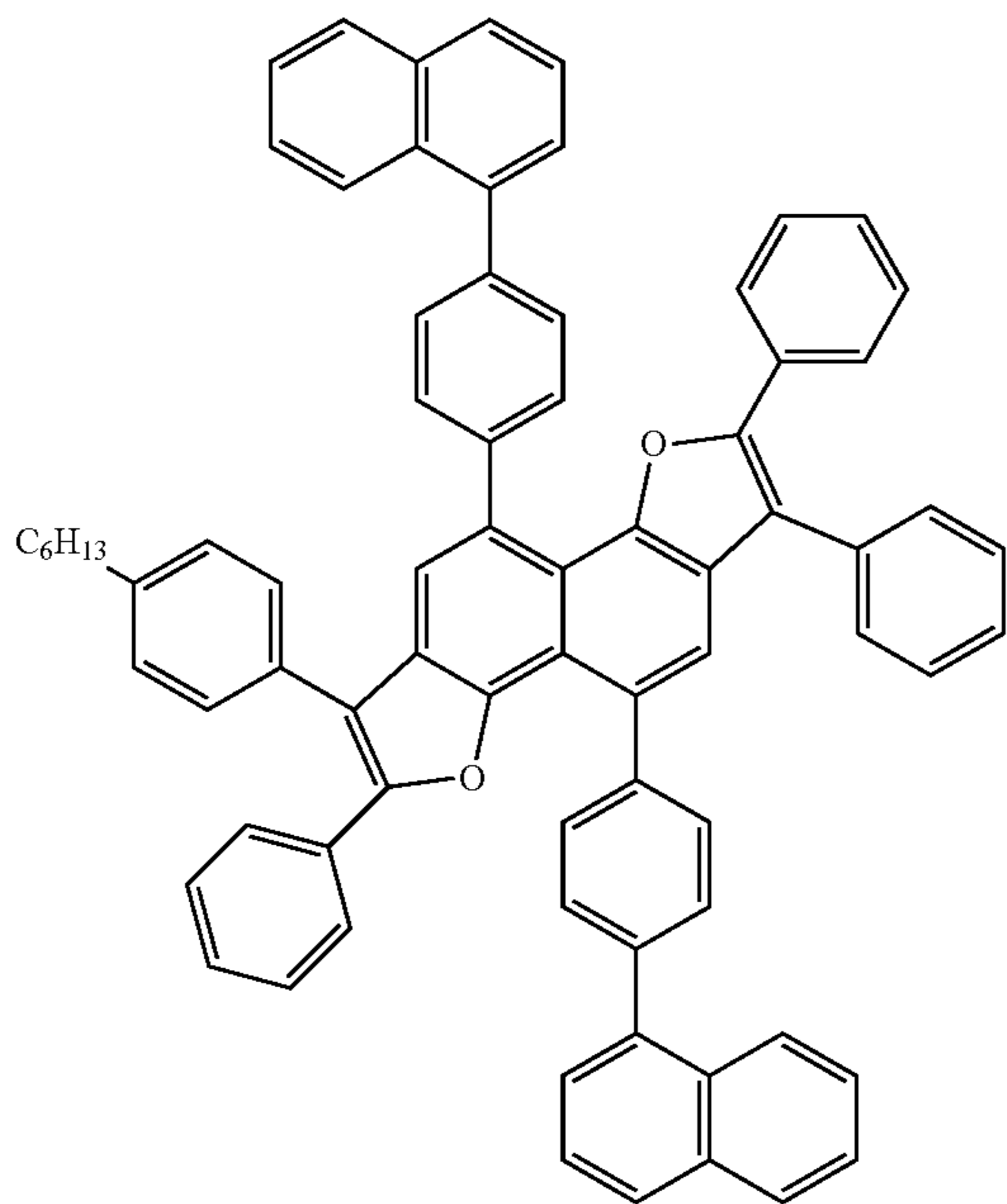
Compound 35
