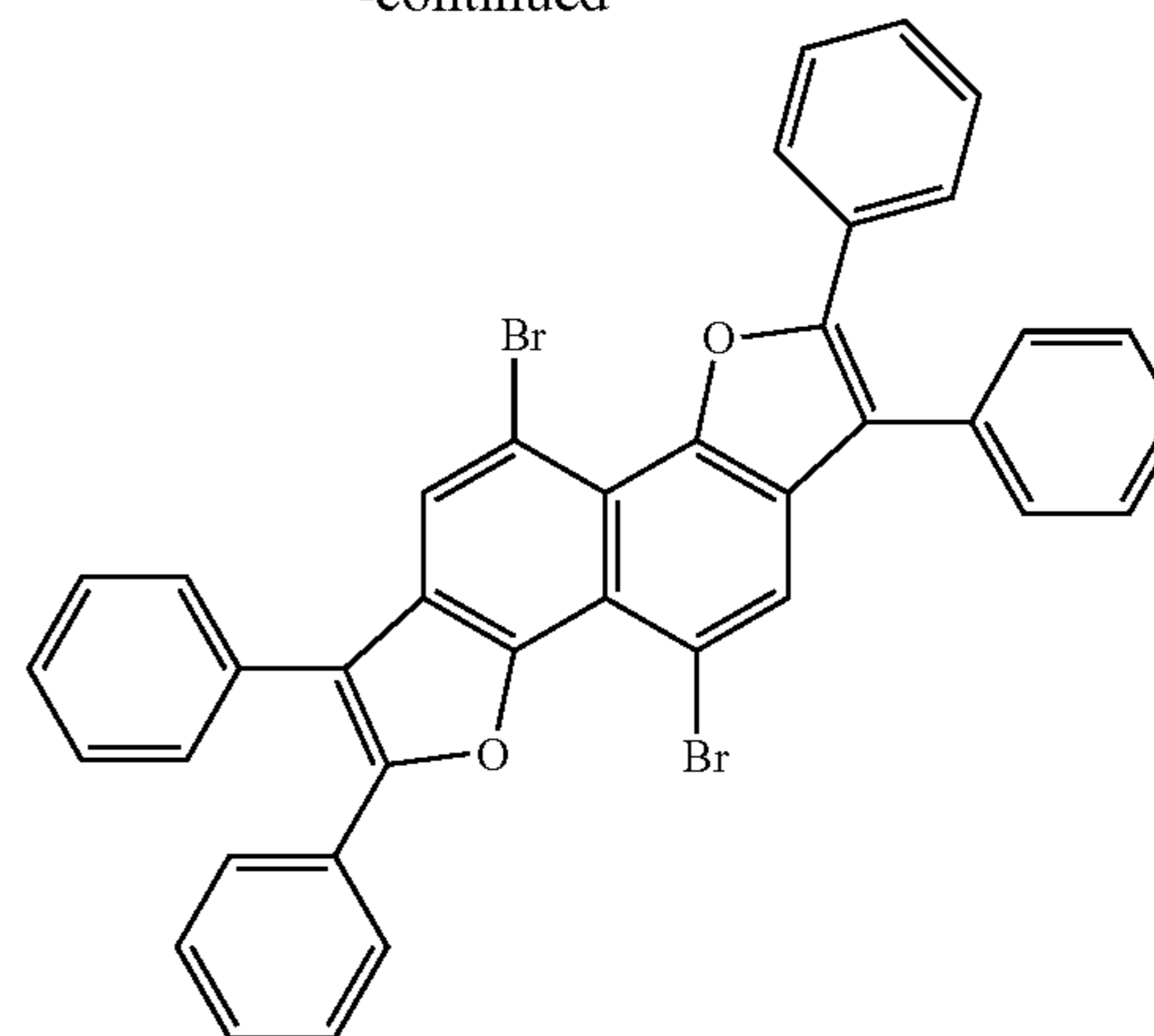
Intermediate C
