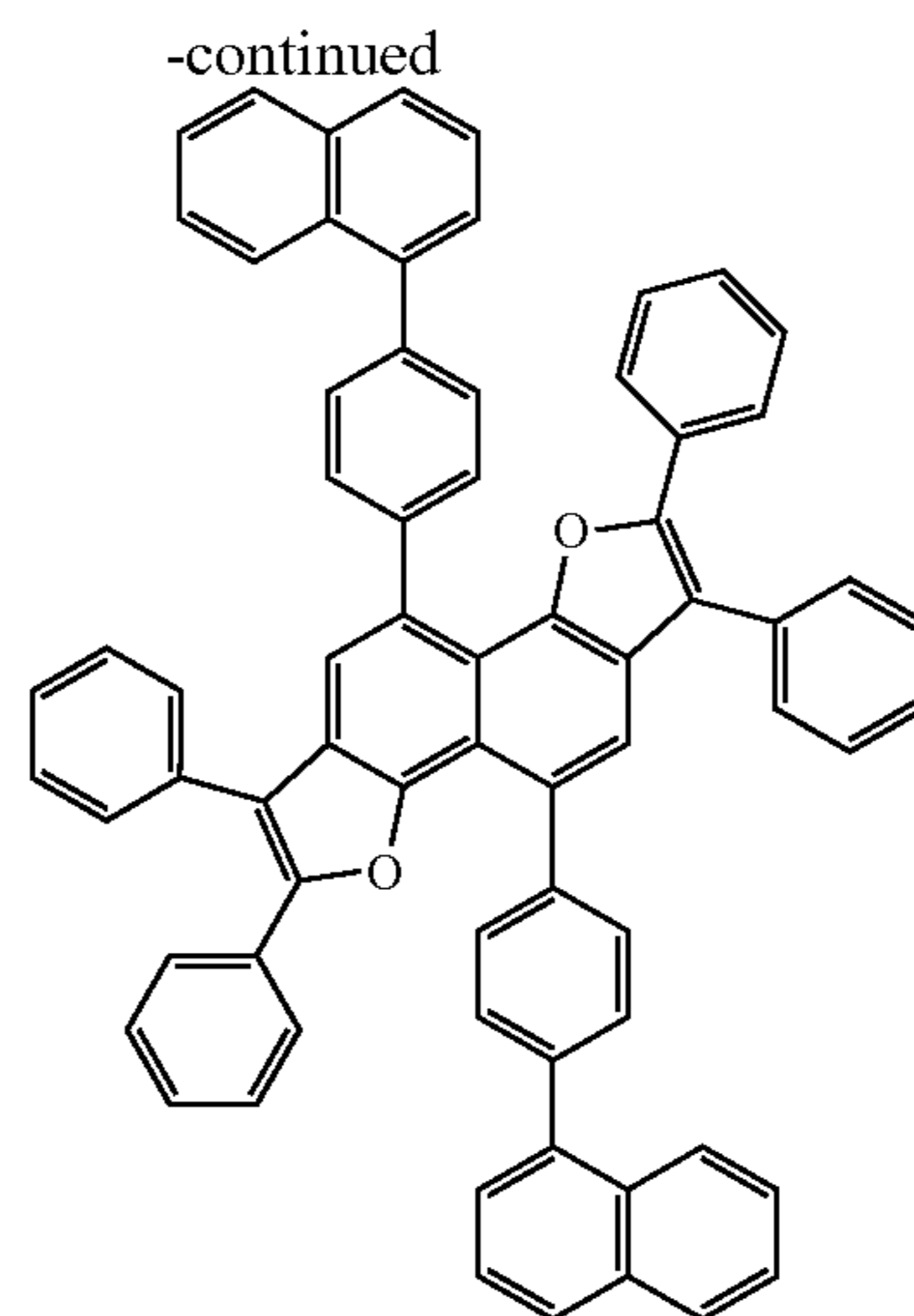
Compound 5
