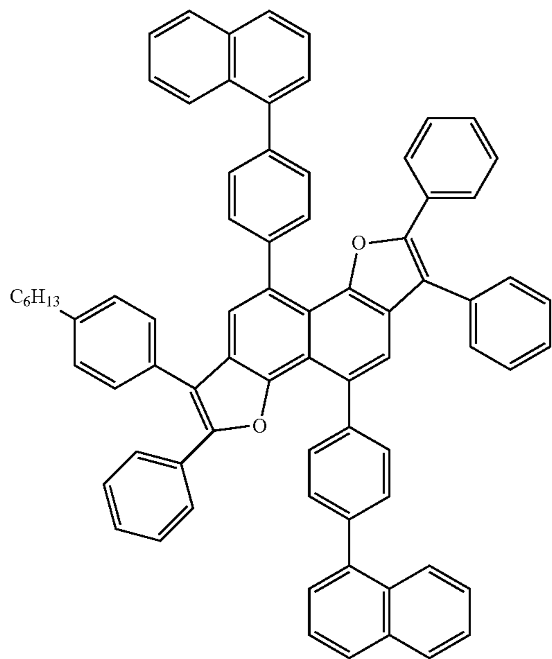
Compound 35
