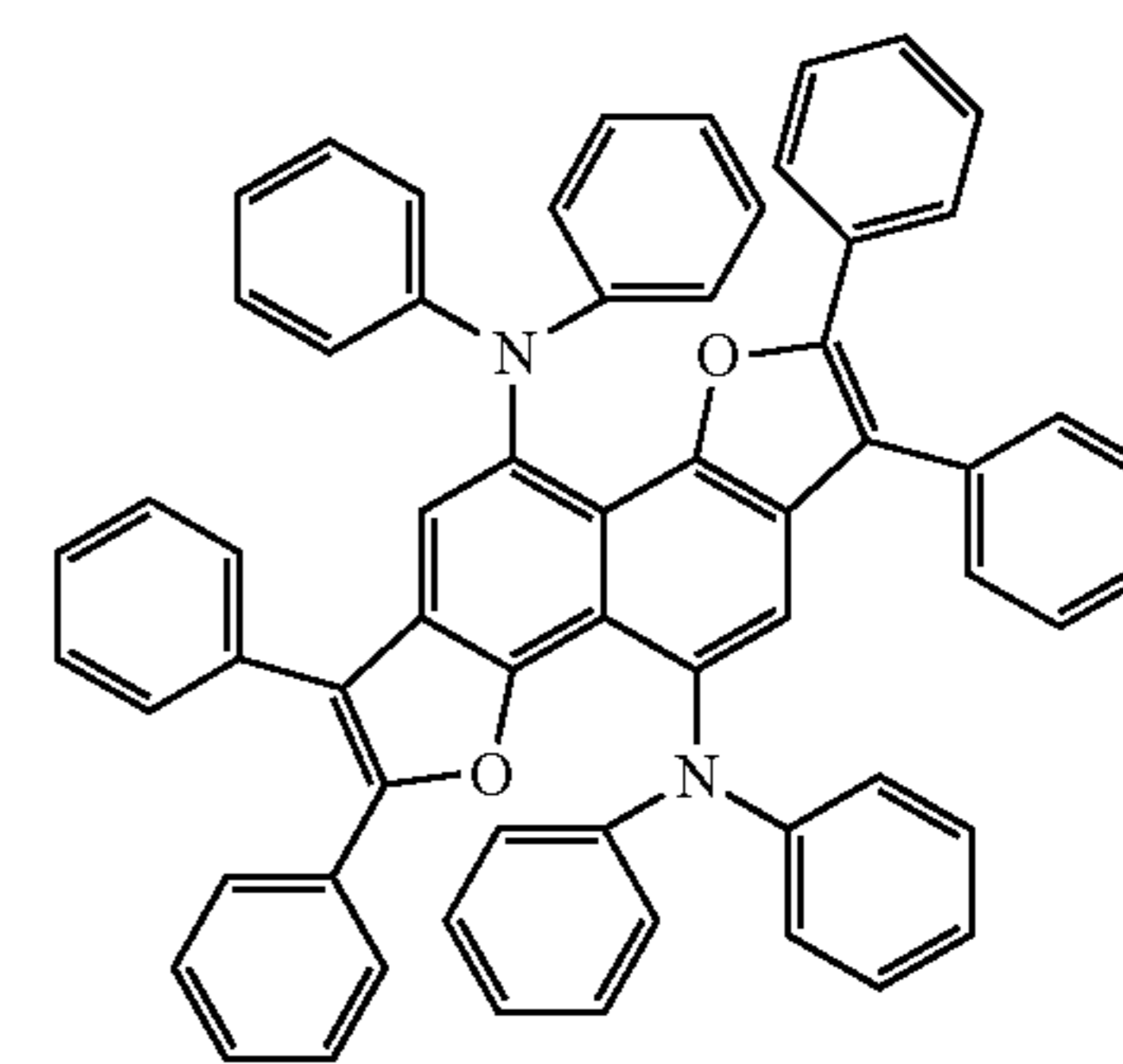
Compound 8
