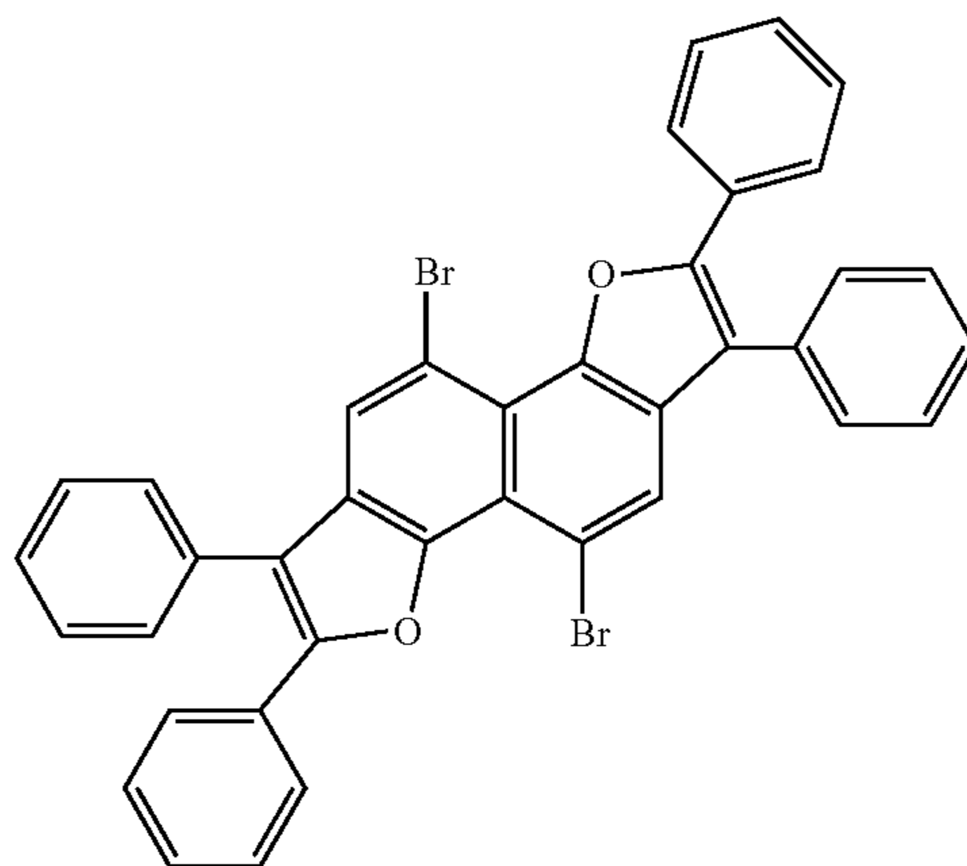
Intermediate C
