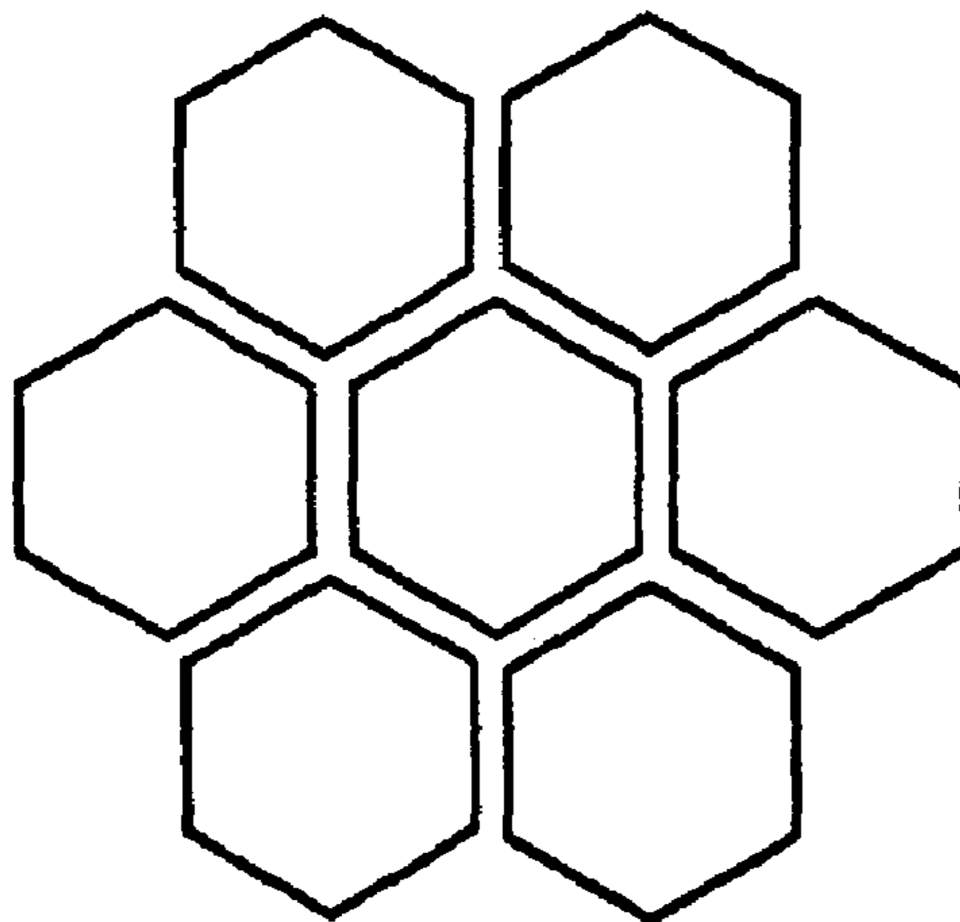
API structure
