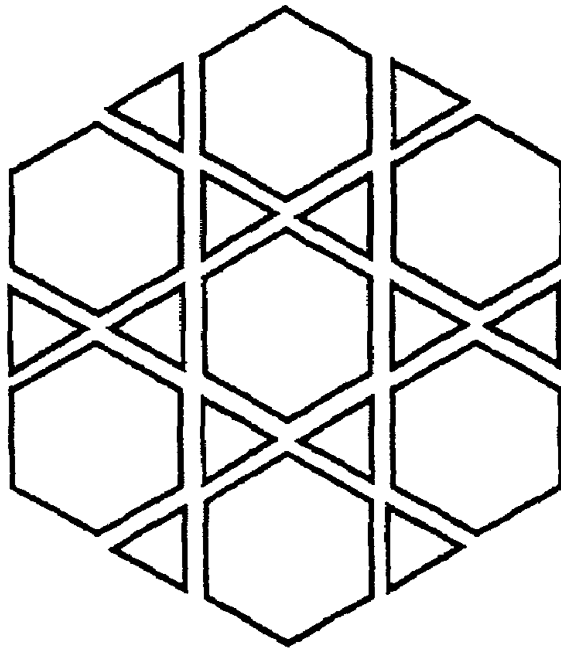
1:2 API:guest co-crystal
