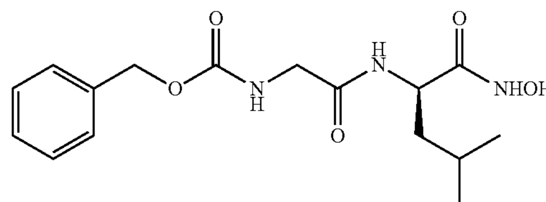
N-Cbz-Gly-Leu-NHOH
