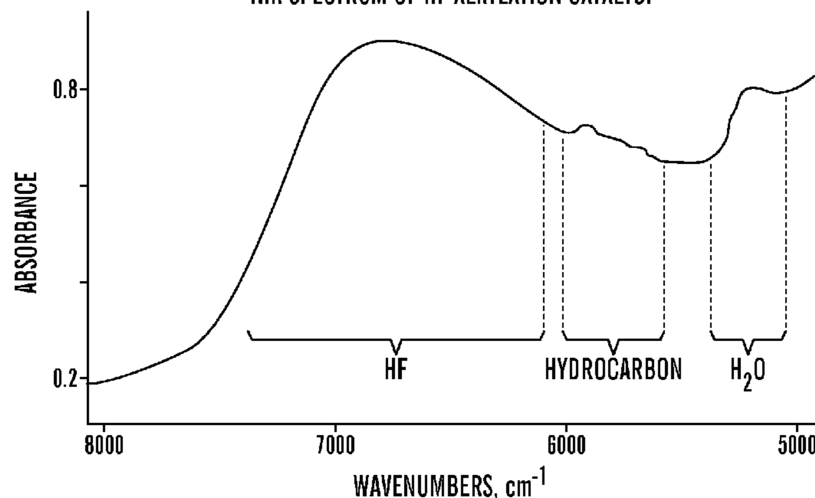
NIR SPECTRUM OF HF ALKYLATION CATALYST
